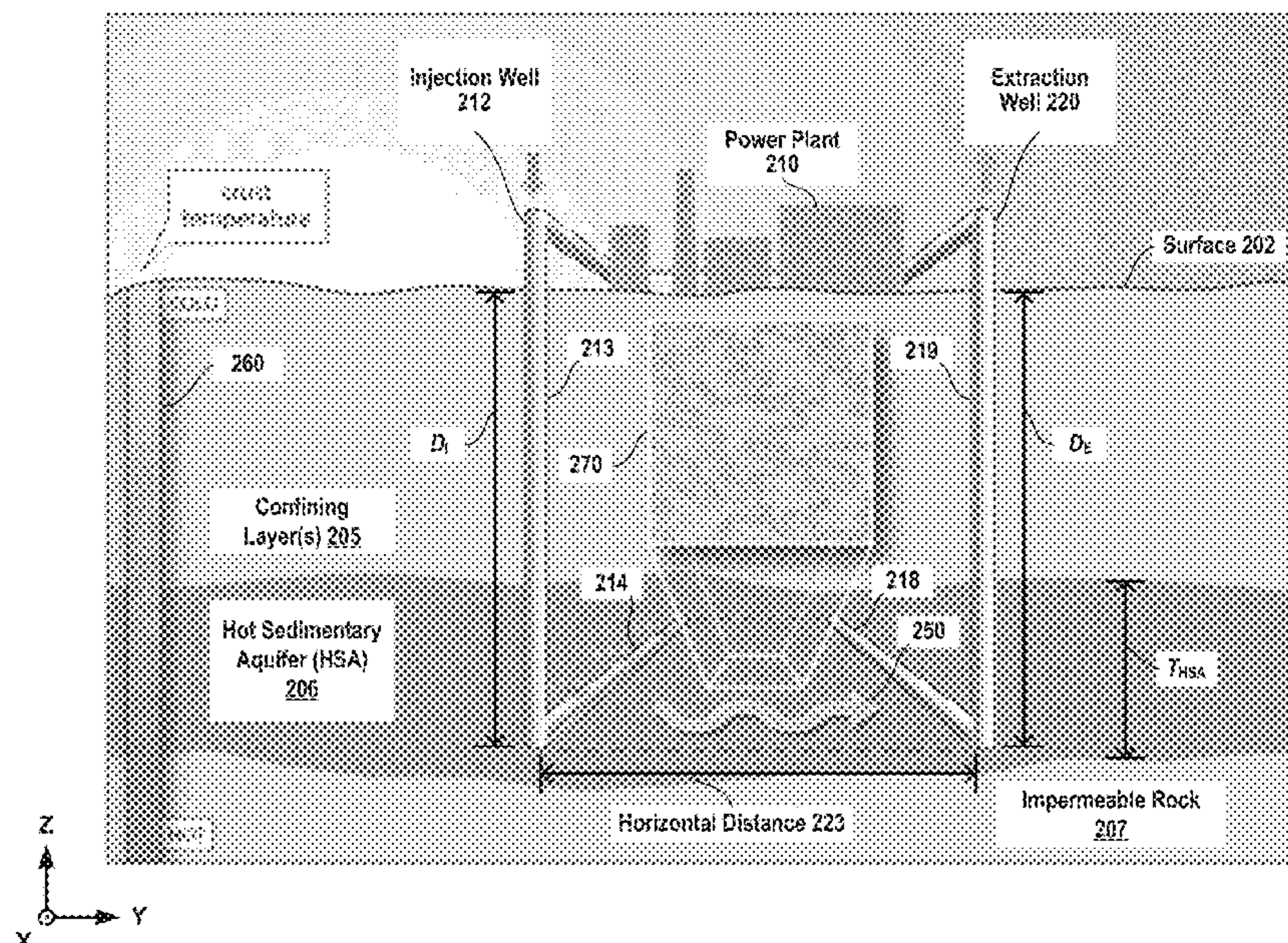
Natural Enhanced Geothermal System (NAT-EGS) 200
