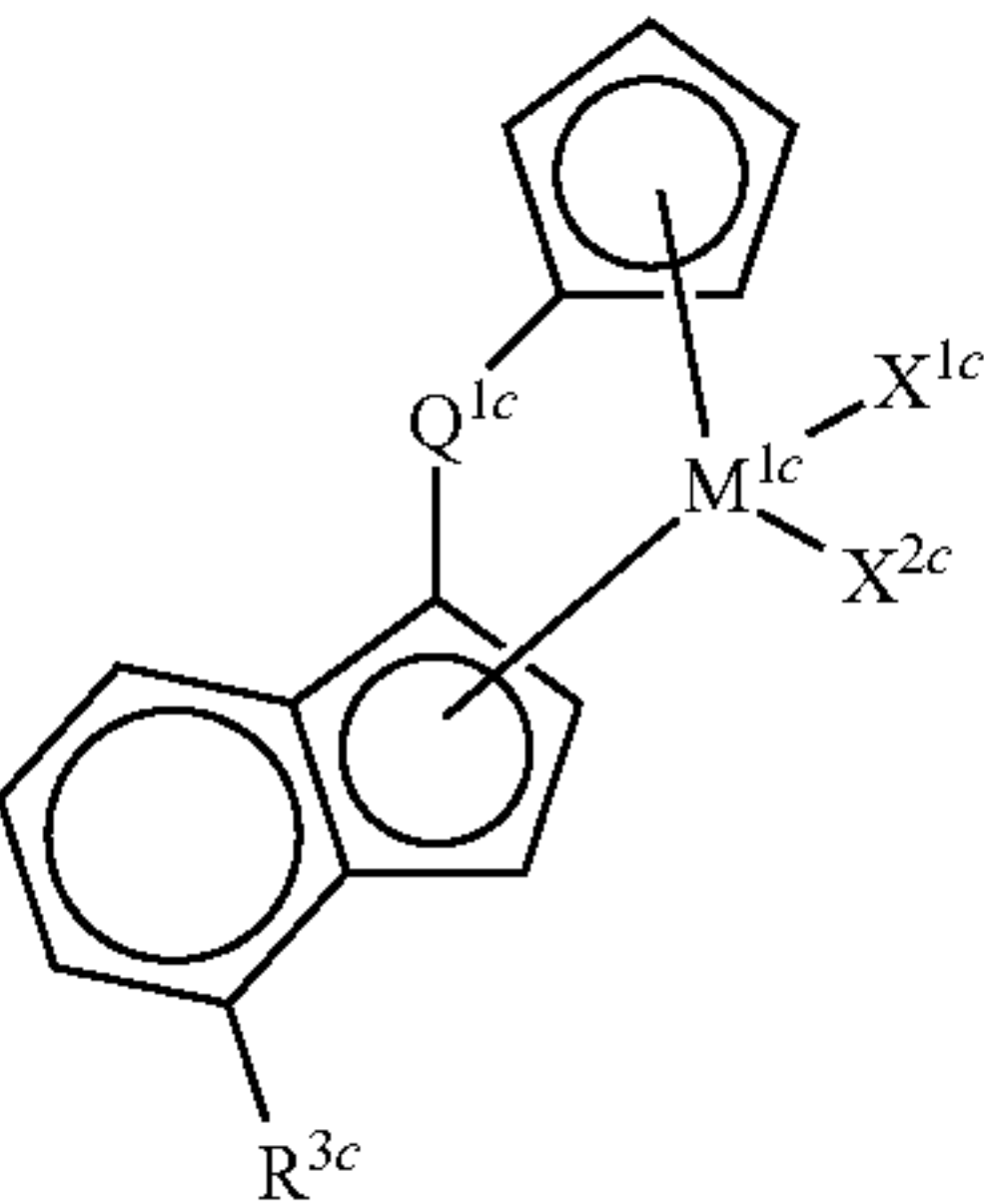
[Chem. 28]
