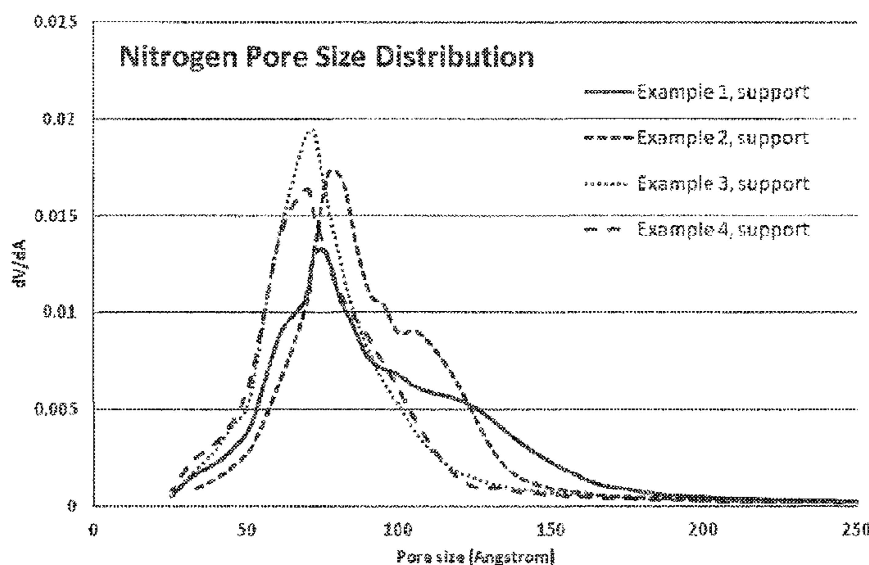
Nitrogen pore size distribution of Examples 1 - 4.
