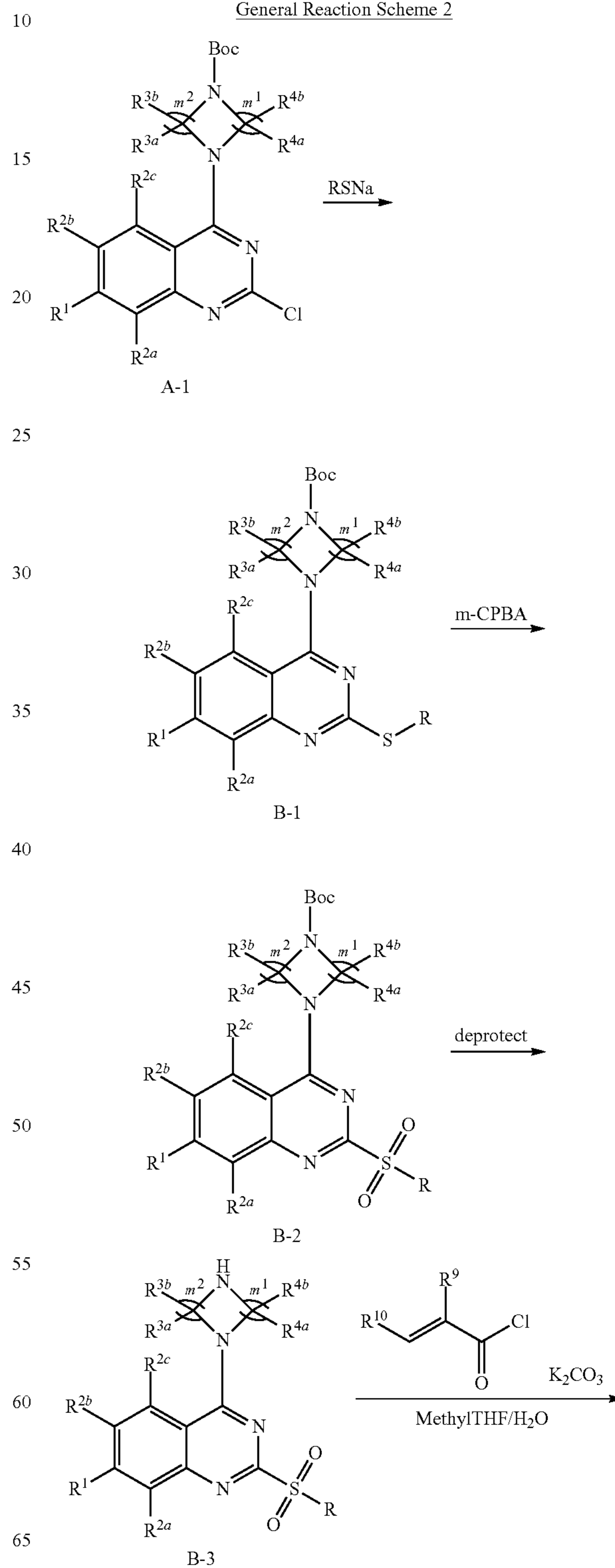
General Reaction Scheme 2
