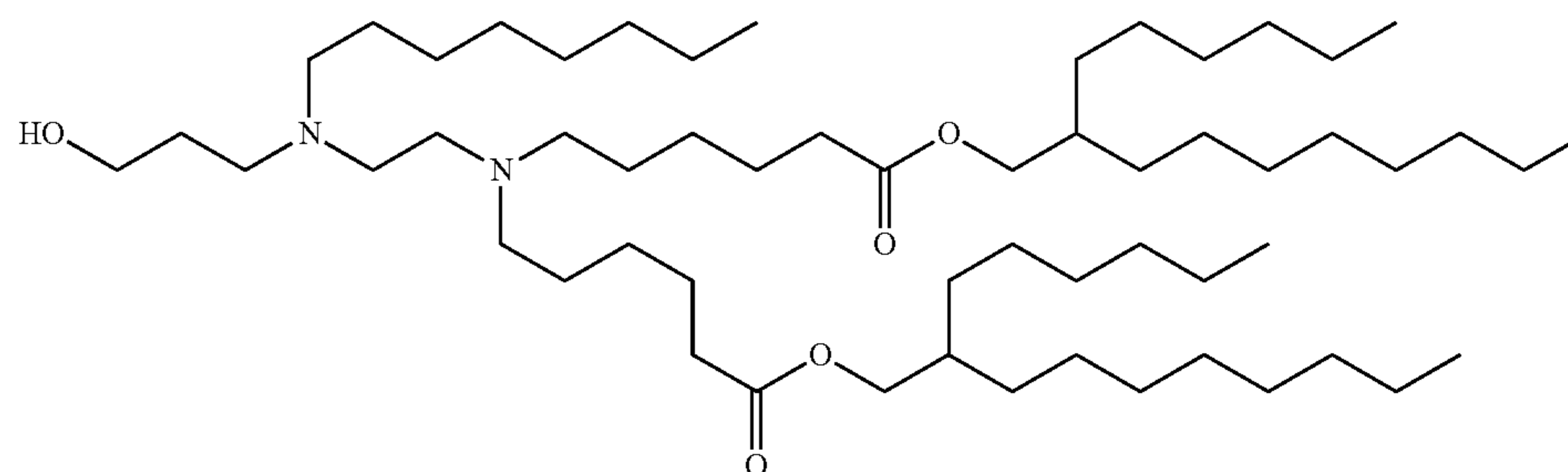
Compound 2
