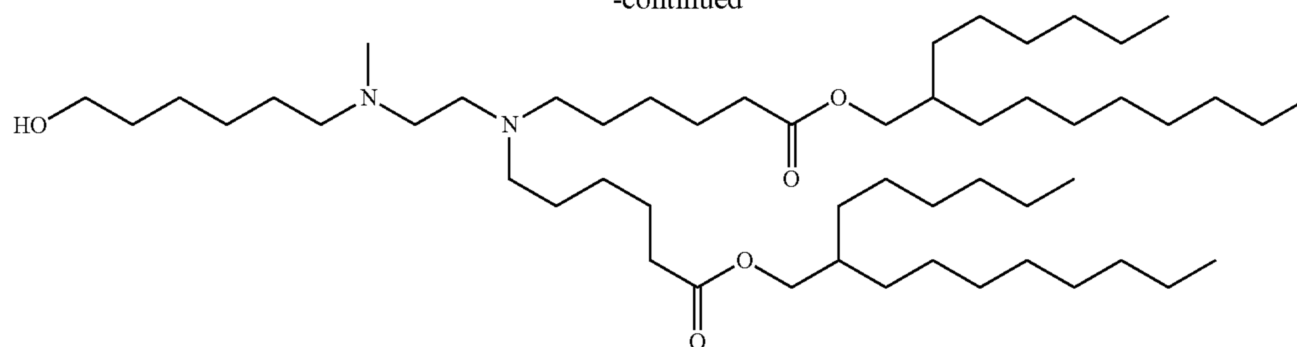
Compound 7
