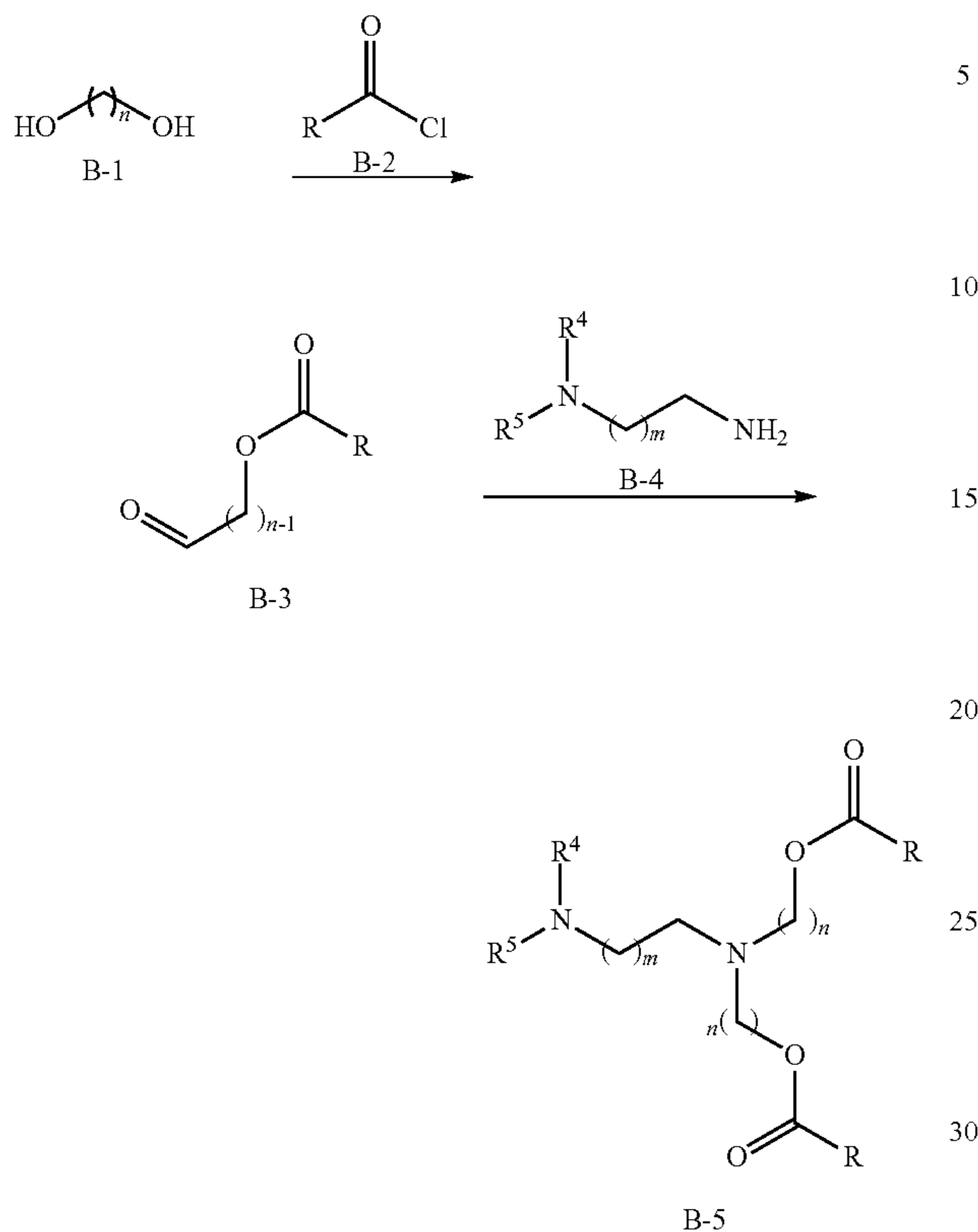
GENERAL REACTION SCHEME 2
