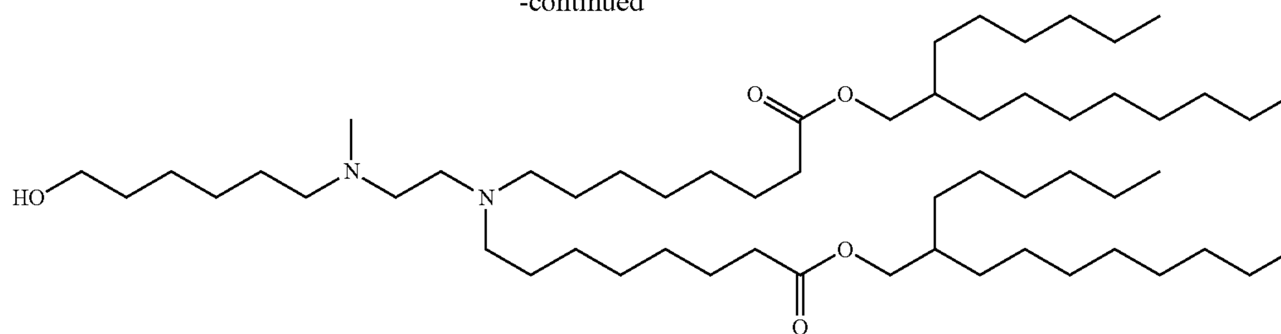
Compound 9
