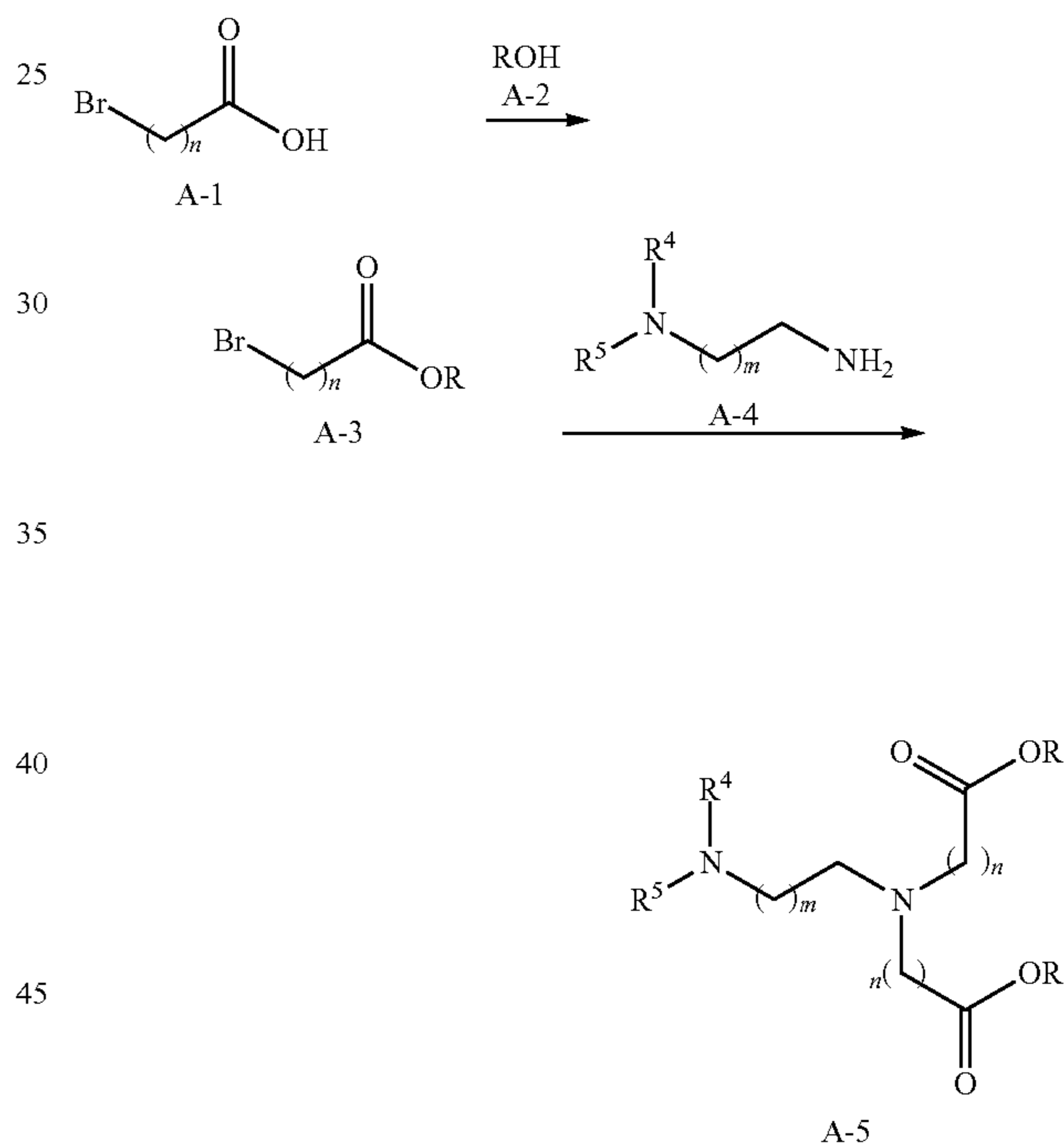
GENERAL REACTION SCHEME 1
