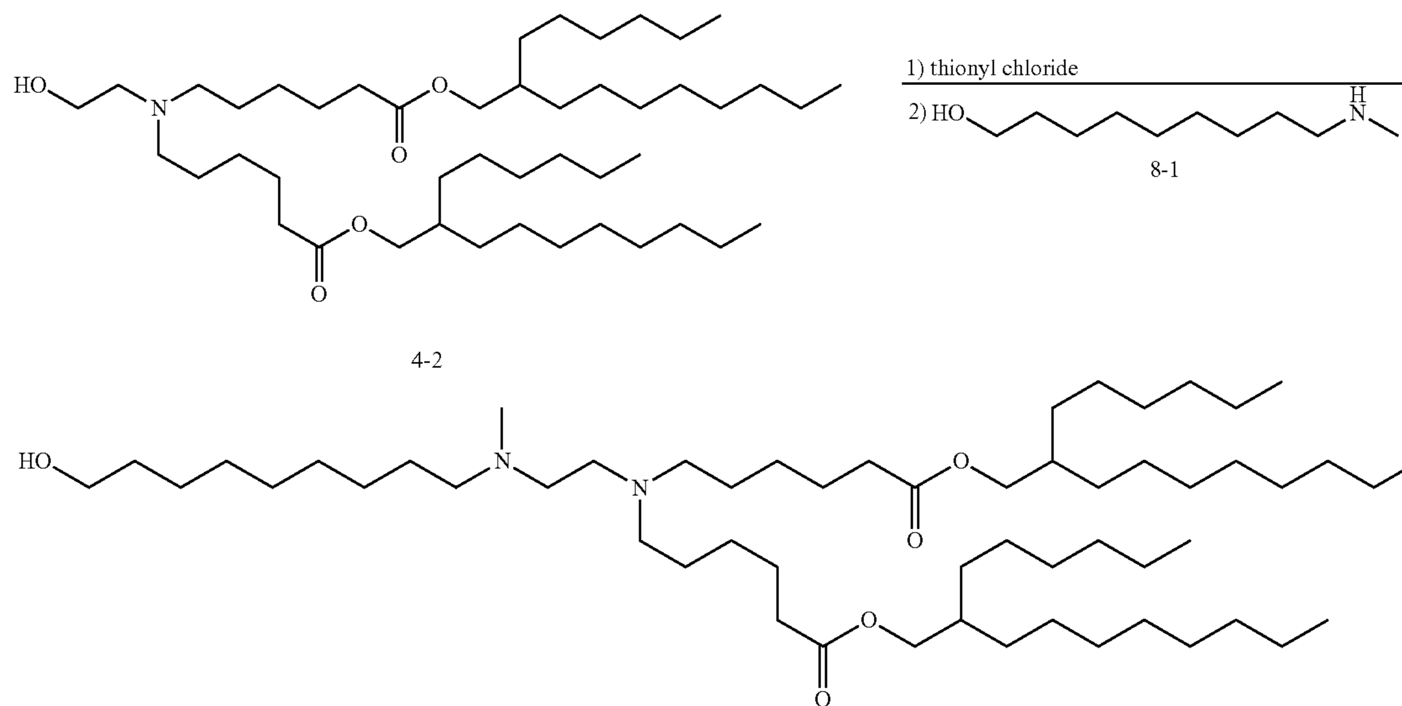
Compound 5
