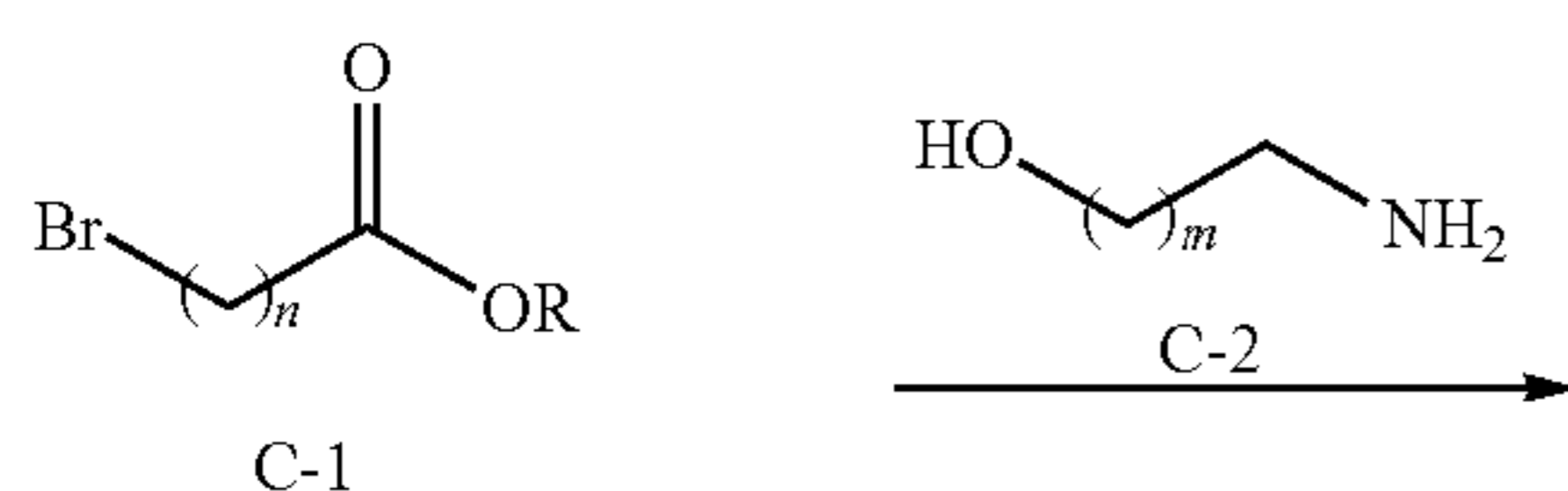
GENERAL REACTION SCHEME 3
