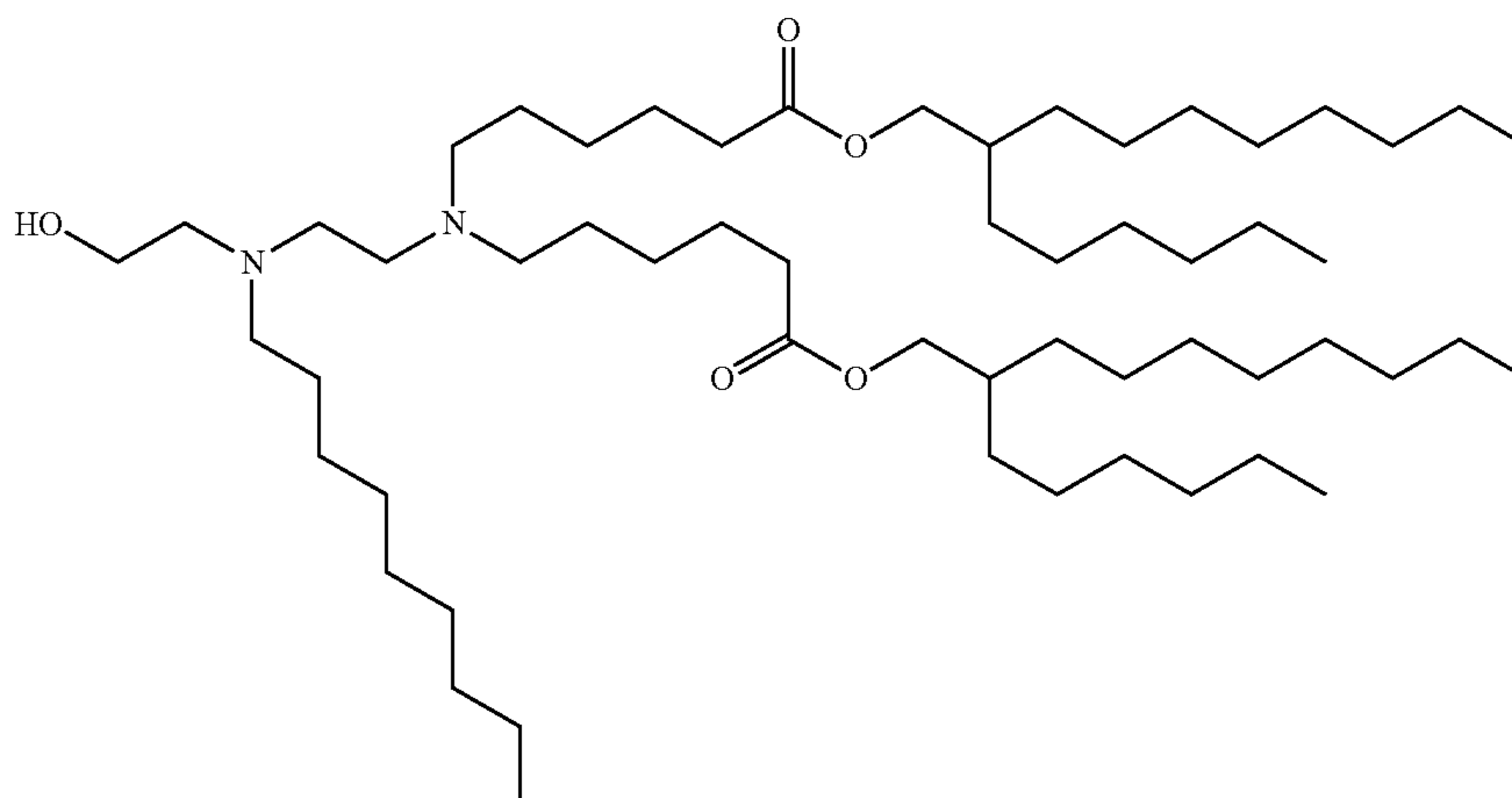
Structure
