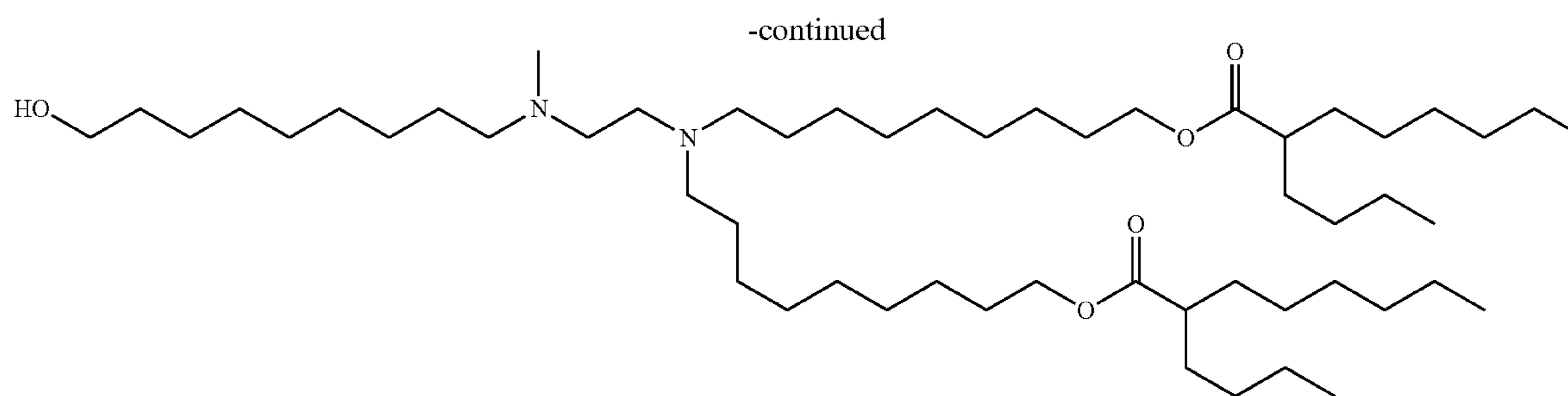
Compound 8
