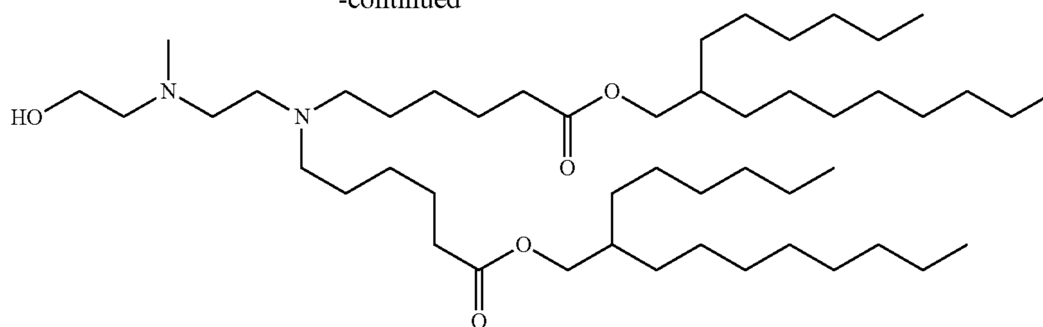
Compound 4
