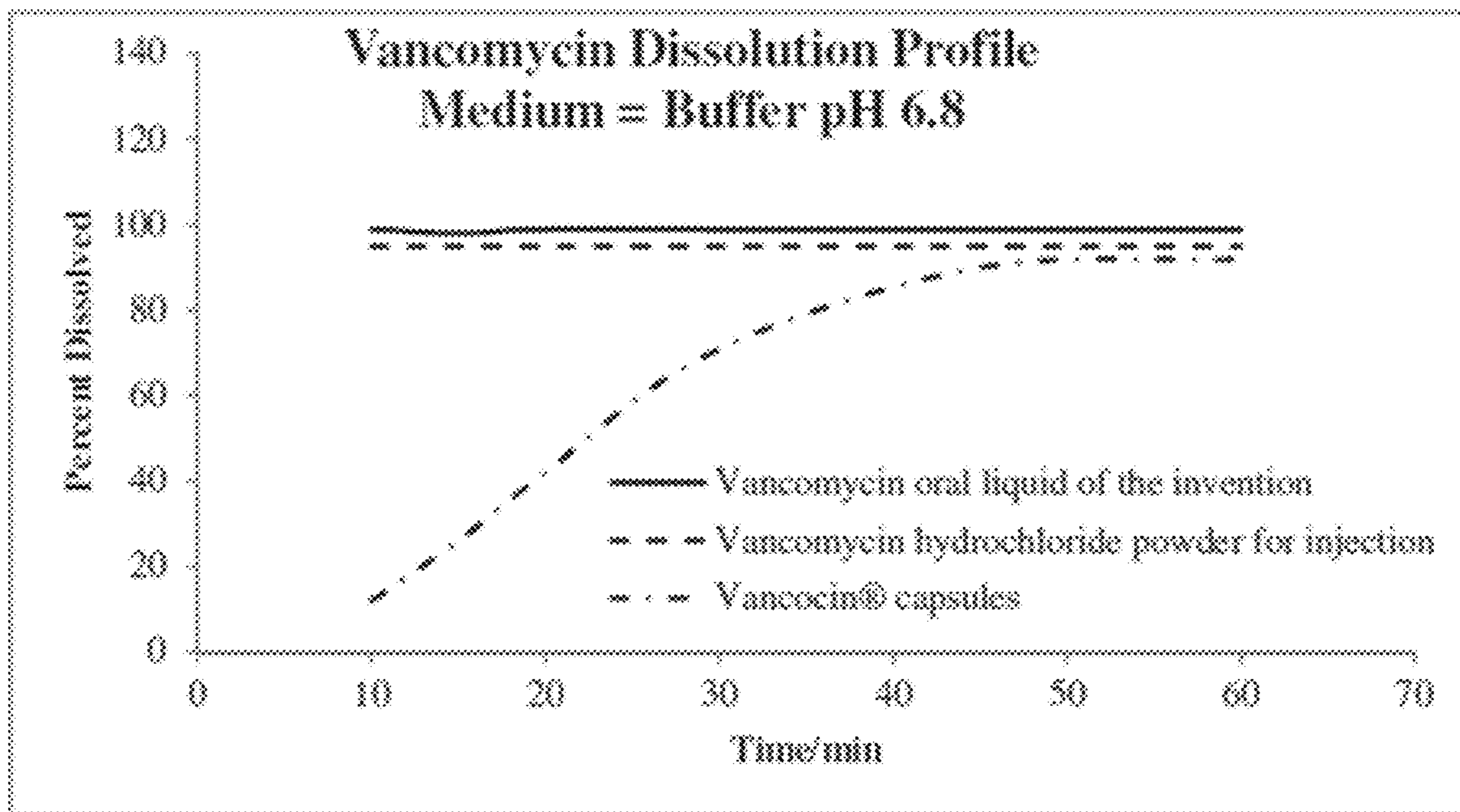
FIG. 5 Vancomycin Dissolution Profile in Buffer pH 6.8
