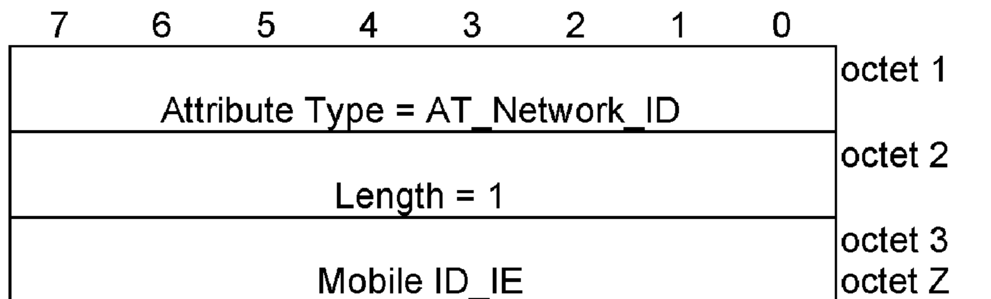
Figure 8.2.X.3-1: AT_ME_ID attribute_RESP
