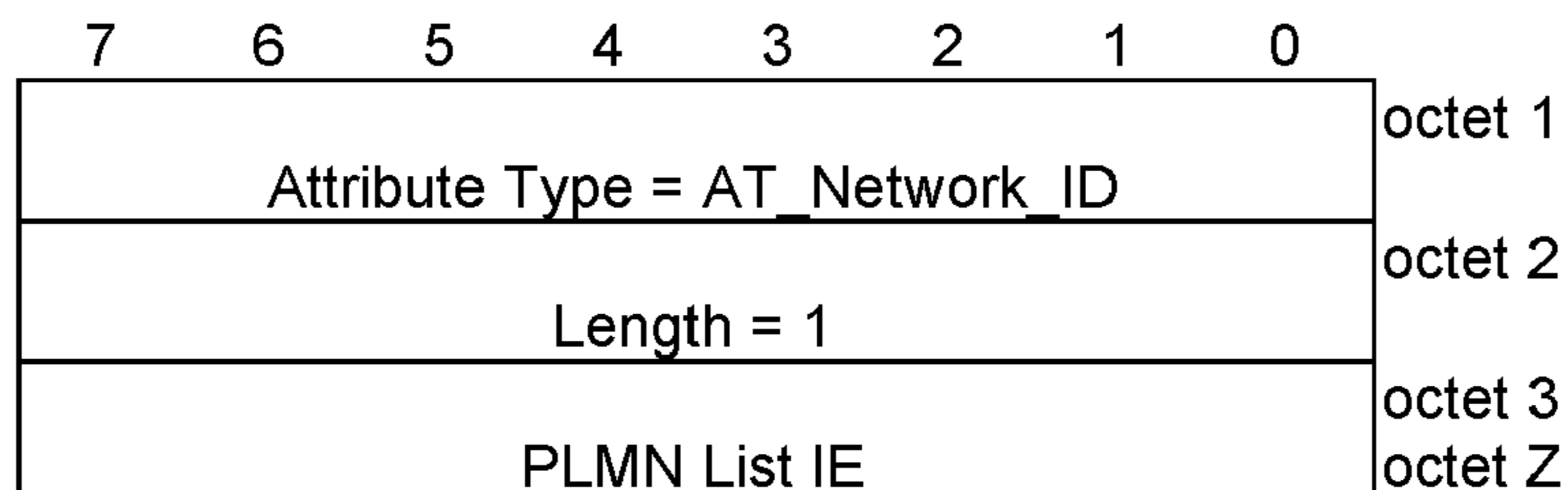
Figure 8.2.X.1-1: AT_PLMN_ID attribute_RESP
