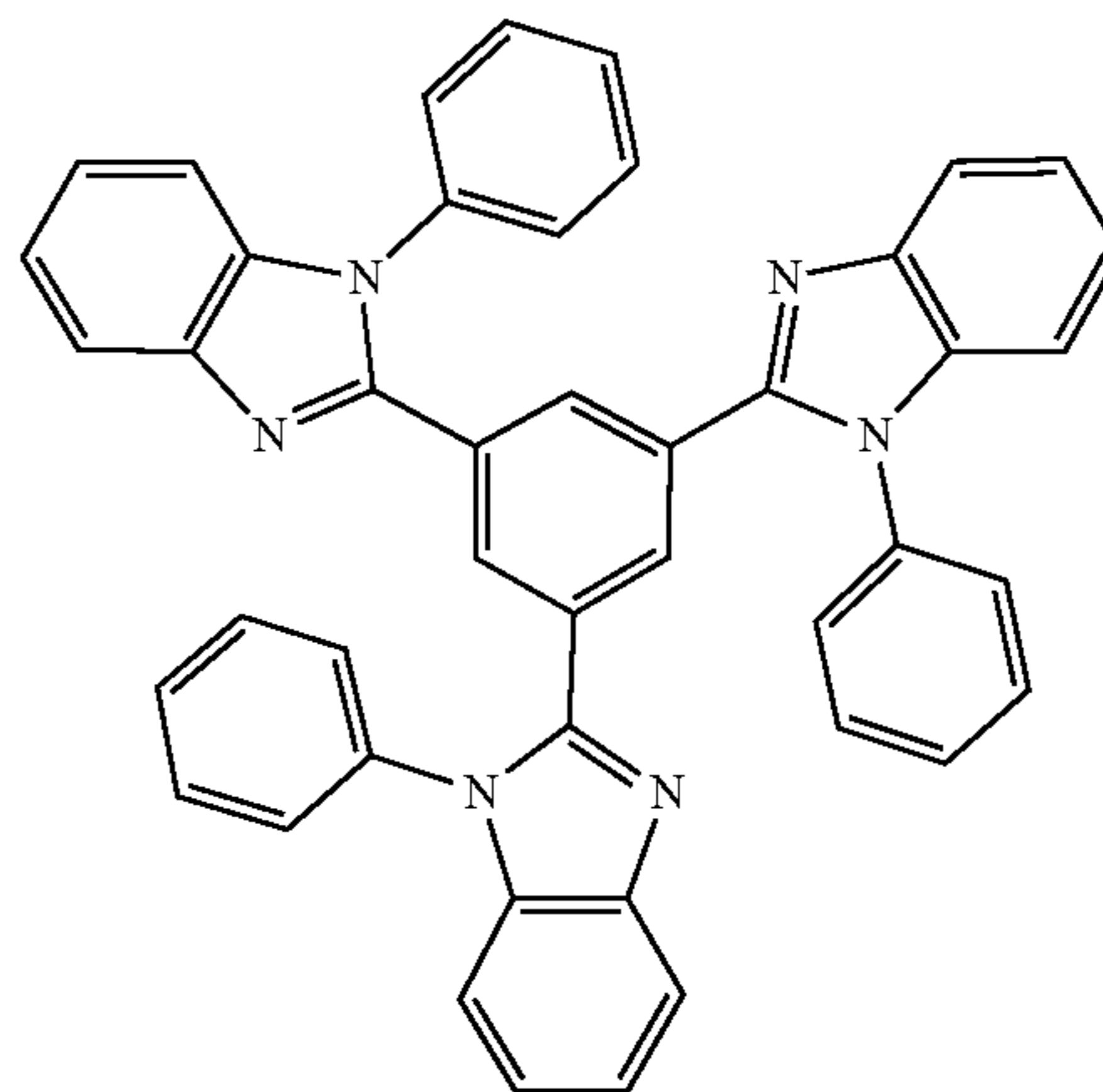
TPBi
