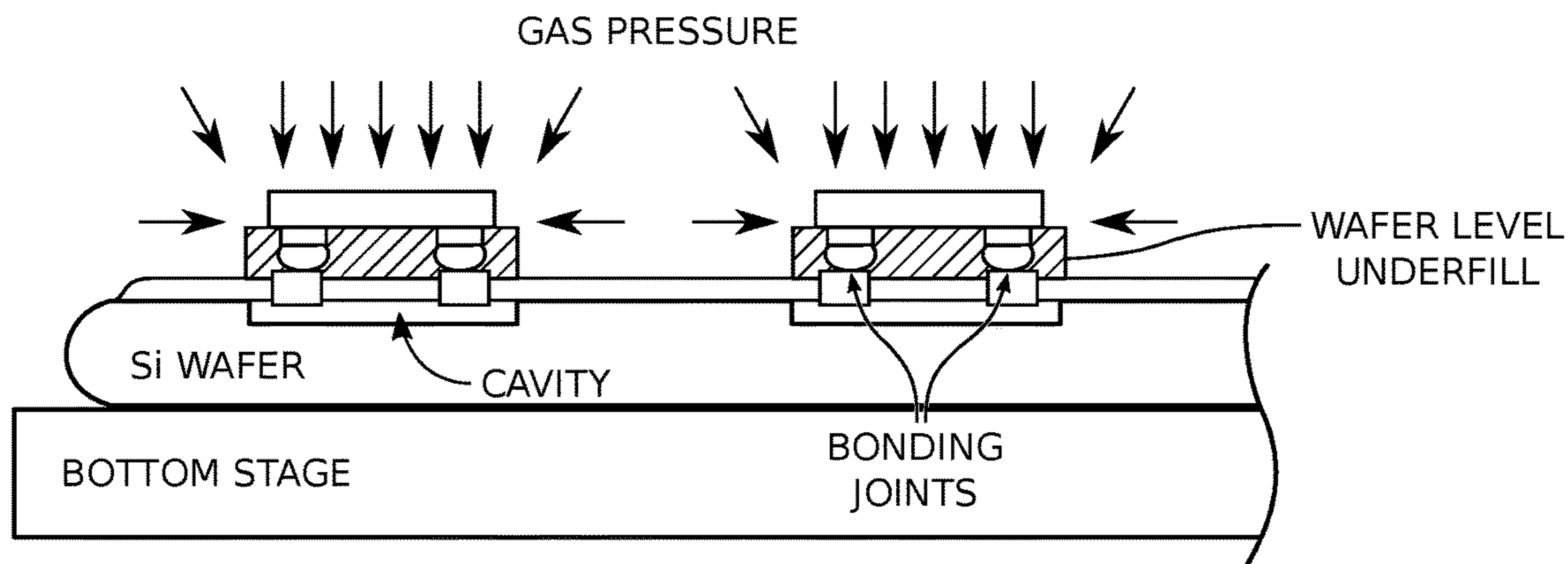
Fig. 4 (PRIOR ART)
