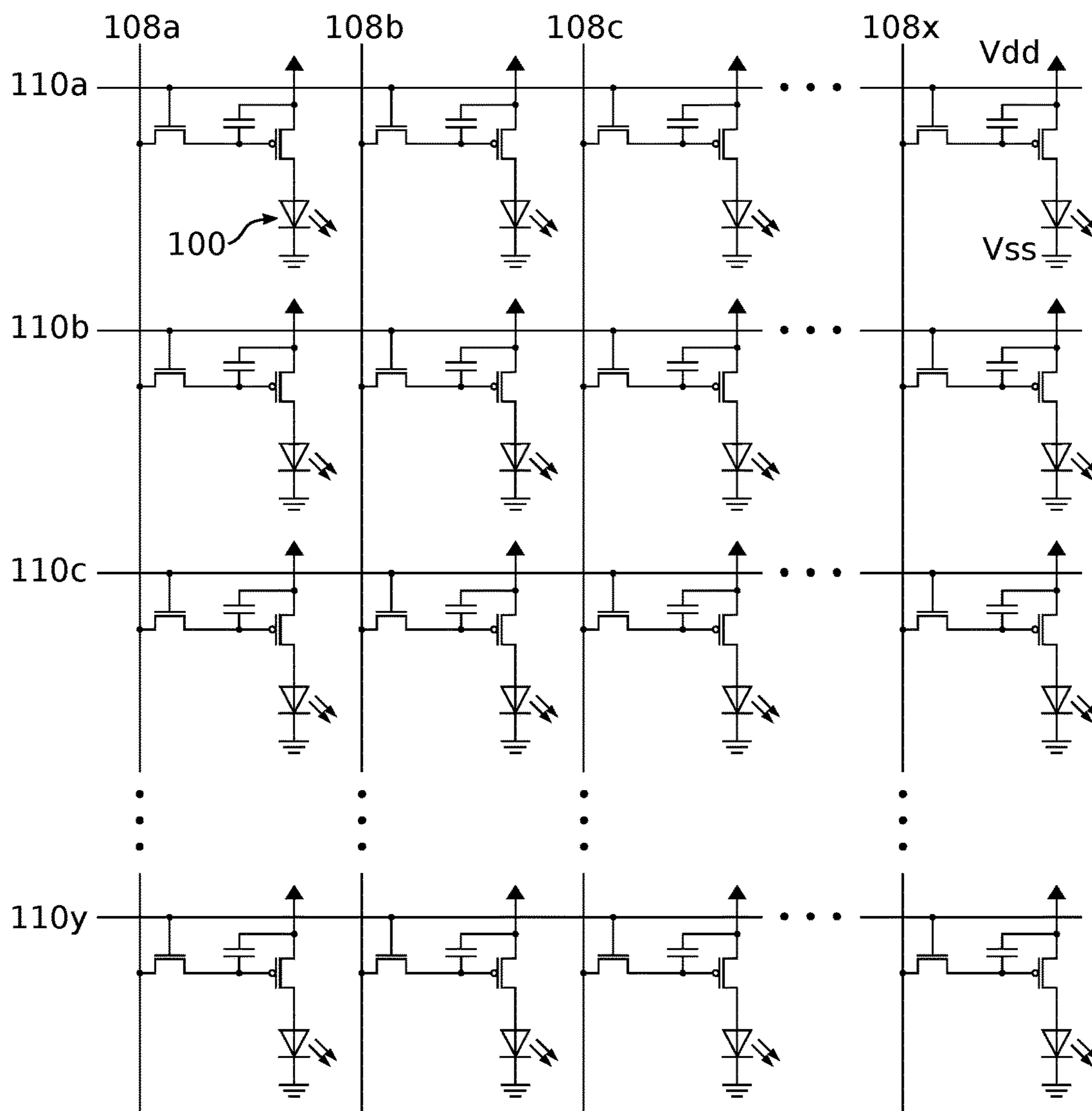
Fig. 2 (PRIOR ART)
