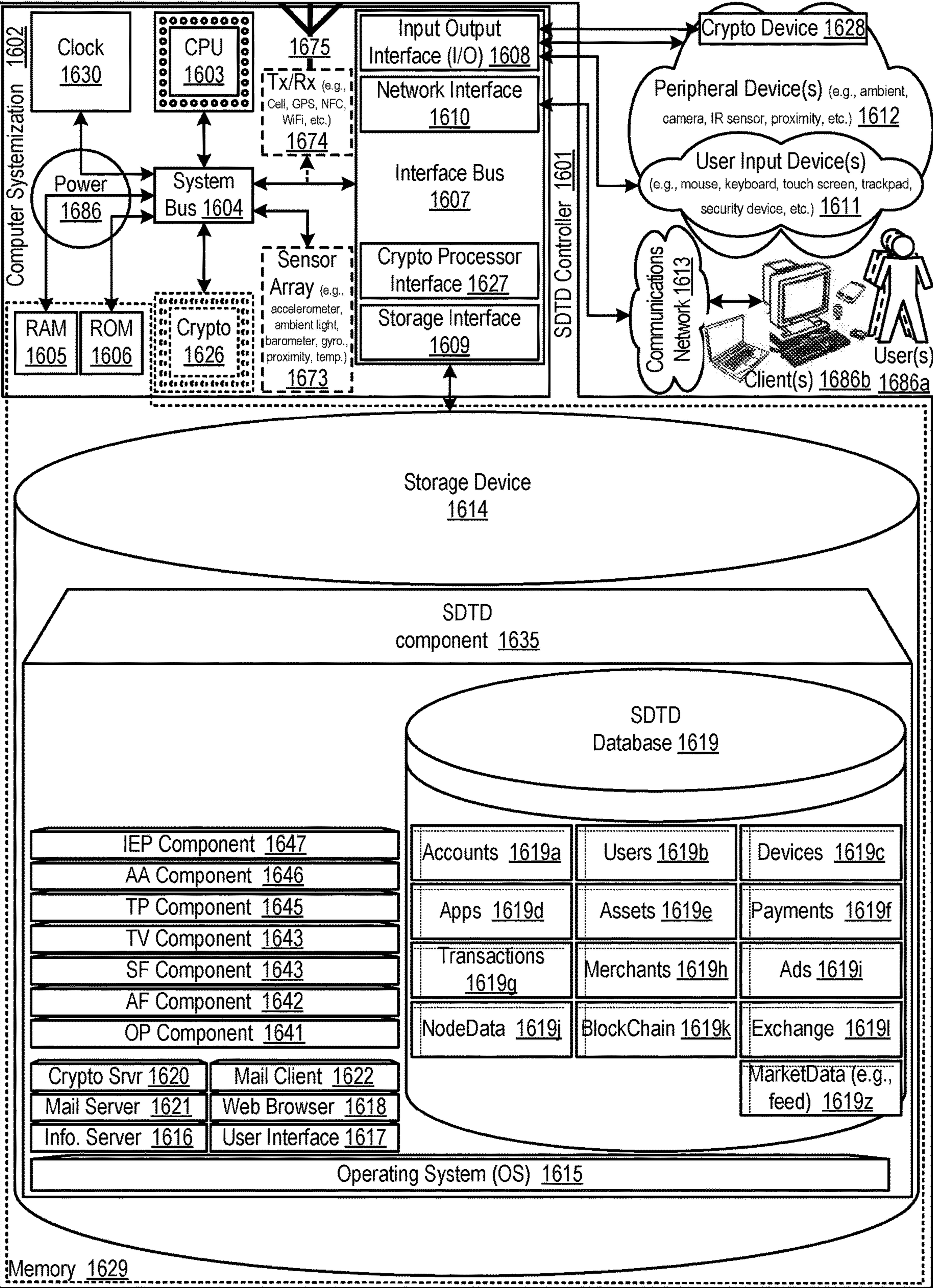
FIGURE 16: SDTD Controller
