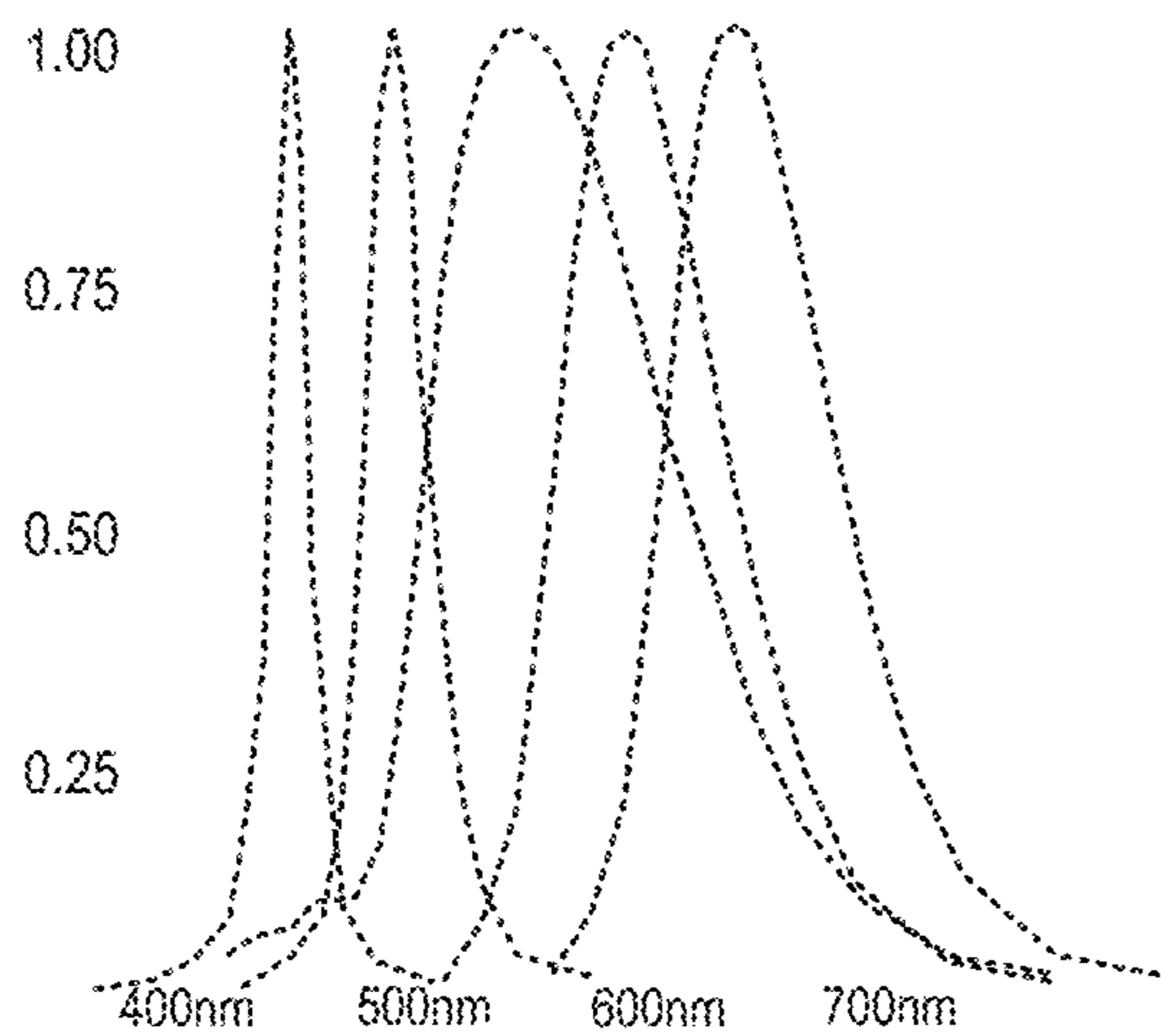
Illuminance Profile for Each Color Channel of Multi-Channel Light Source
