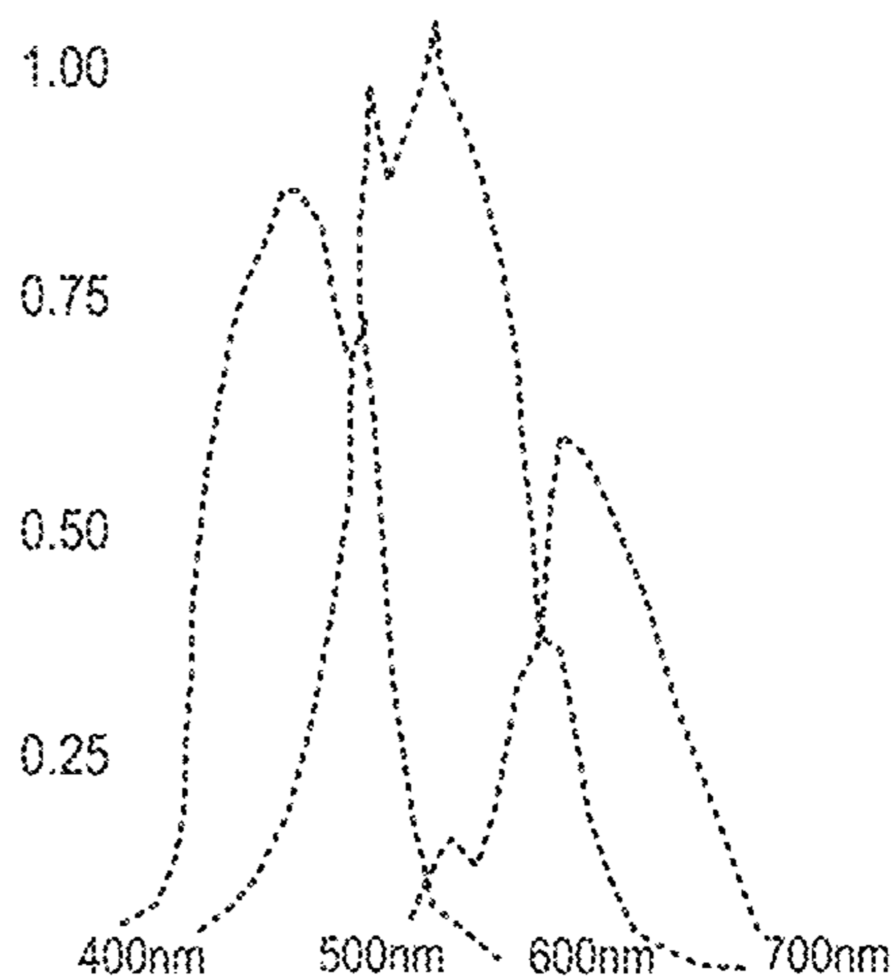
Response Profile for Each Color Channel of Multi-Channel Image Sensor
