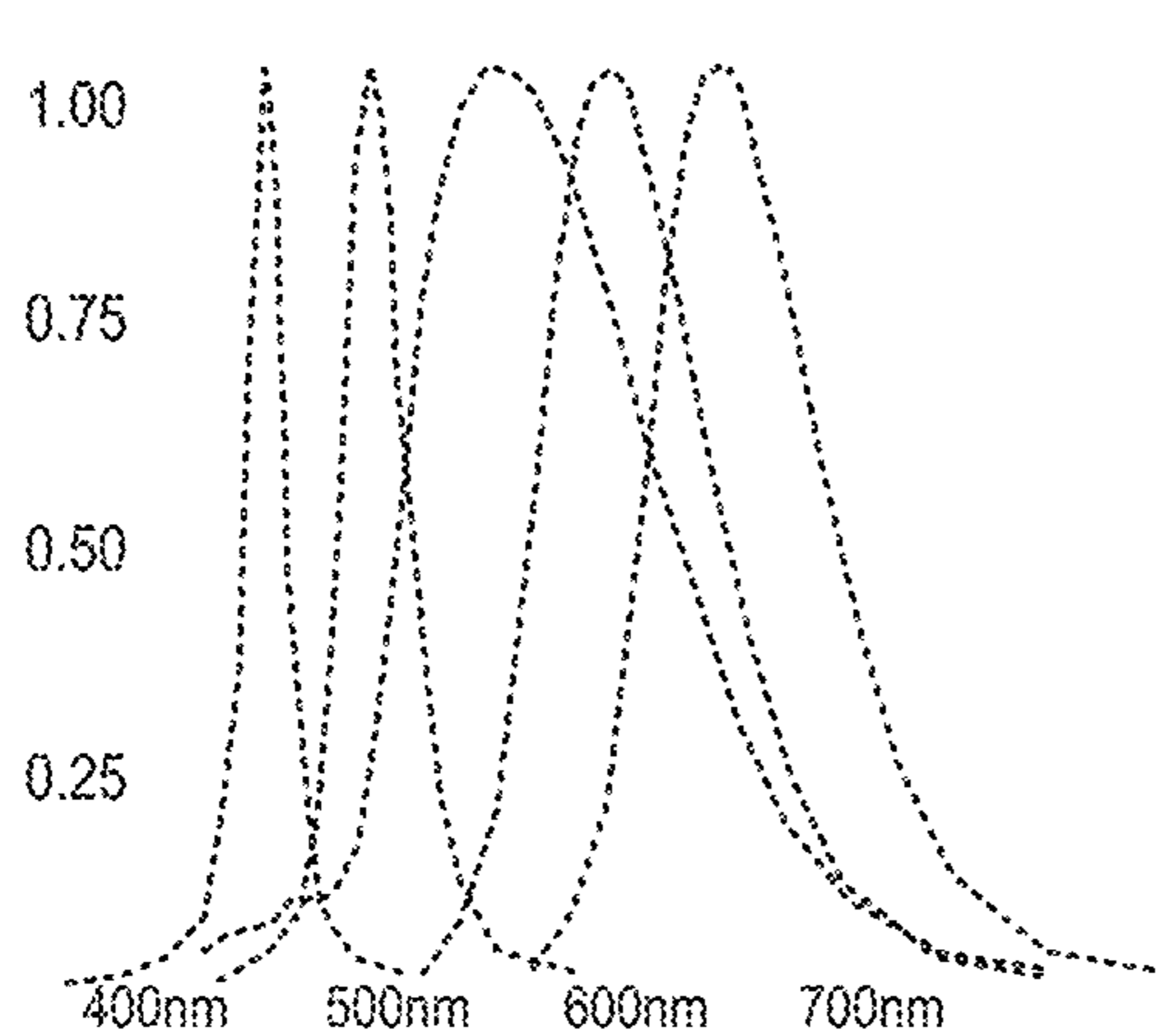
A set of known illuminant SPDs, in case they are our 5 LED channels
