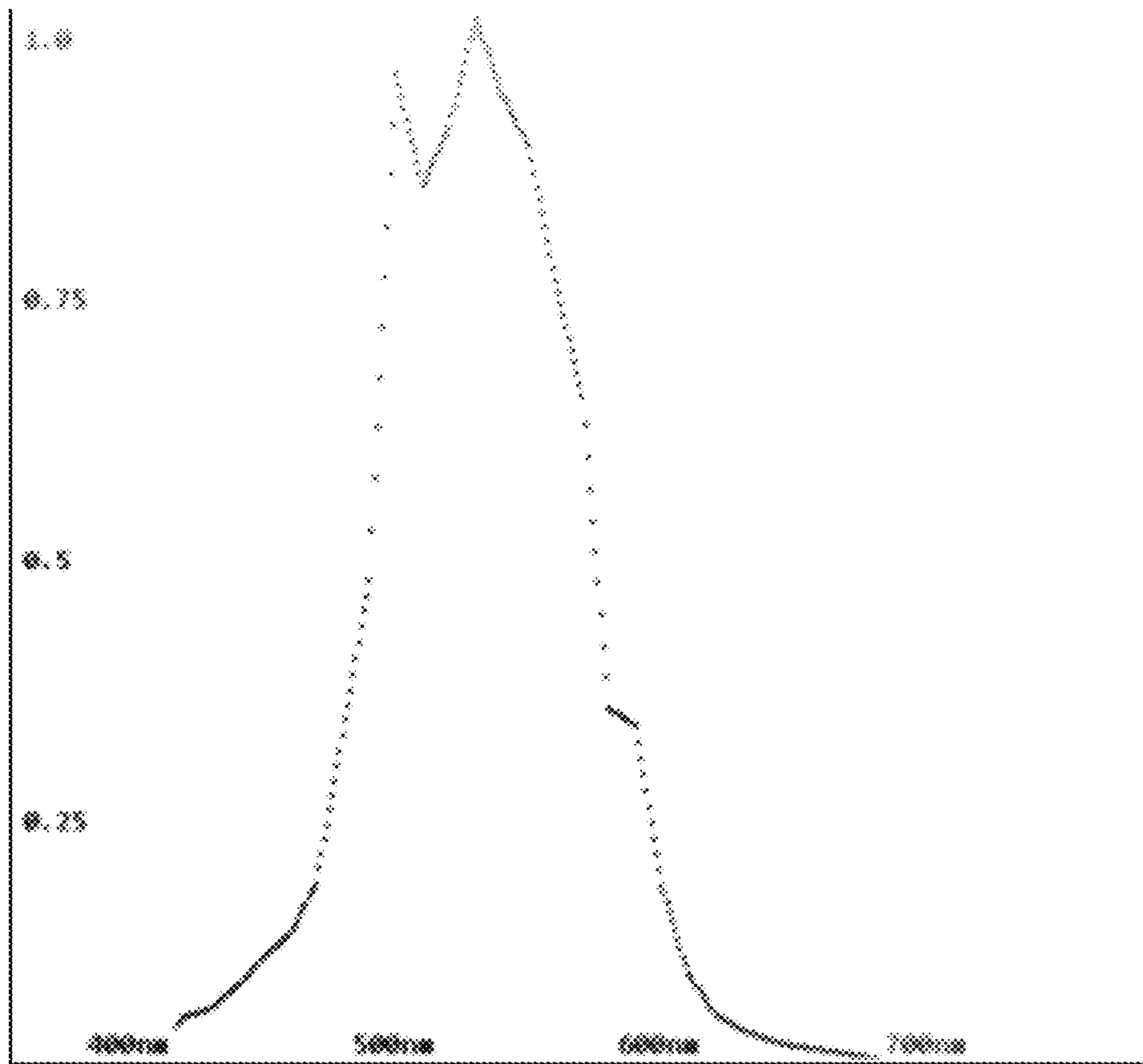
Sensor Response Over Visible Spectrum (~400-700 nm)
