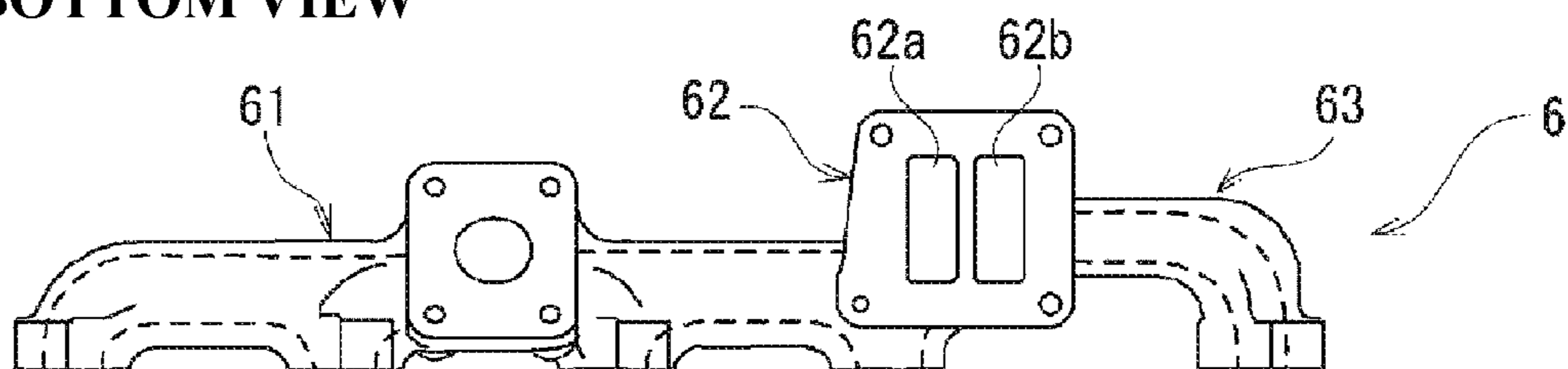
FIG. 4C BOTTOM VIEW
