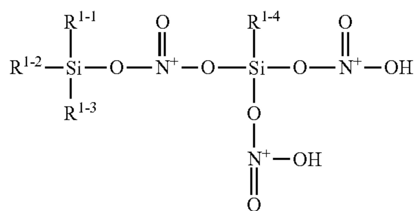
[Chemical Formula C5-4]
