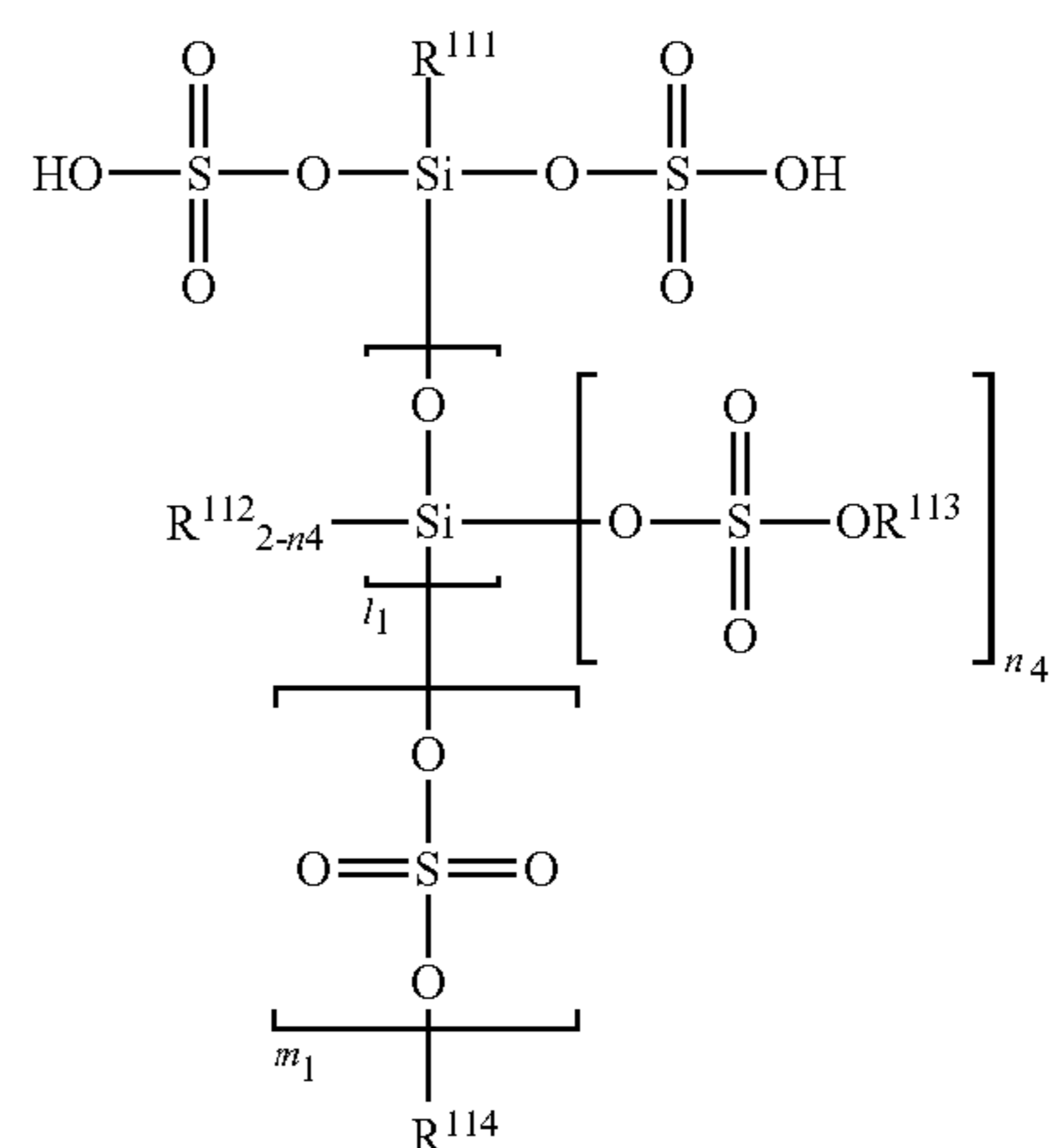
[Chemical Formula C12]
