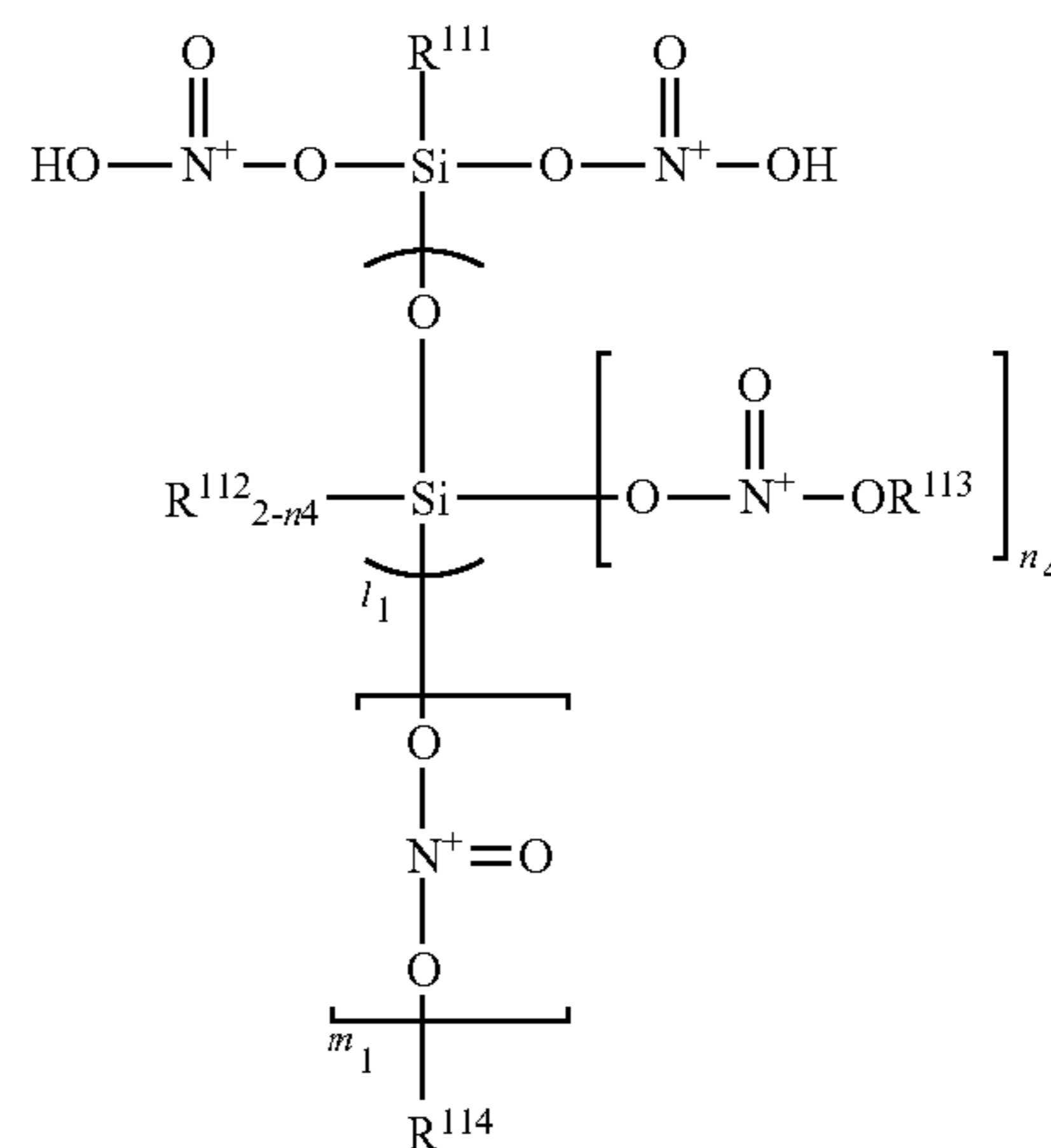
[Chemical Formula C13]
