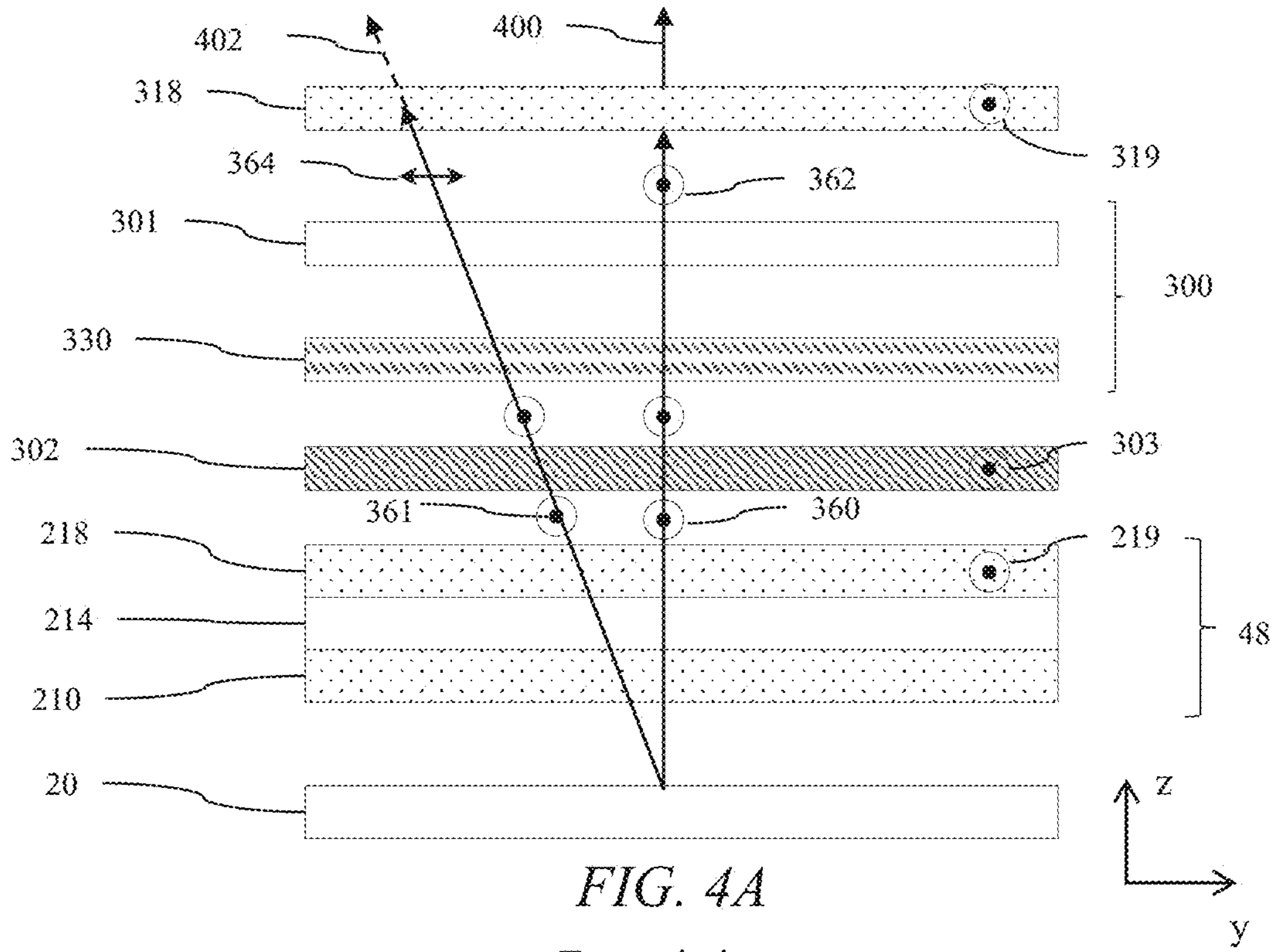
Transmission
