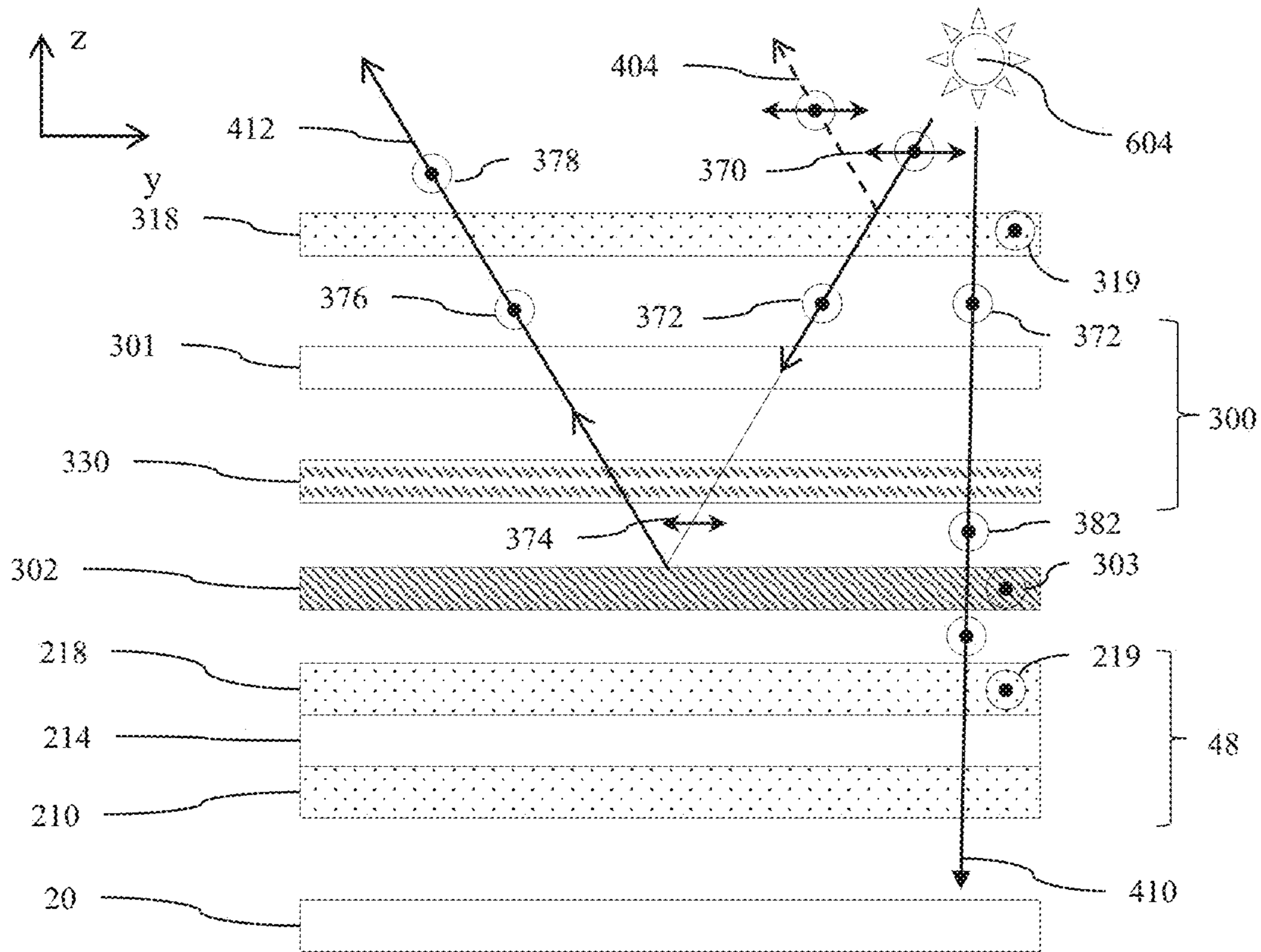
FIG. 5A Reflectivity
