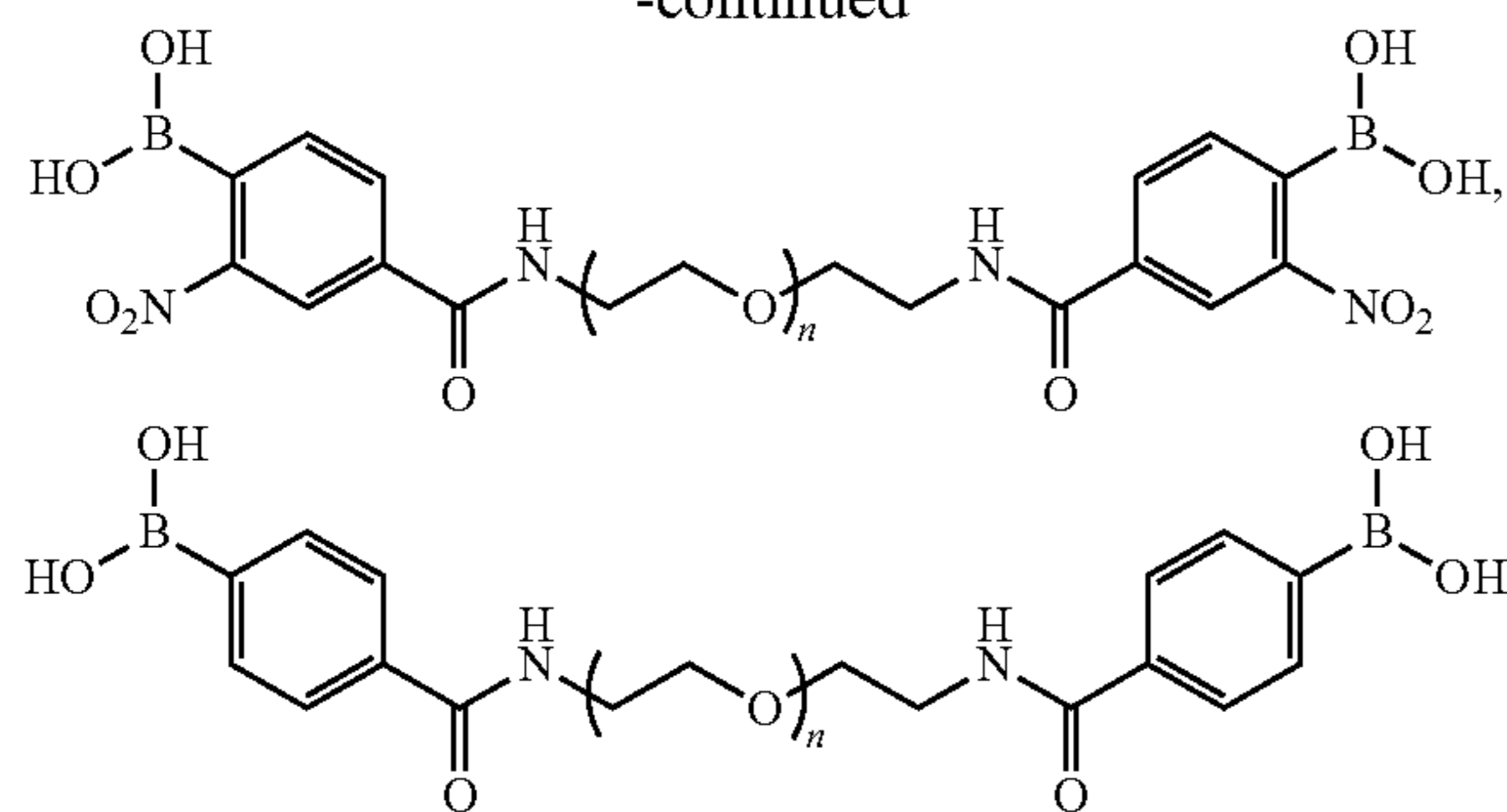
Imine Bonding
