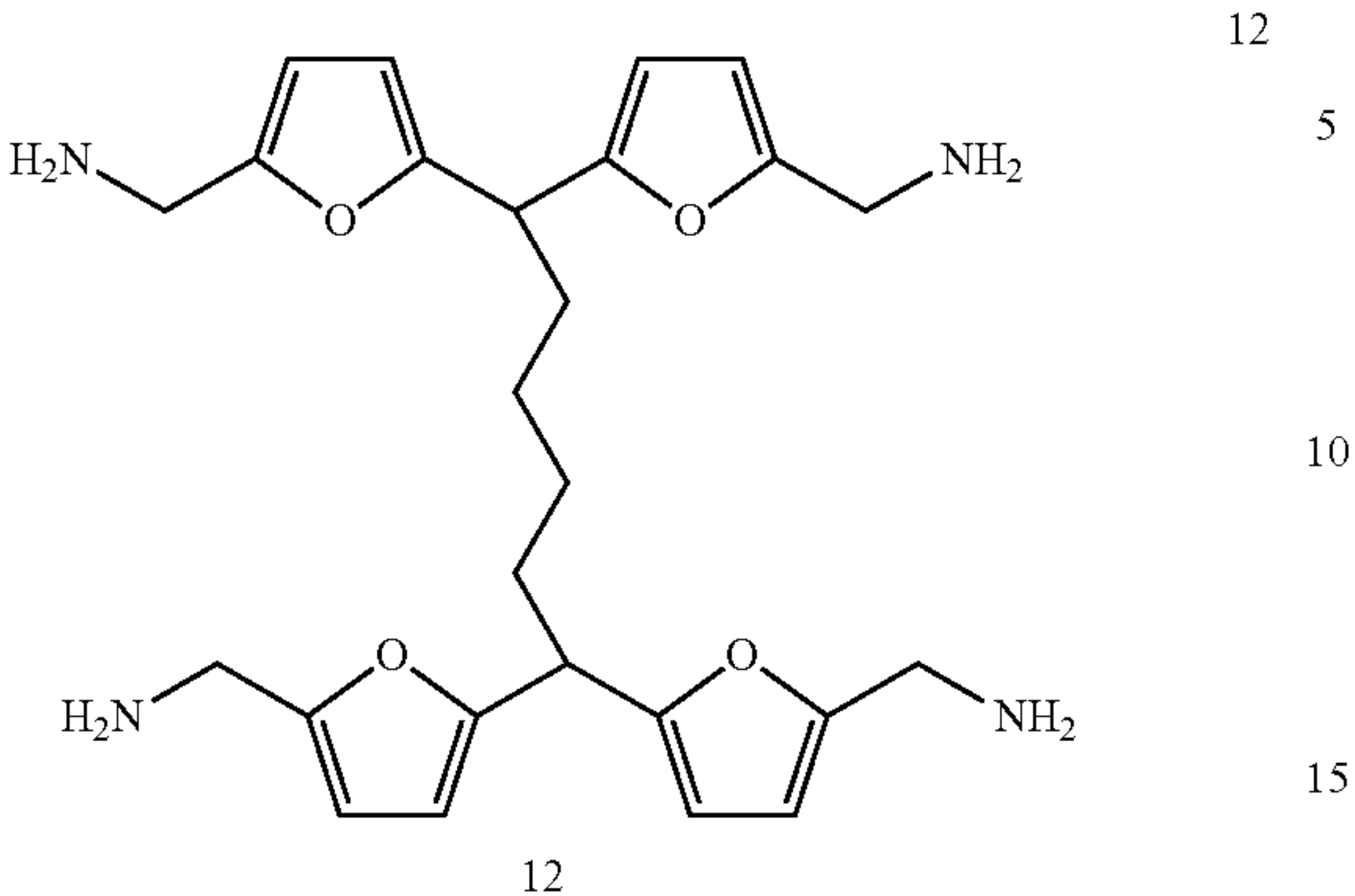
Chemical Structures of Various Furan Based Amines Used in the Examples
