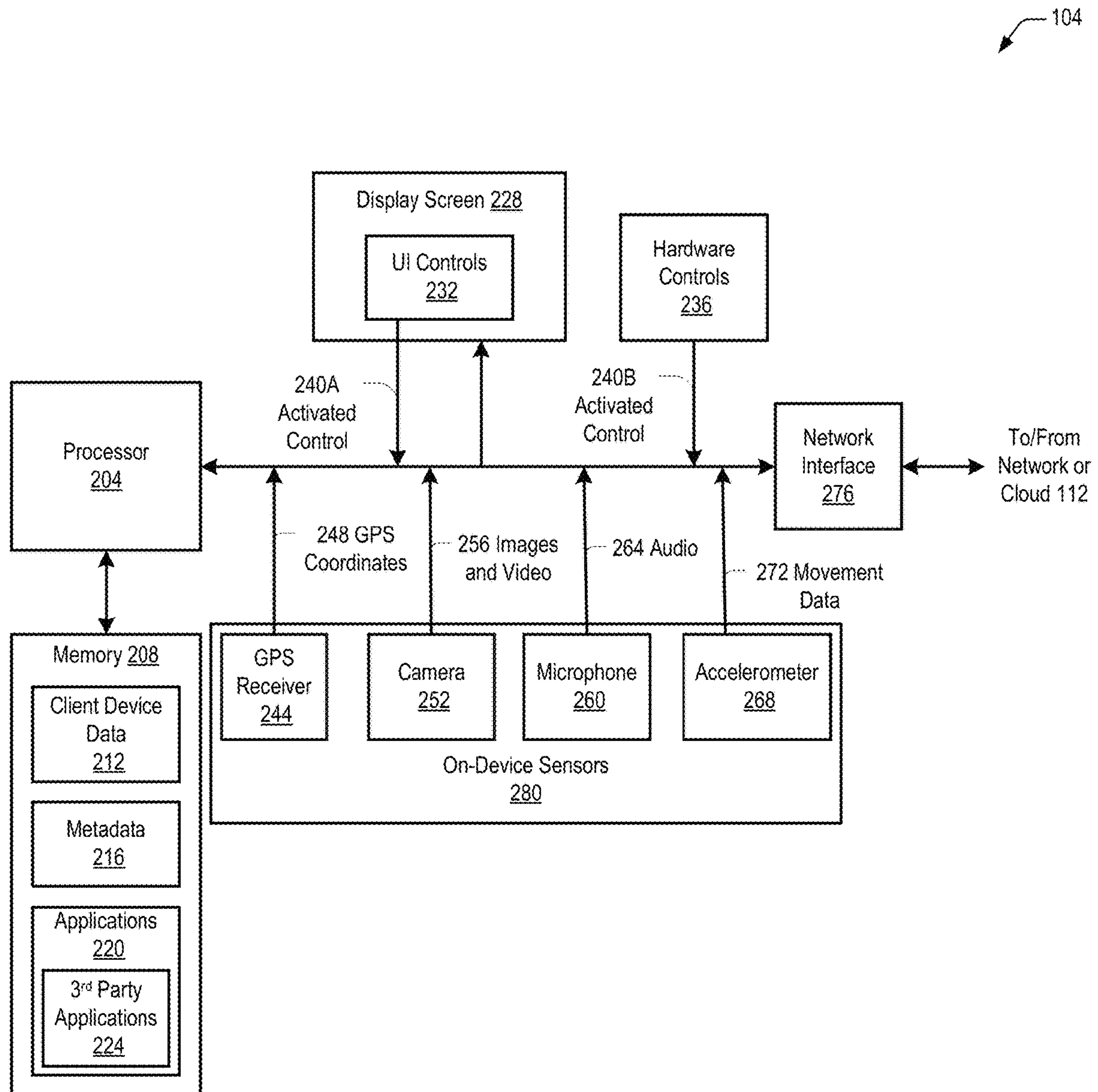
Fig. 2 Client Device
