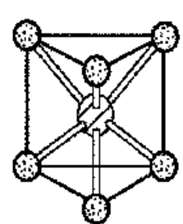
Trigonal Prismatic
