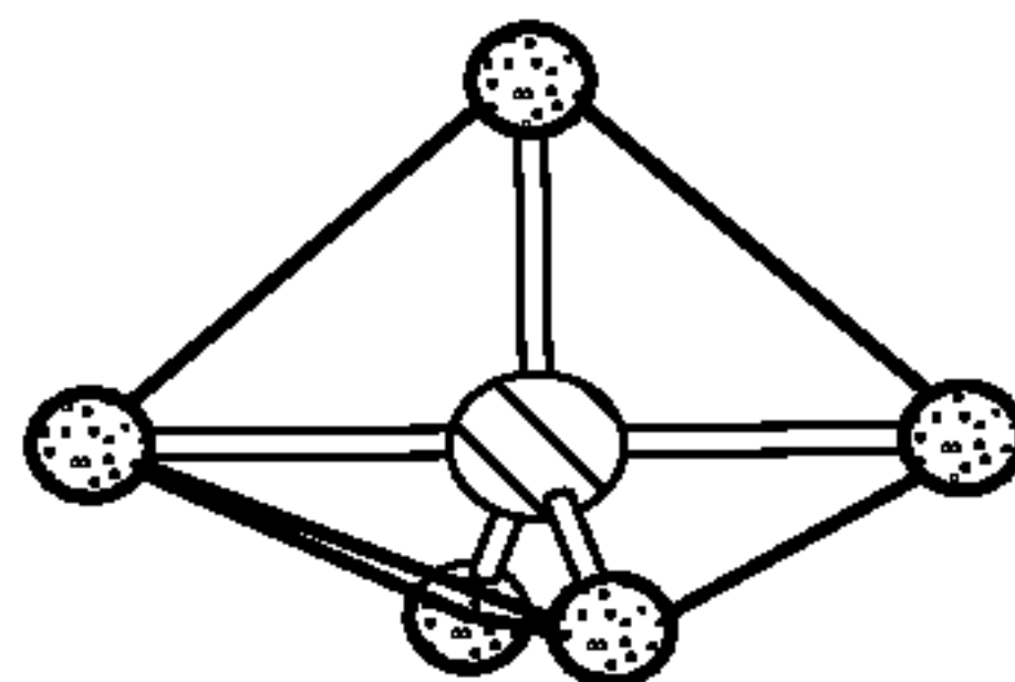
Trigonal Bipyramidal
