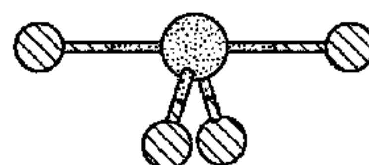
Seesaw
