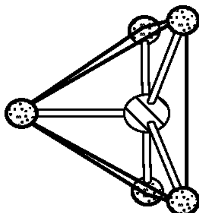
Square Pyramidal
