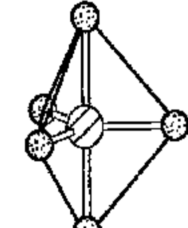
Trigonal Bipyramidal
