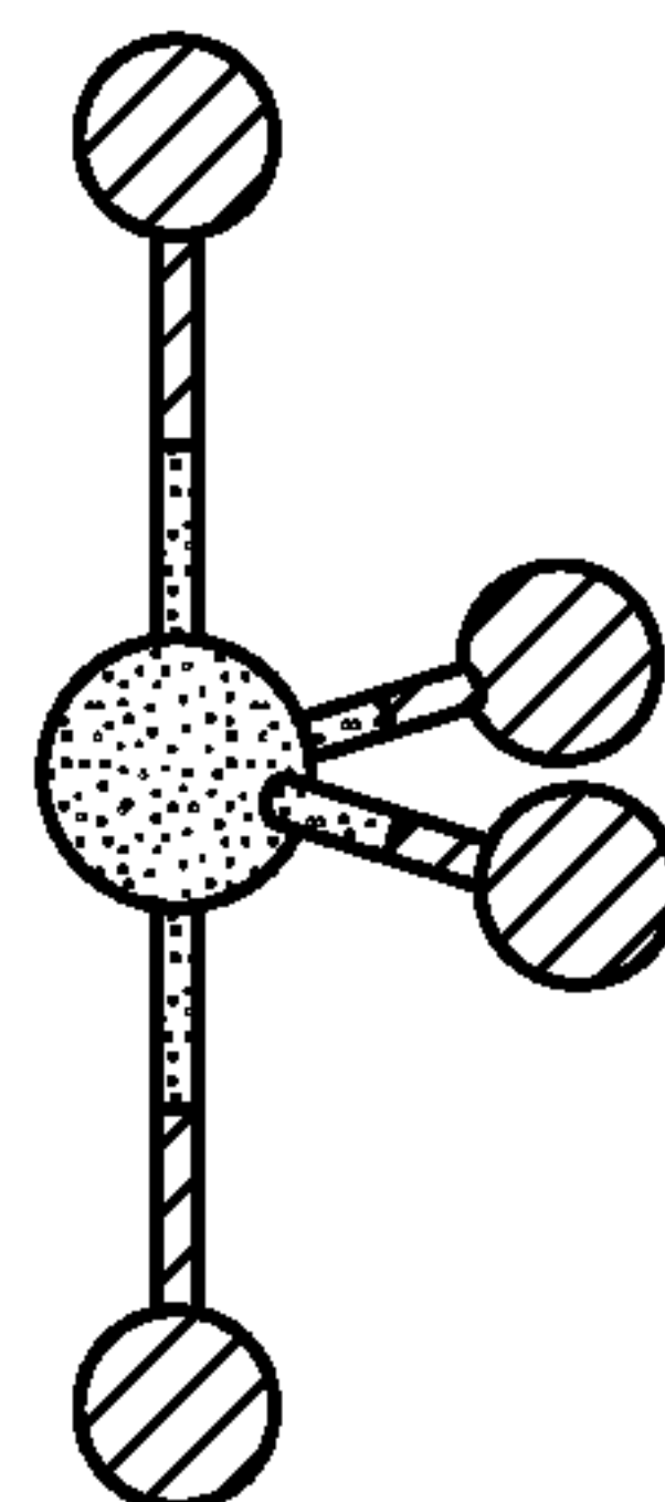
Seesaw
