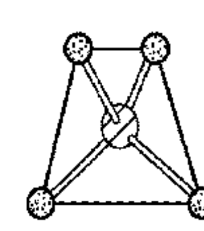
Tetrahedral
