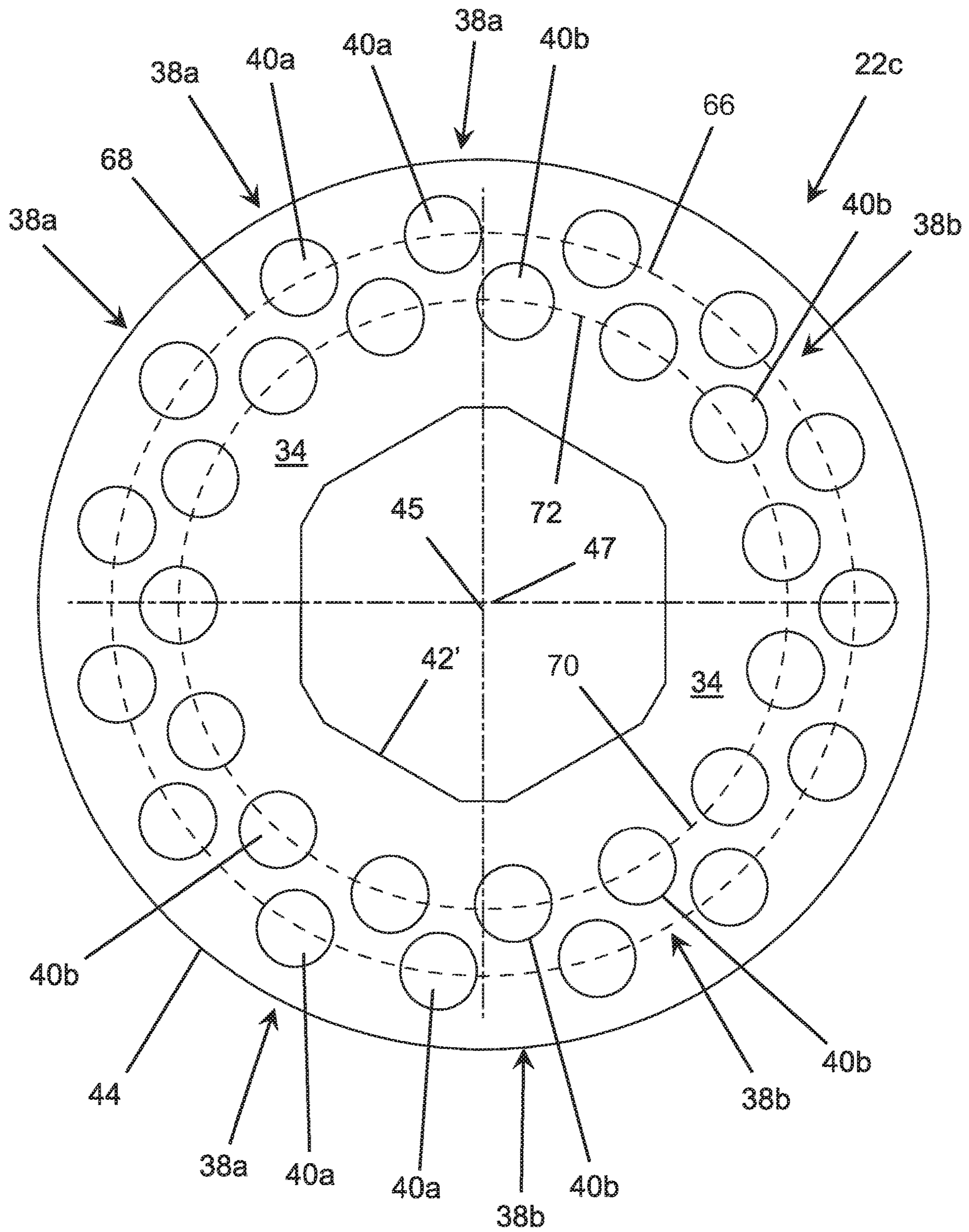
FIG. 3 (PRIOR ART)
