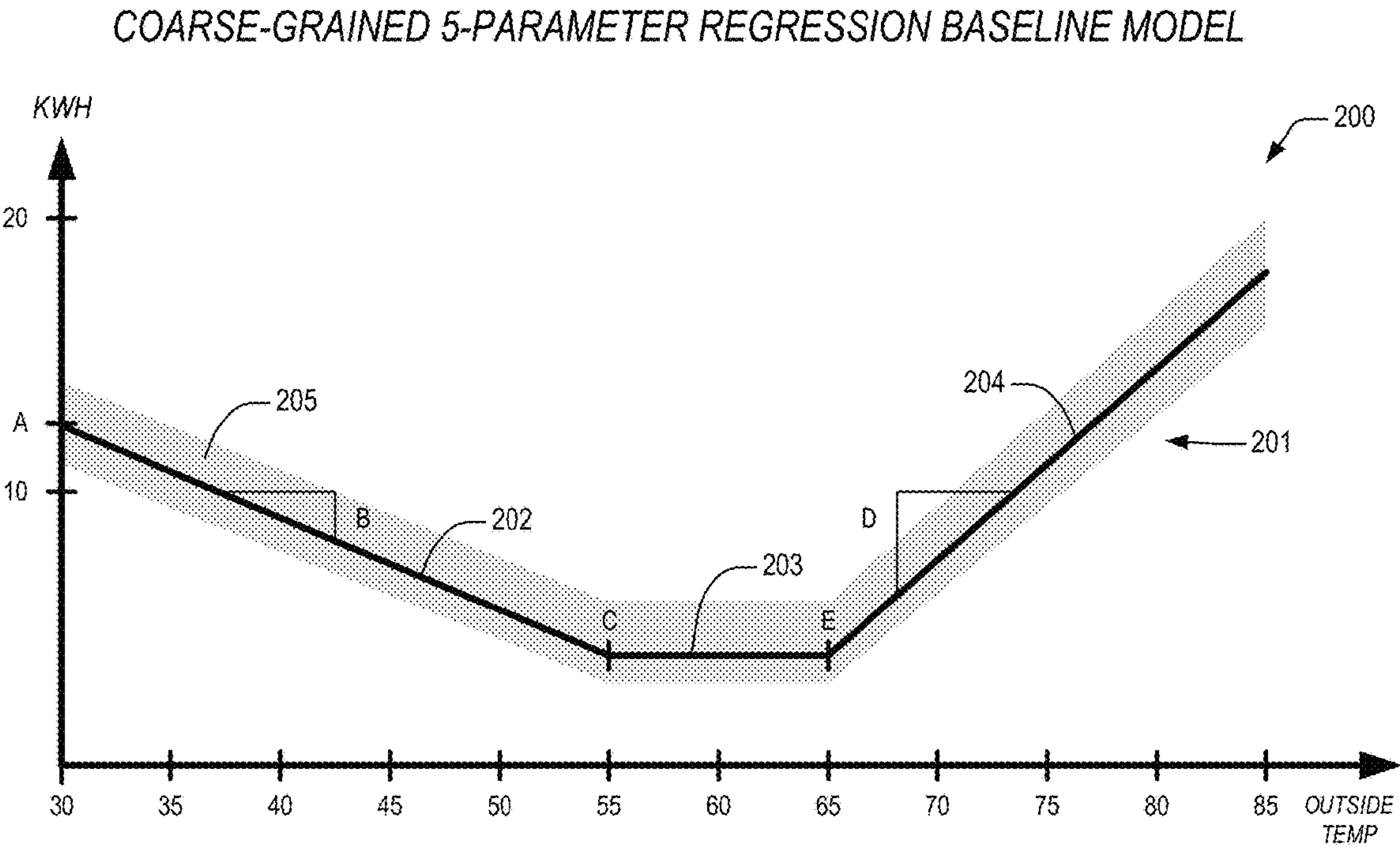
FIG. 2 (Prior Art)
