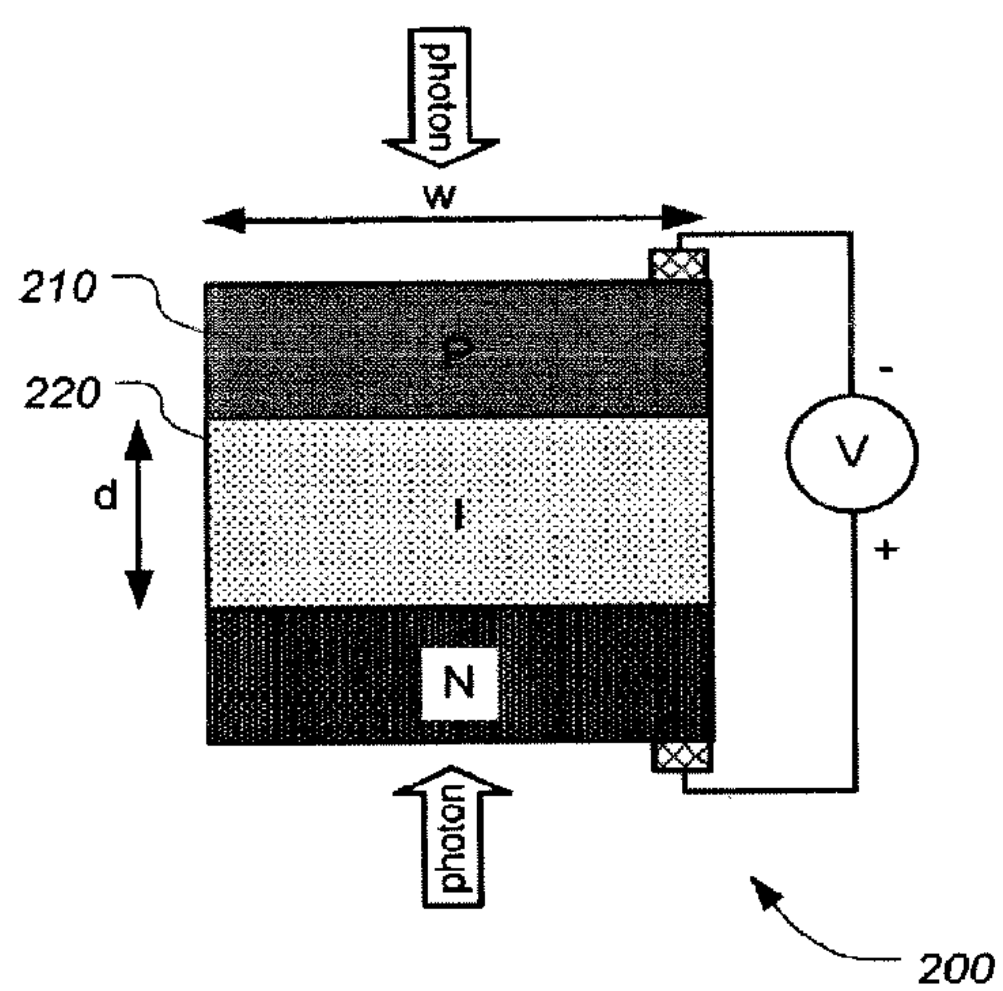
FIG. 2 (prior art)
