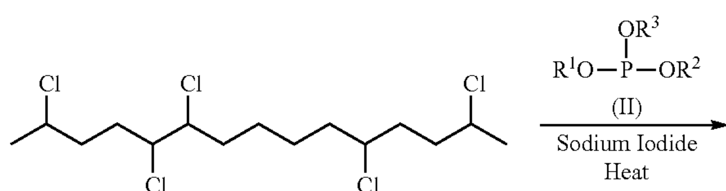
Scheme 1
