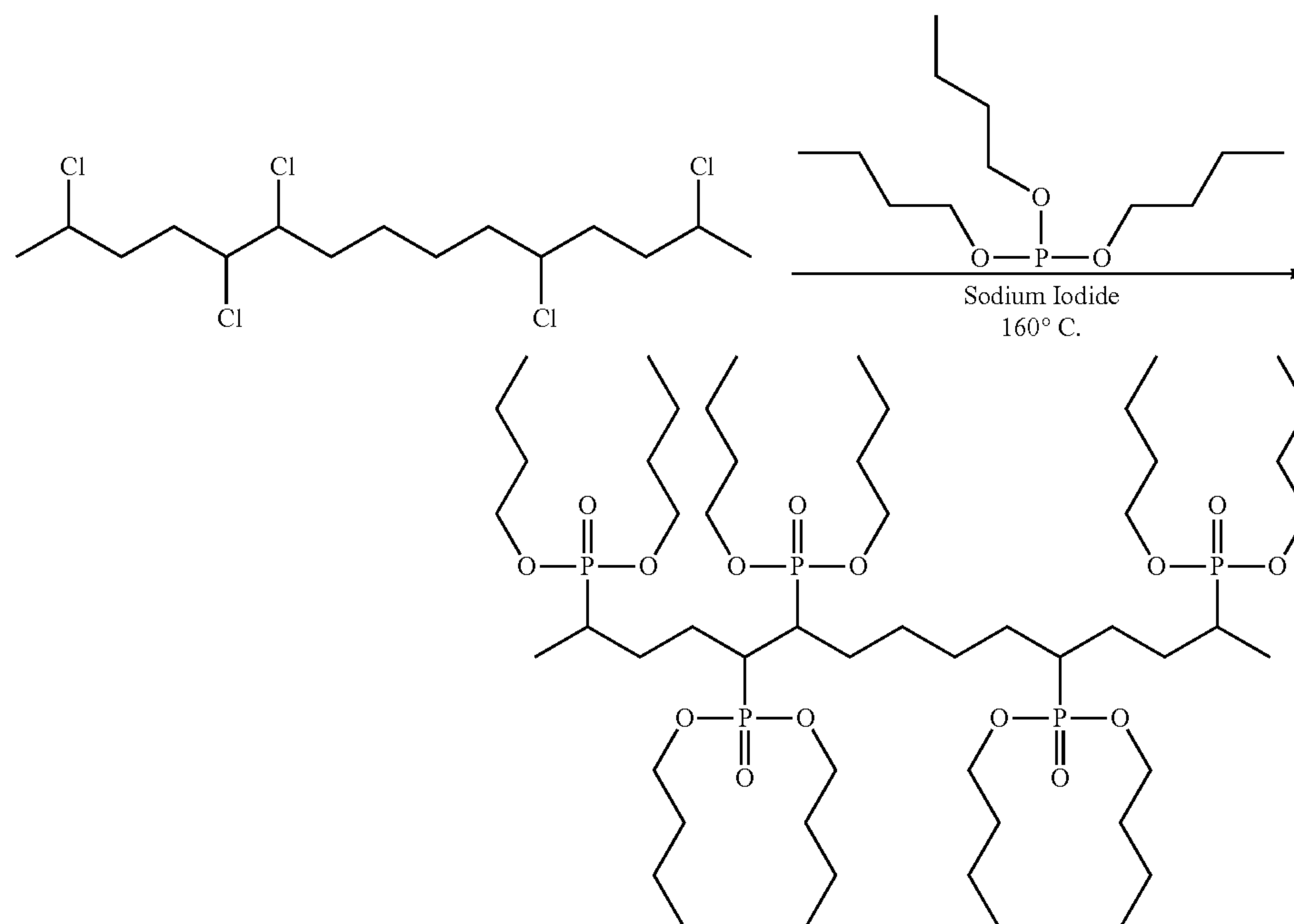
Scheme 2
