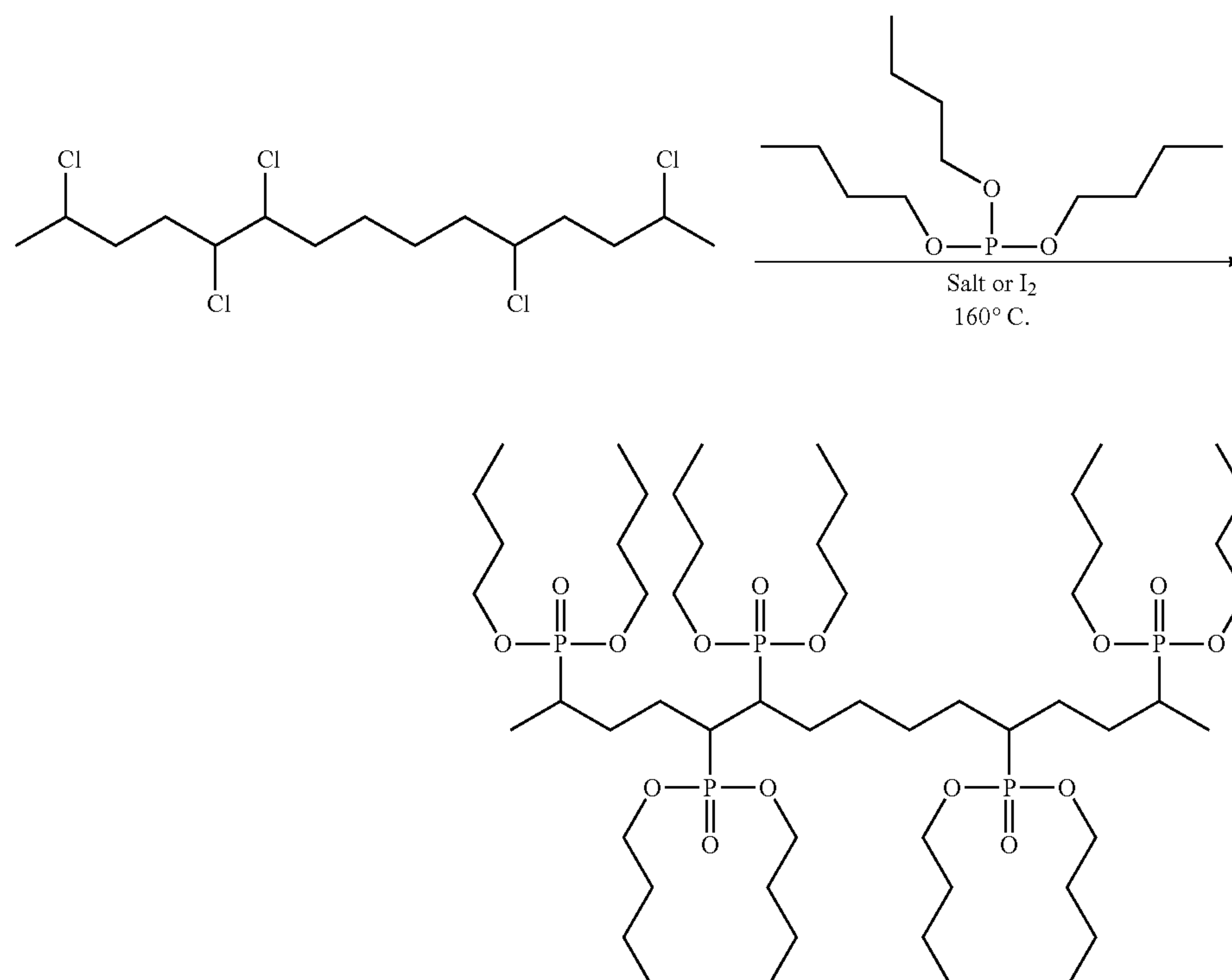
Scheme 4
