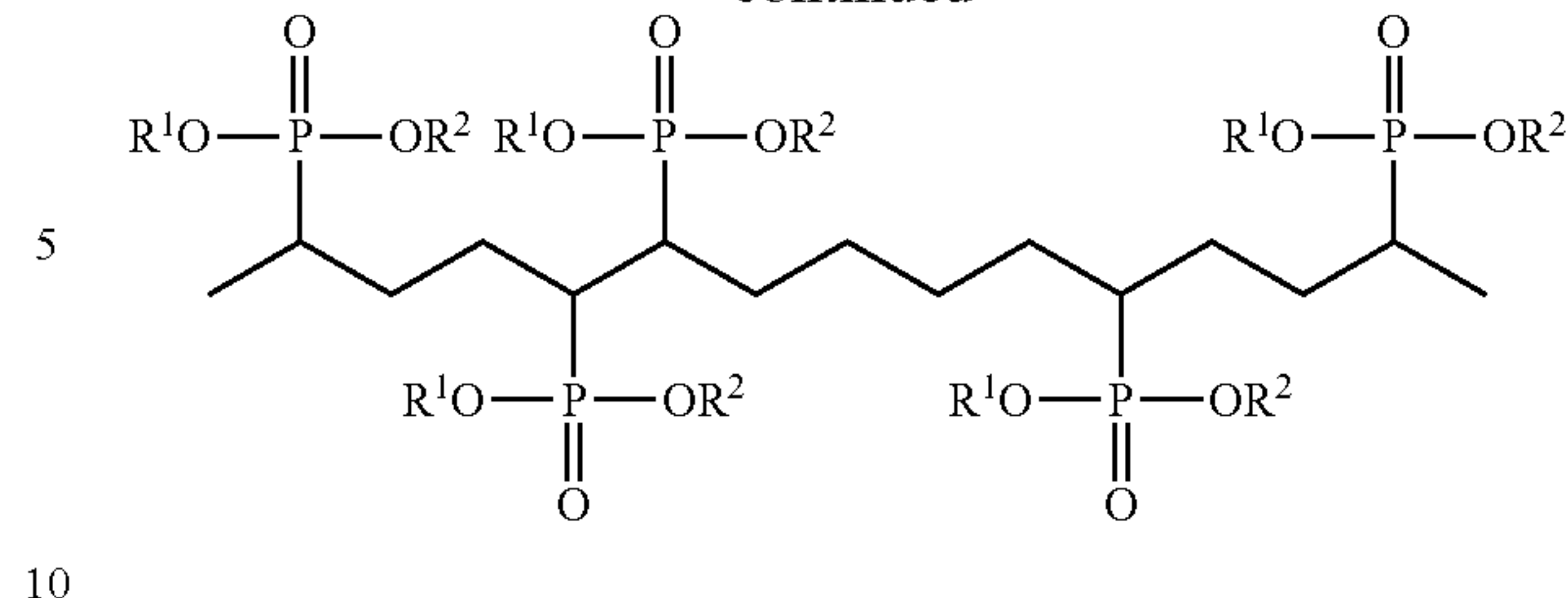
Scheme 2
