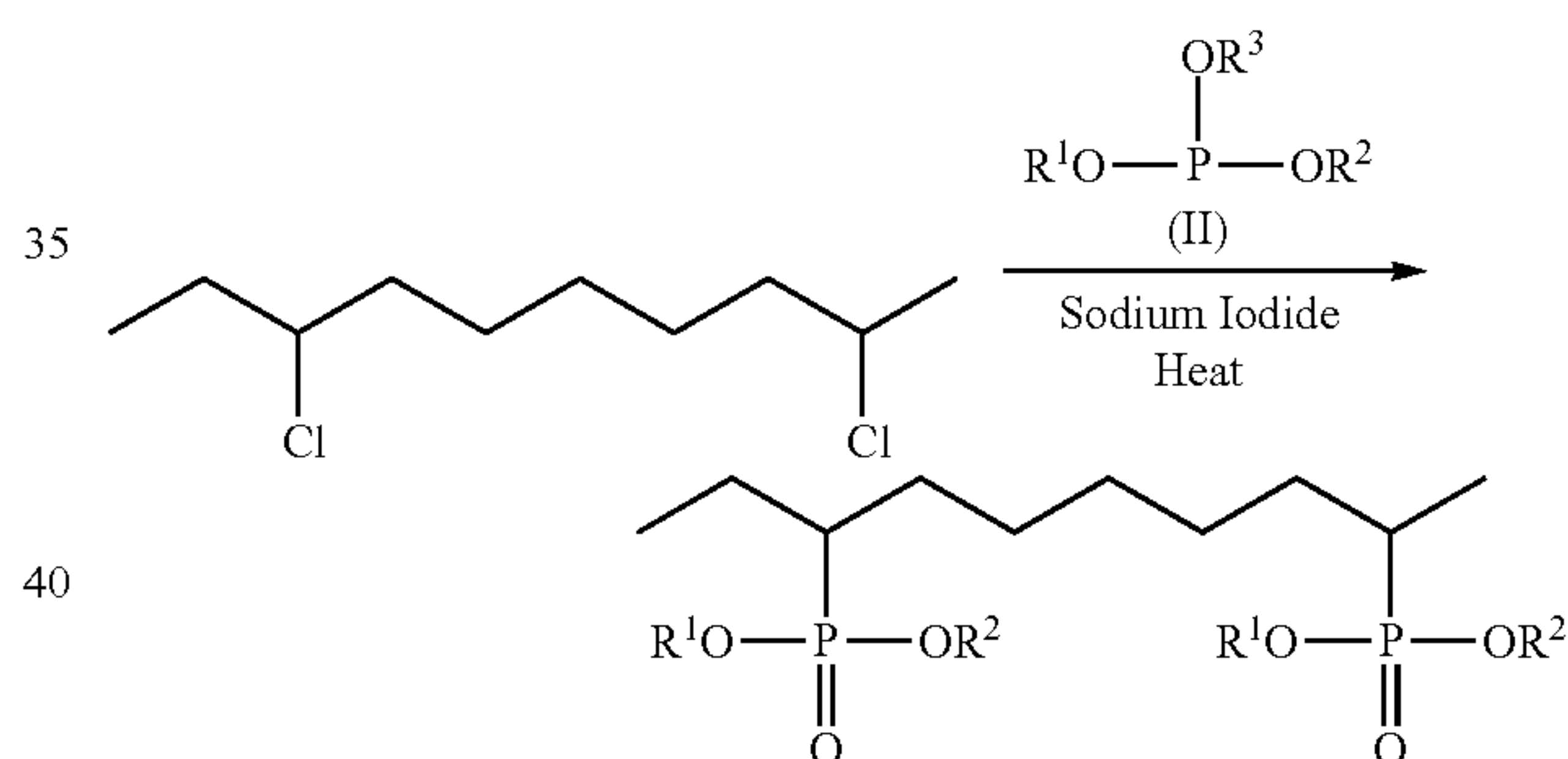
Scheme 3
