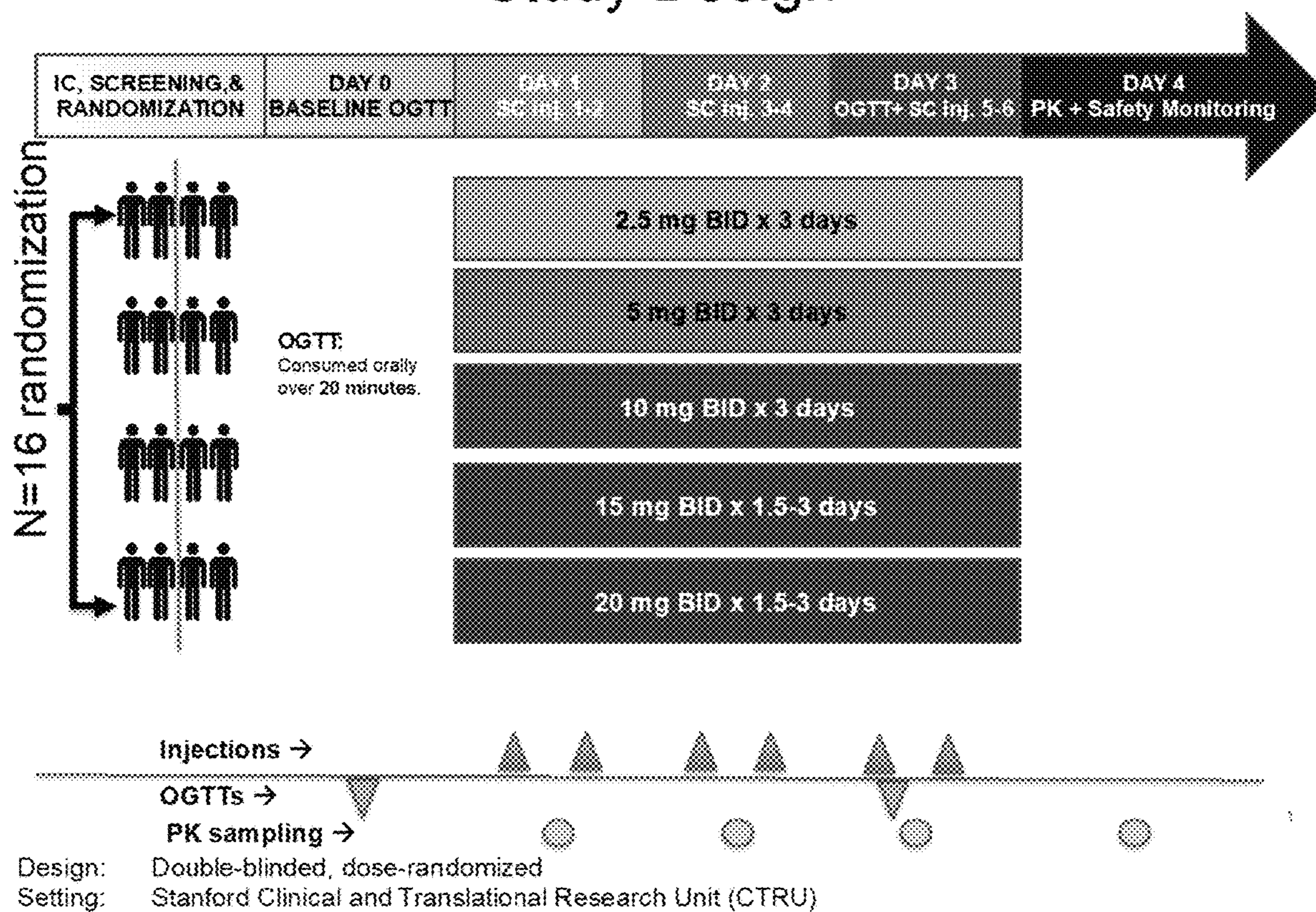
FIG. 9 Study Design
