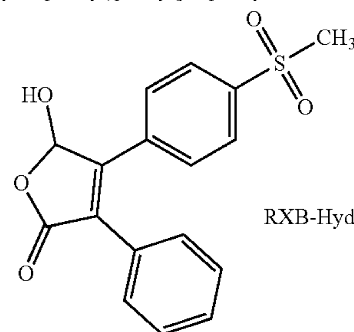
4-[4-(methylsulphonyl)phenyl]-3-phenyl-2,5-furandione
