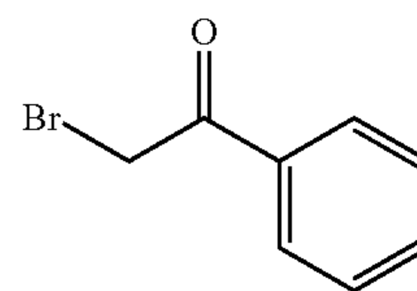
2-bromoacetophenone
