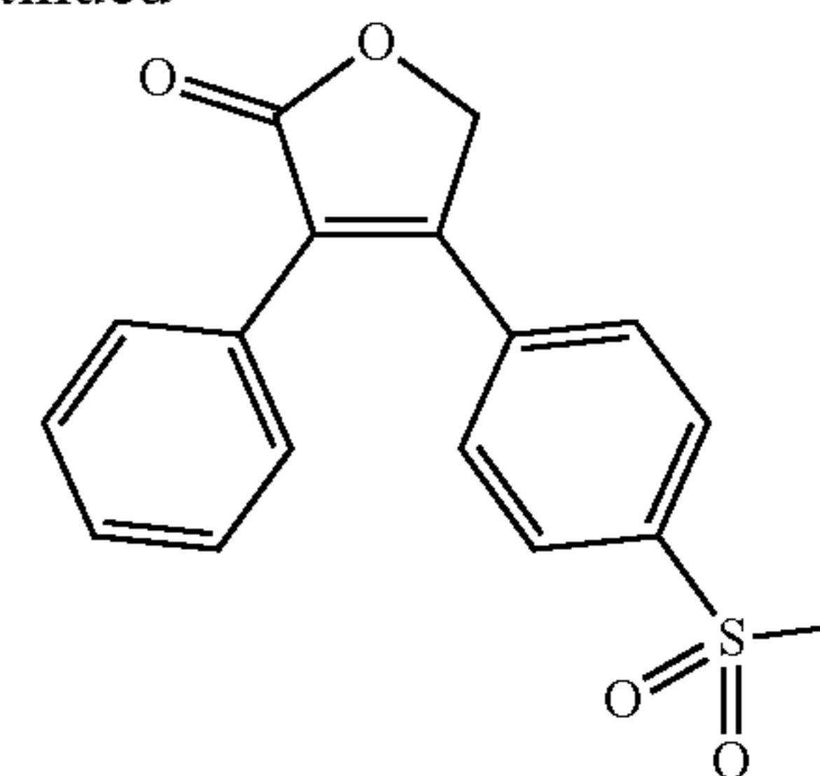
Stage 4 crude RXB-201 C_{17}H_{14}O_4S MW = 314.36
