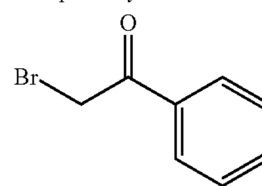
2-bromoacetophenone
