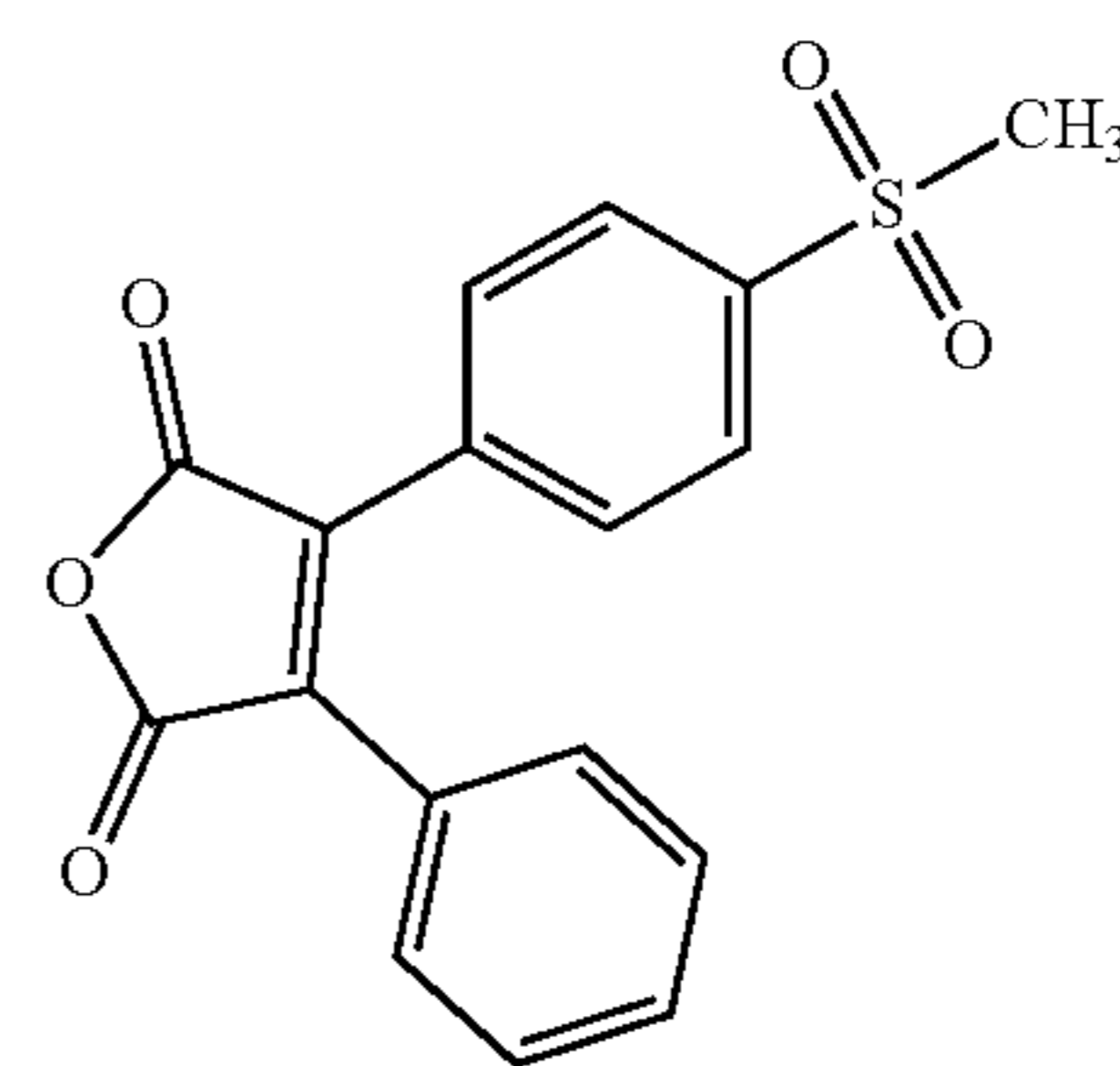
4-[4-(methylsulphonyl)phenyl]-3-phenyl-2,5-furandione
