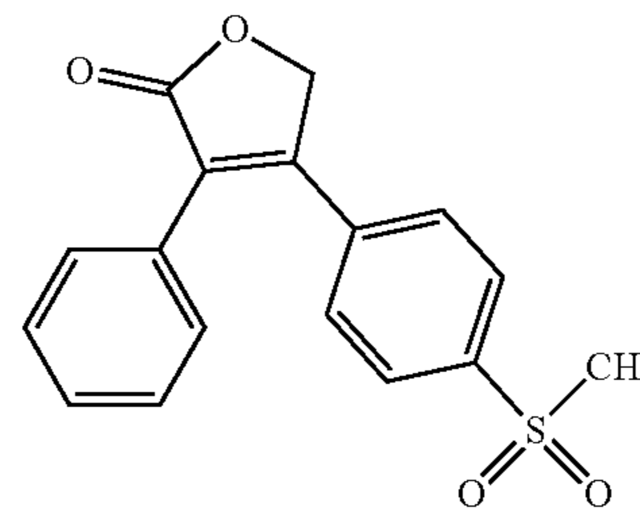
Chemical Structure of Rofecoxib
