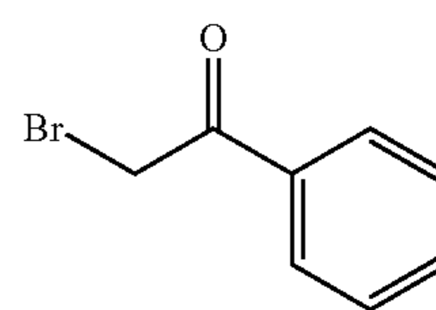
phenacyl bromide
