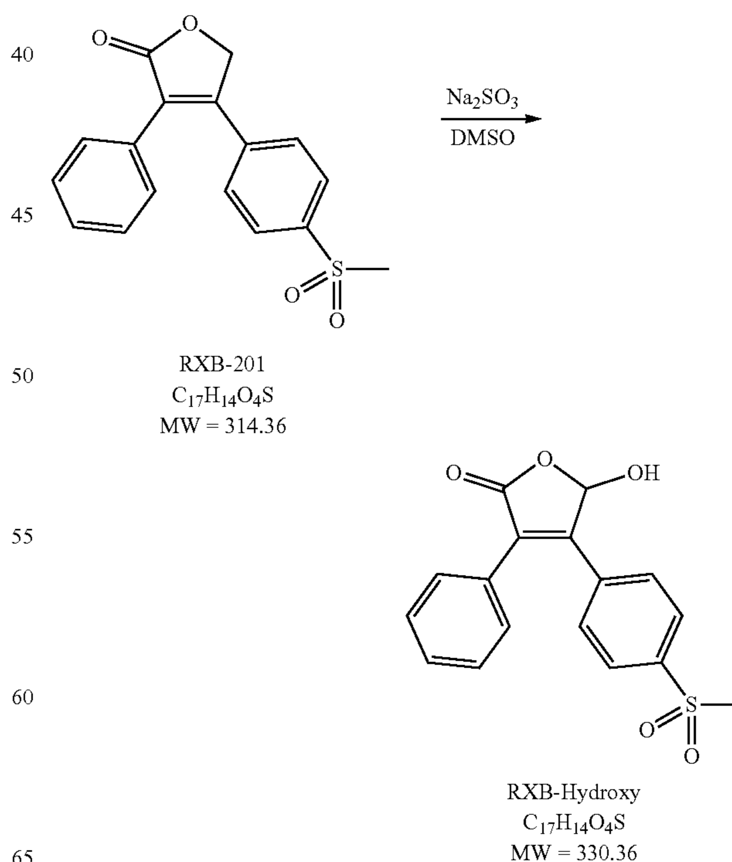
Scheme 2. Formation of 4-[4-(methylsulphonyl)phenyl]-3-phenyl-5-hydroxyfuran-2-one (RXB-Hydroxy) impurity
