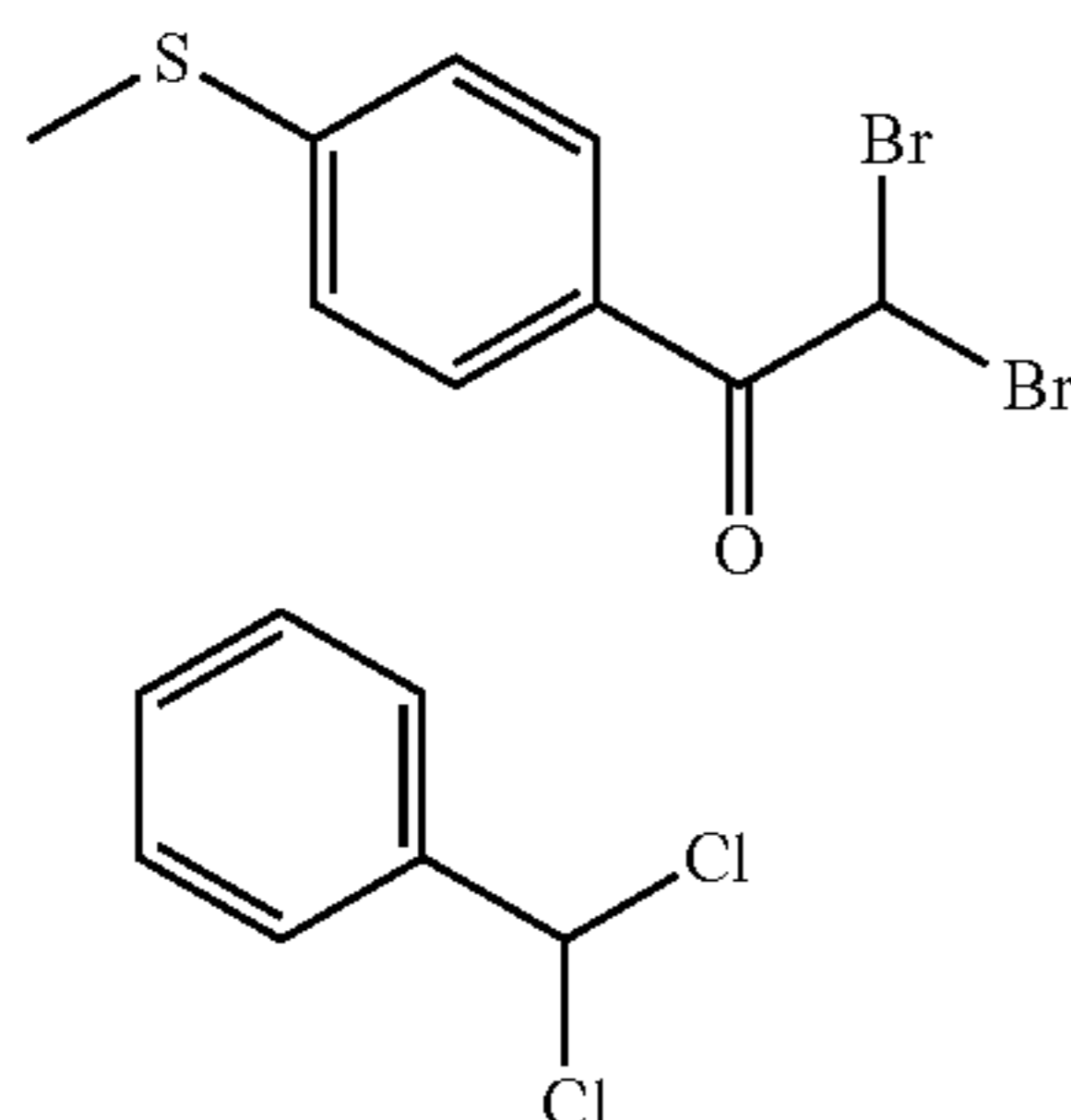
alpha, alpha-dichlorotoluene
