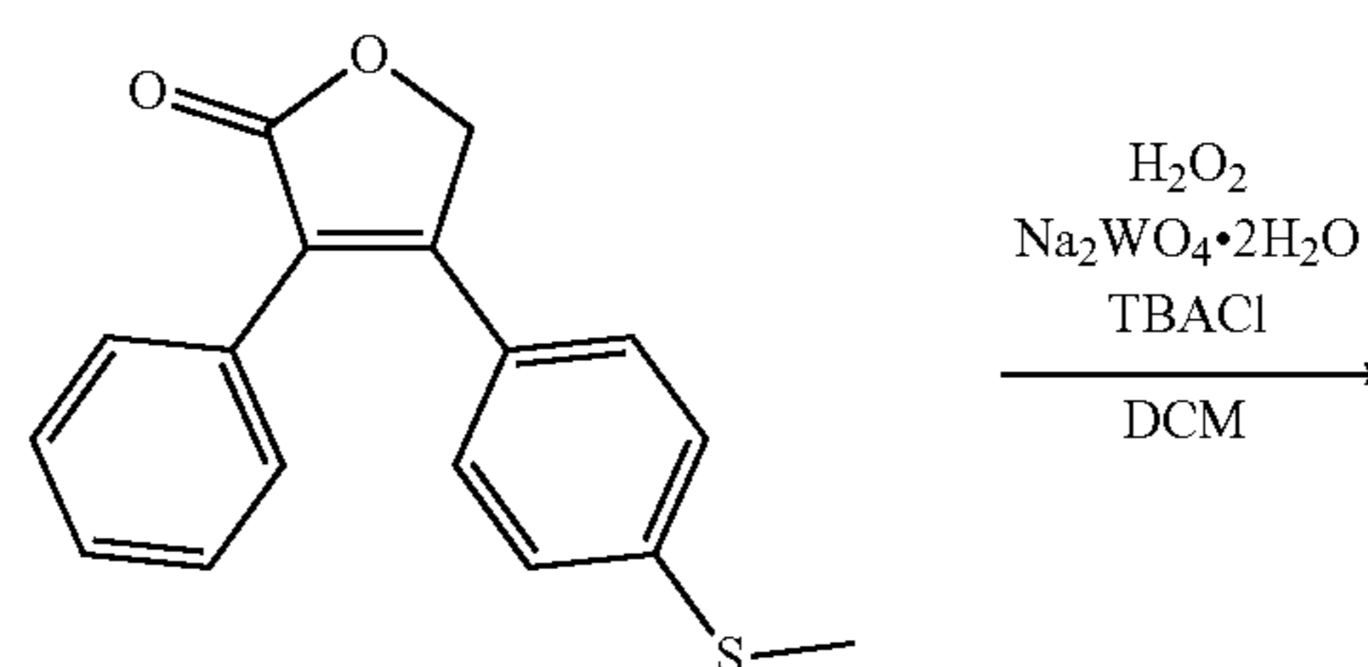
Scheme 4. Oxidation of 4-[4-(methylthio)phenyl]-3-phenyl-2(5H)-furanone in DCM/H 2 O
