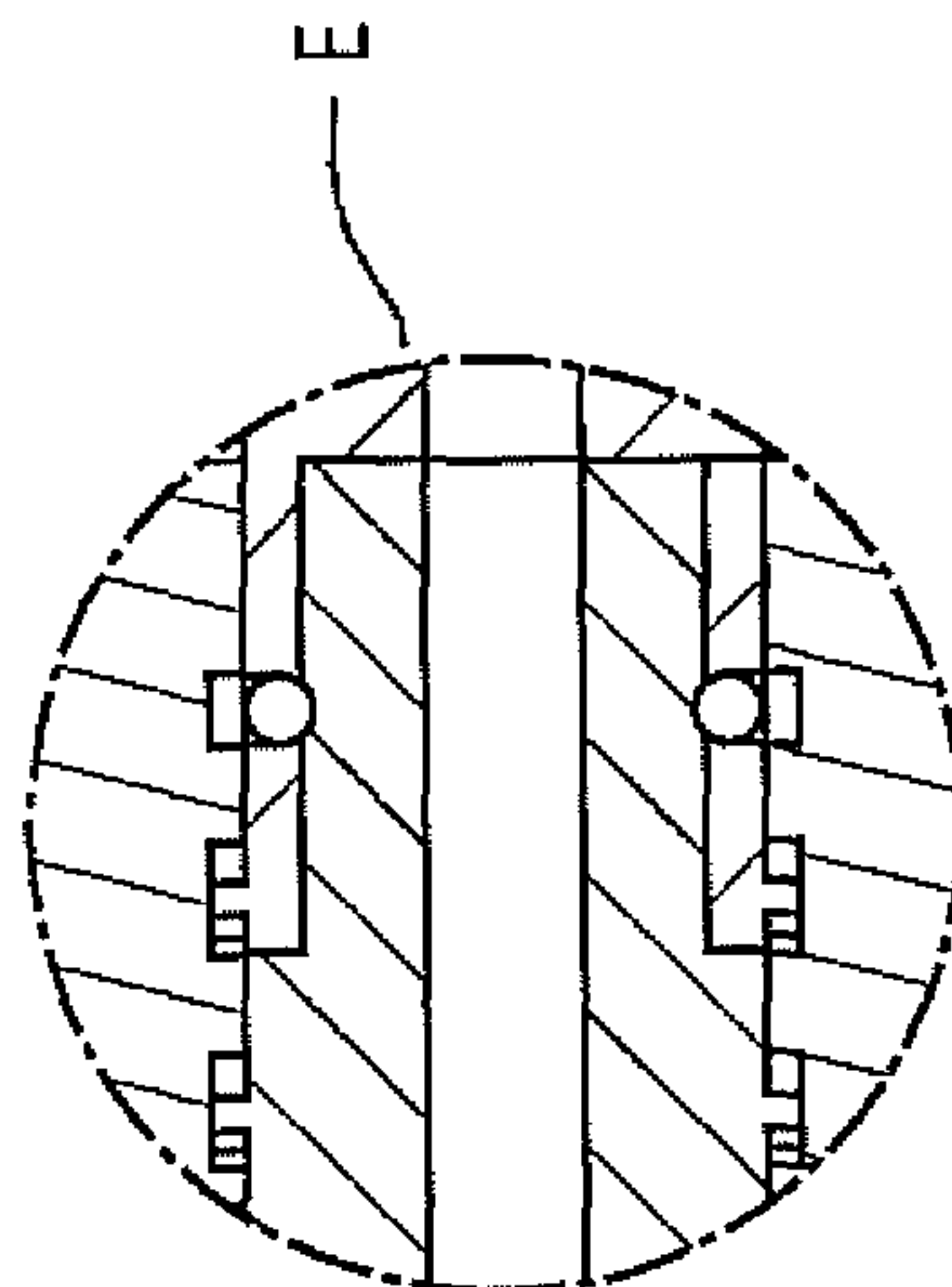
DETAIL E SCALE 1:1
