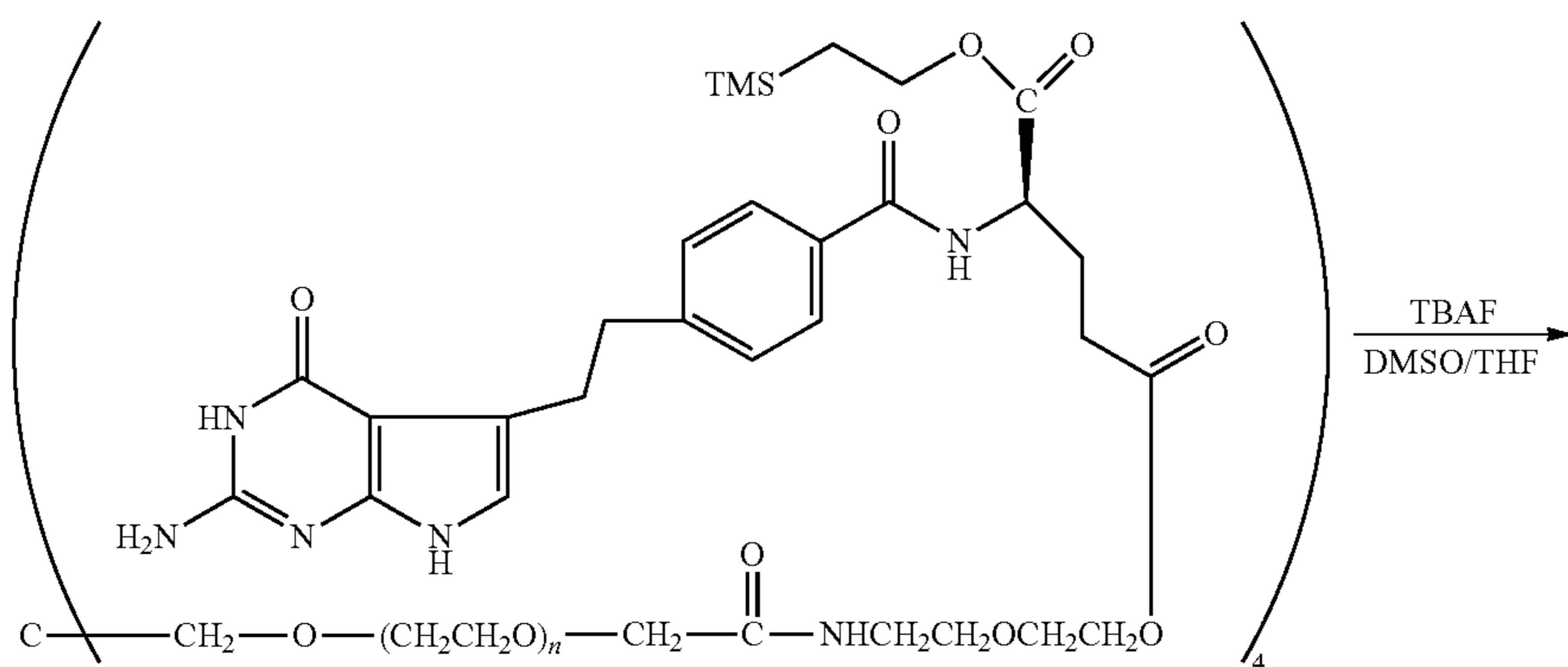
Compound 23a (n is defined to provide a 4-arm-PEG 10k) Compound 23b (n is defined to provide a 4-arm-PEG 20k) Compound 23c (n is defined to provide a 4-arm-PEG 40k)
