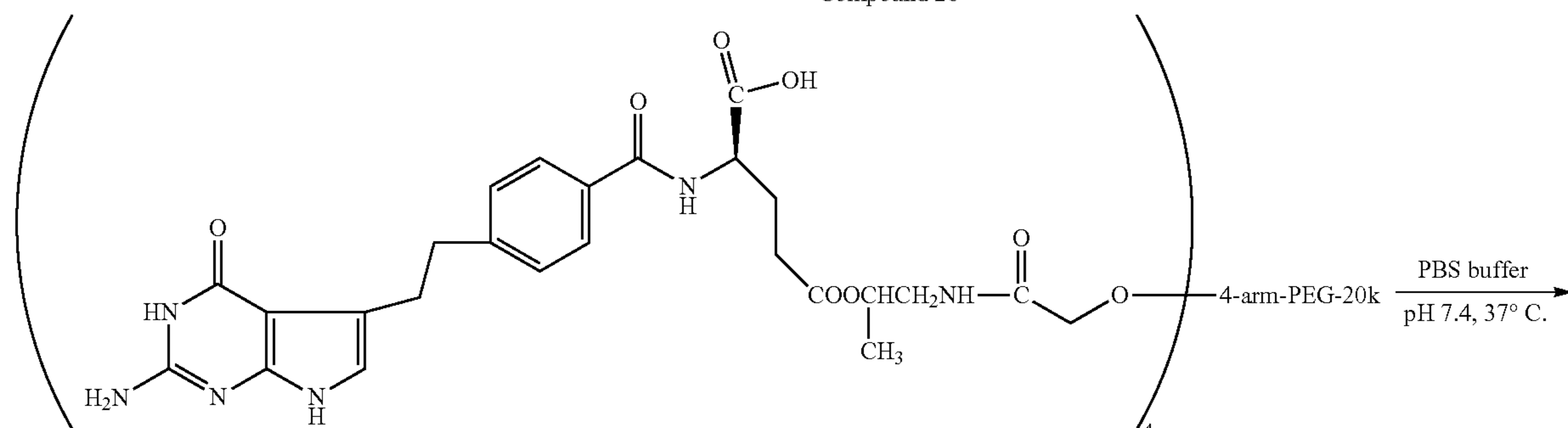
Compound 28
