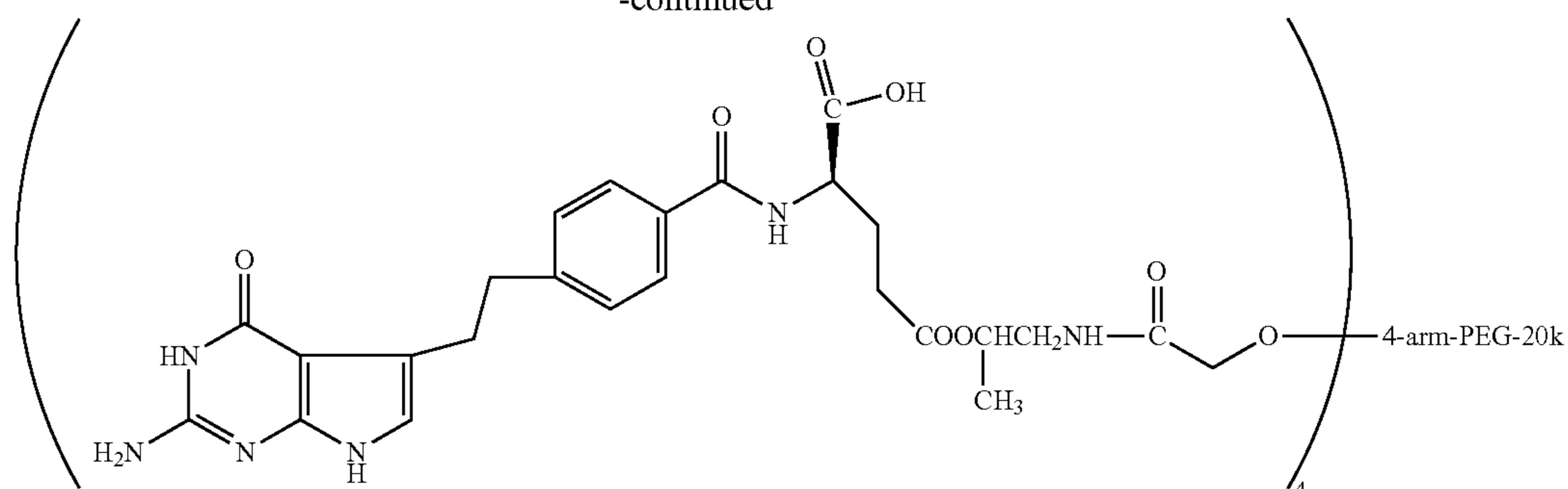
Compound 28
