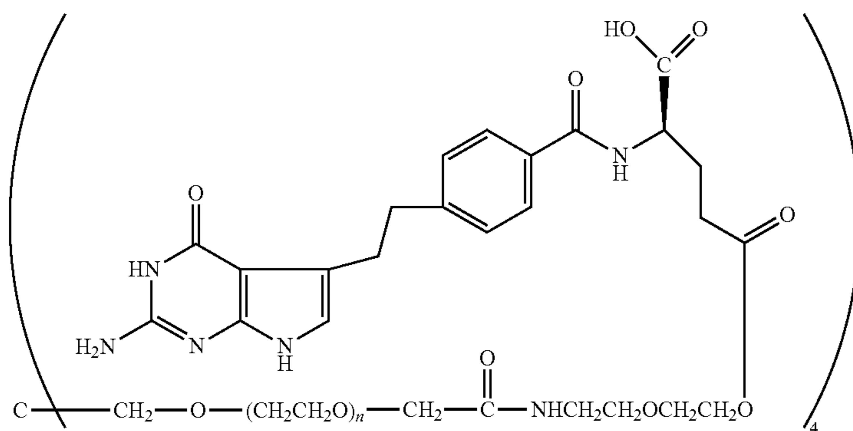
Compound 24a (n is defined to provide a 4-arm-PEG 10k) Compound 24b (n is defined to provide a 4-arm-PEG 20k) Compound 24c (n is defined to provide a 4-arm-PEG 40k)
