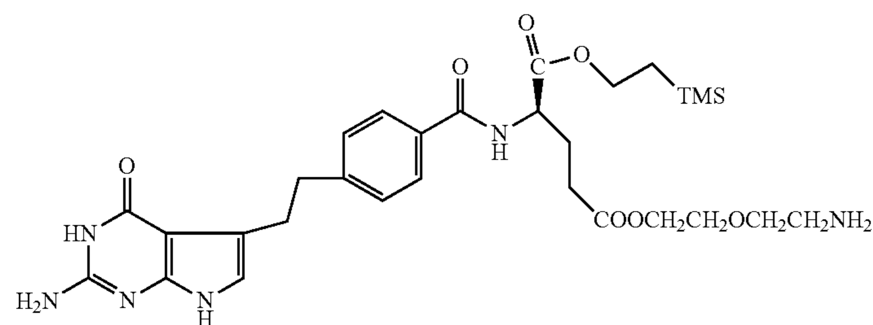
Compound 22
