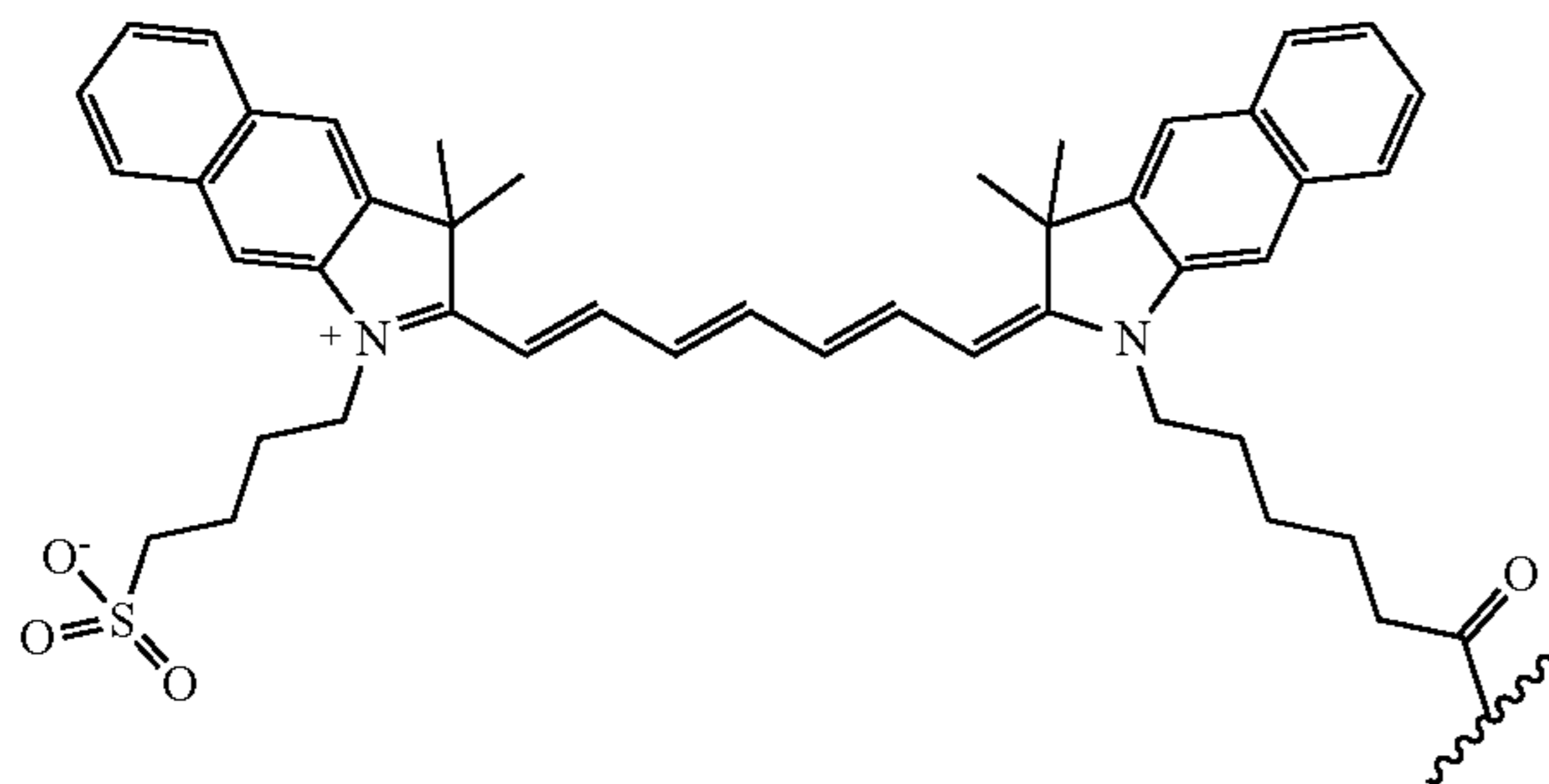
Indocyanine Green
