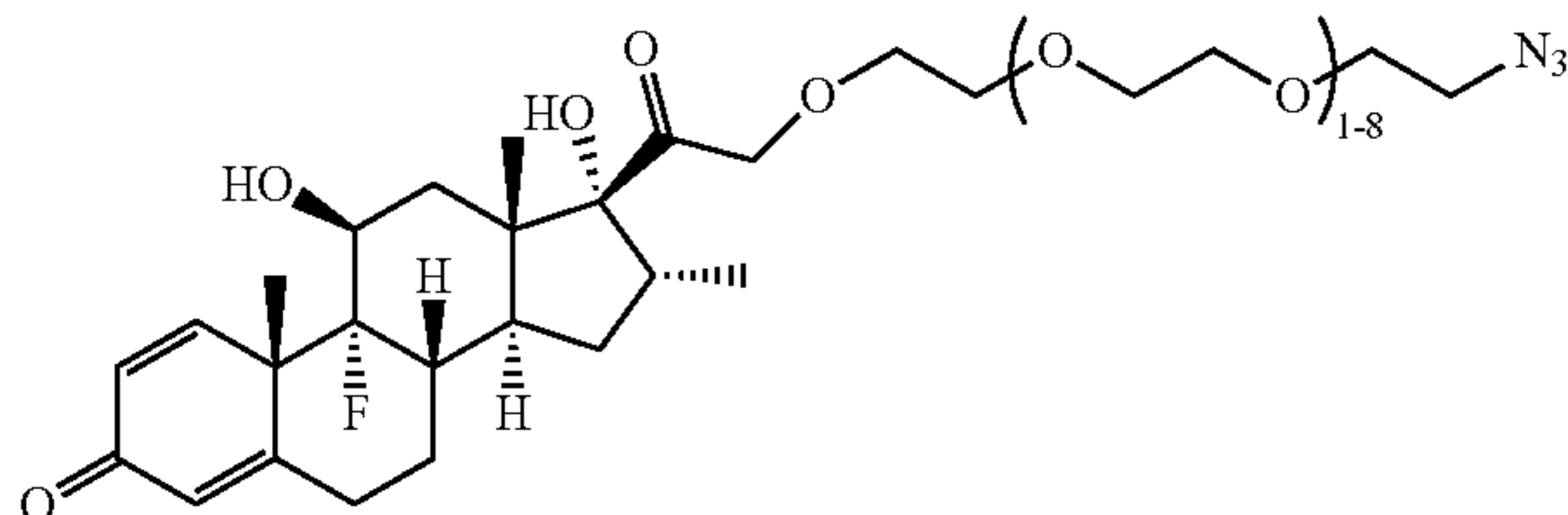
Dexamethasone analogue
