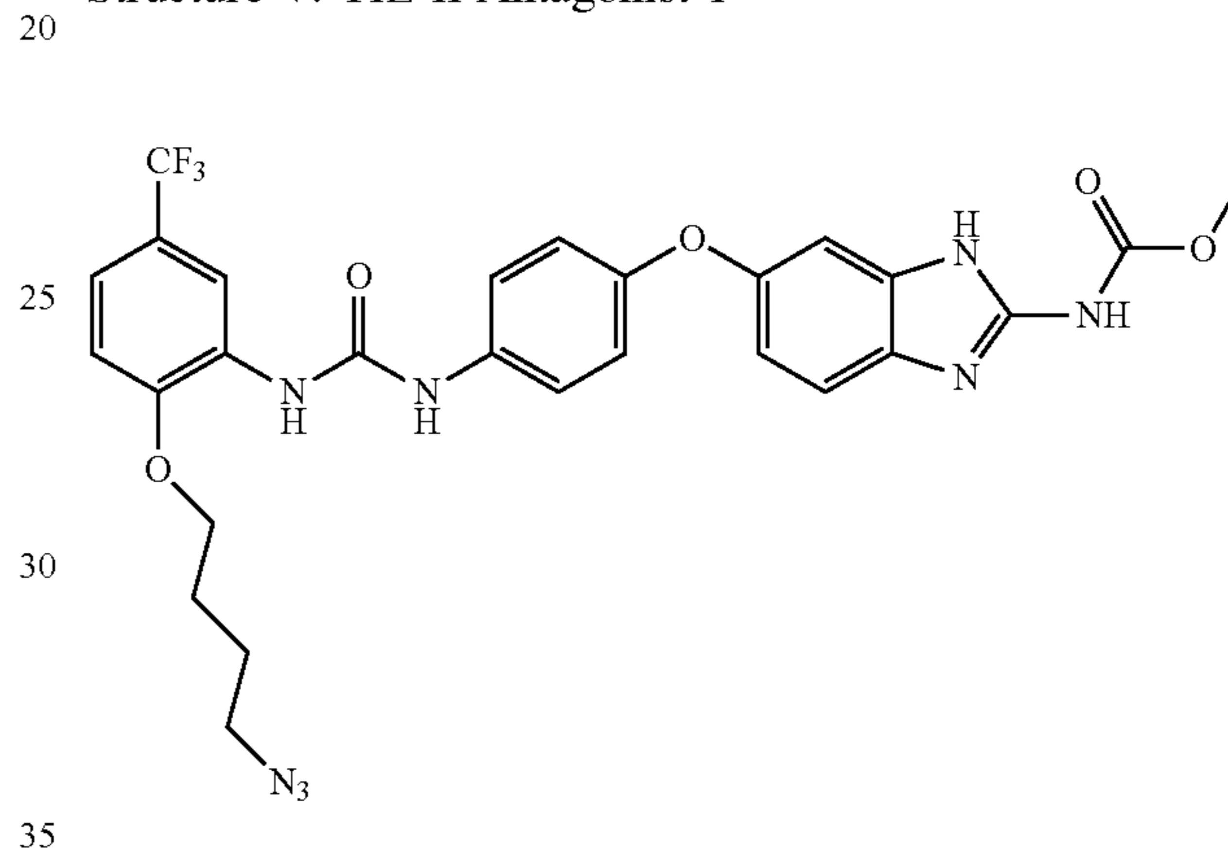
Structure V: TIE II Antagonist 1
