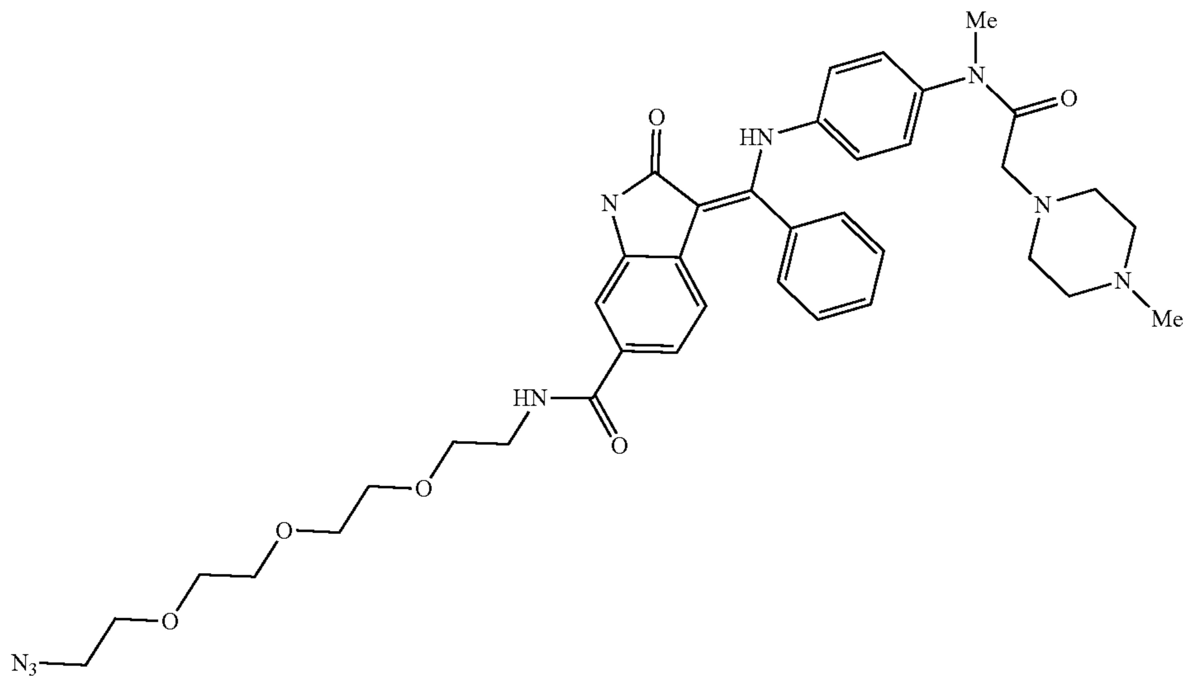
Nintedanib-amide-linker azide
