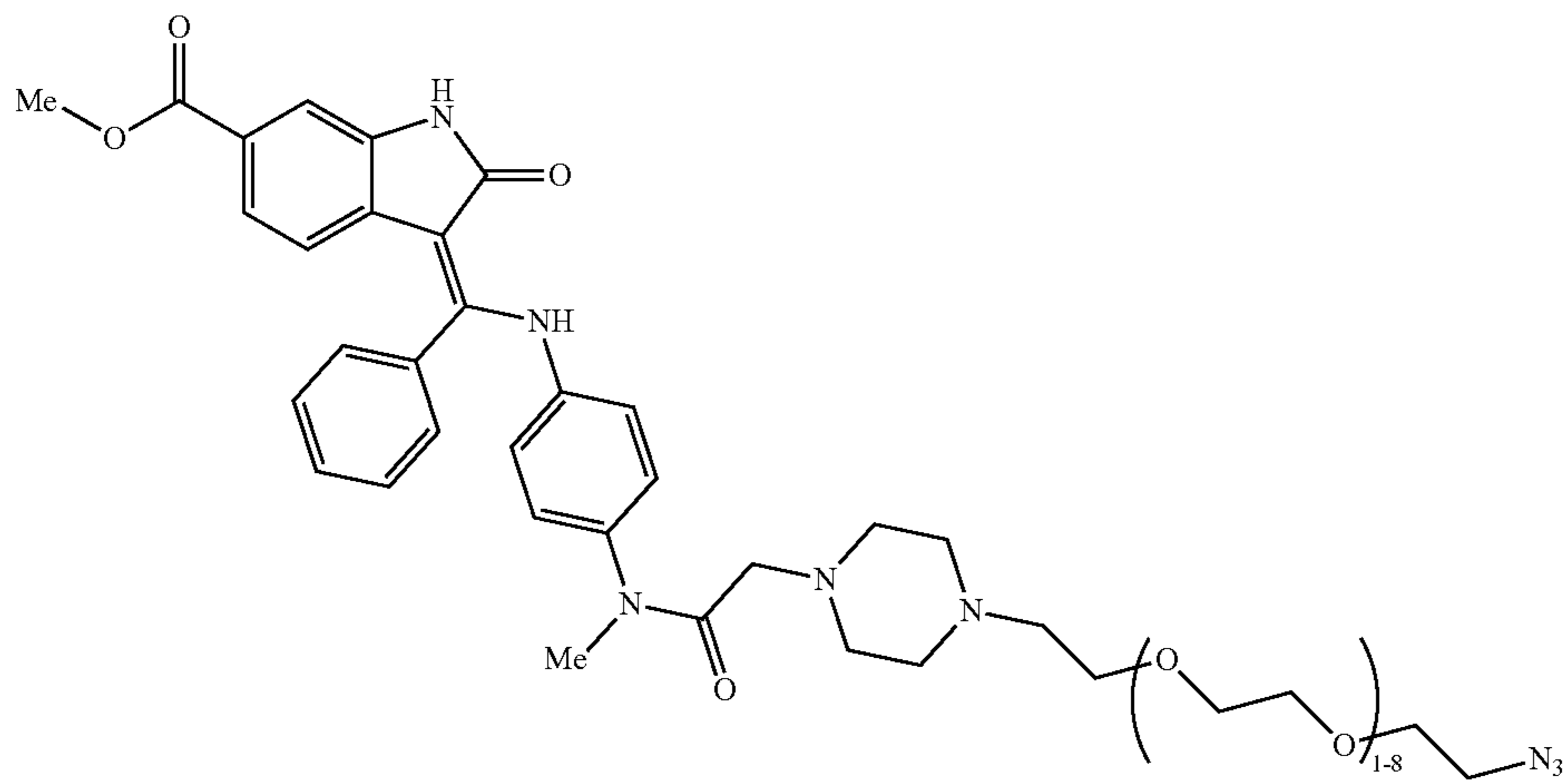
Nintedanib-amide-linker azide
