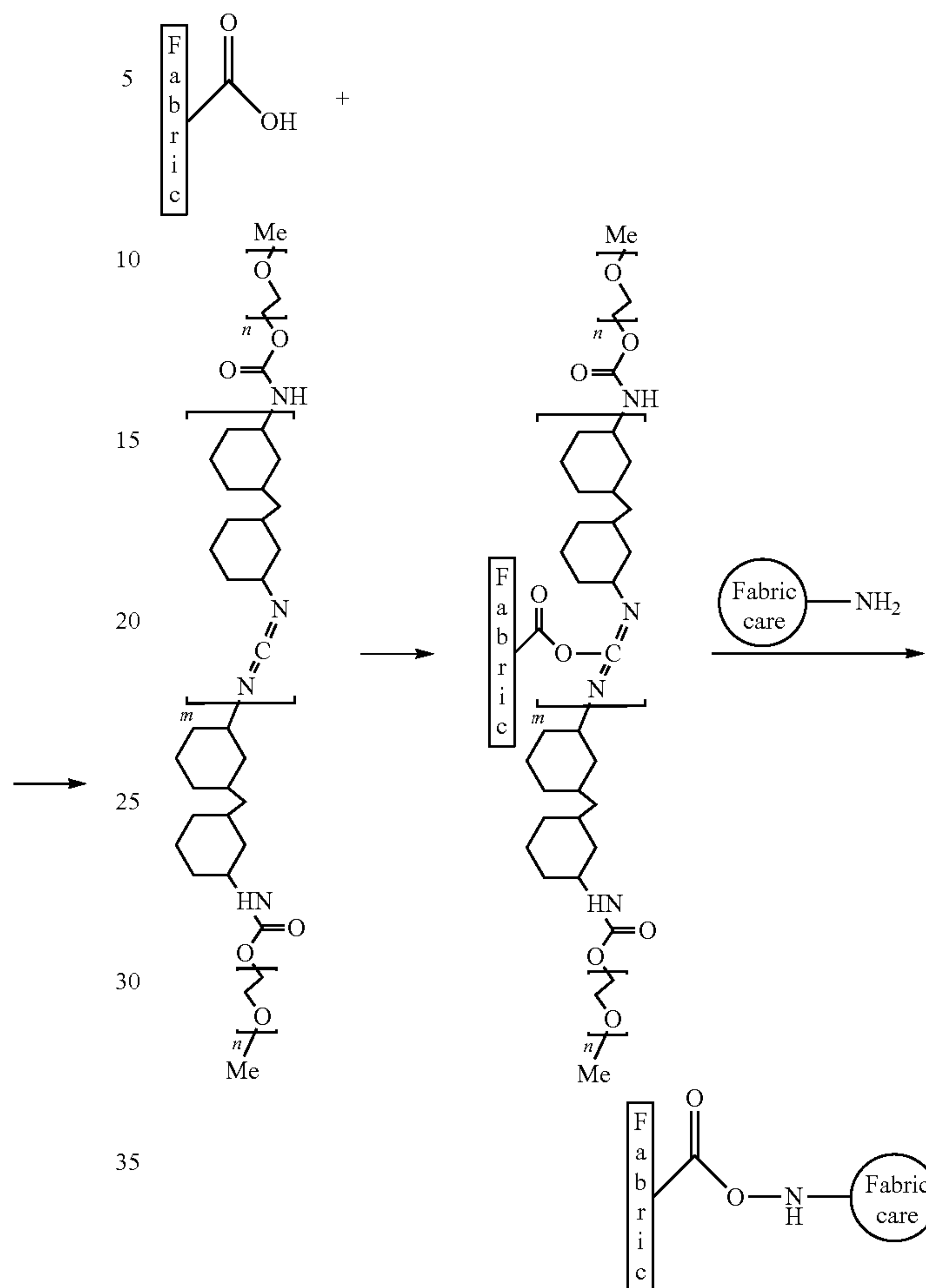
[Reaction Scheme 6]
