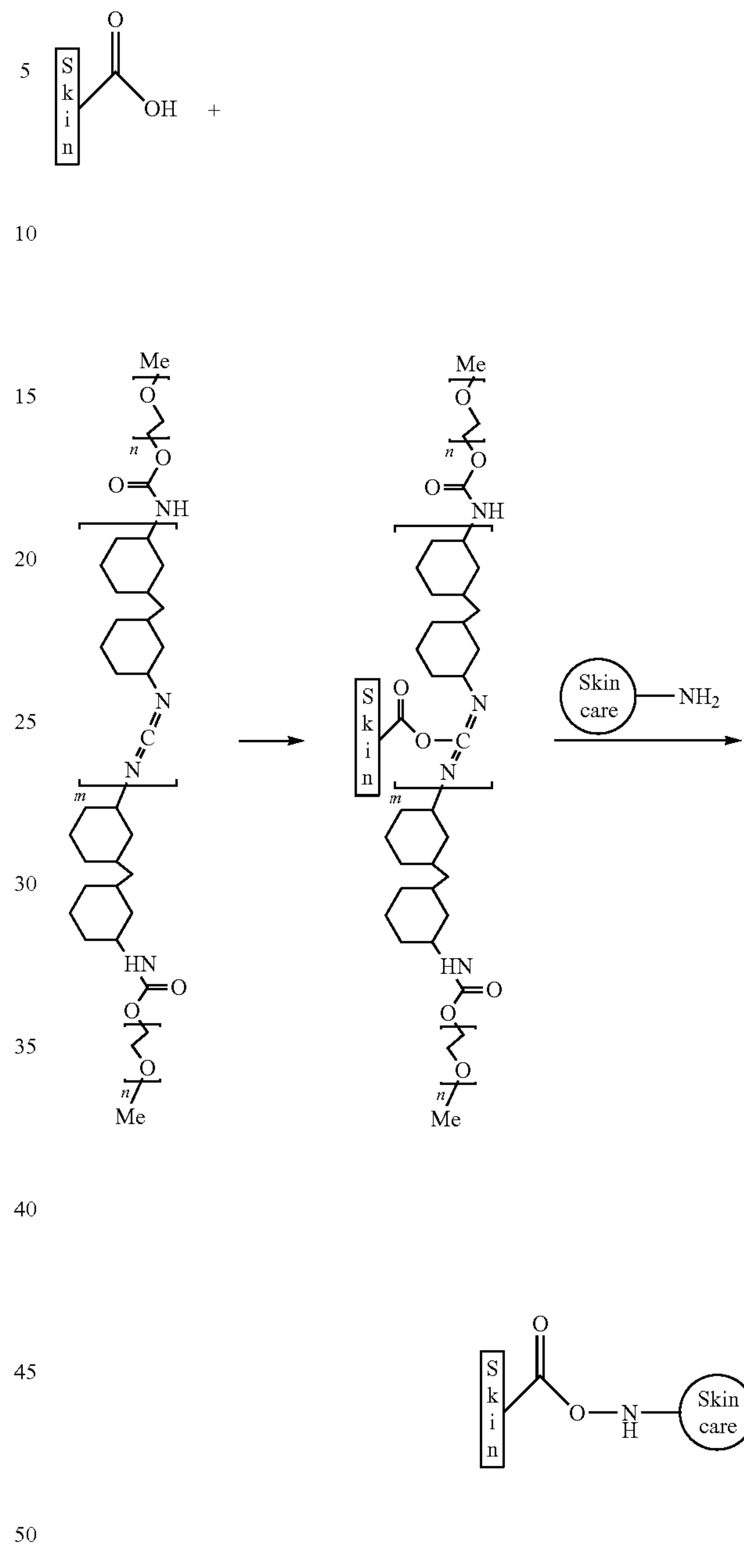
[Reaction Scheme 2]
