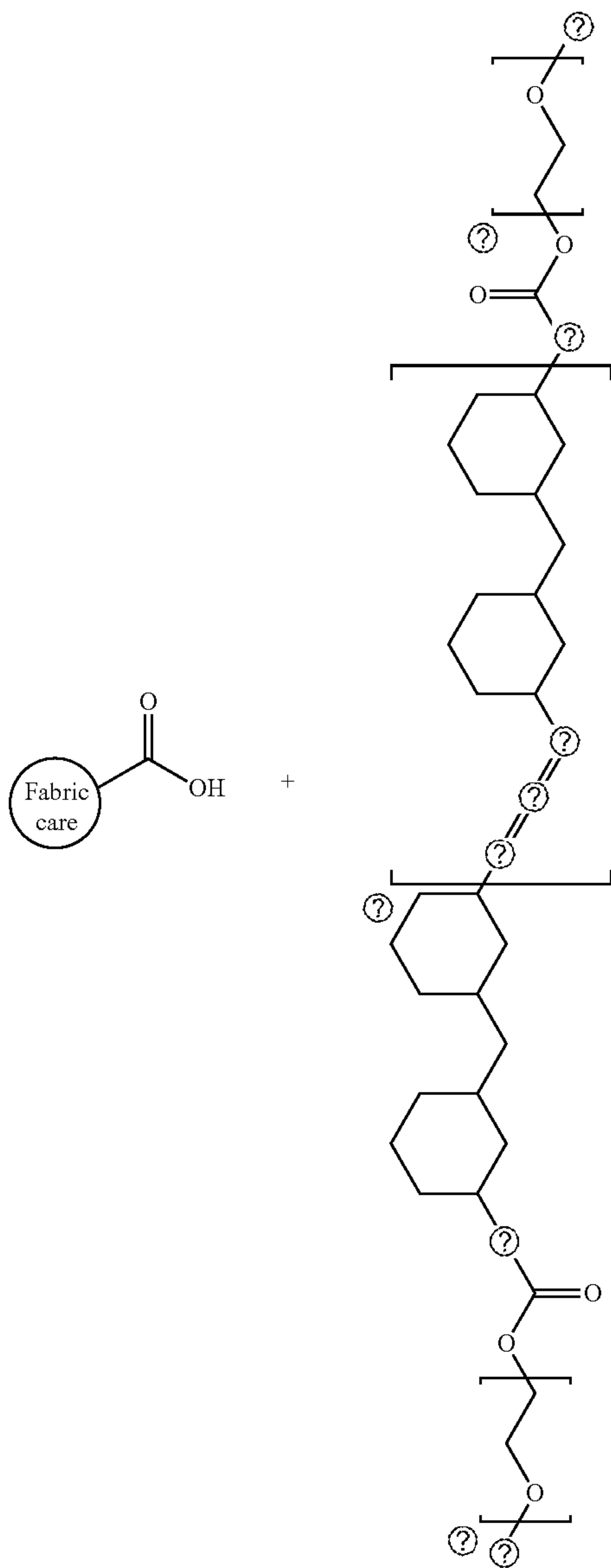
[Reaction Scheme 5]
