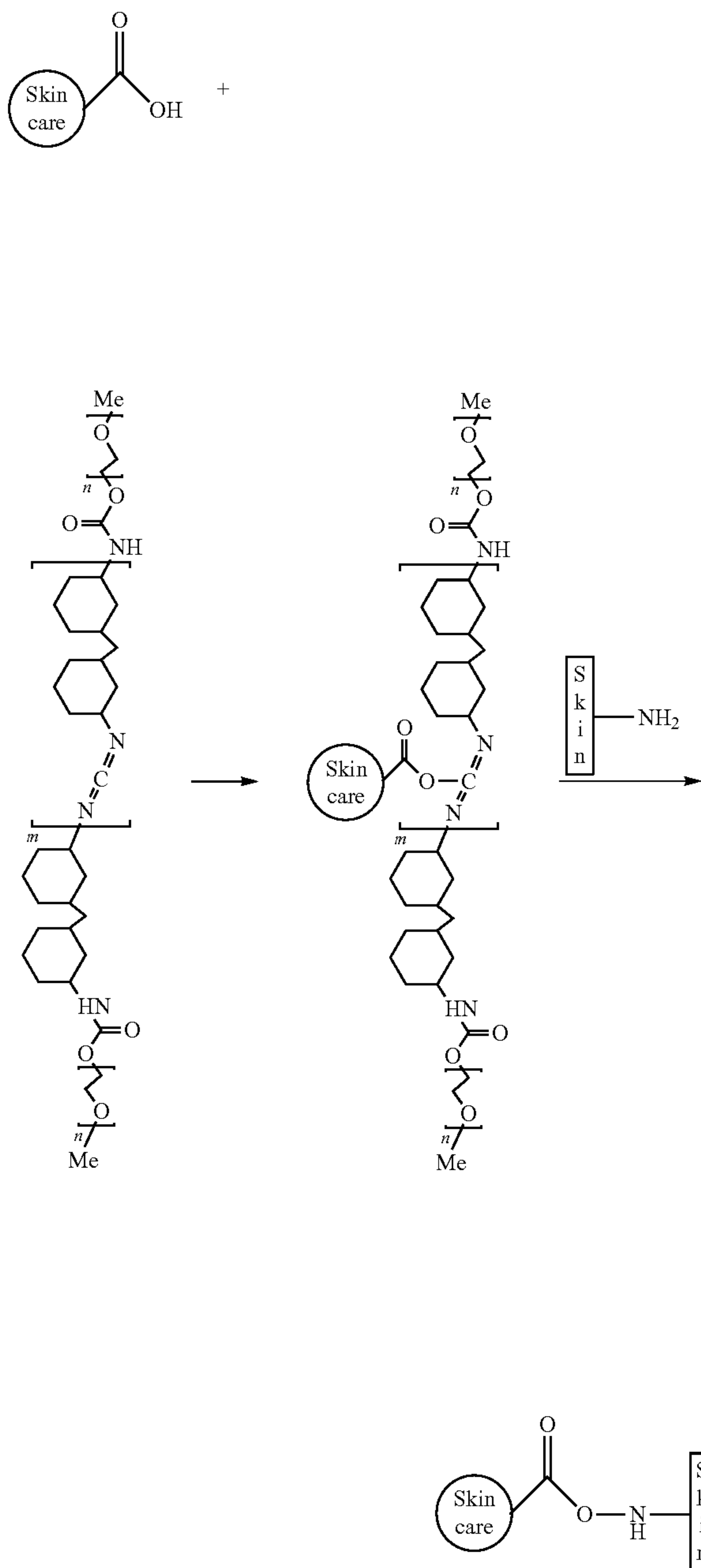
[Reaction Scheme 1]
