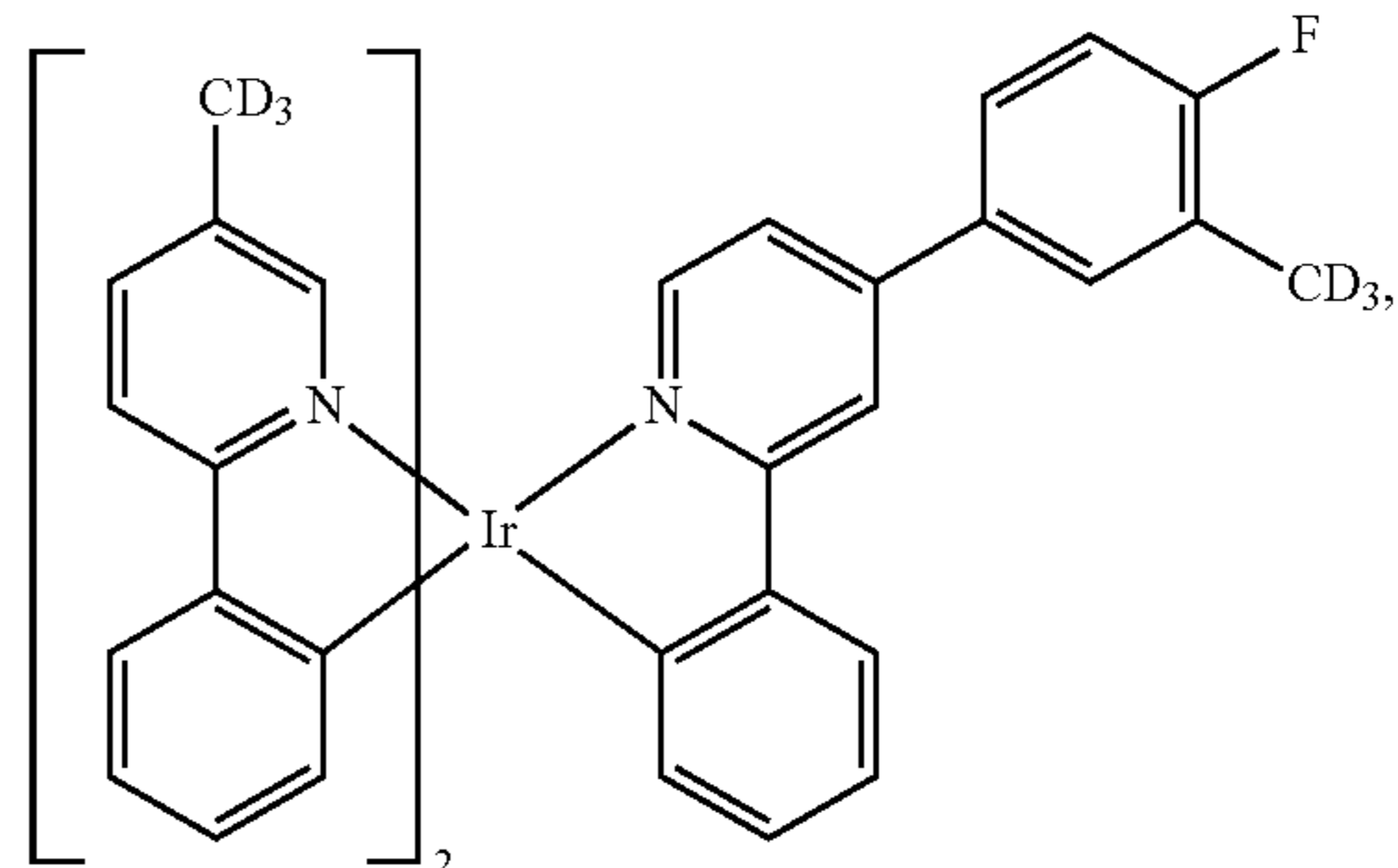
Compound 126
