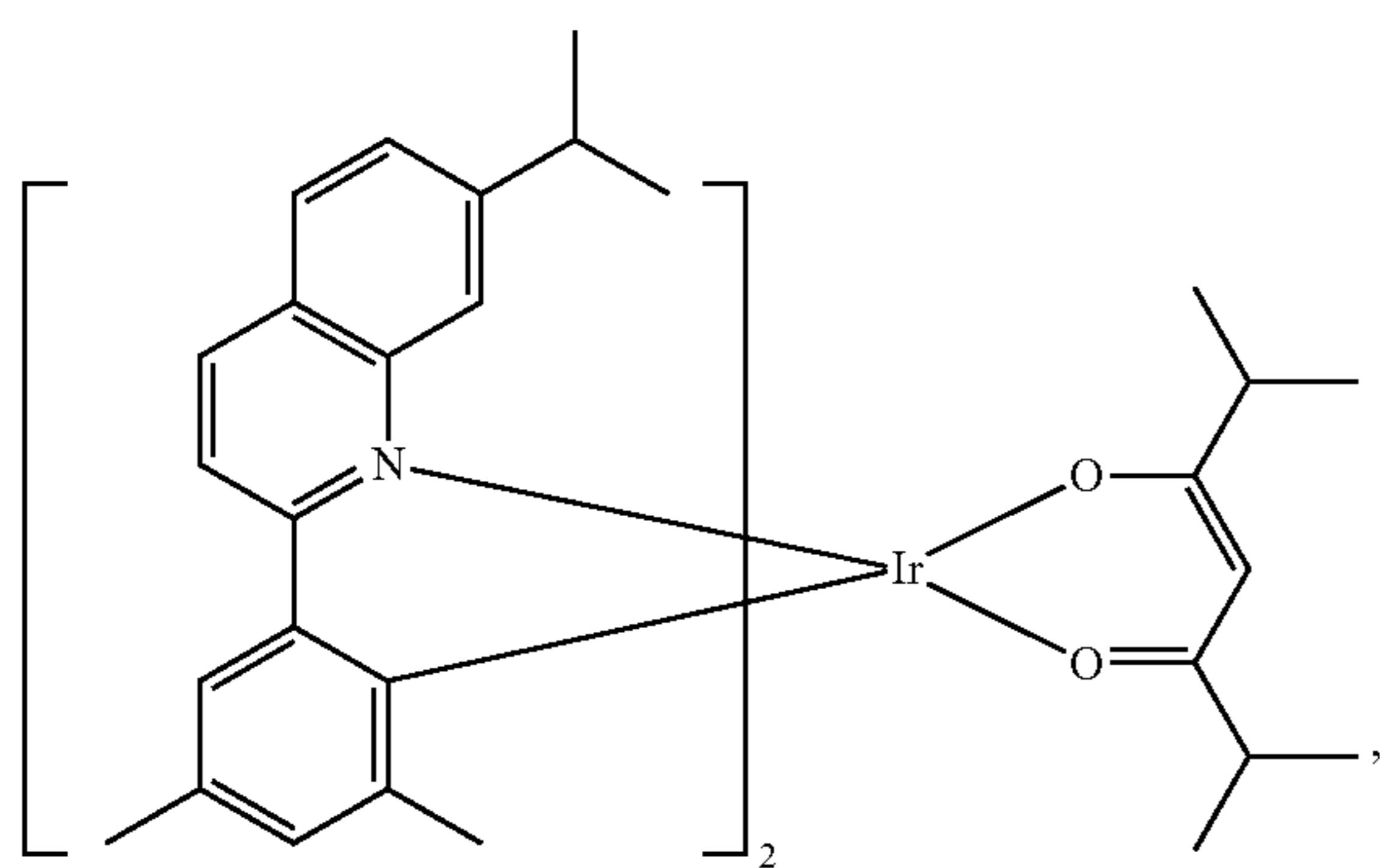
Compound E35
