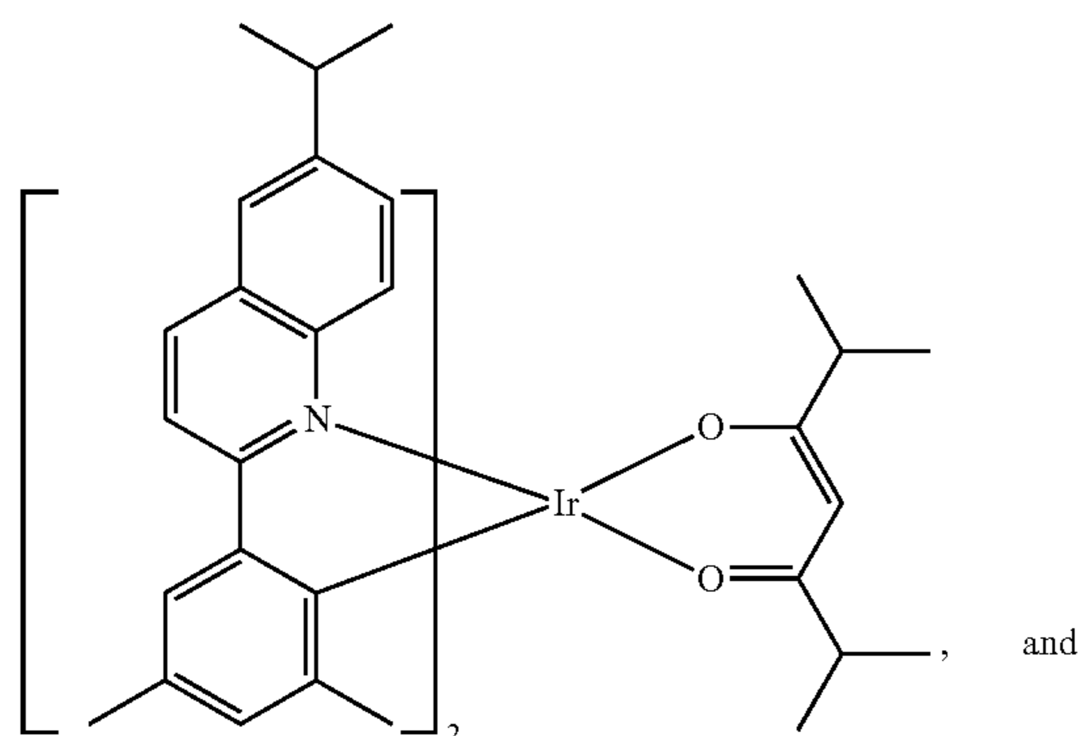
Compound E40
