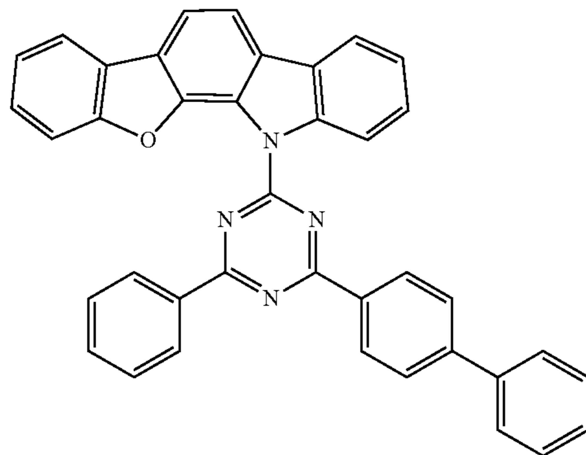
Compound EH7
