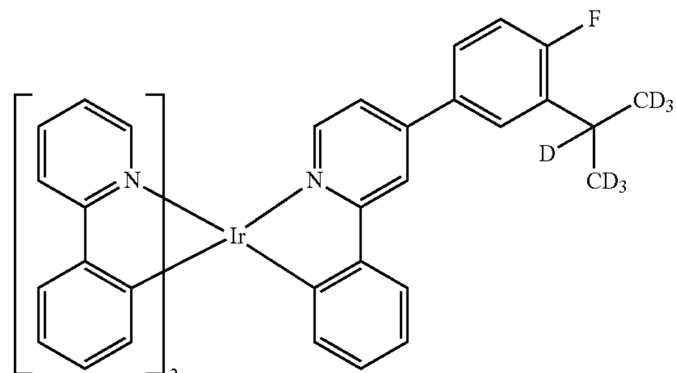
Compound 95
