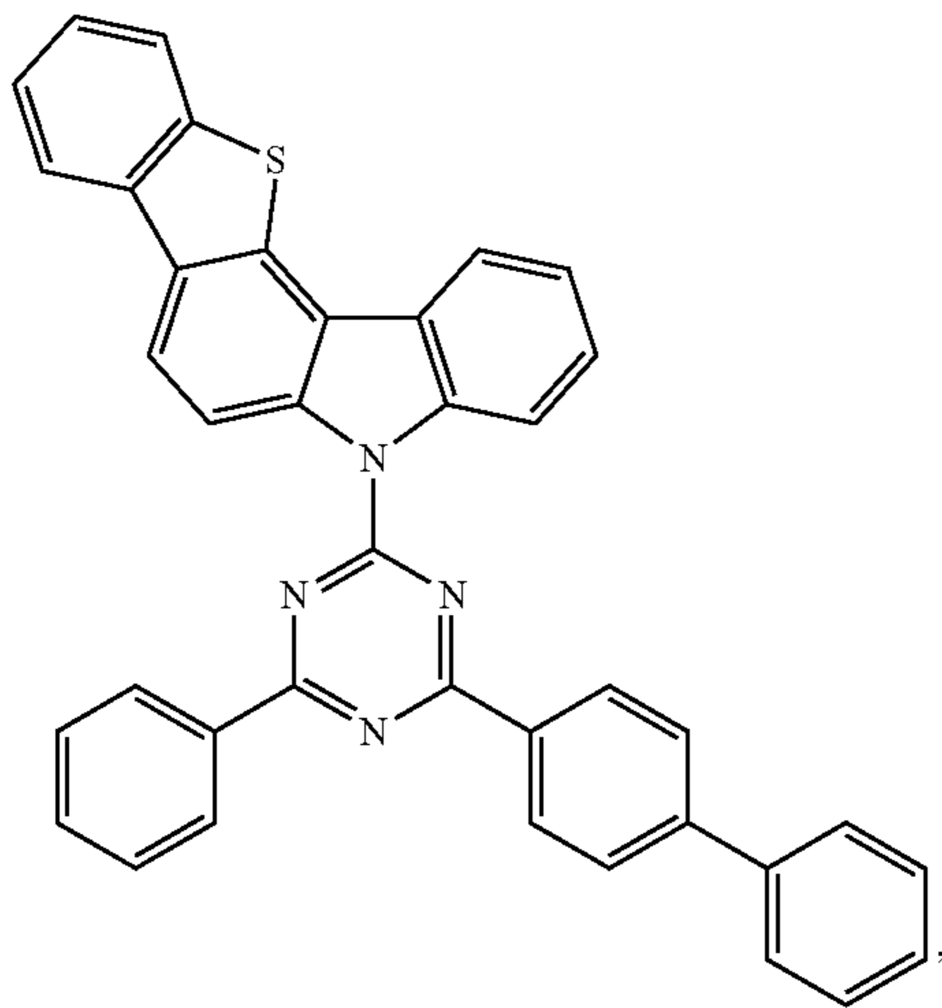
Compound EH35
