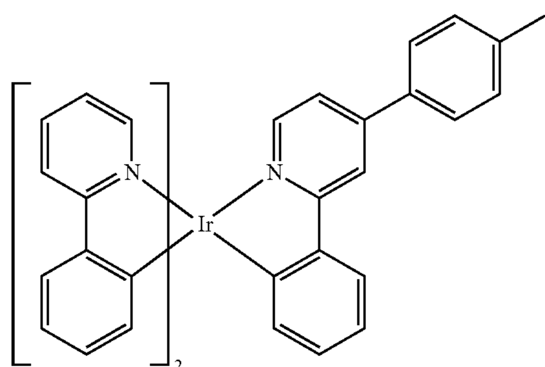
Compound 21
