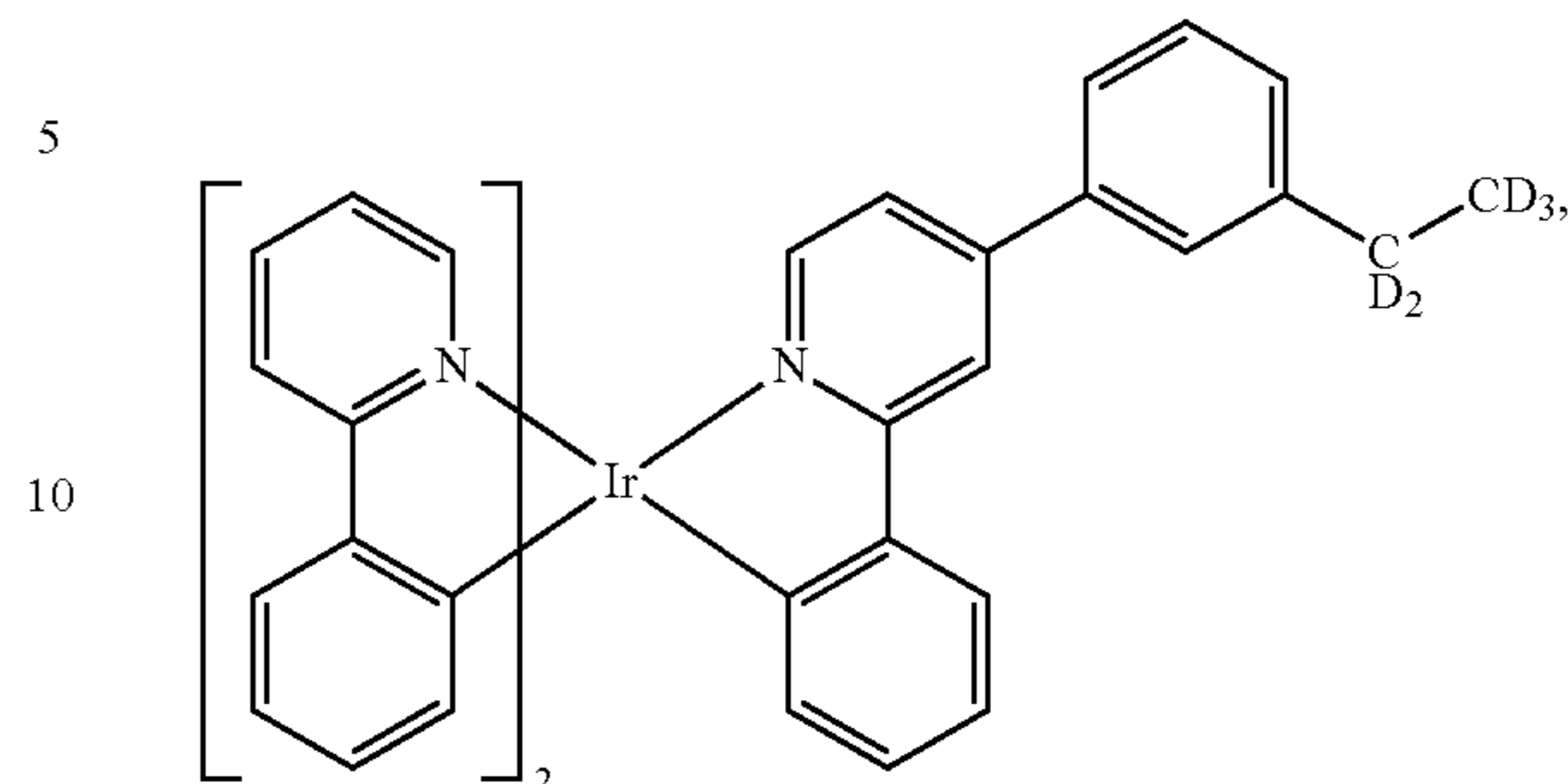
Compound 91
