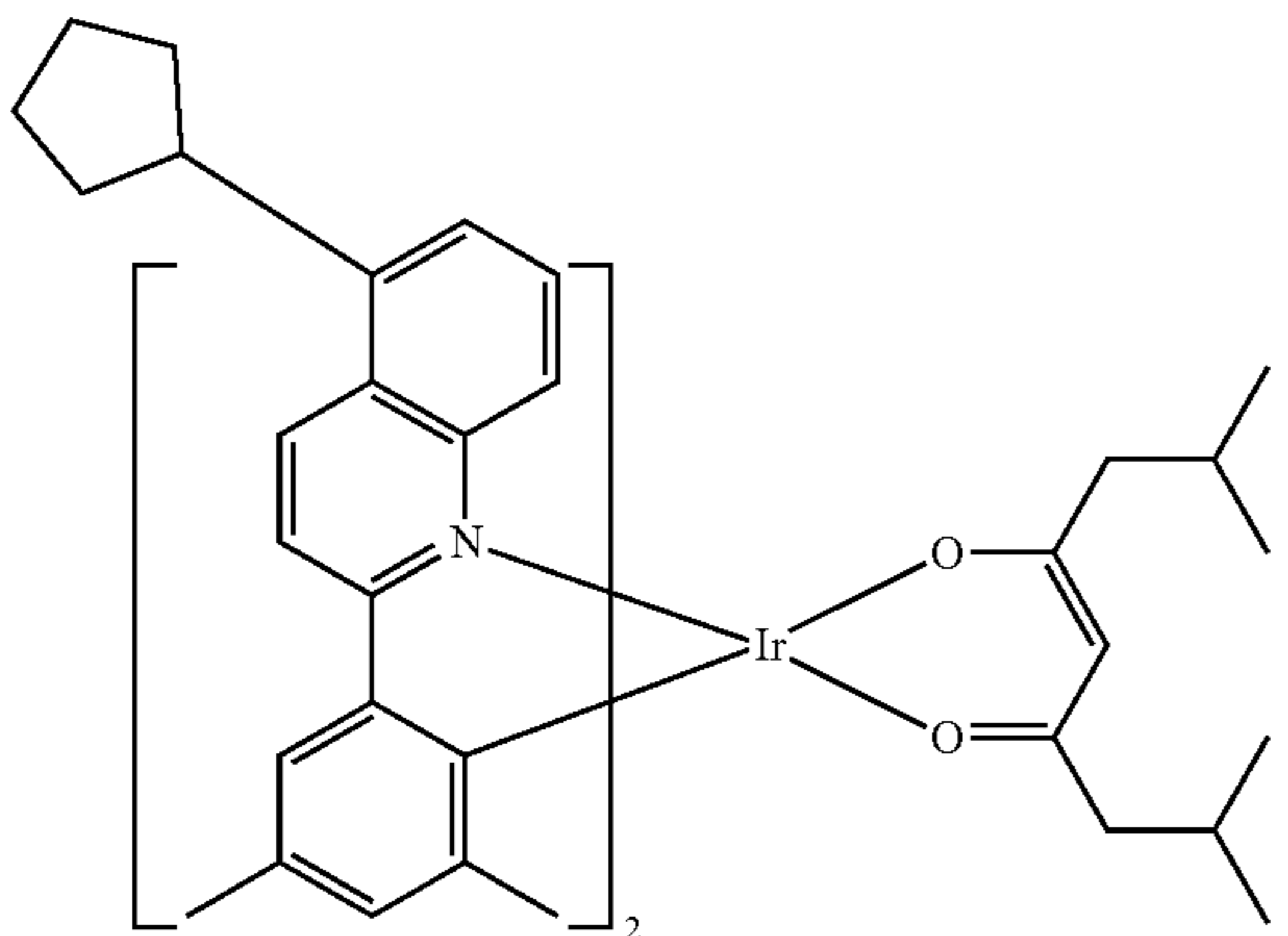
Compound E21
