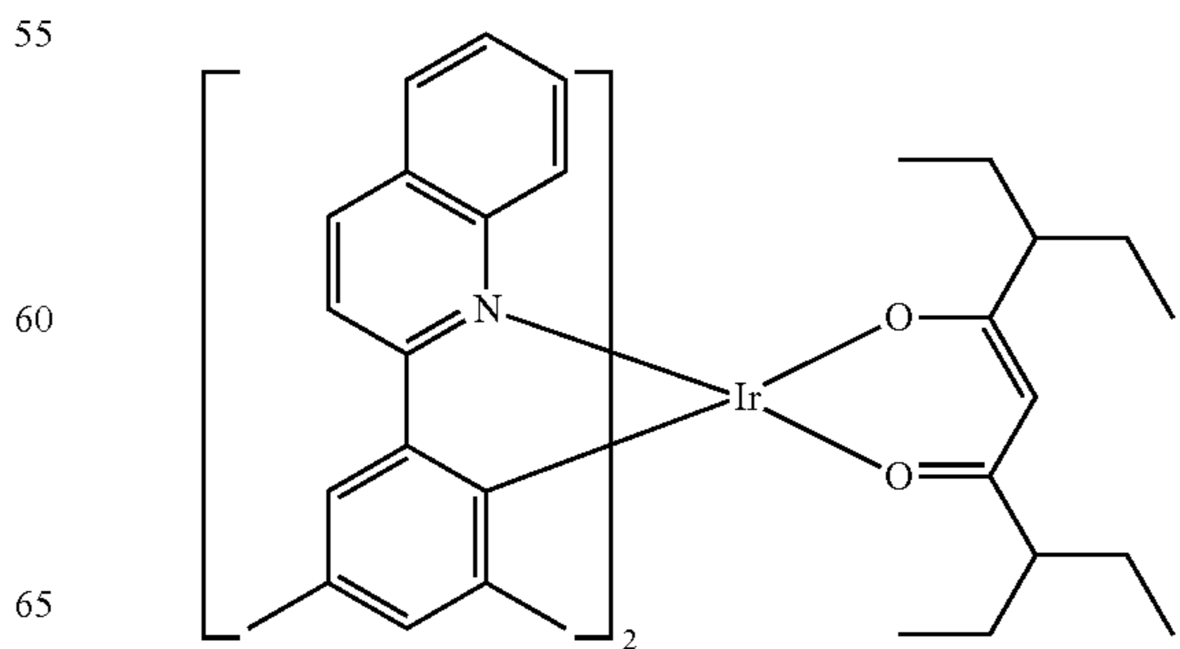
Compound E2
