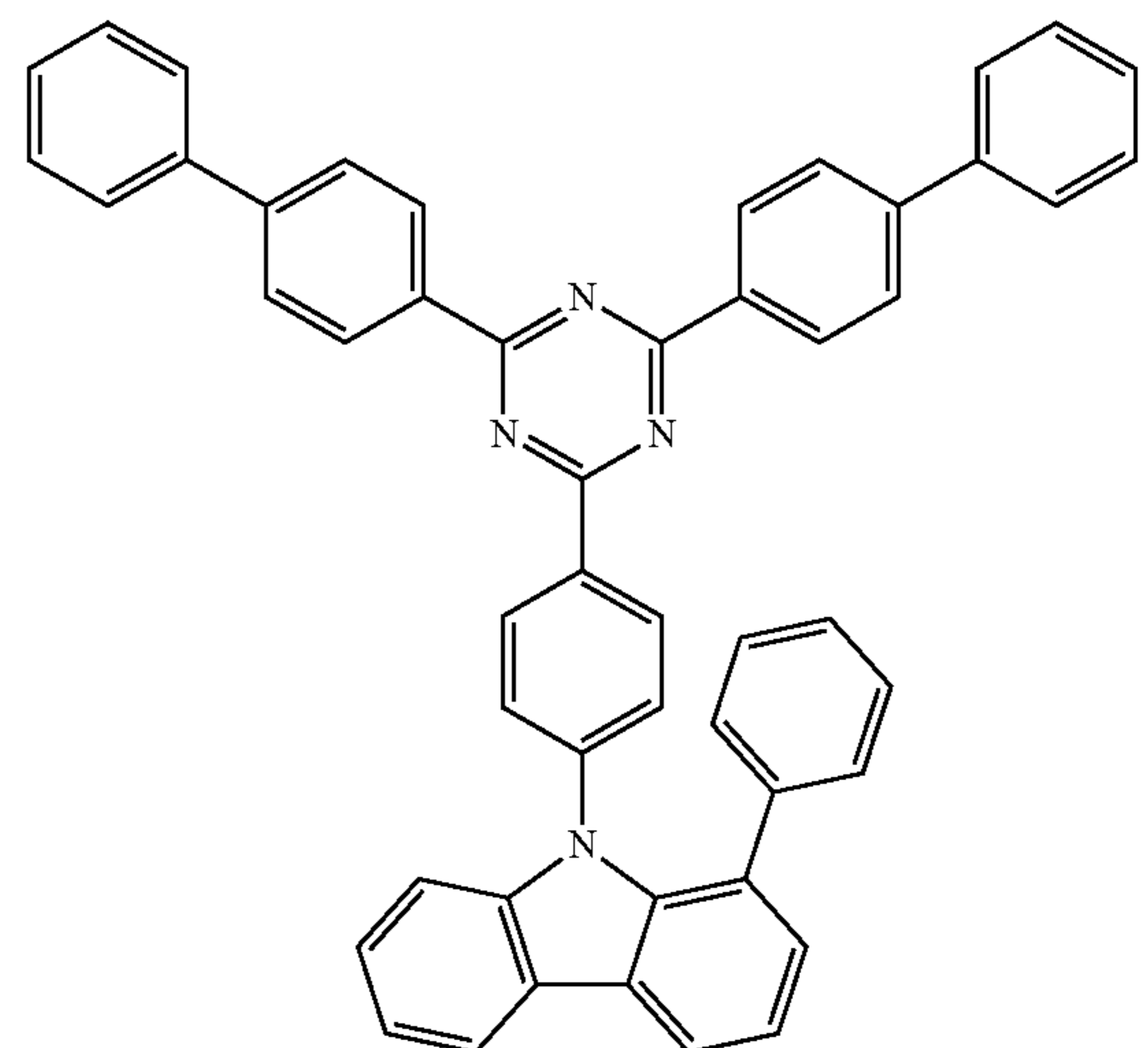
Compound H10
