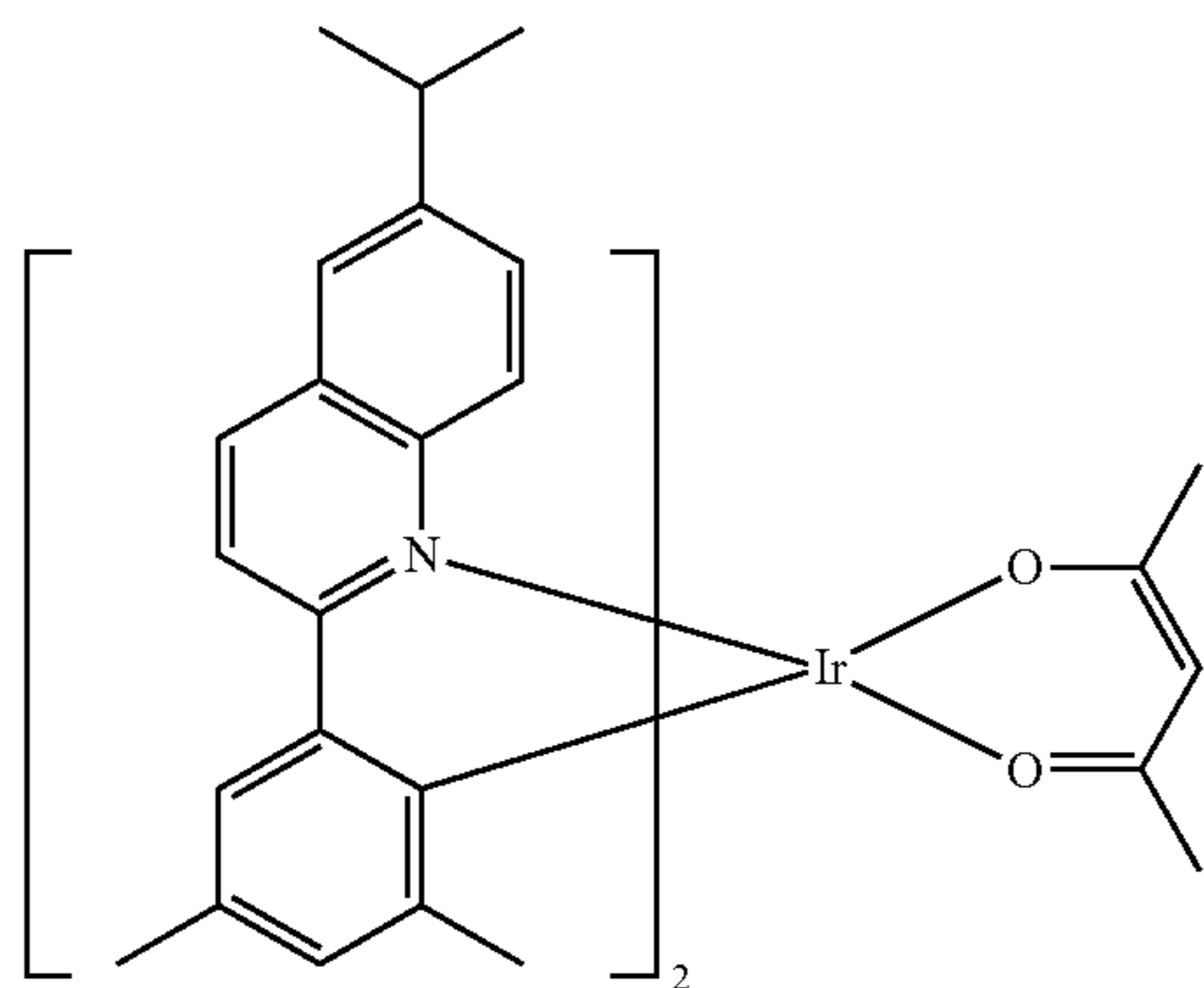
Compound E38
