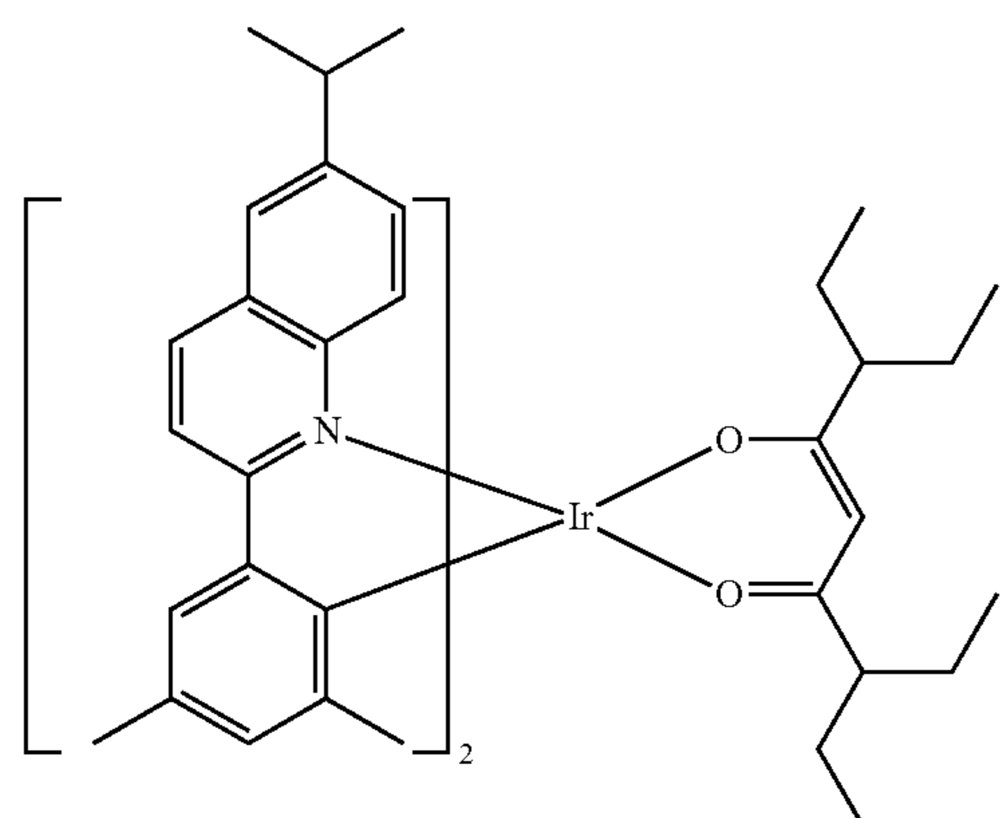
Compound E39
