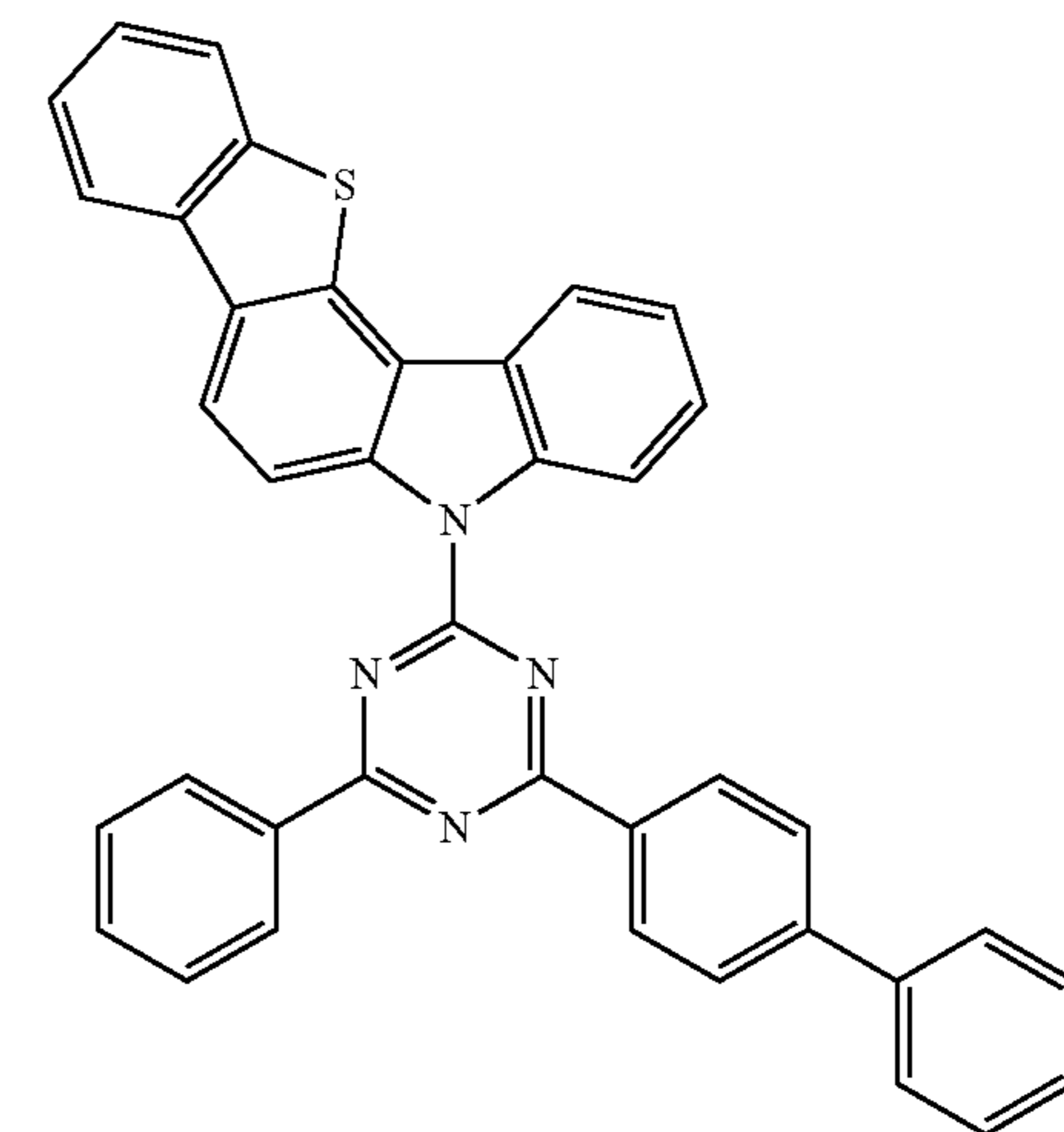
Compound EH35
