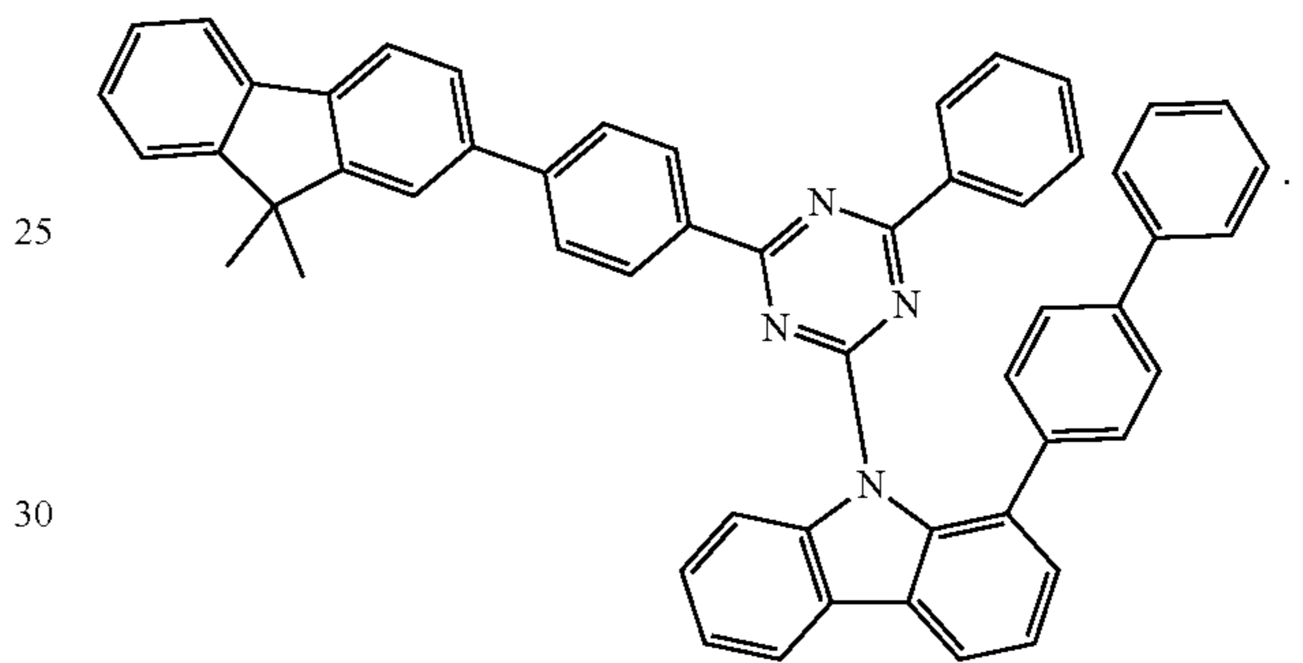
Compound H50
