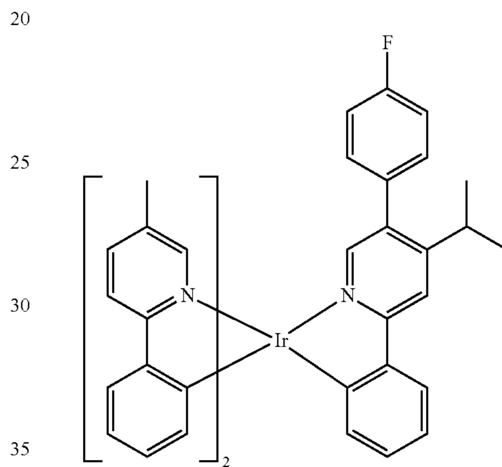
Compound 39
