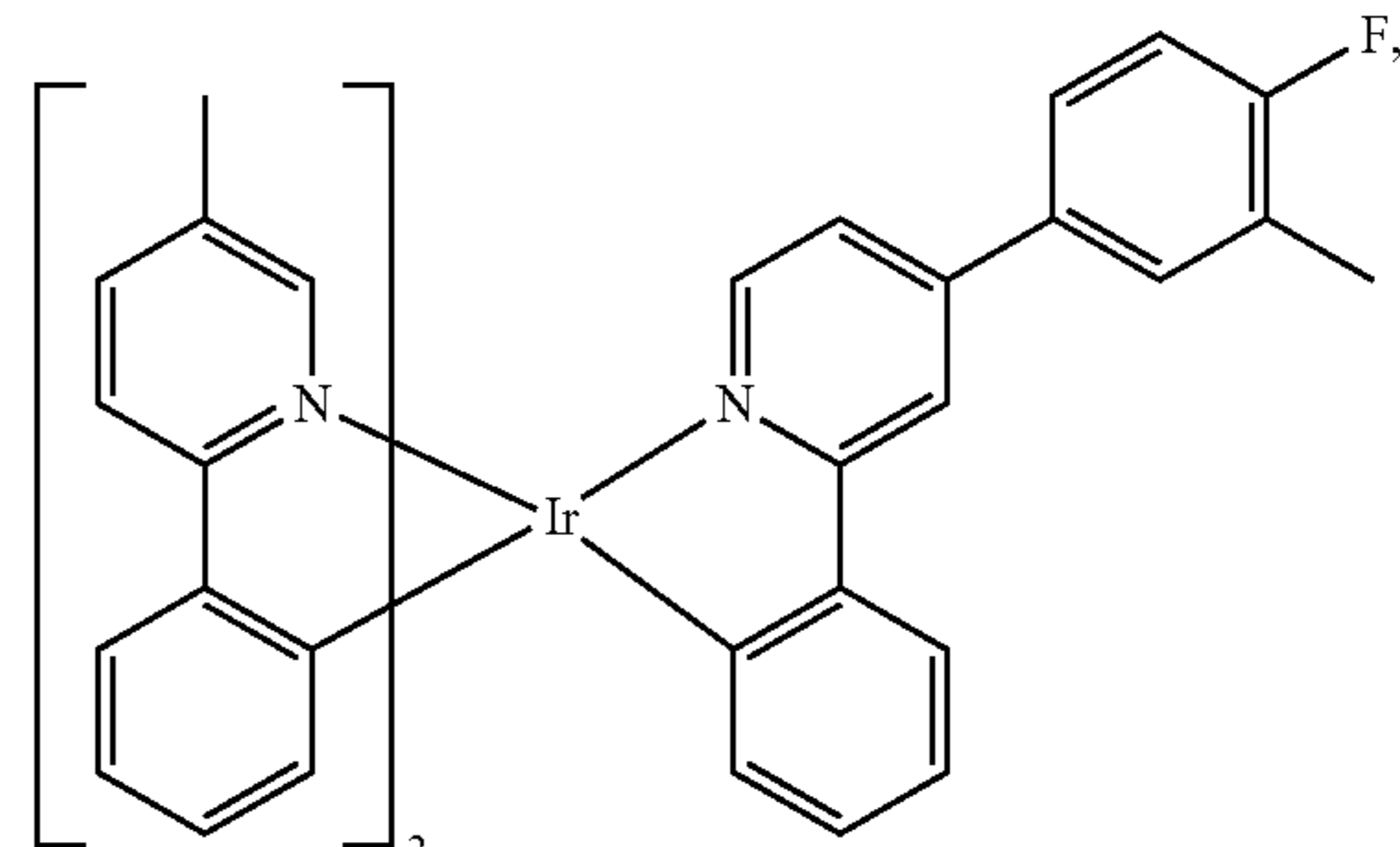
Compound 64
