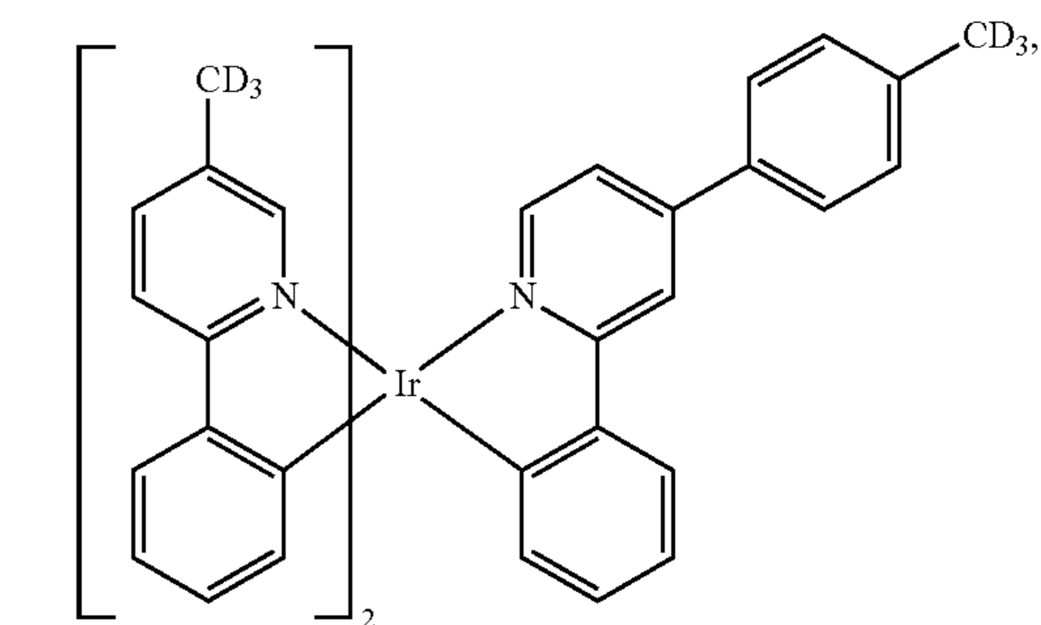
Compound 117
