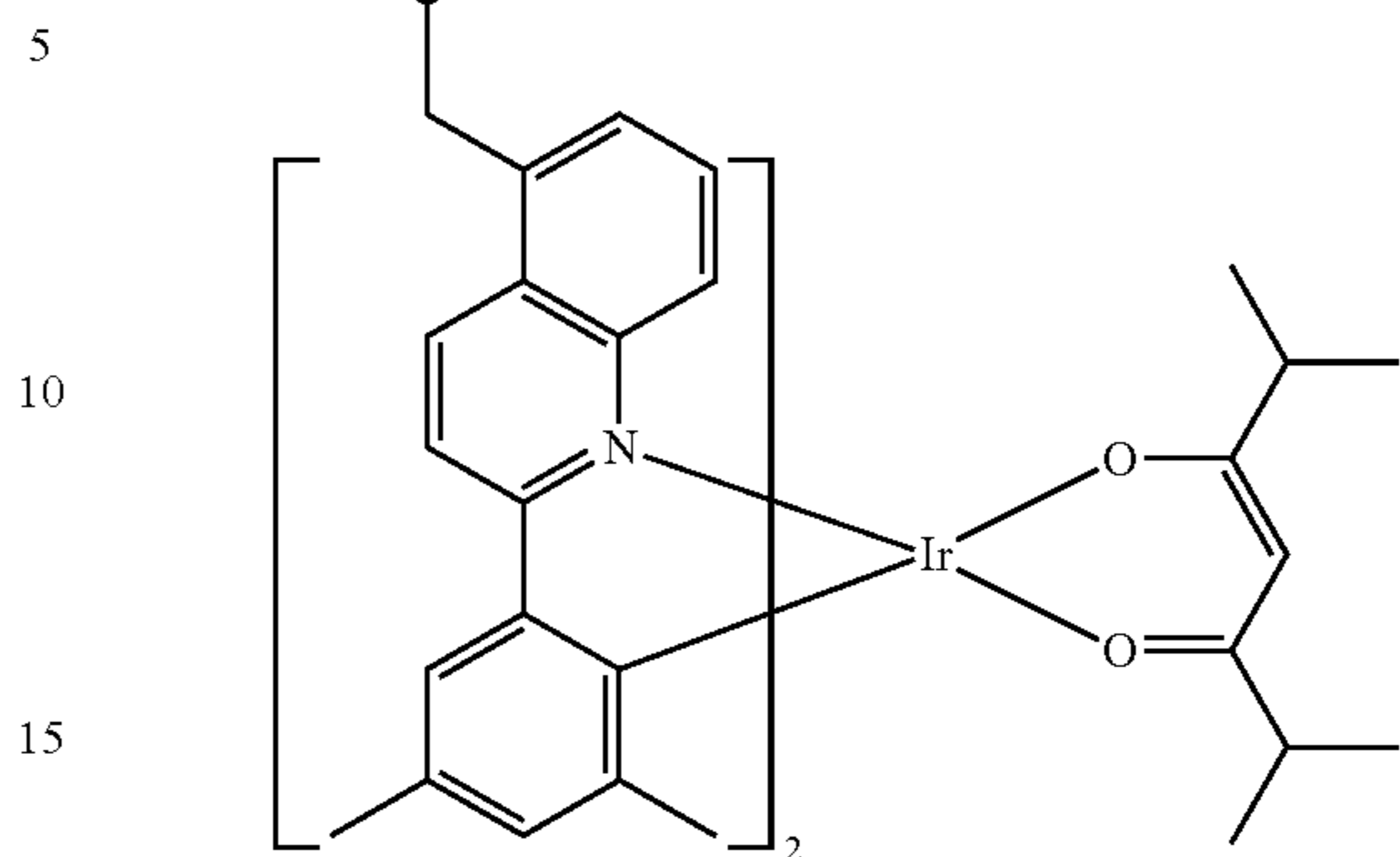
Compound E7
