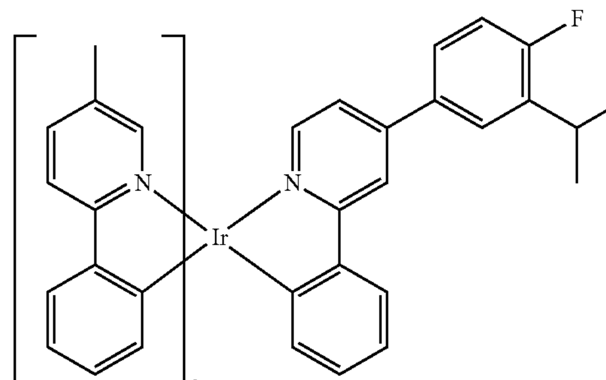
Compound 65
