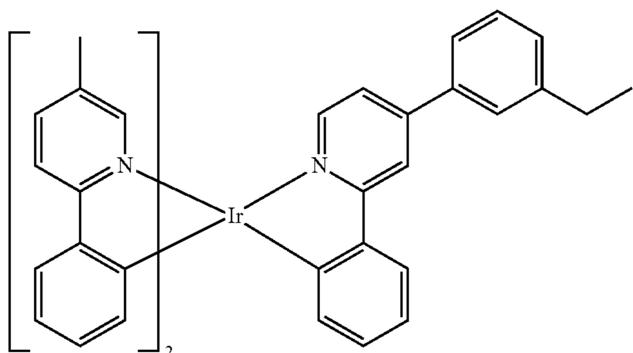
Compound 60
