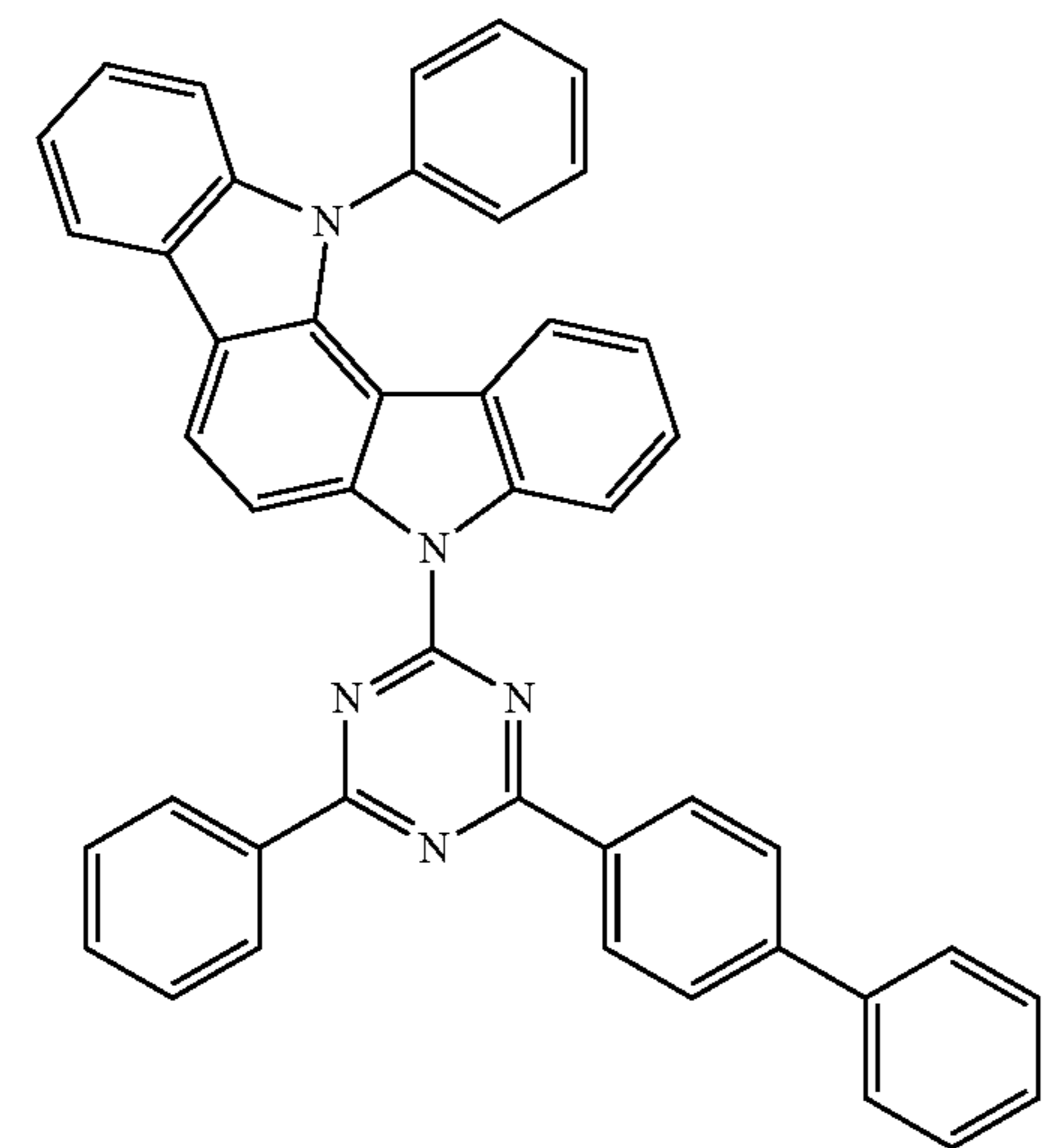
Compound EH32
