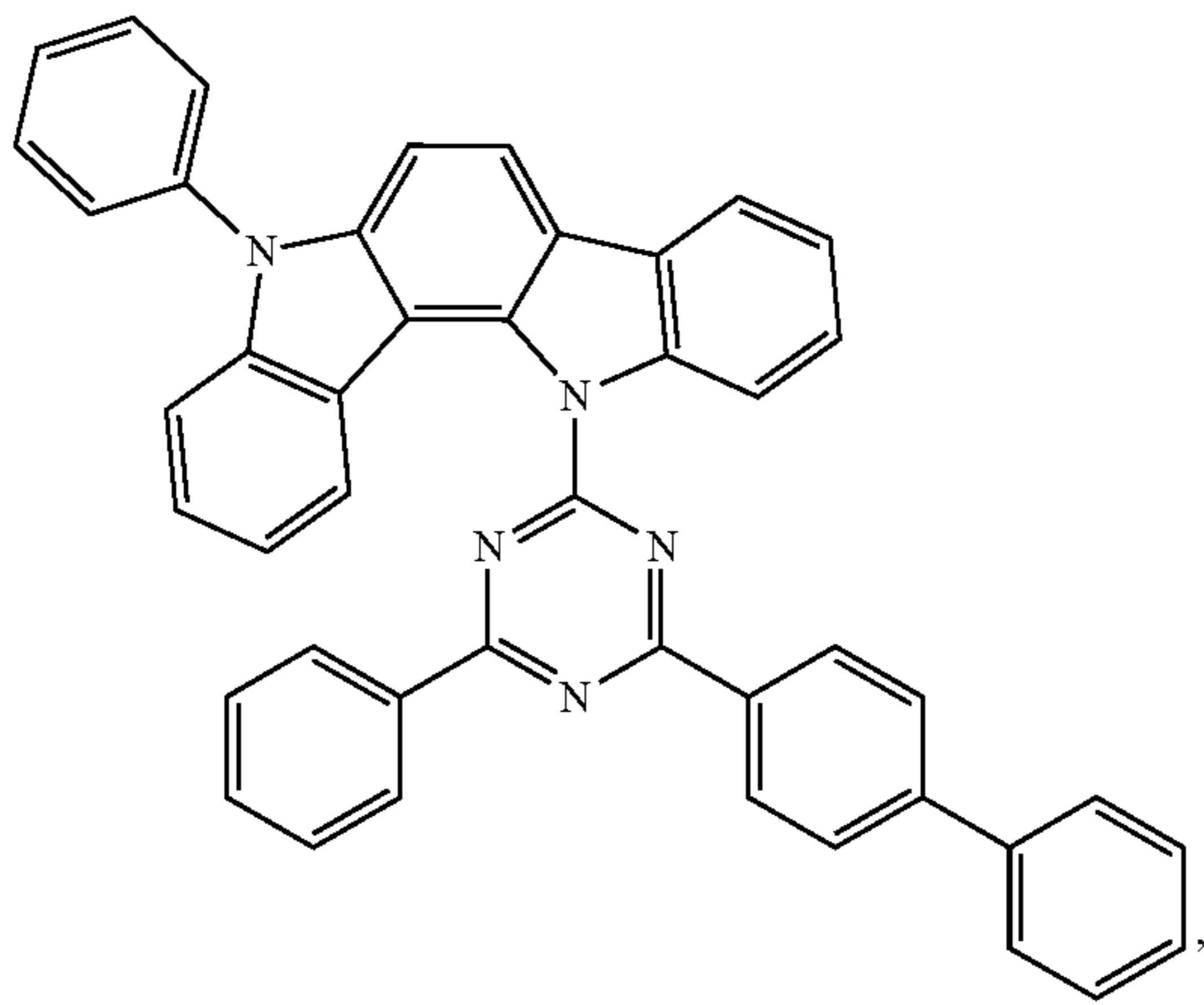
Compound EH42
