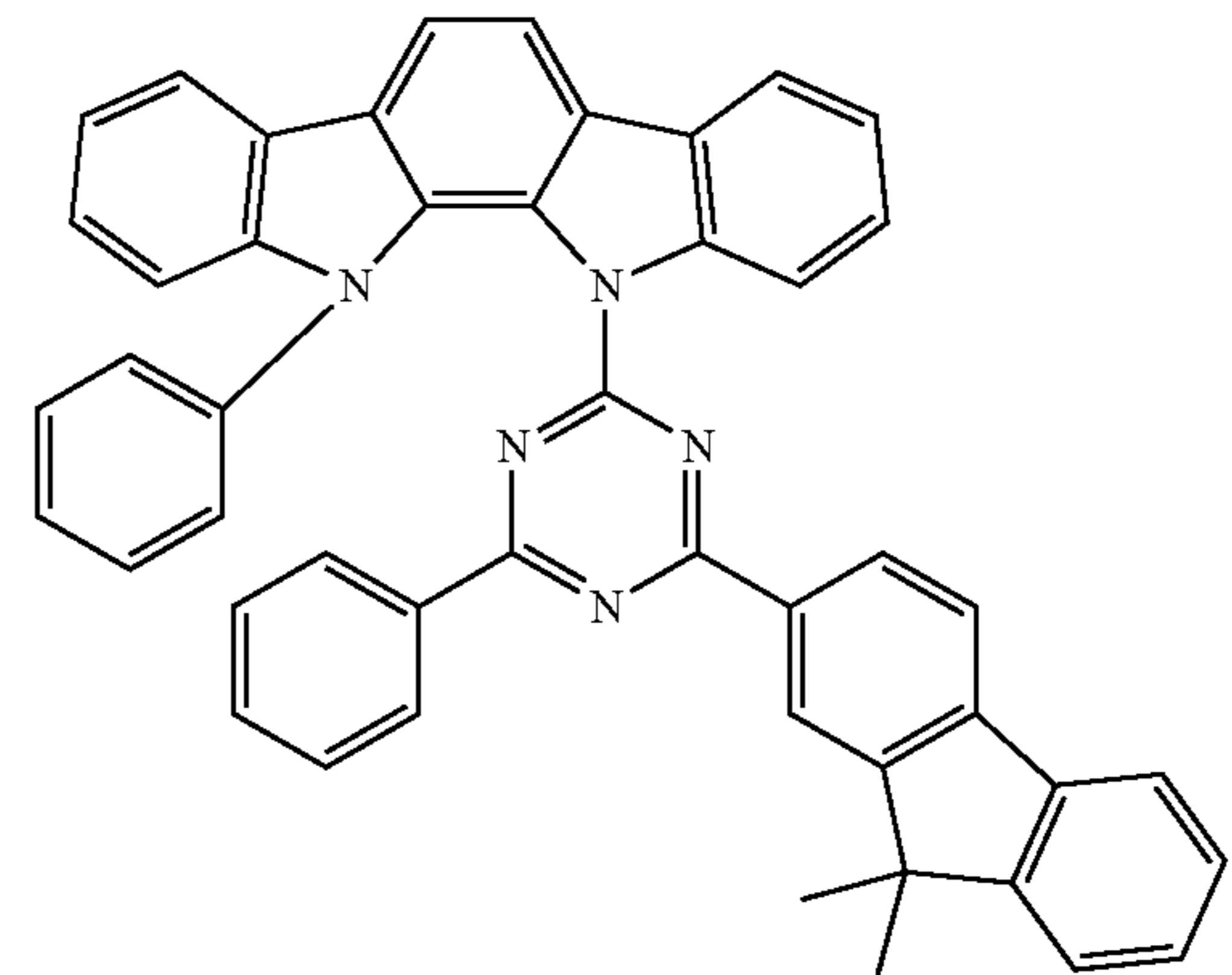
Compound EH6
