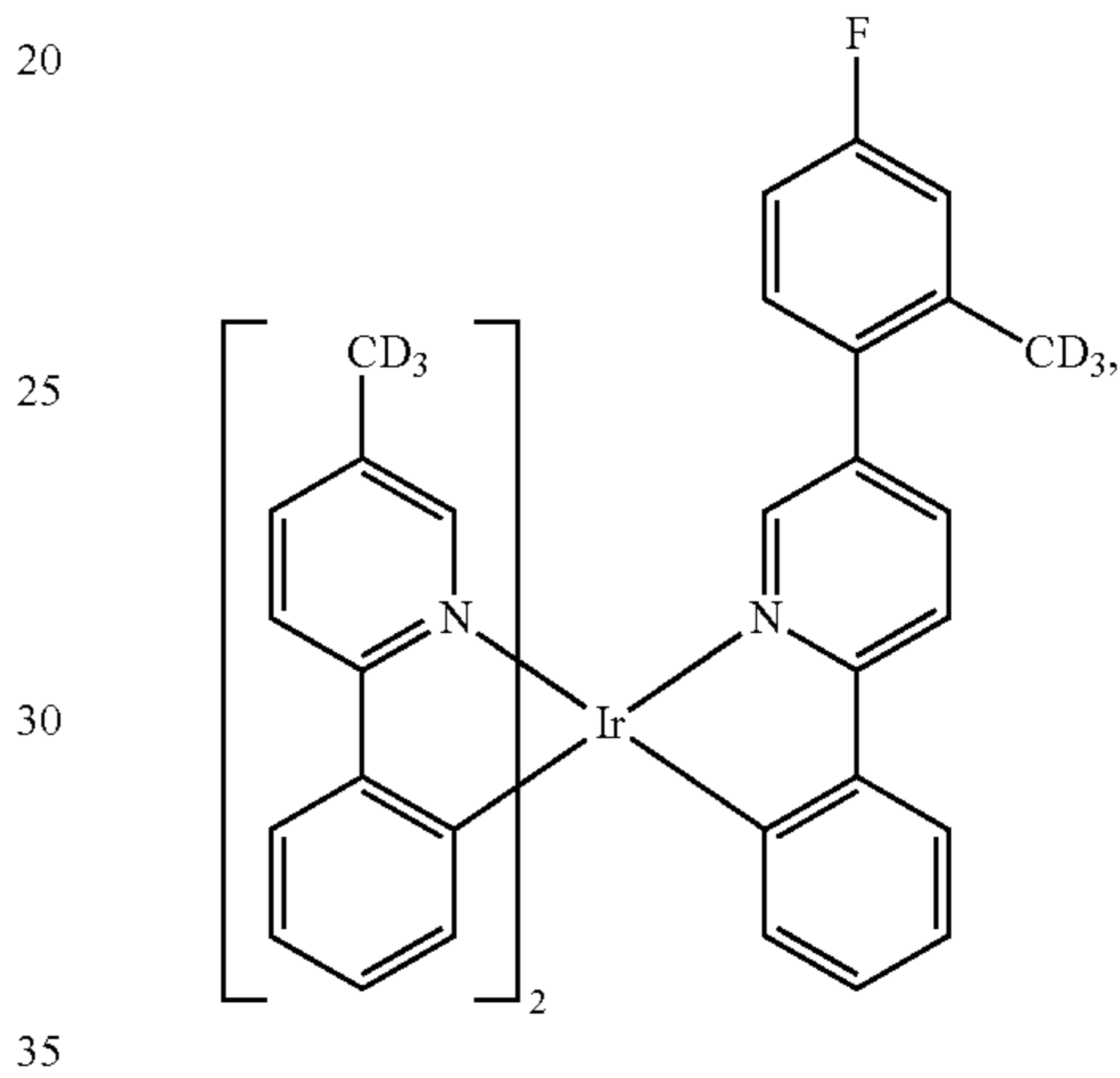
Compound 111
