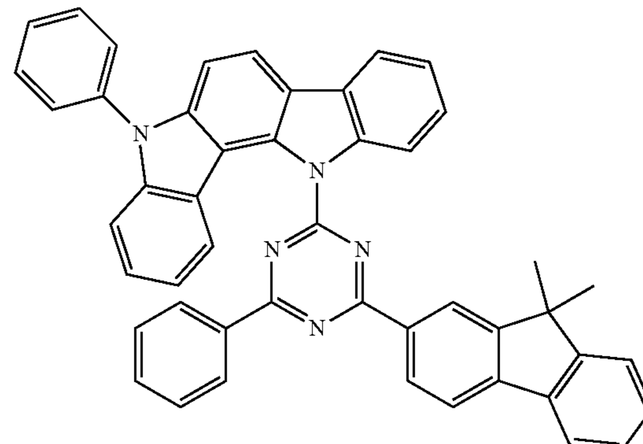
Compound EH42
