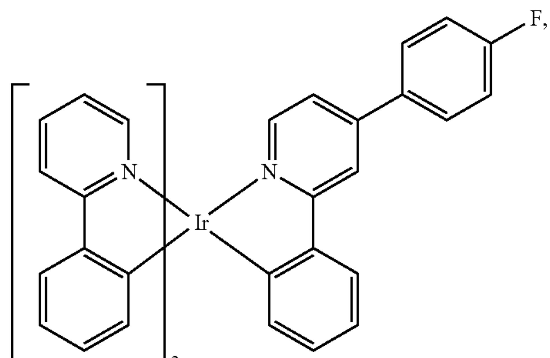
Compound 30
