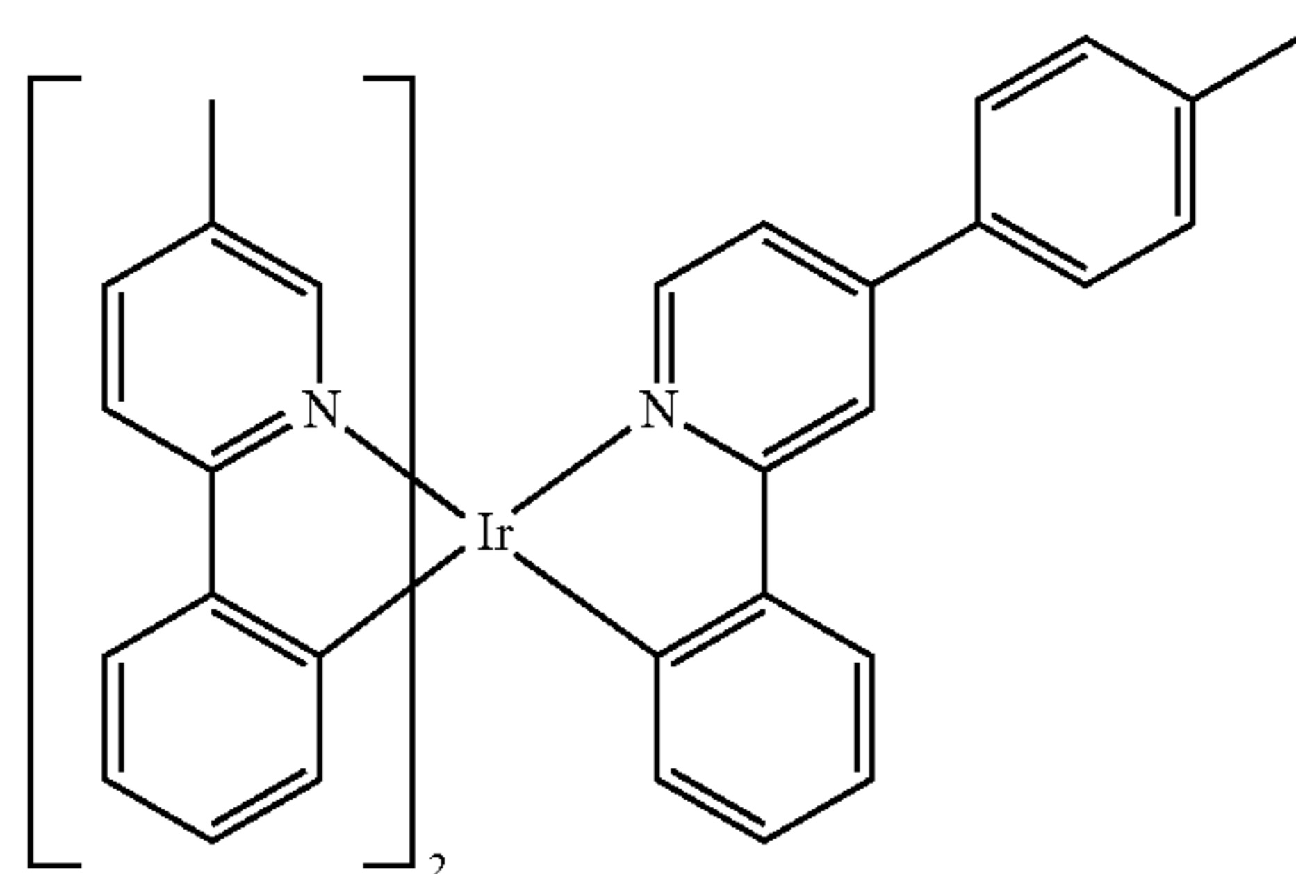
Compound 54
