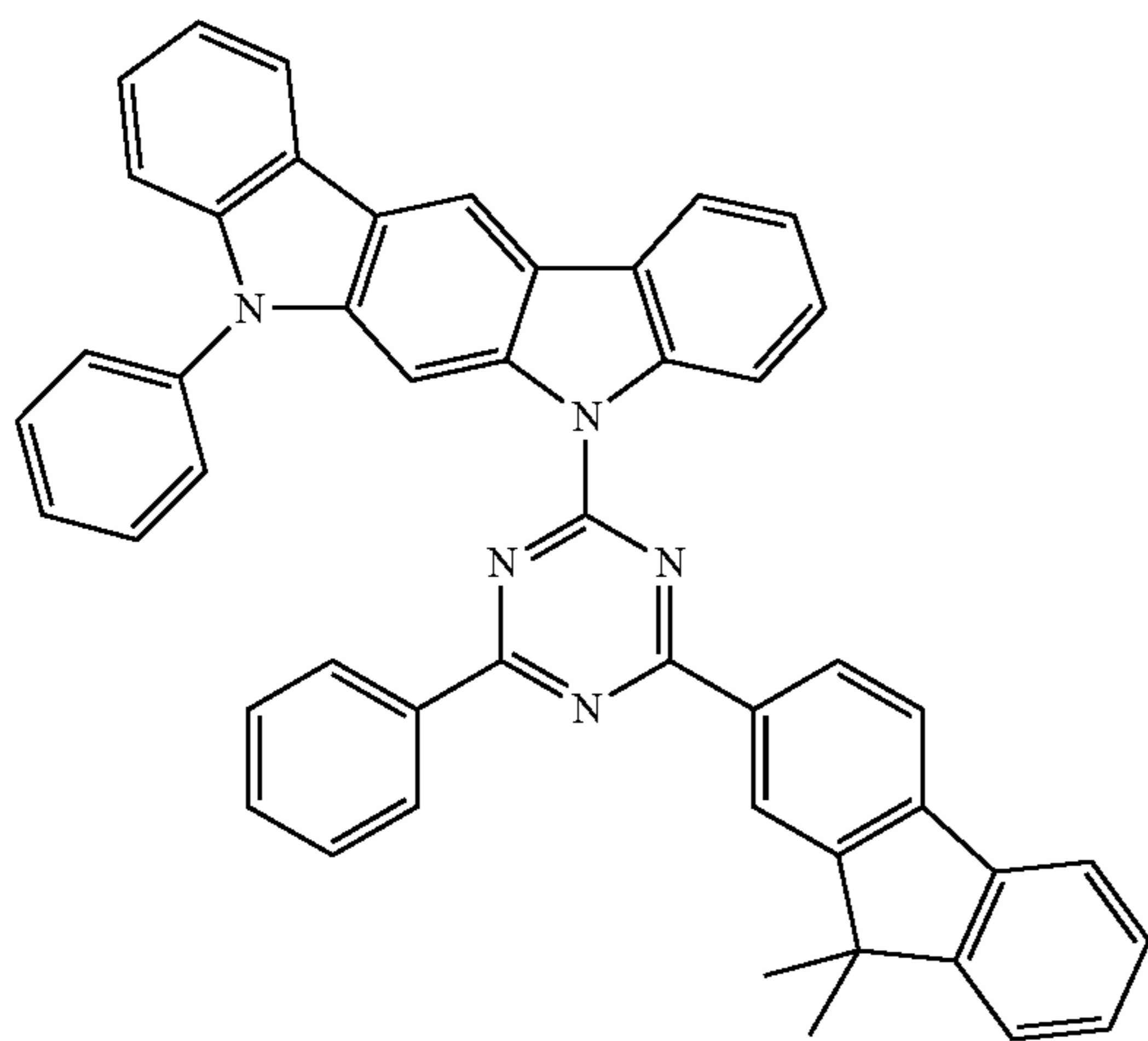
Compound EH20
