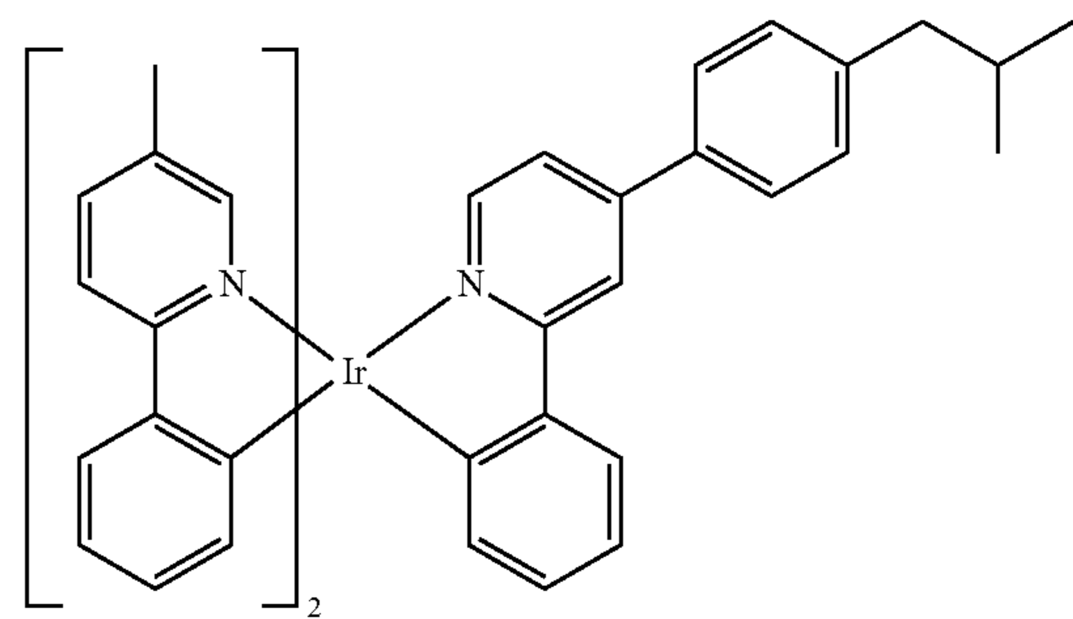
Compound 57
