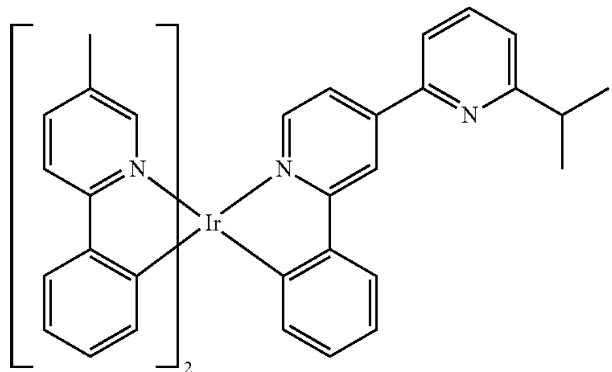
Compound 195
