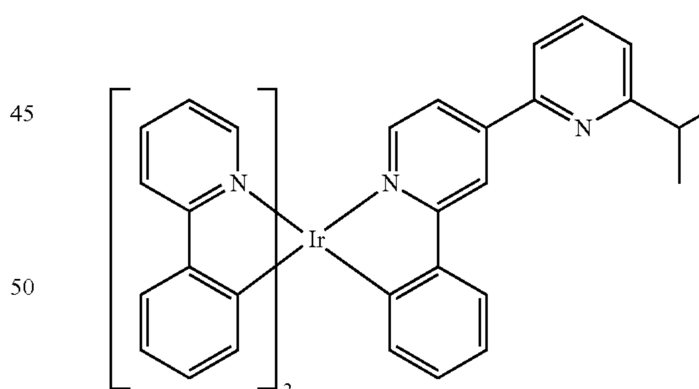
Compound 151
