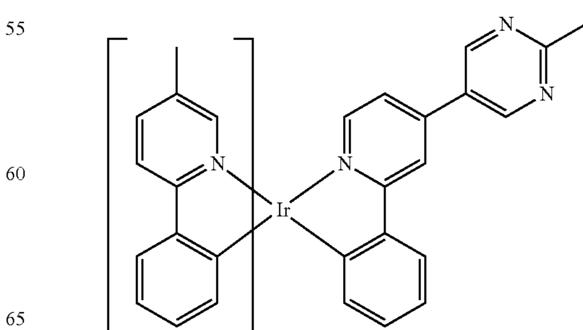
Compound 202
