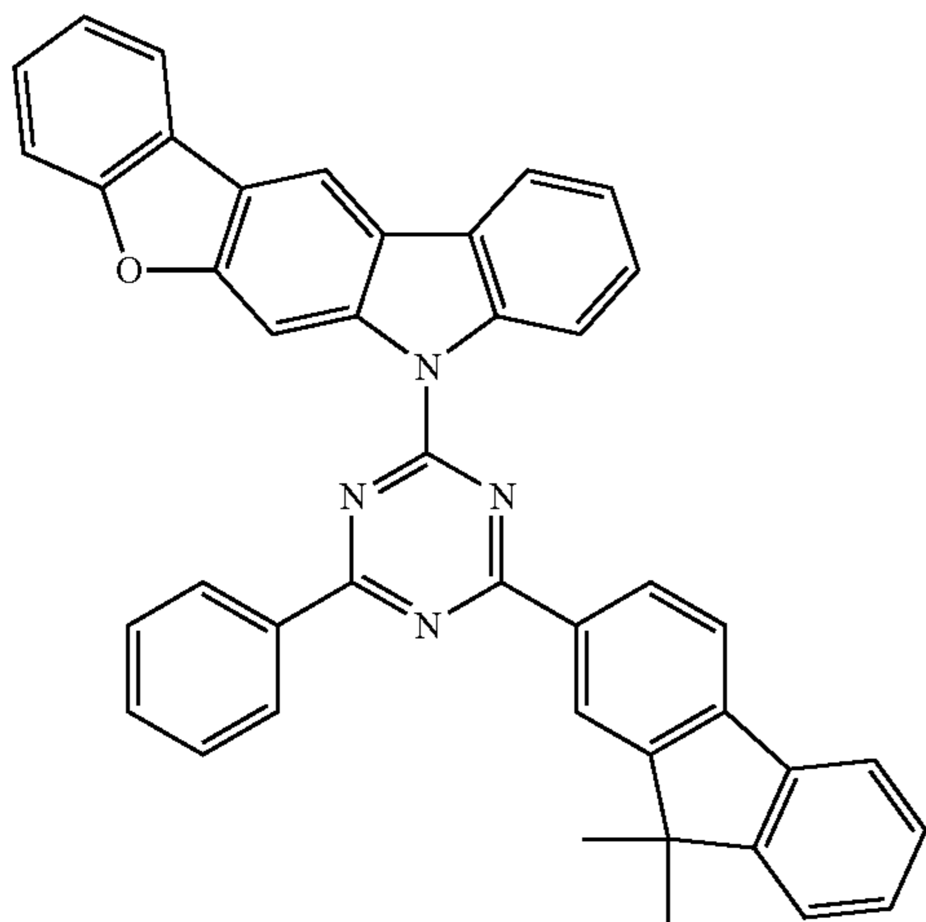
Compound EH26
