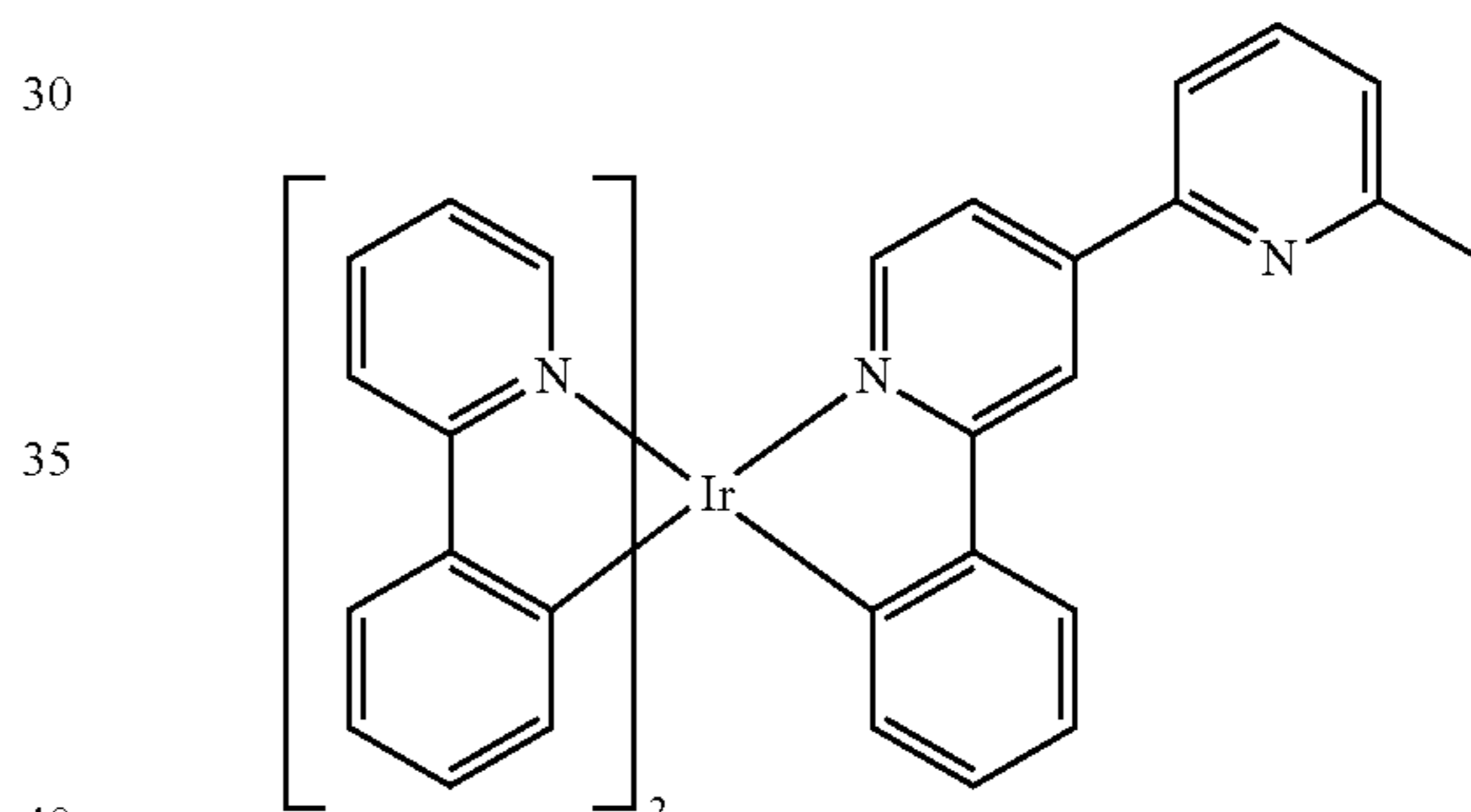
Compound 150
