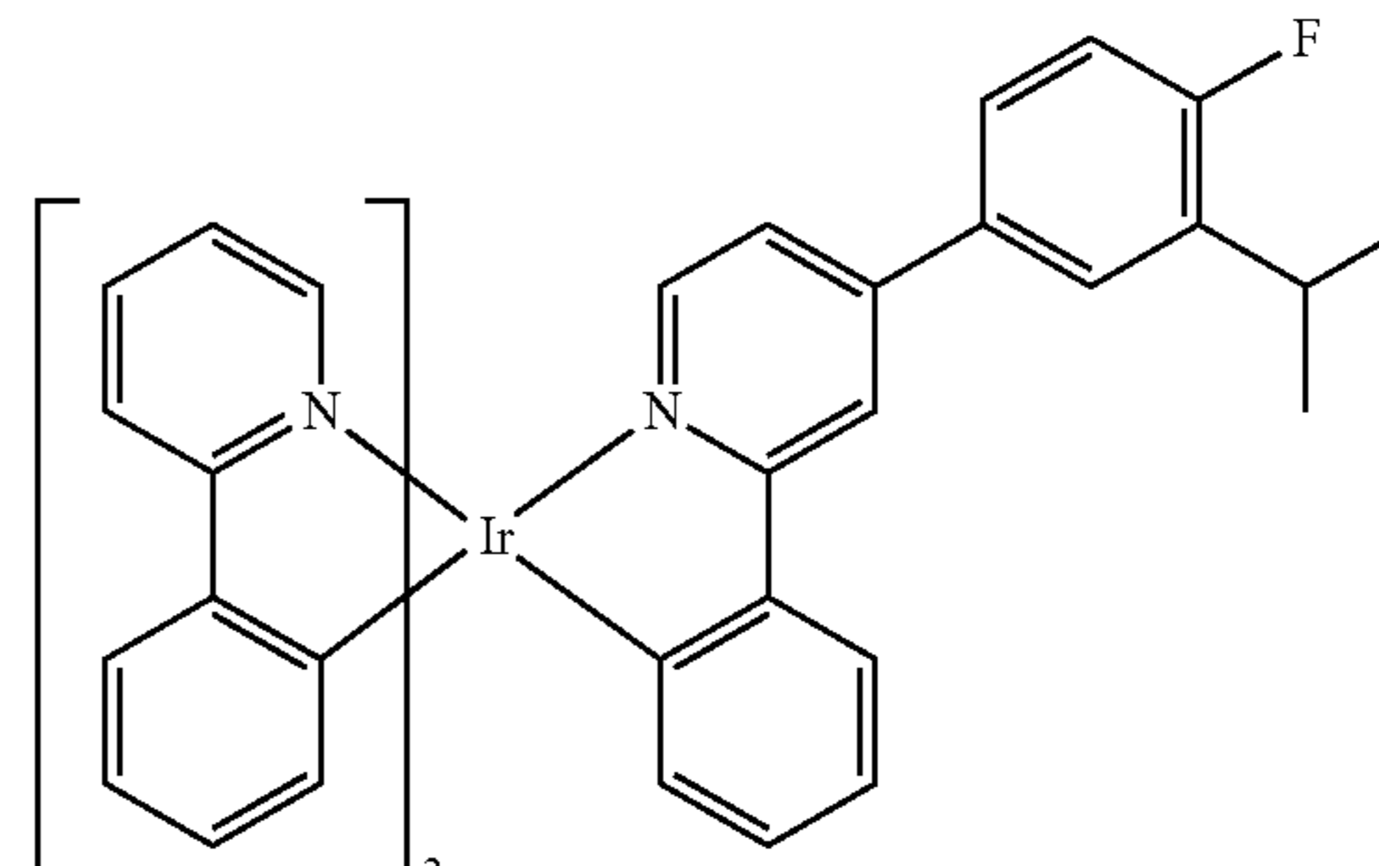
Compound 32
