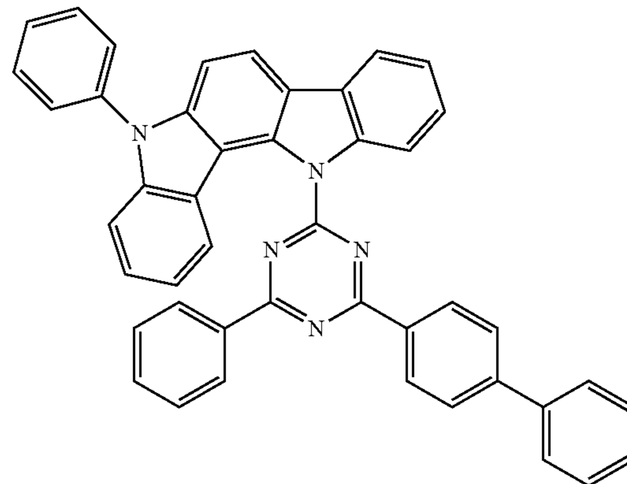
Compound EH42
