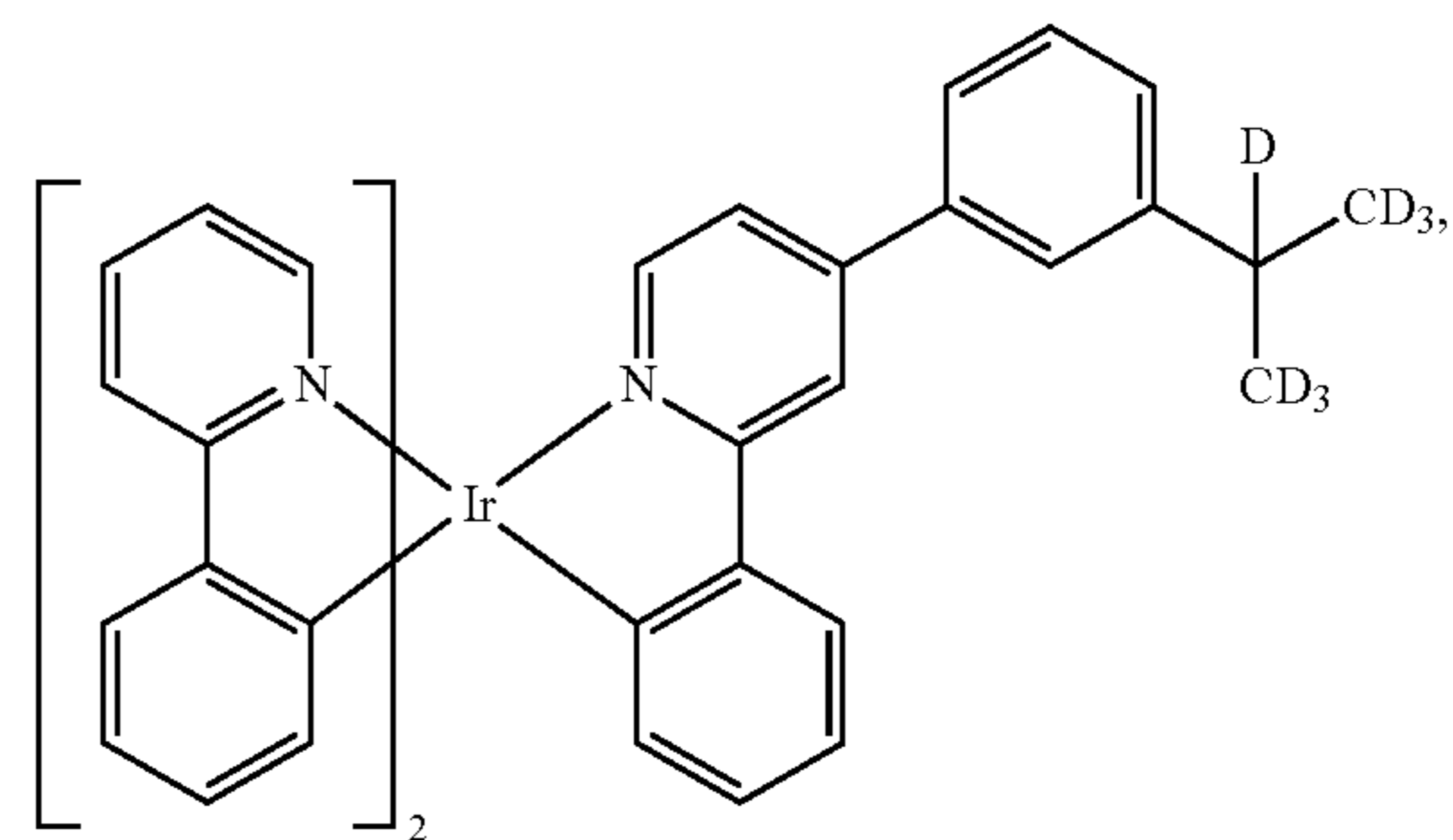
Compound 92
