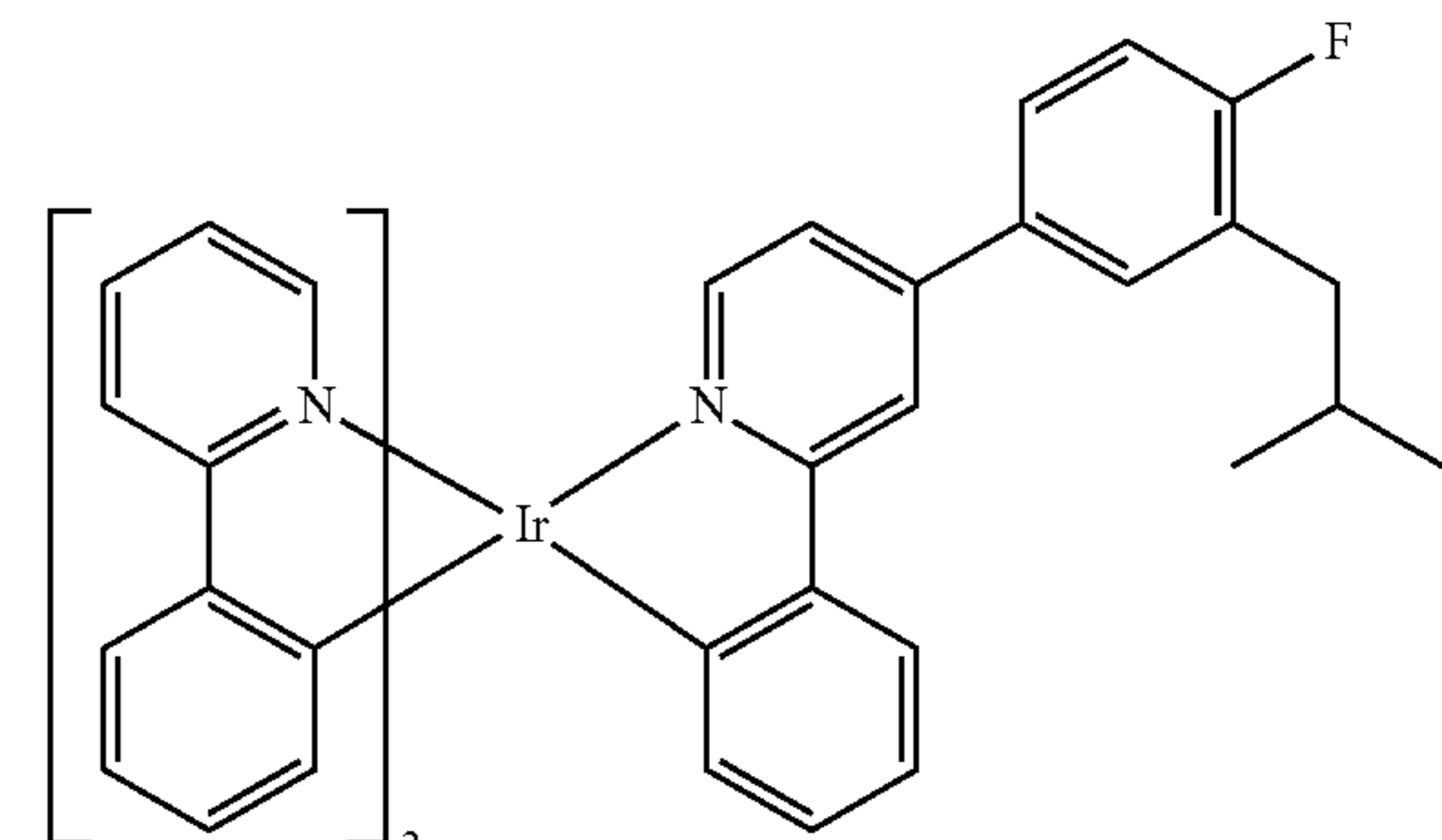
Compound 33
