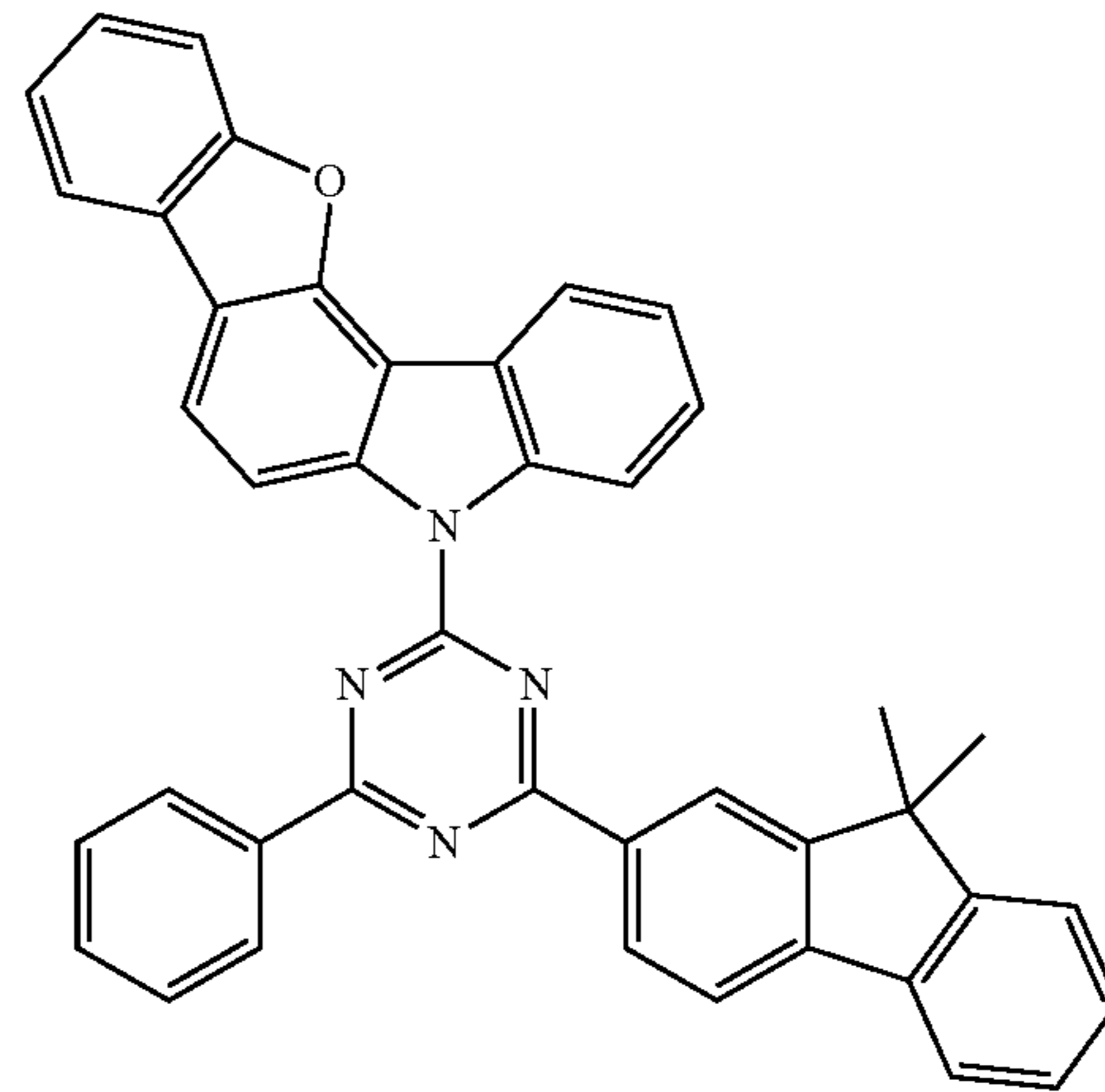
Compound EH40
