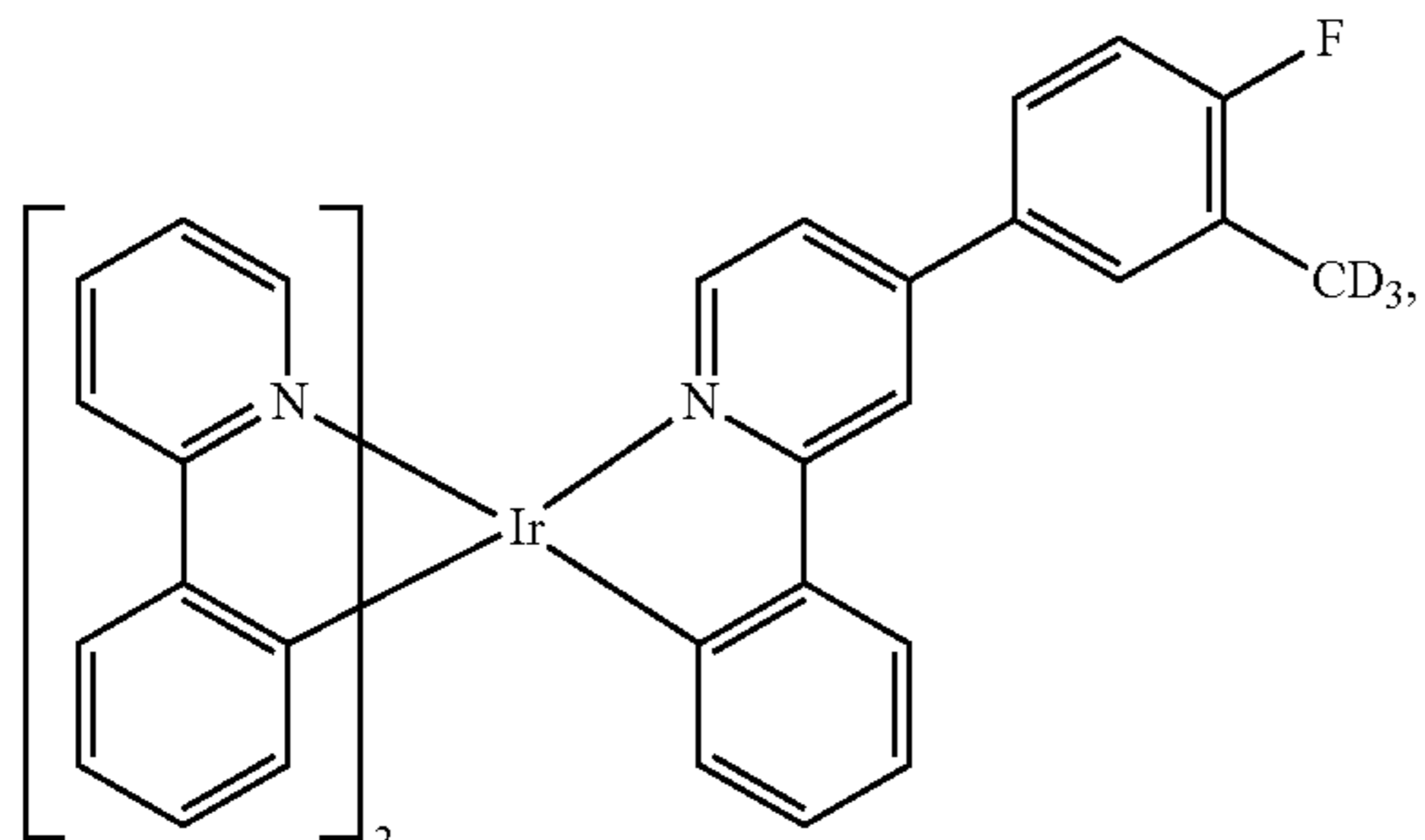
Compound 93
