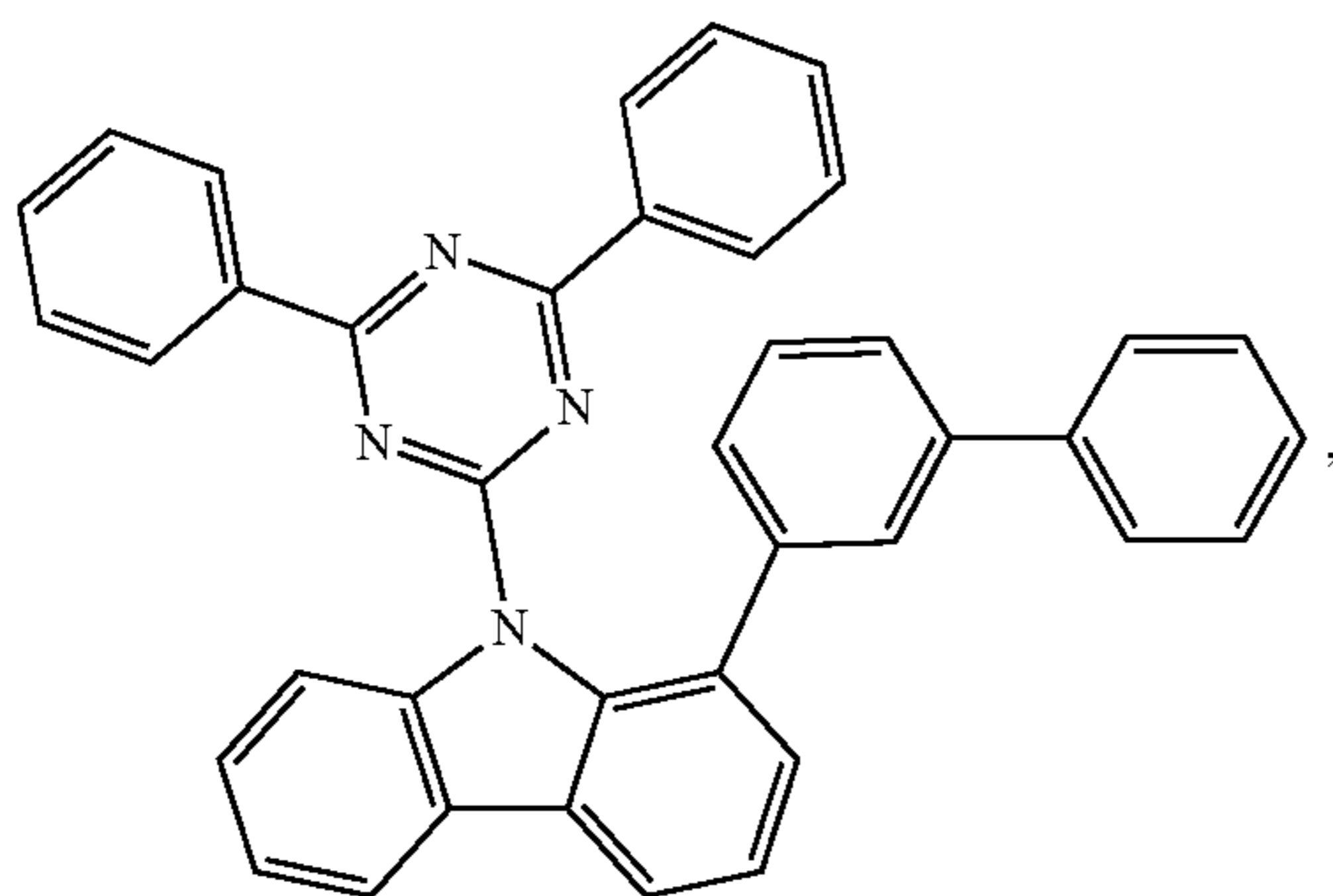
Compound H33
