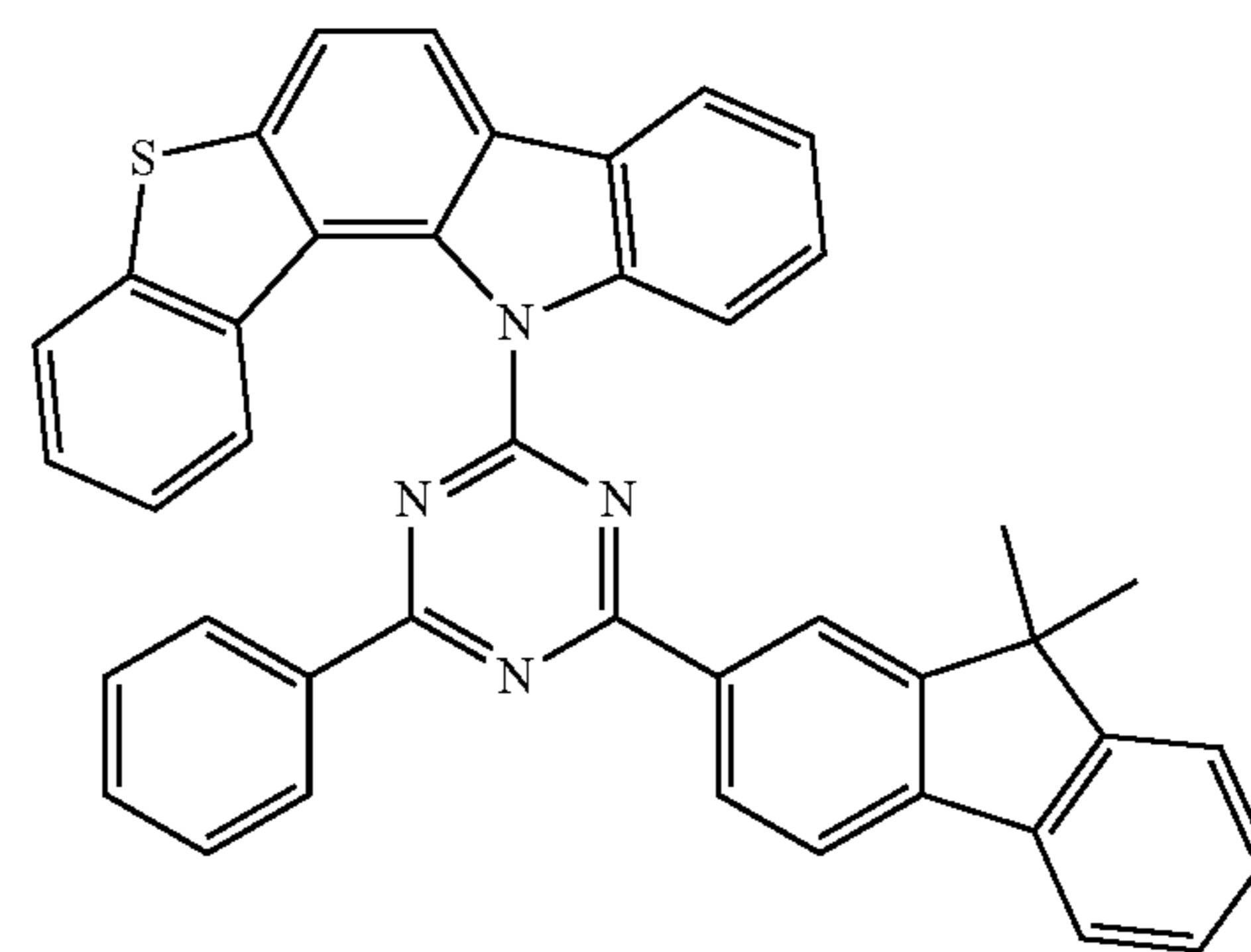
Compound EH45
