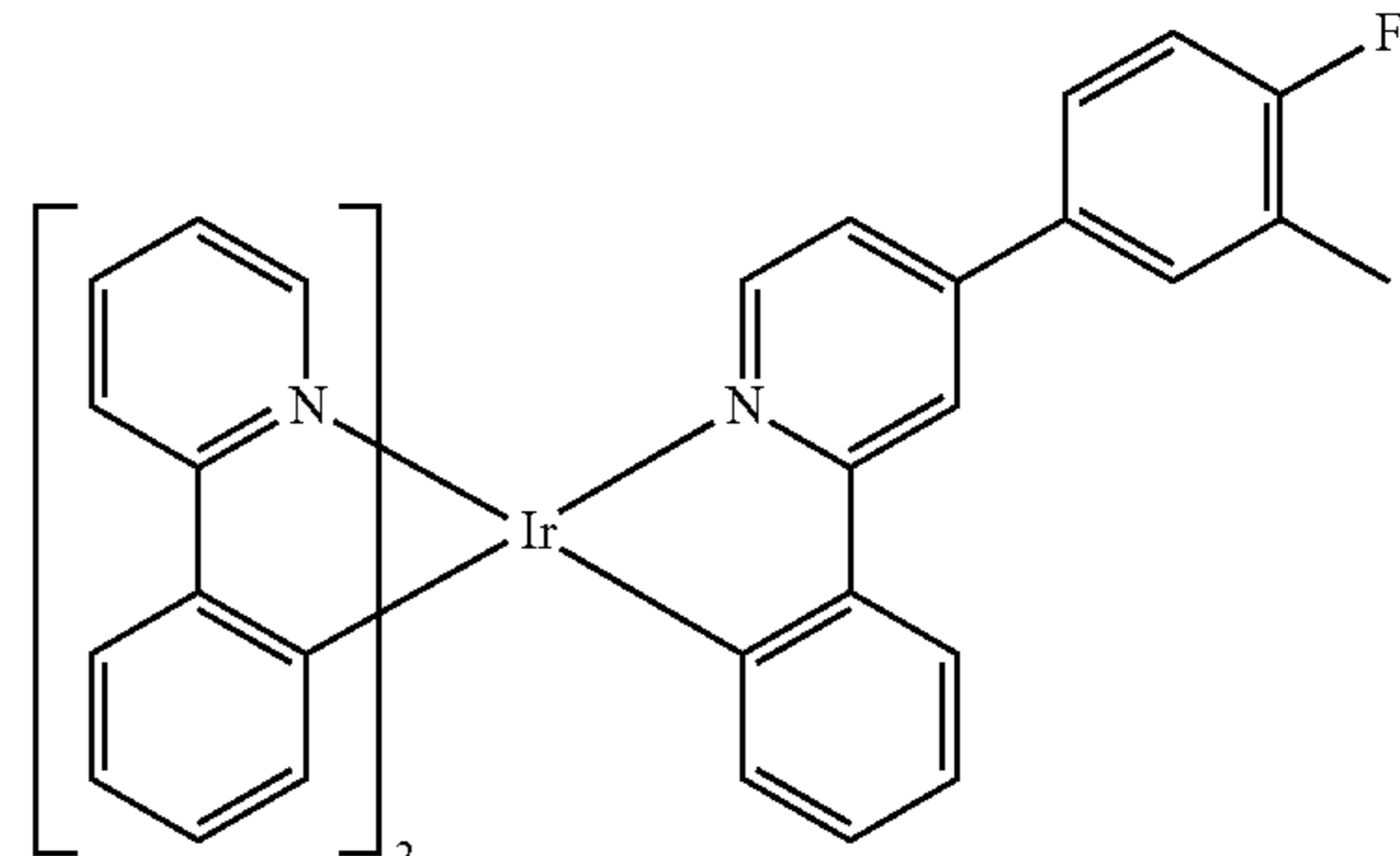
Compound 30
