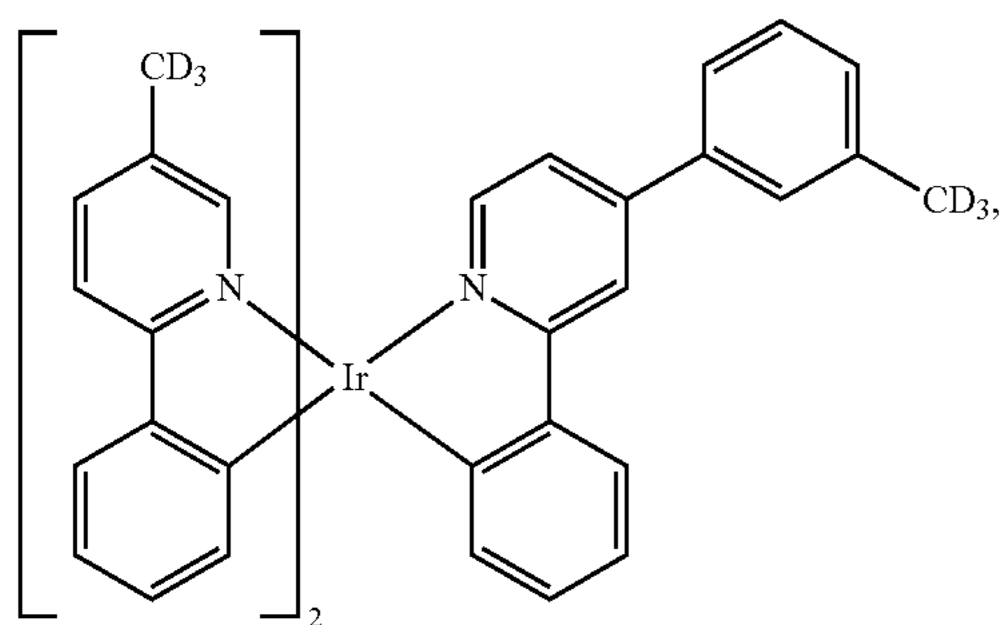
Compound 121
