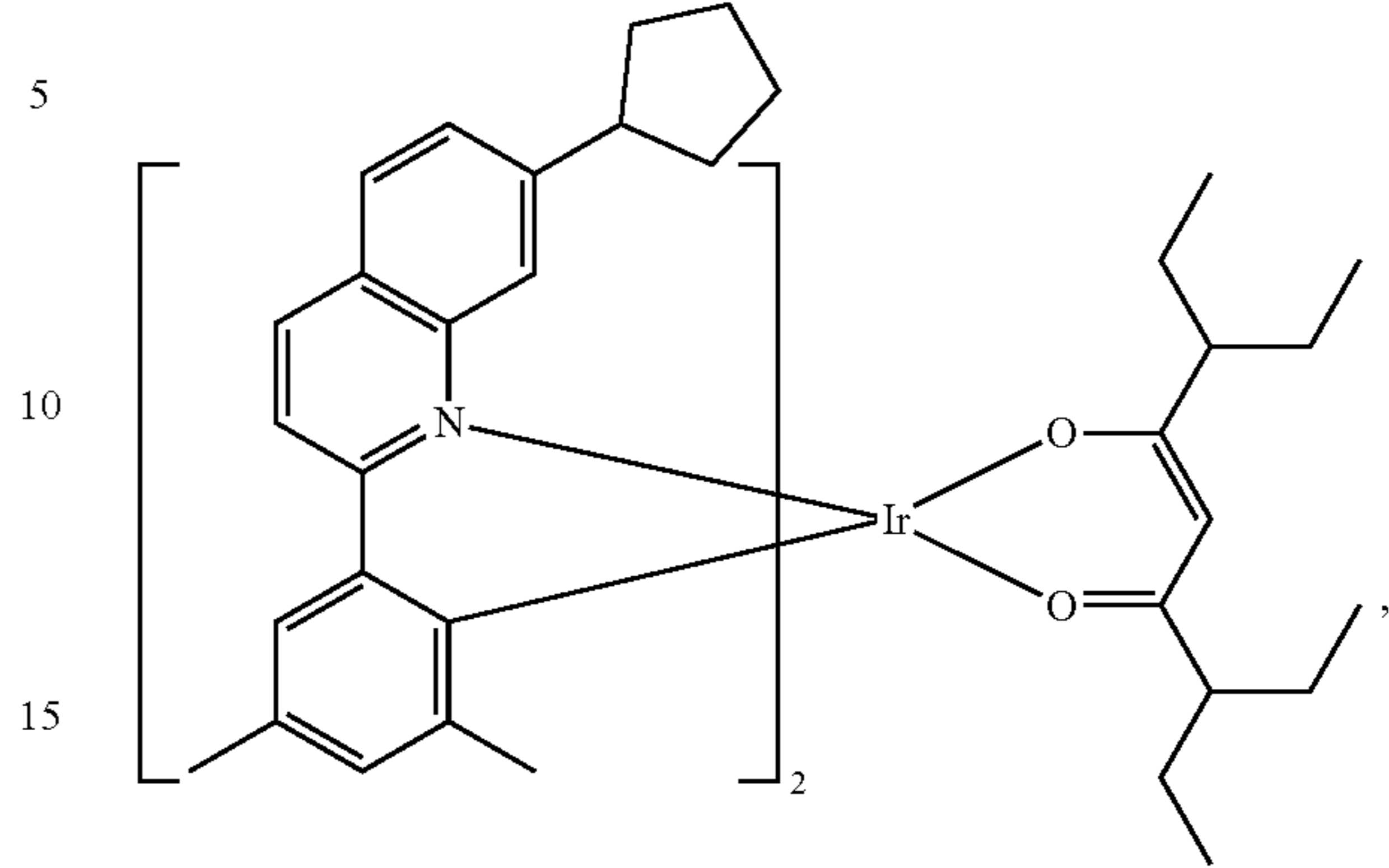
Compound E22
