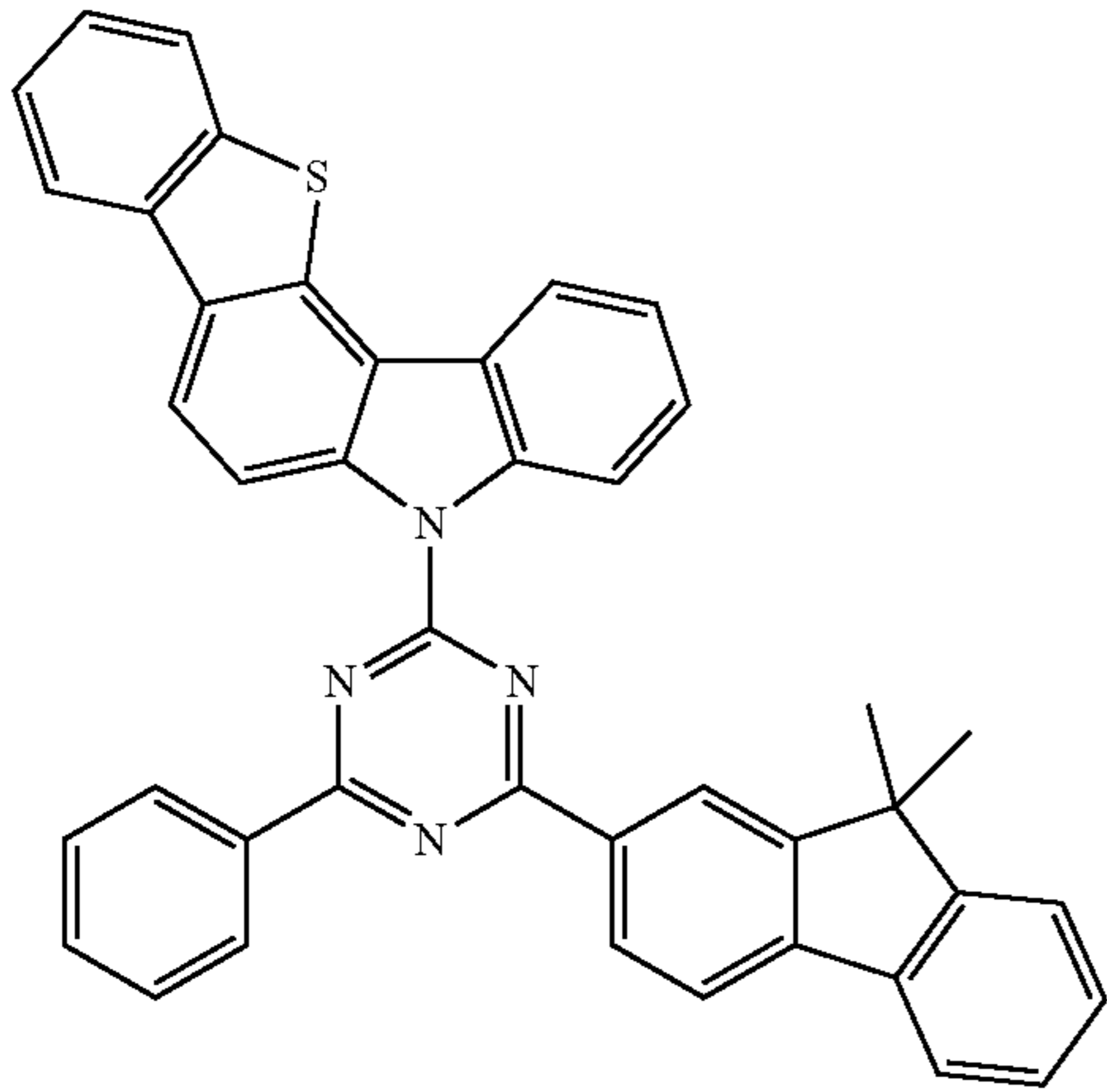
Compound EH36
