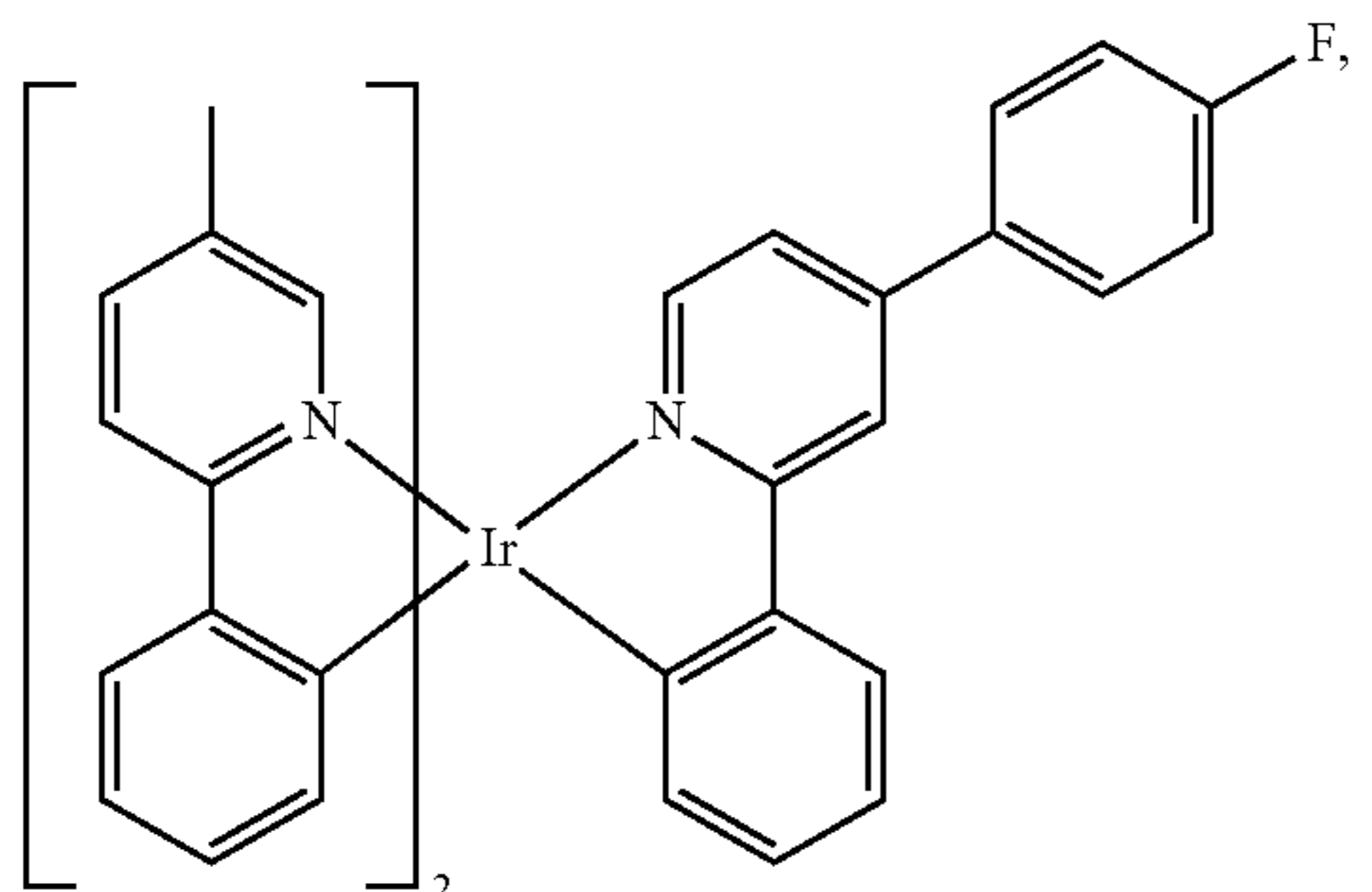
Compound 63
