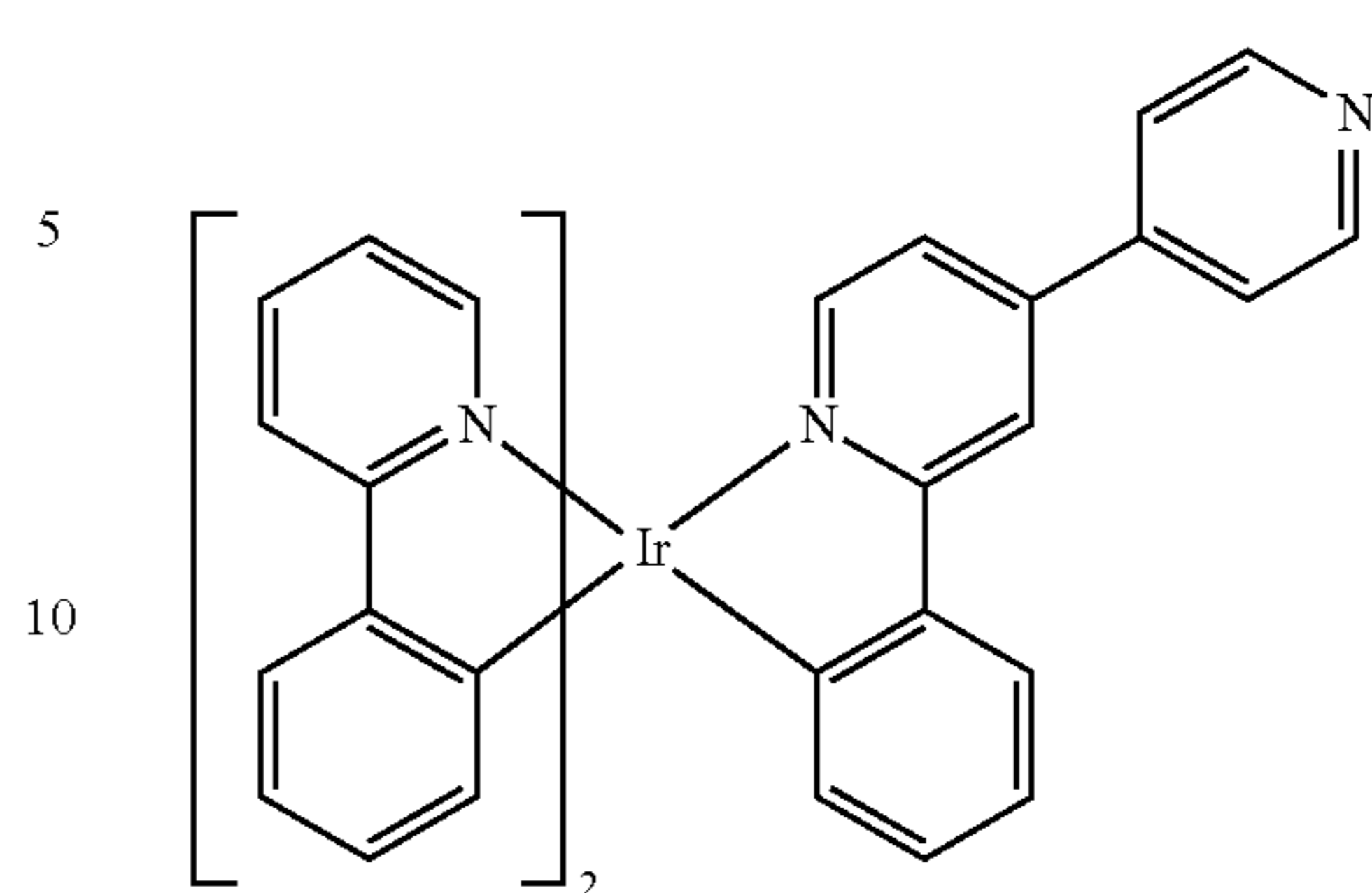
Compound 148
