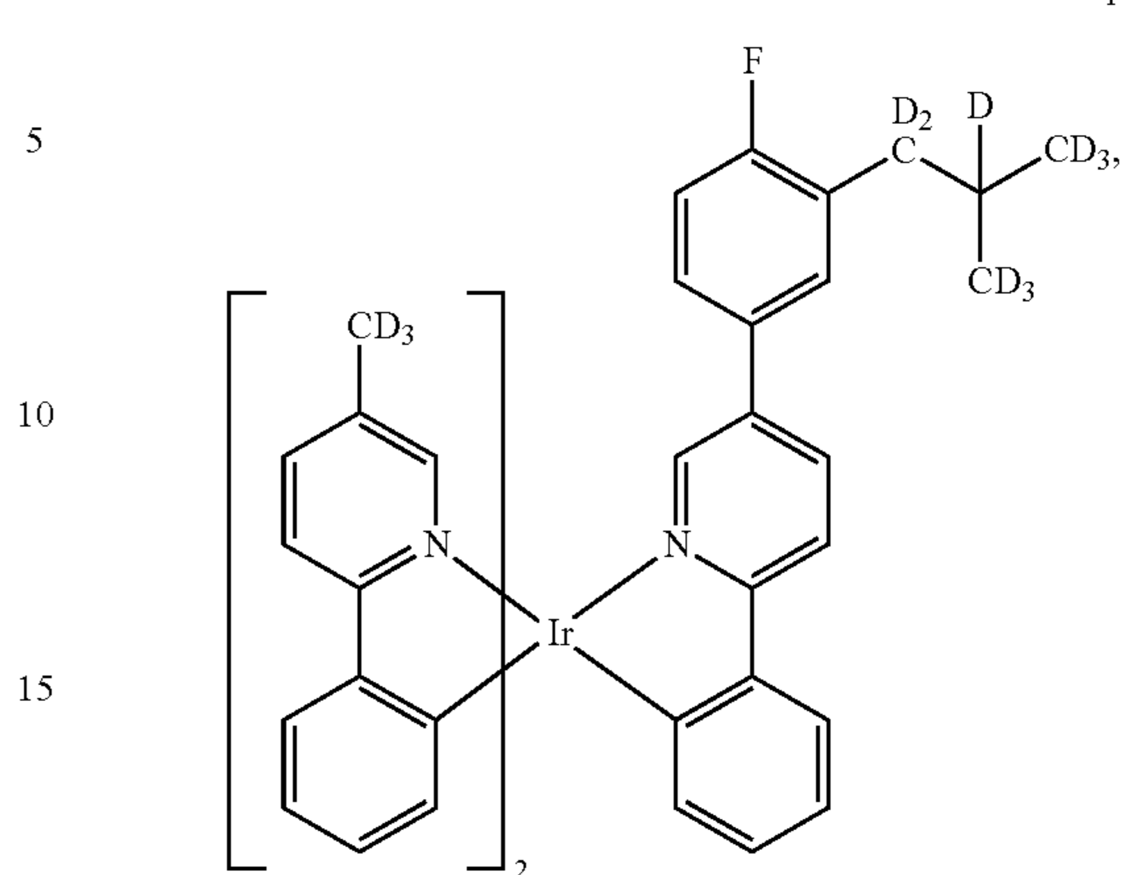
Compound 110
