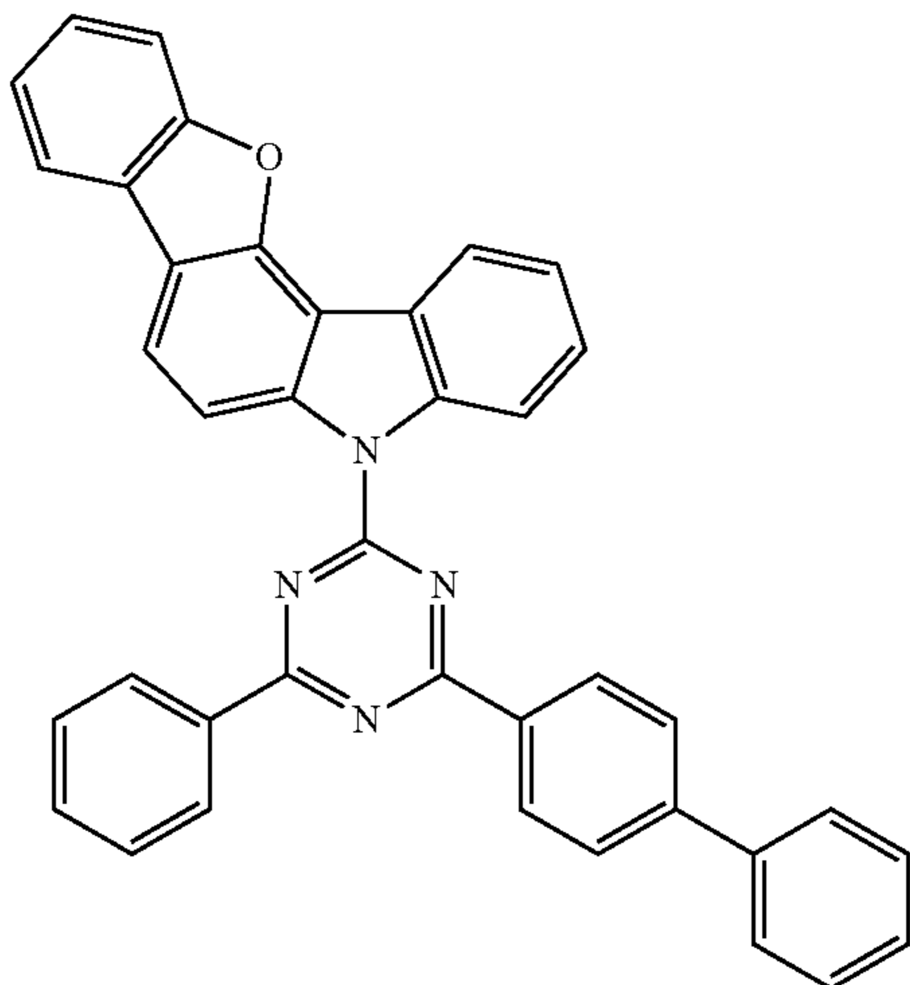
Compound EH38
