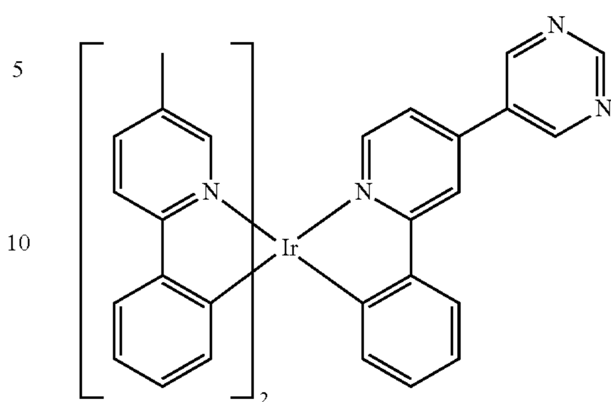
Compound 195
