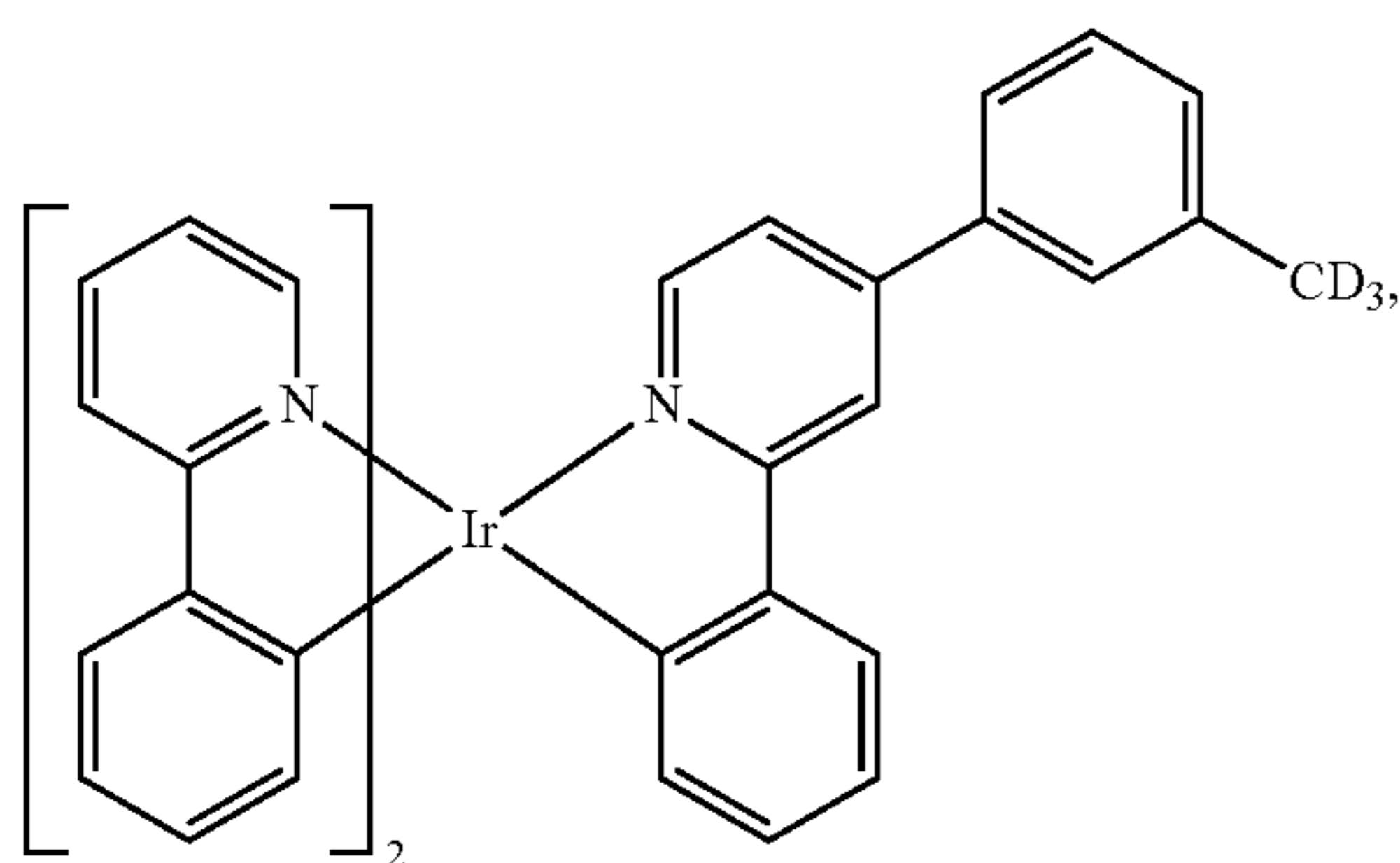
Compound 89
