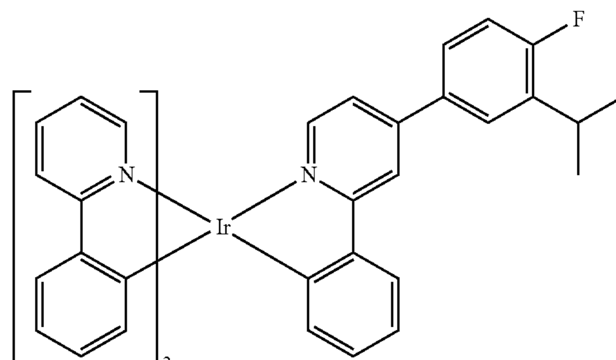
Compound 32
