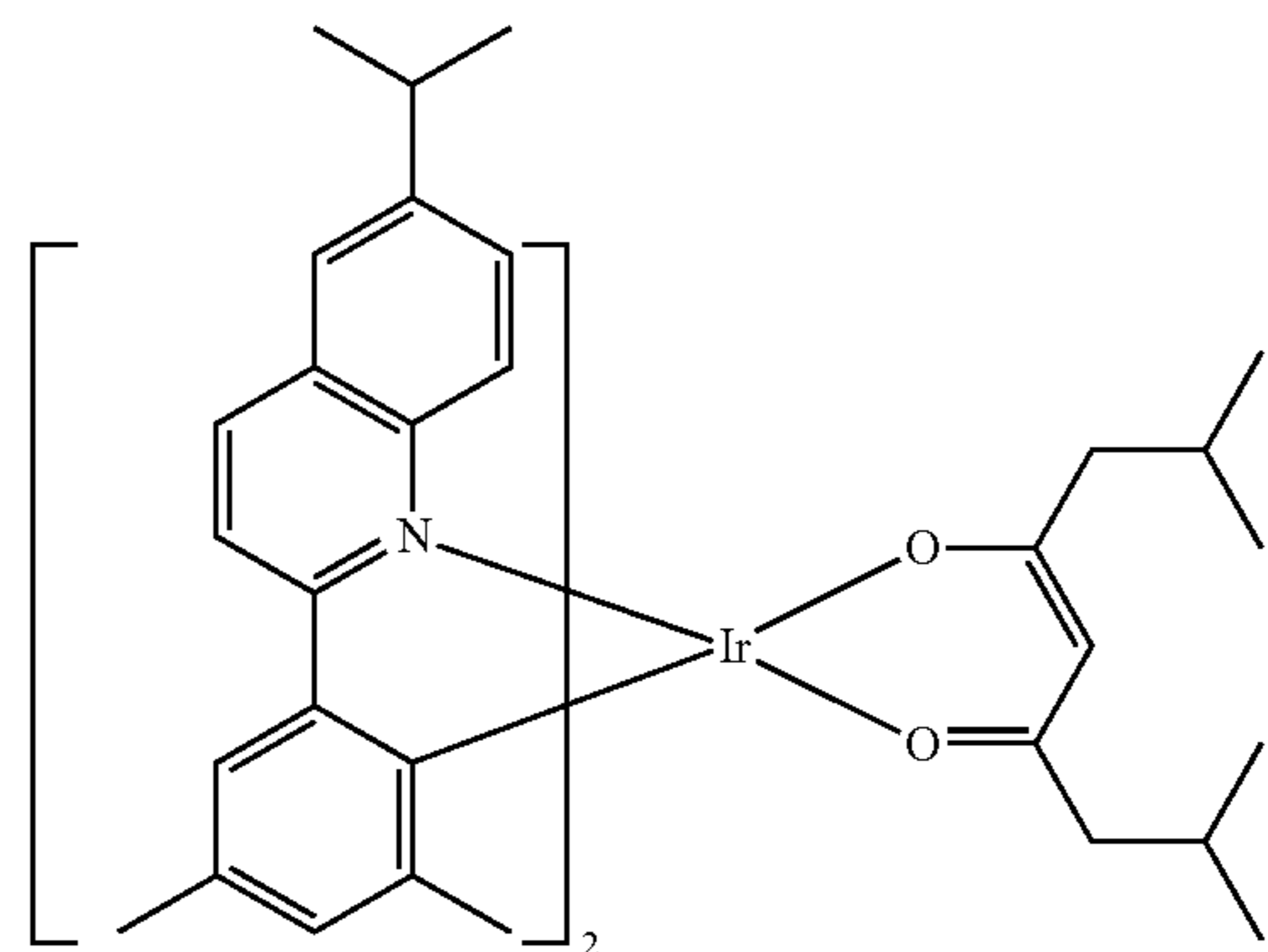
Compound E40
