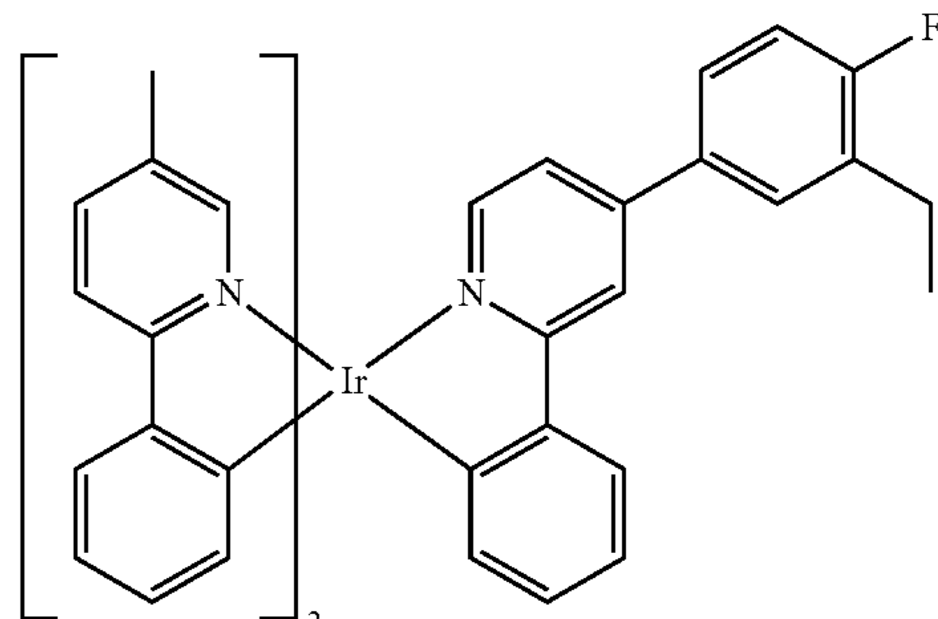
Compound 64
