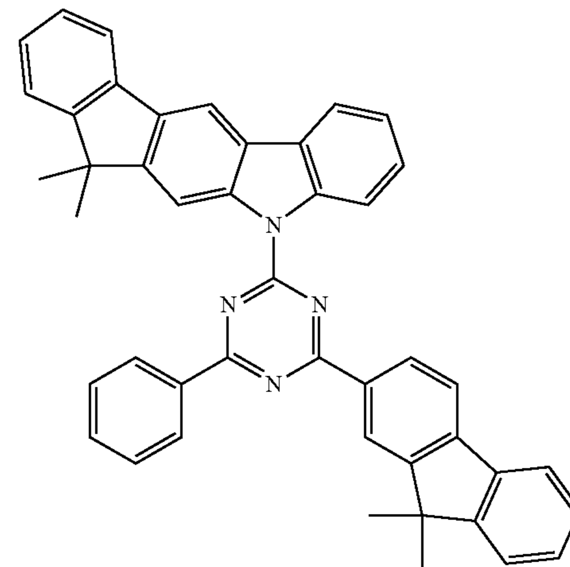
Compound EH29
