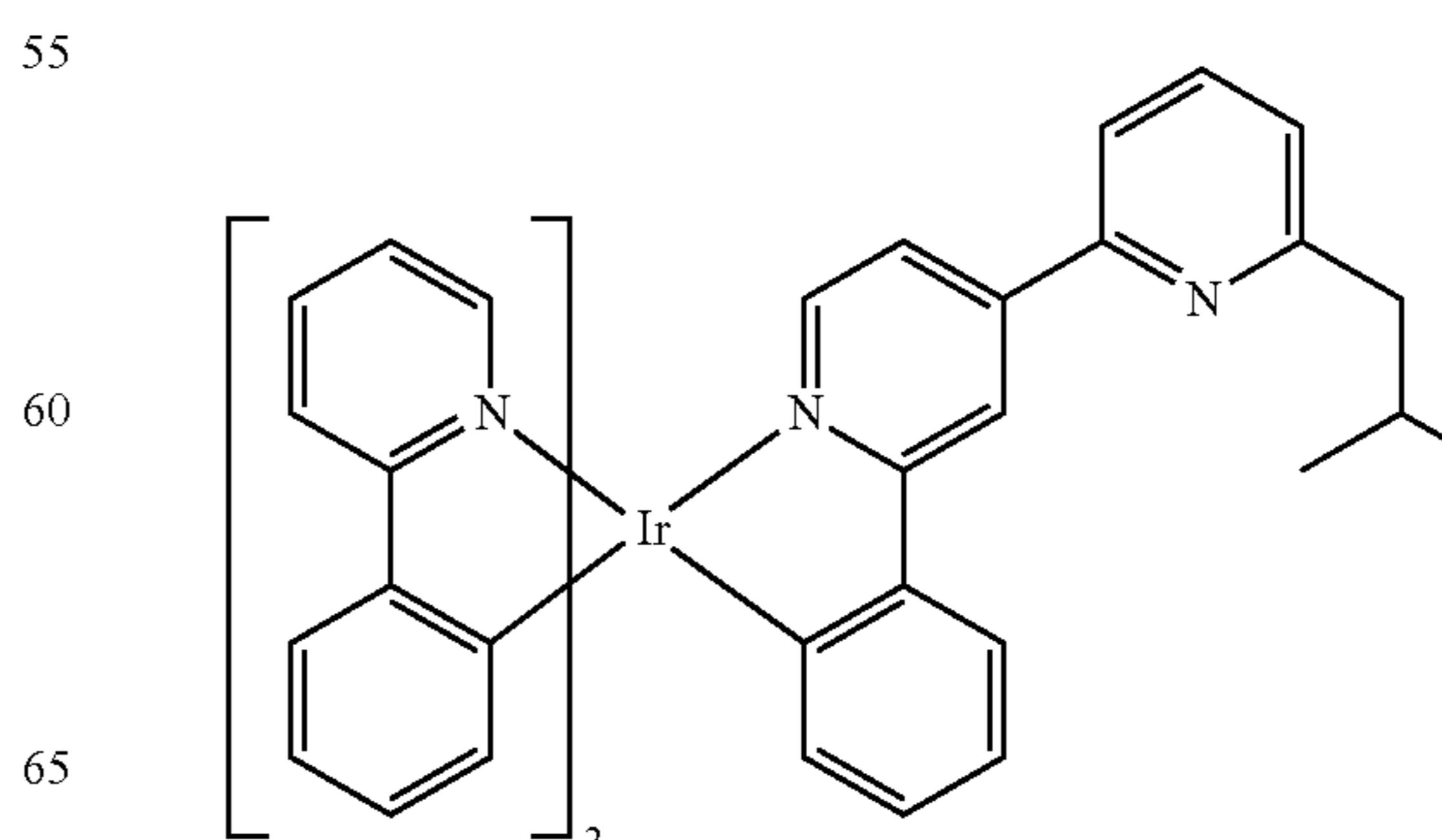
Compound 151
