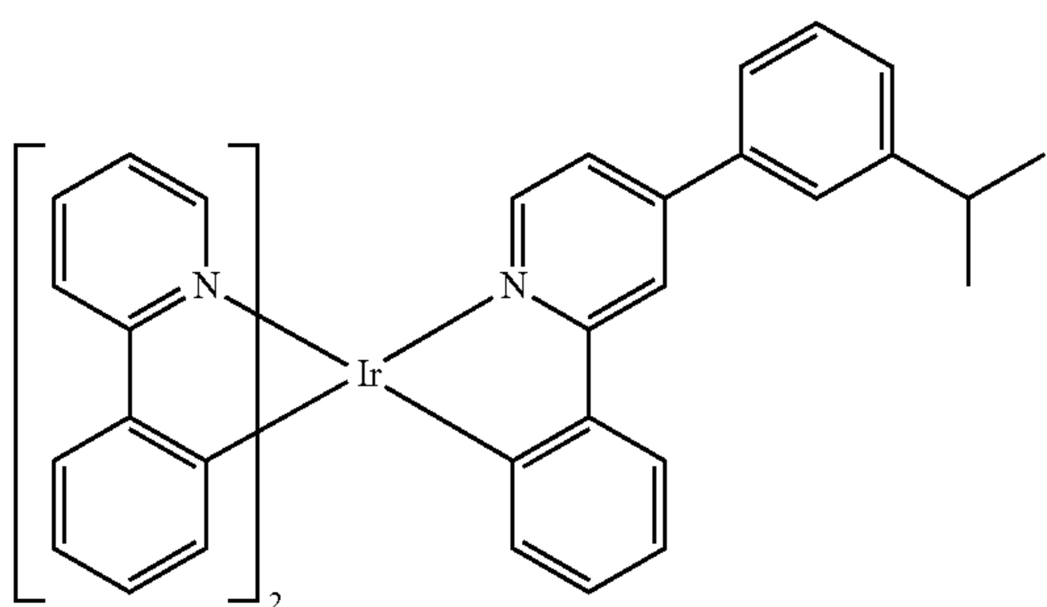
Compound 28
