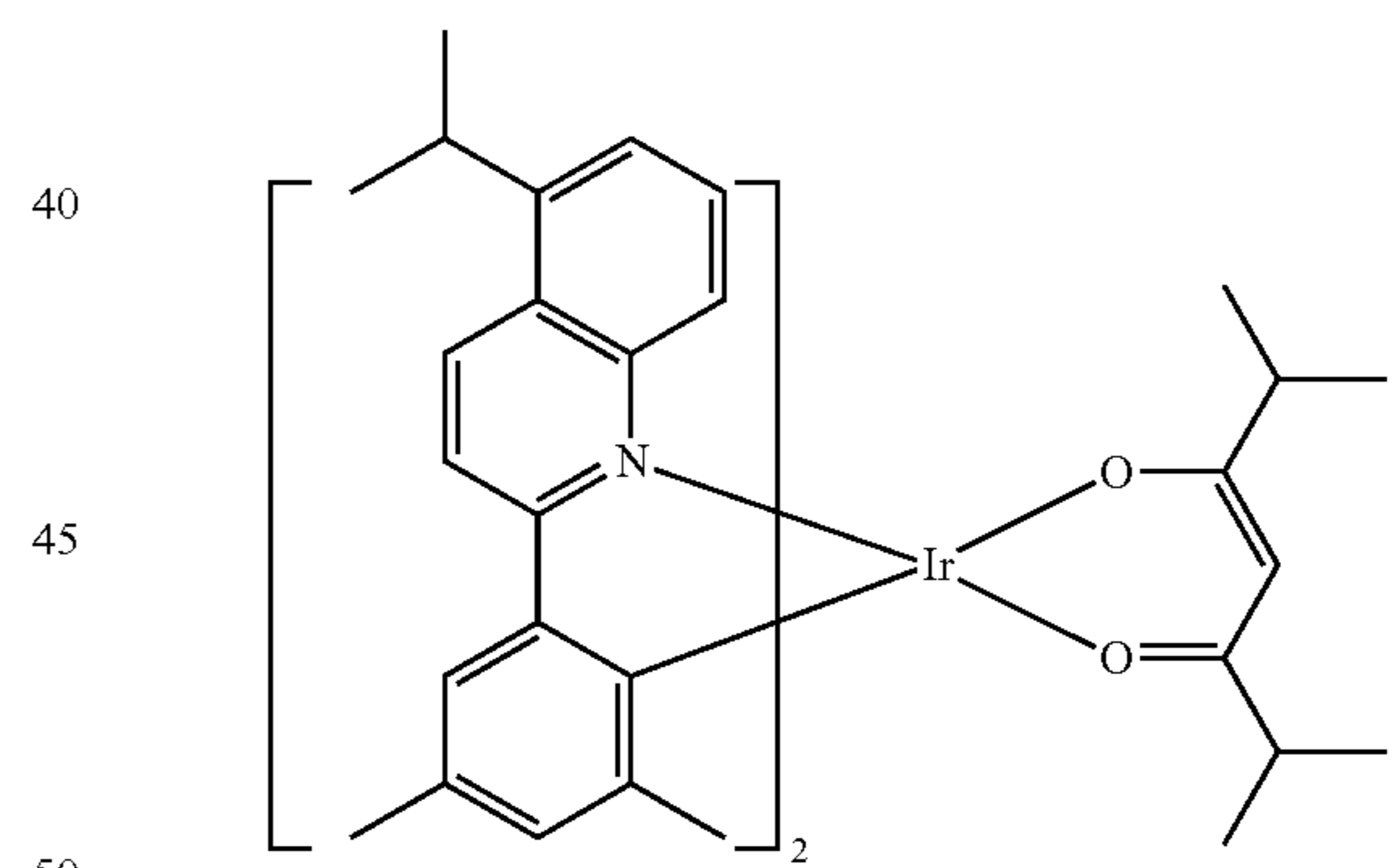
Compound E31
