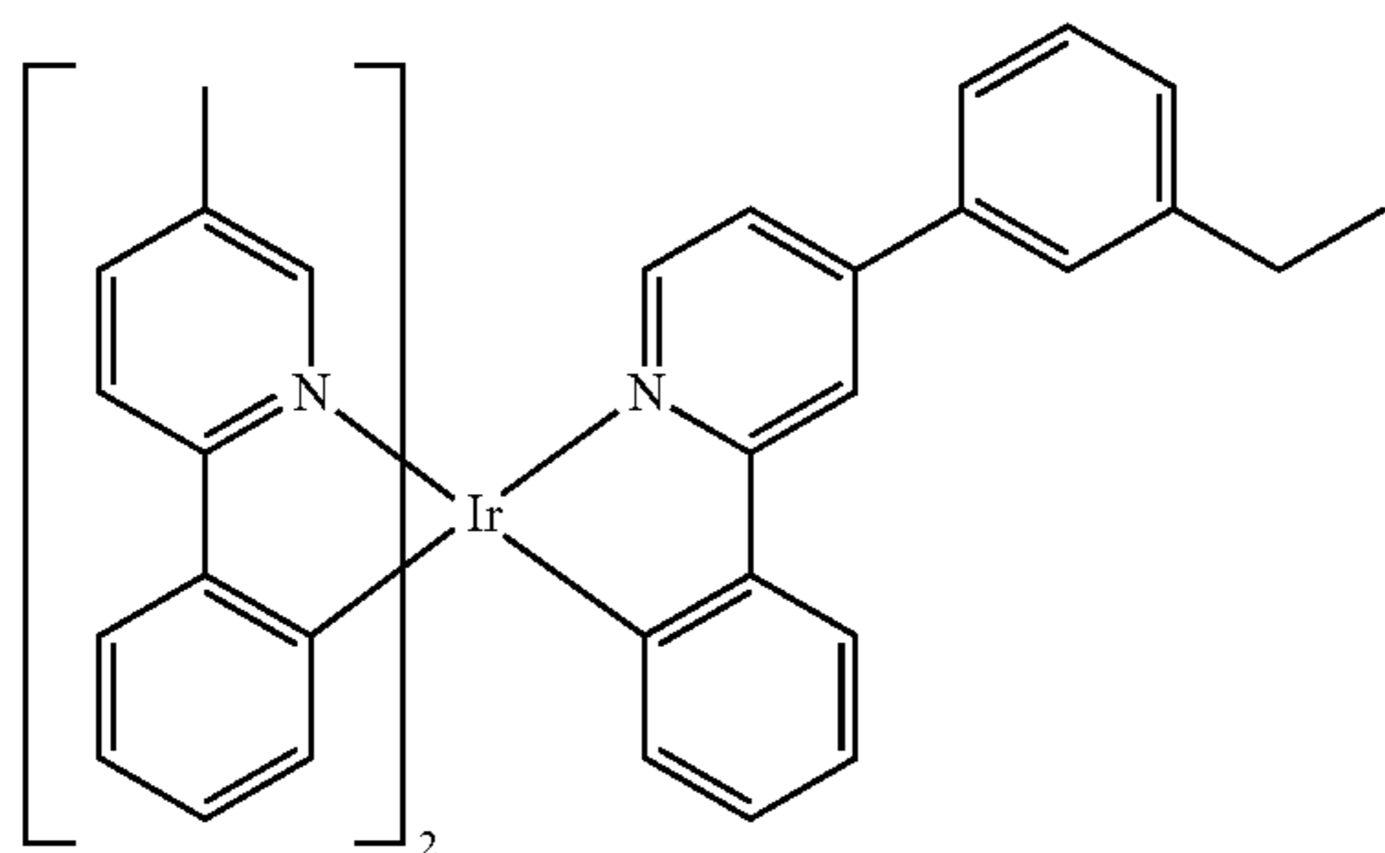
Compound 60
