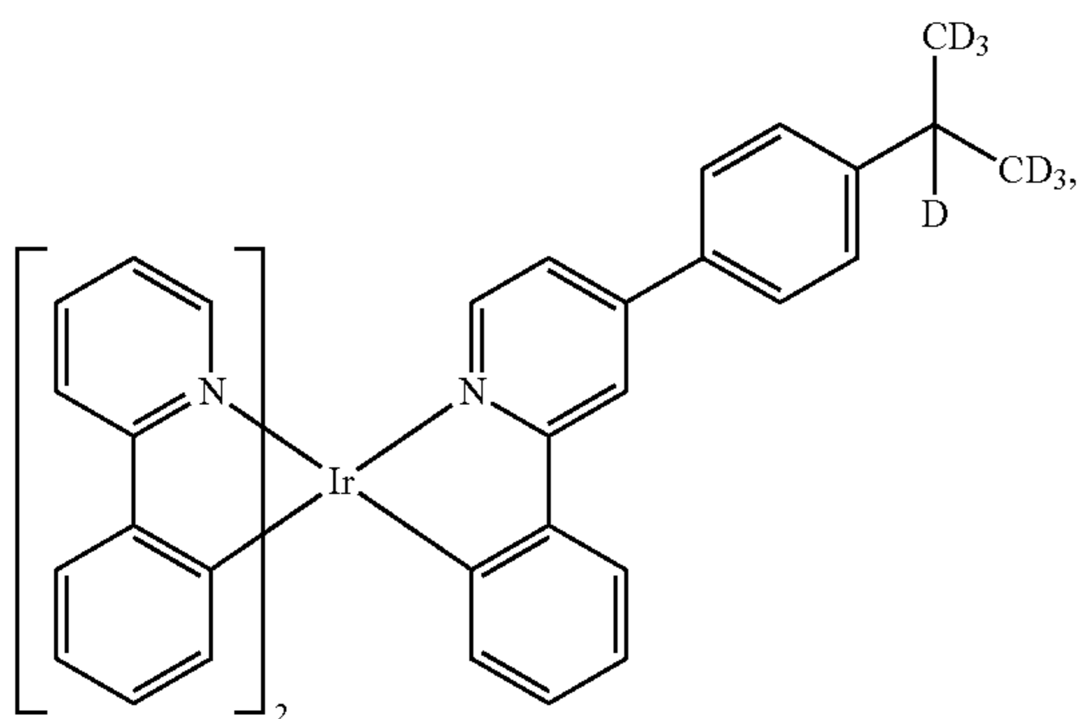
Compound 87
