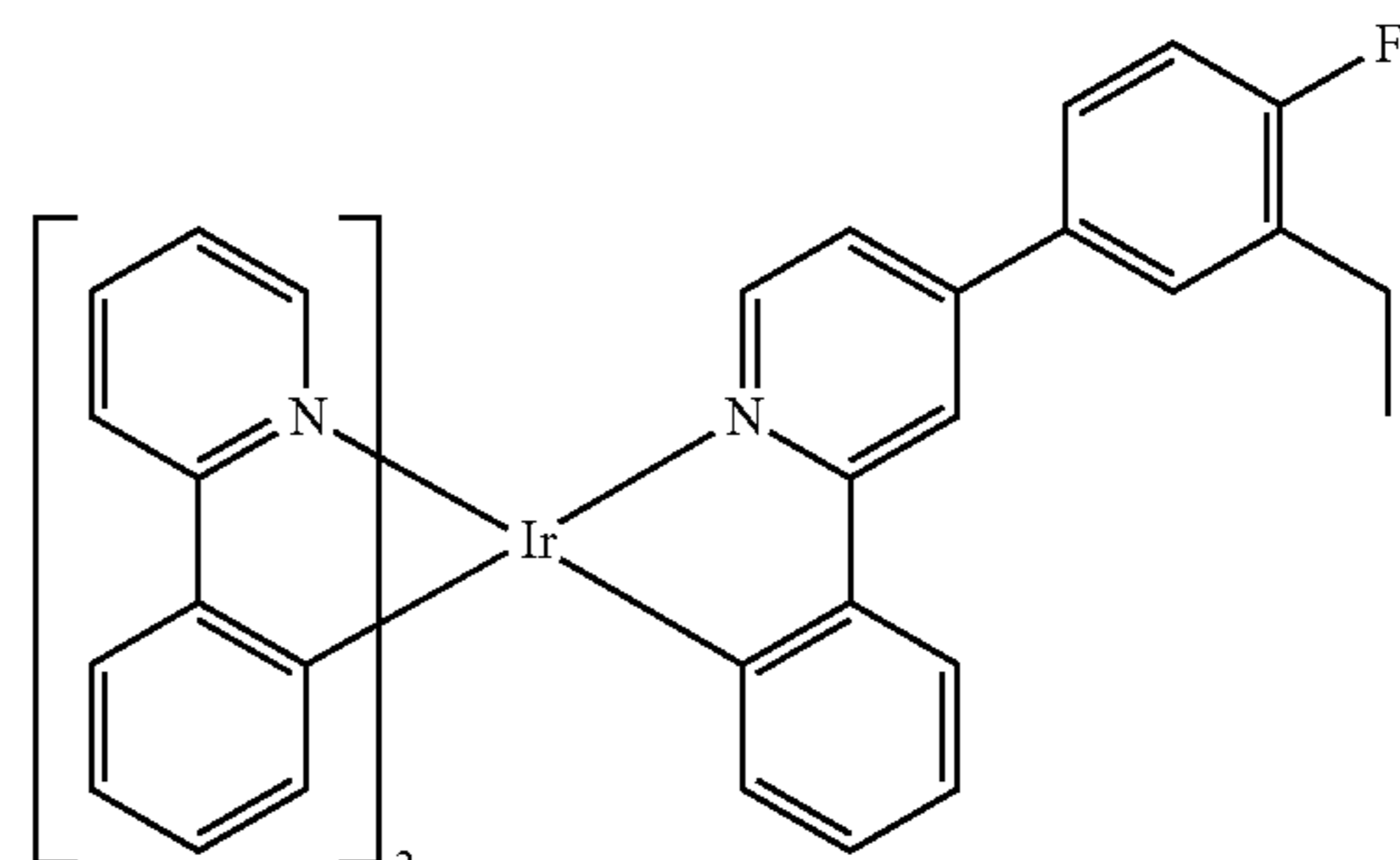
Compound 31
