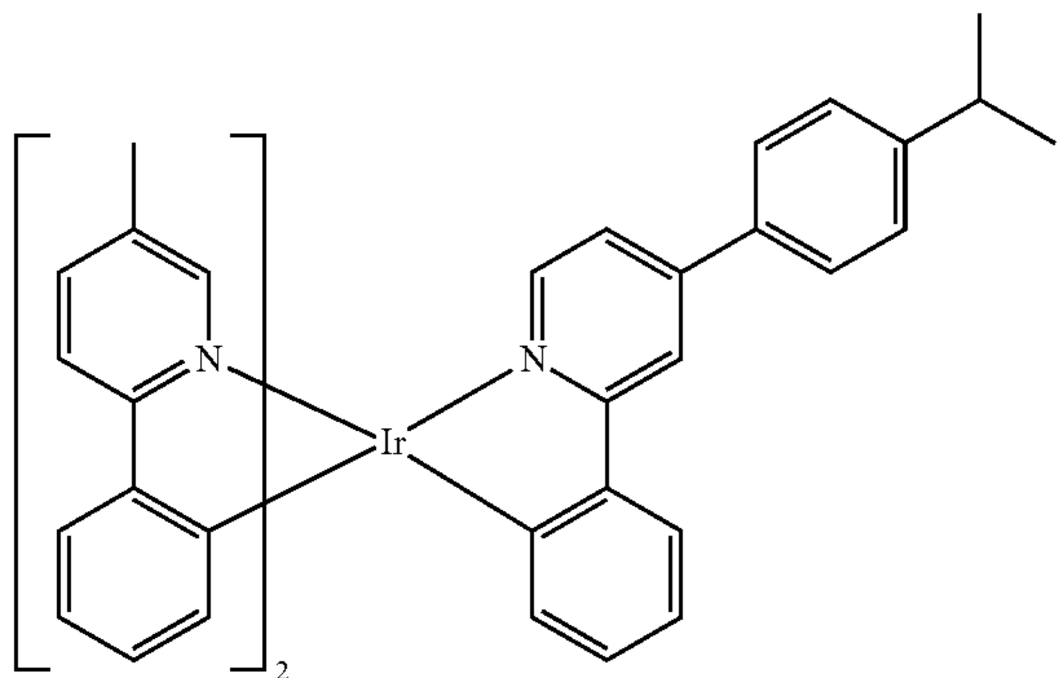
Compound 57
