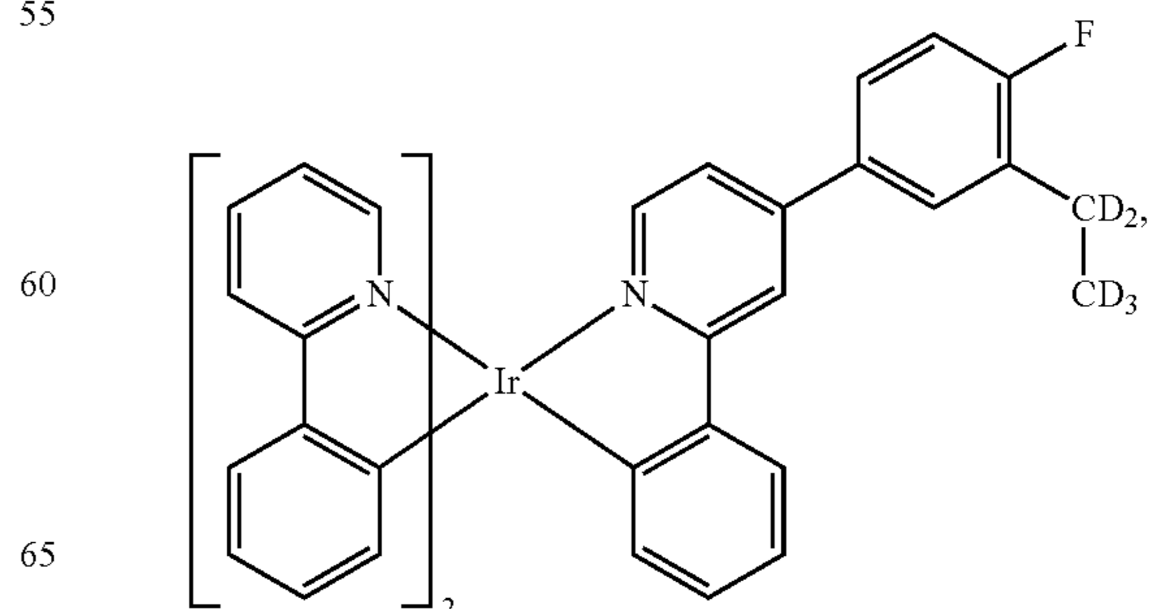
Compound 94
