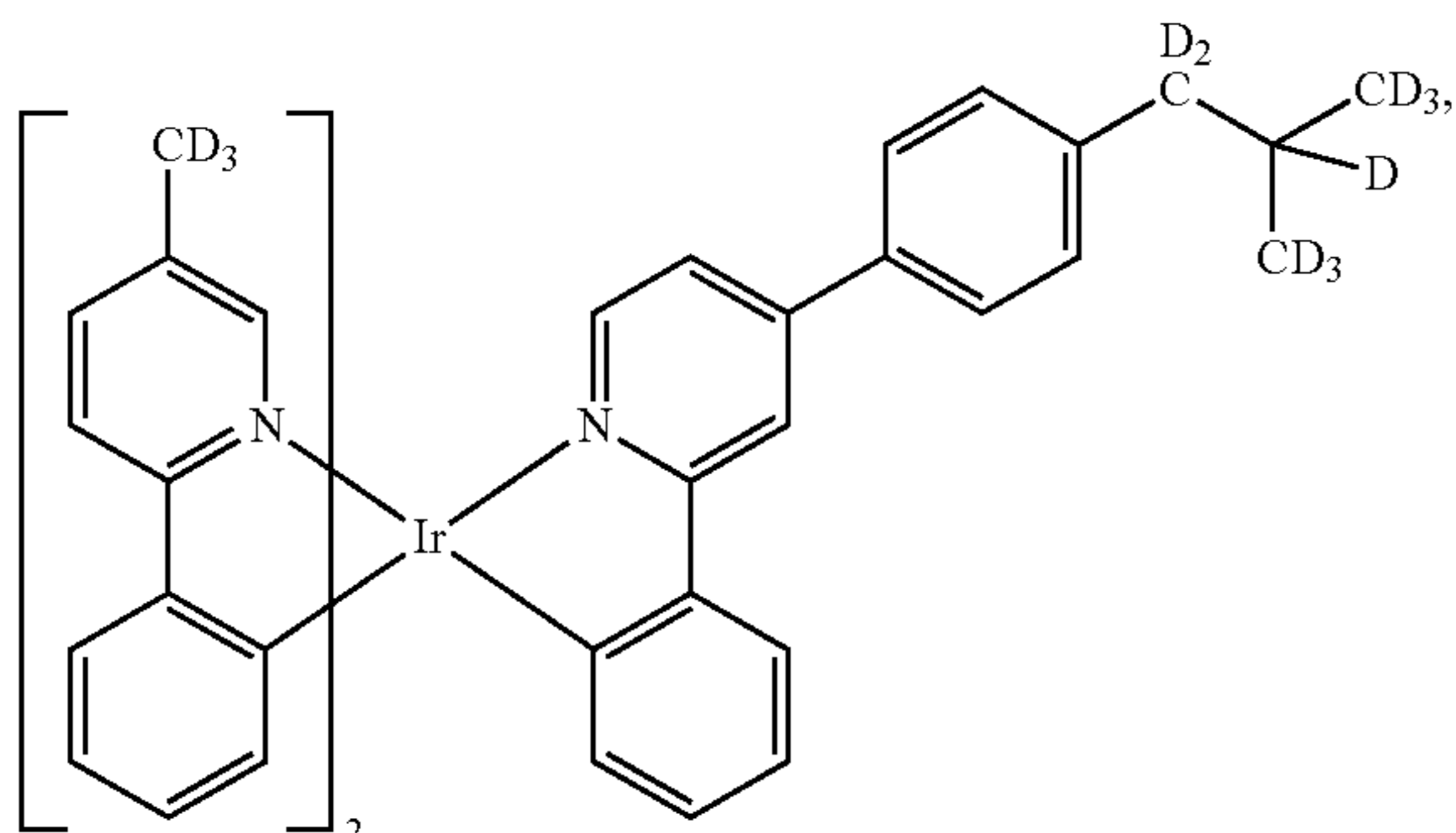
Compound 120
