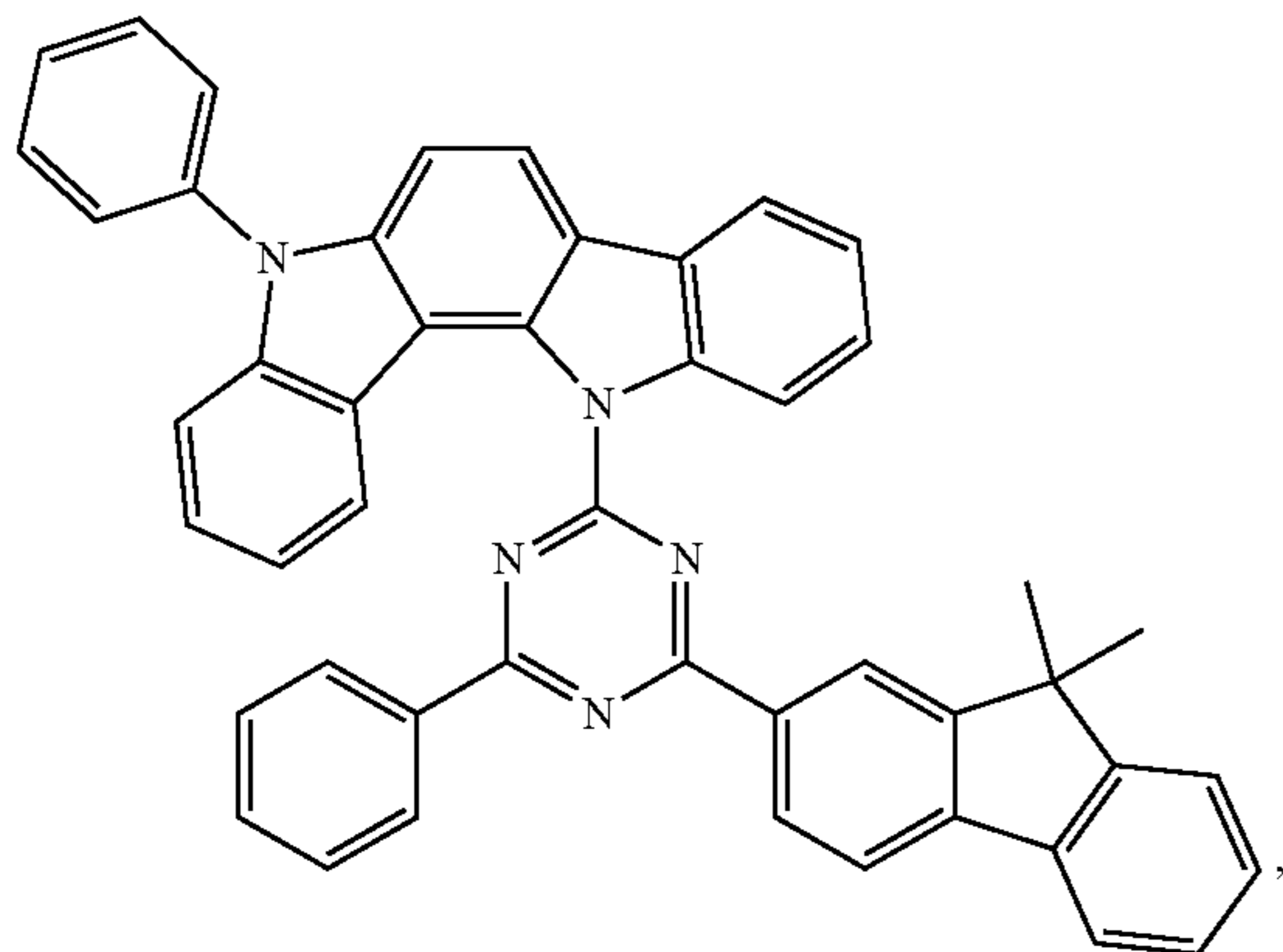
Compound EH43
