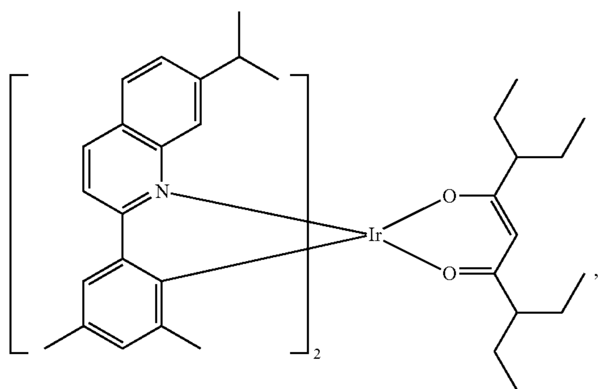
Compound E34
