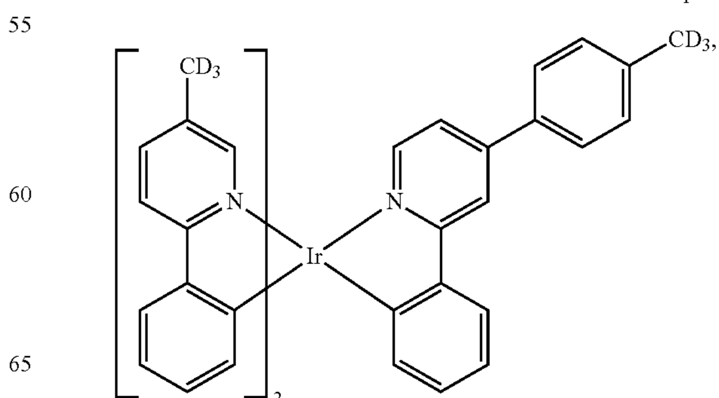
Compound 117
