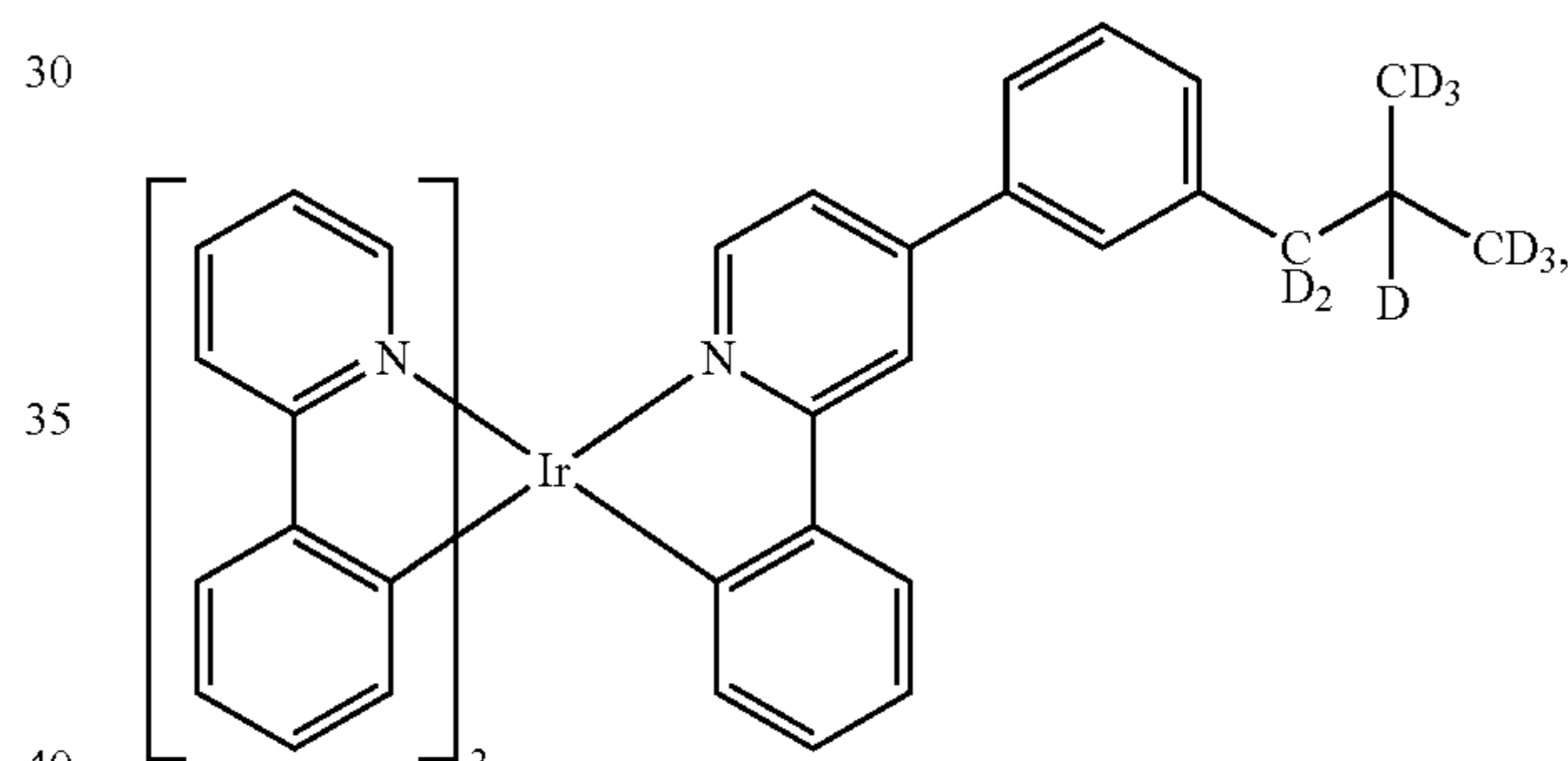
Compound 93
