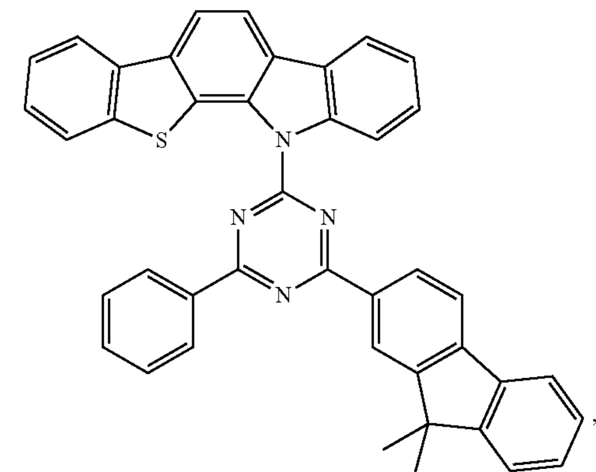
Compound EH7
