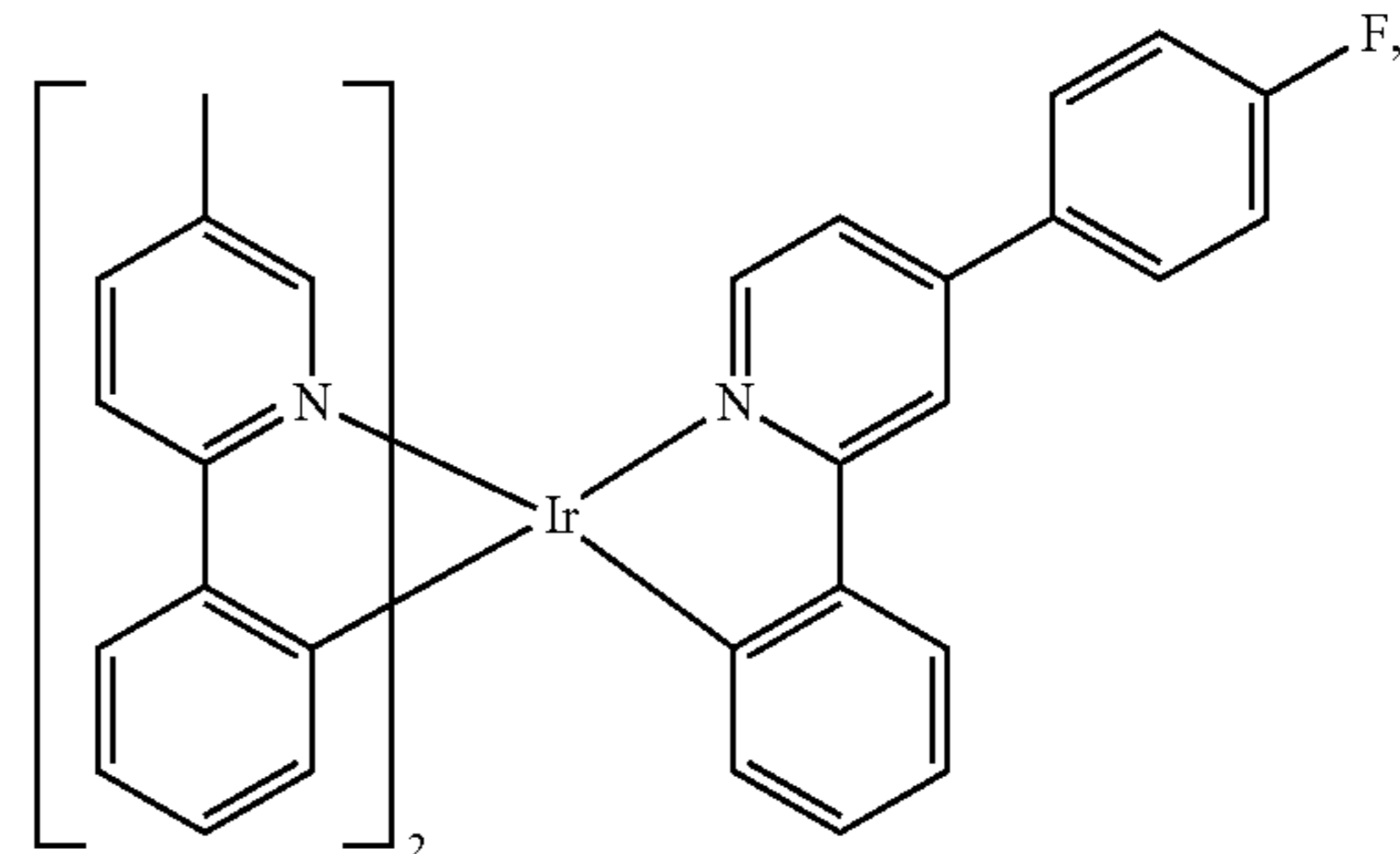
Compound 63
