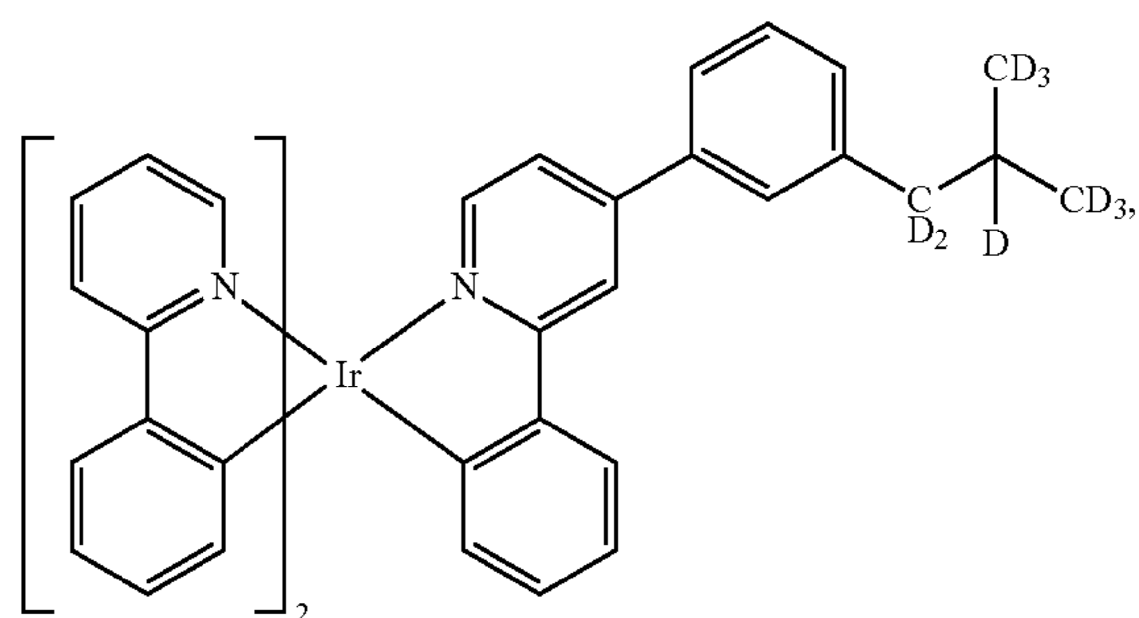
Compound 93
