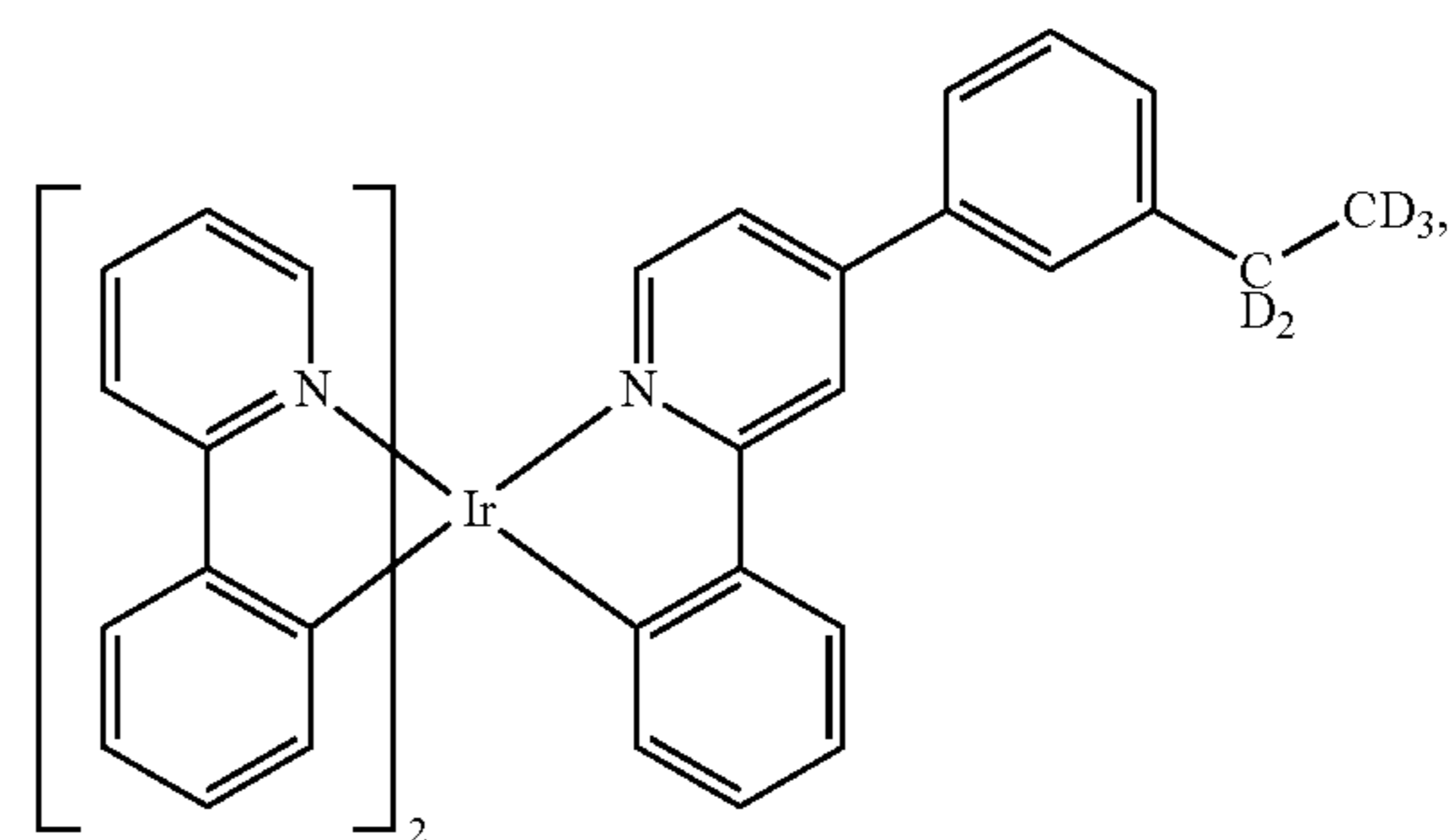
Compound 91
