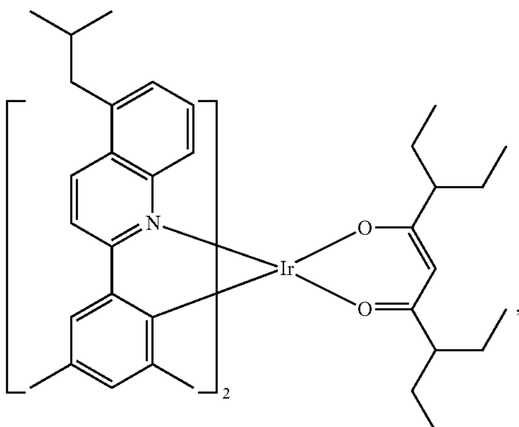
Compound E6
