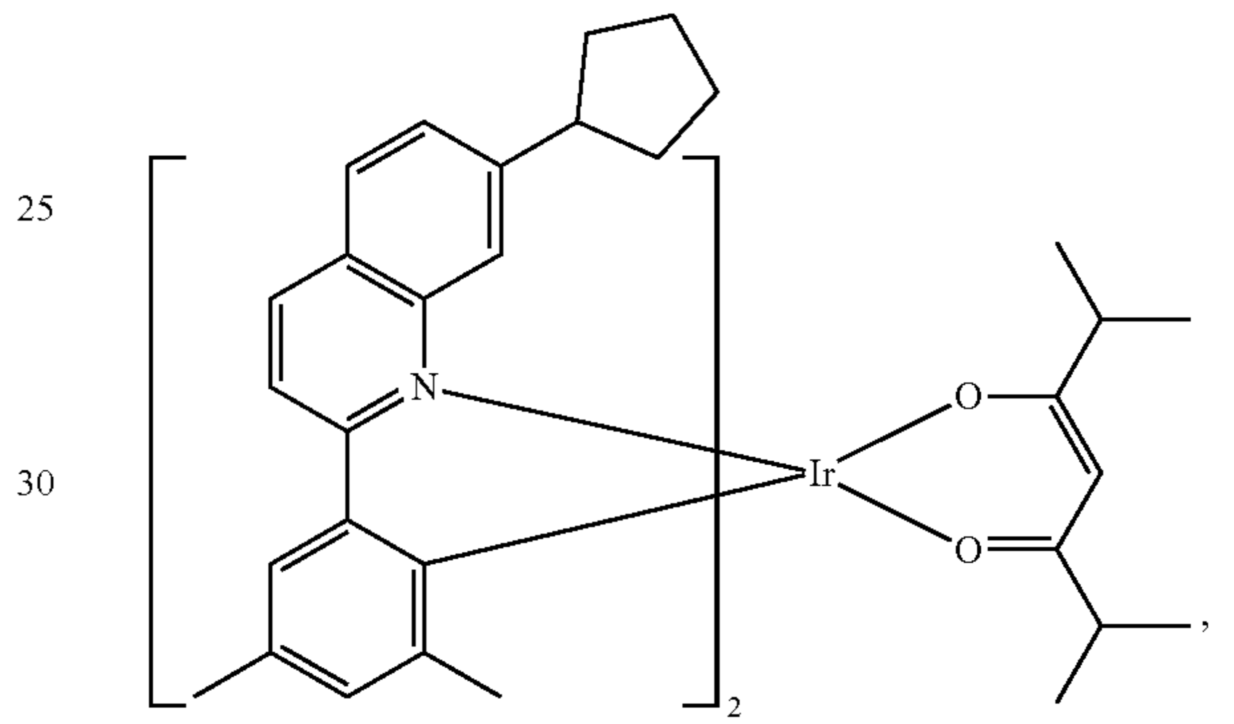
Compound E24
