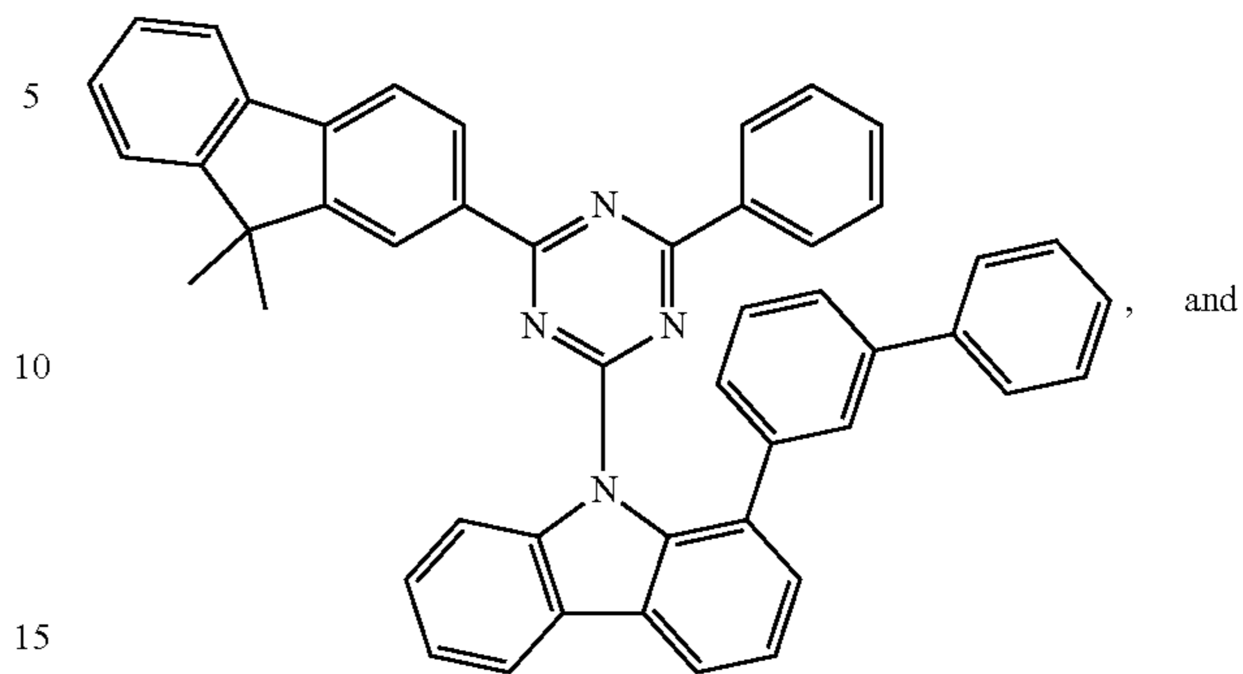
Compound H49
