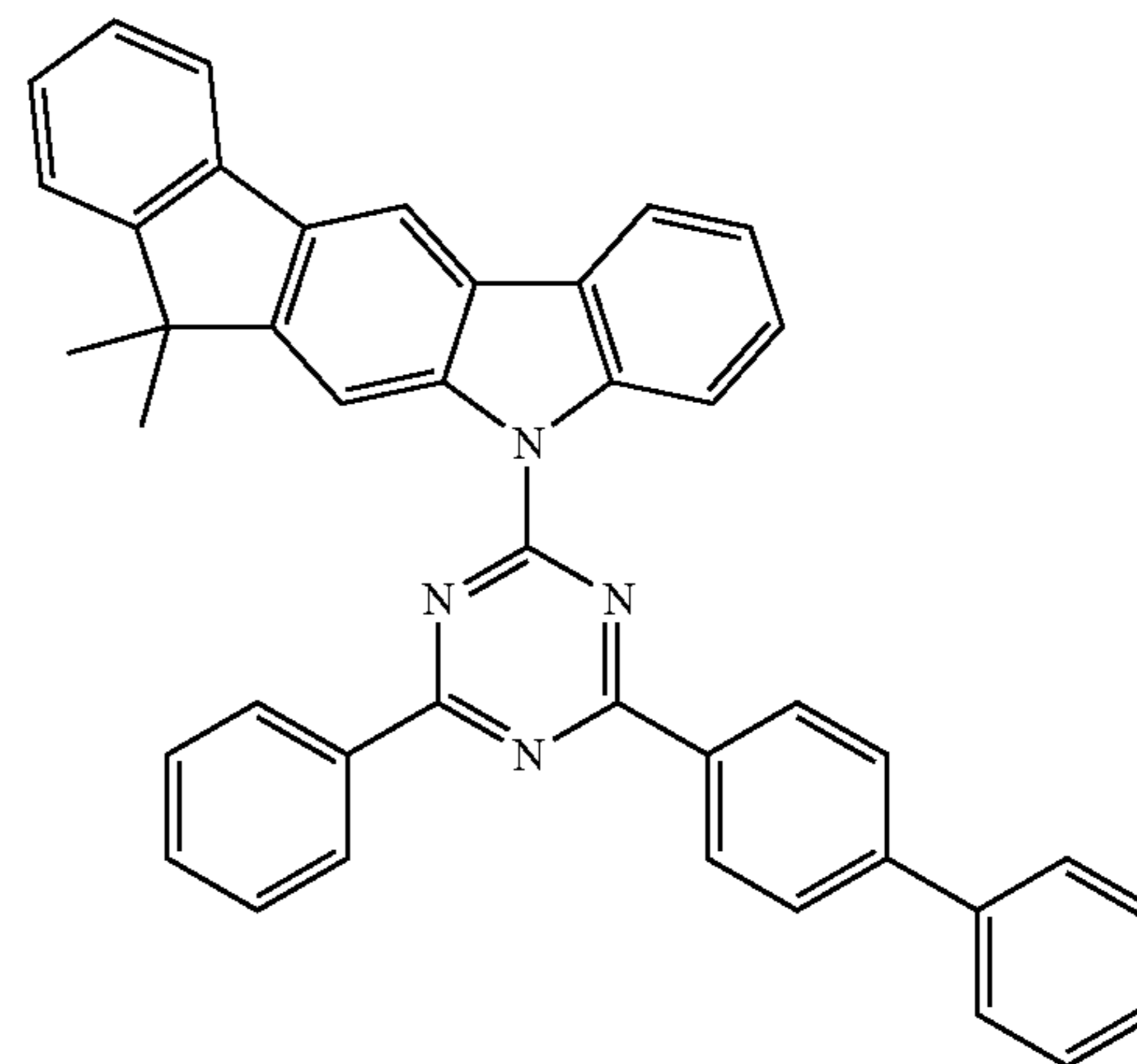
Compound EH28
