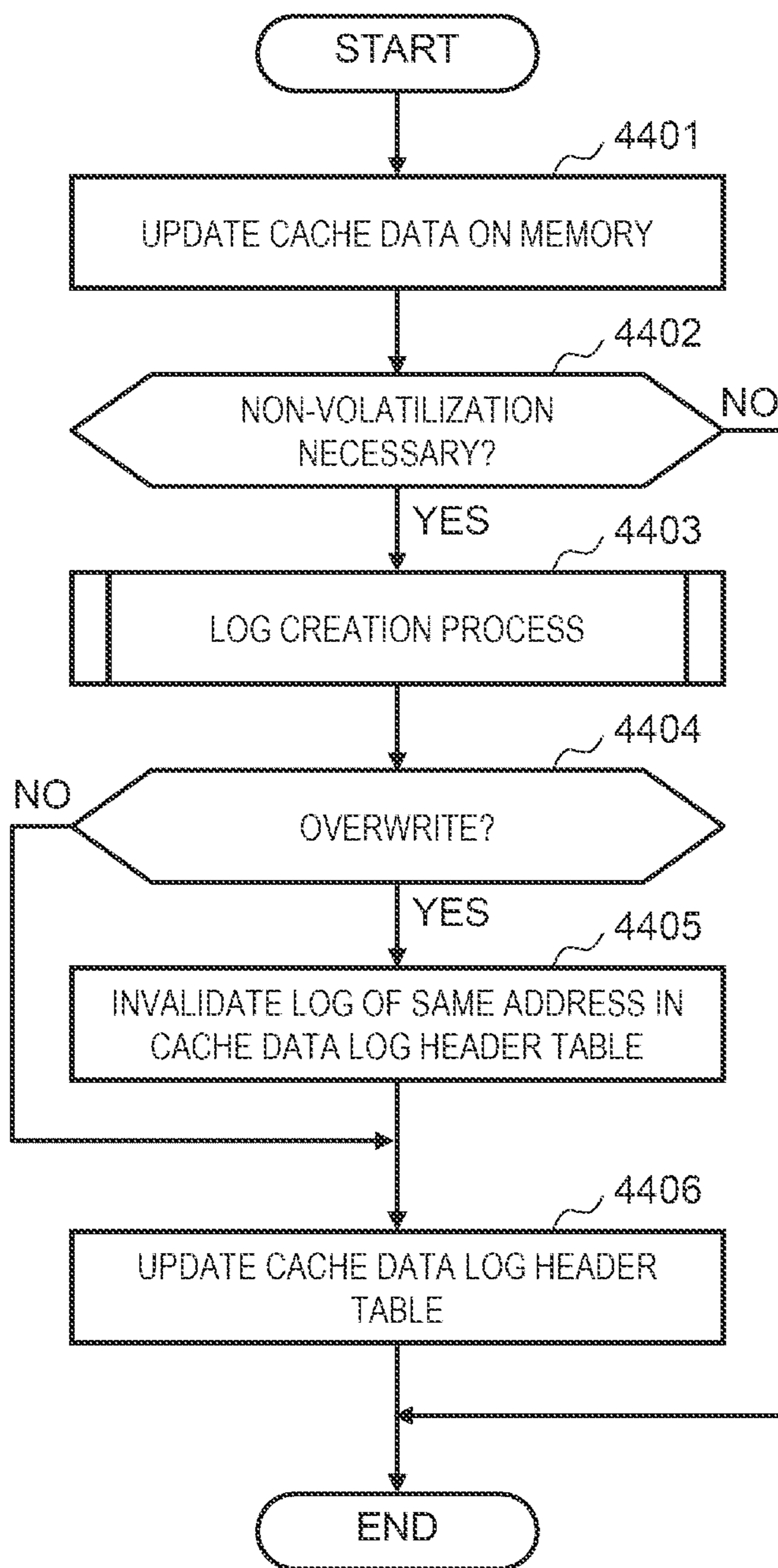
CACHE DATA UPDATE PROCESS
