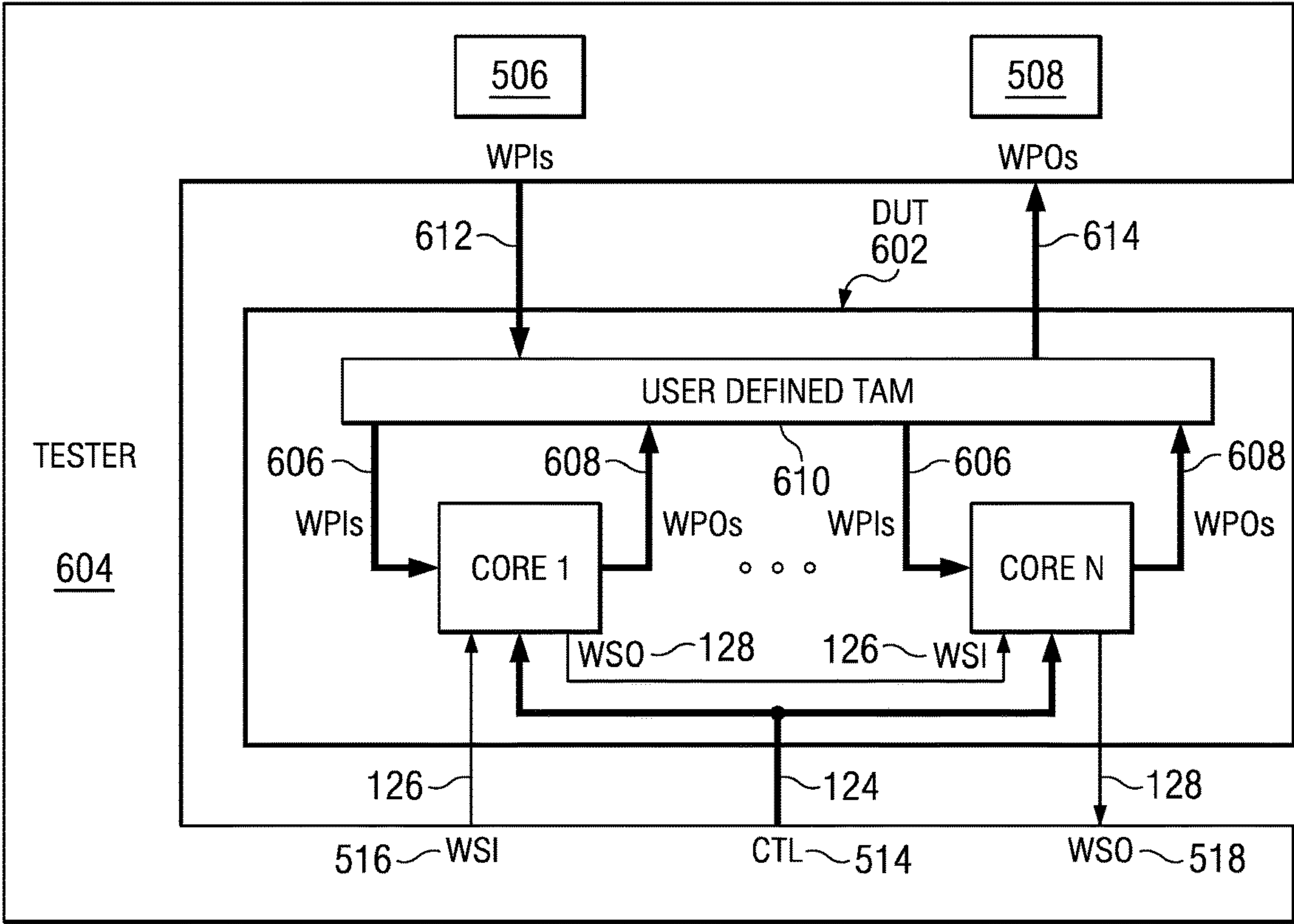
FIG. 6 (PRIOR ART)
