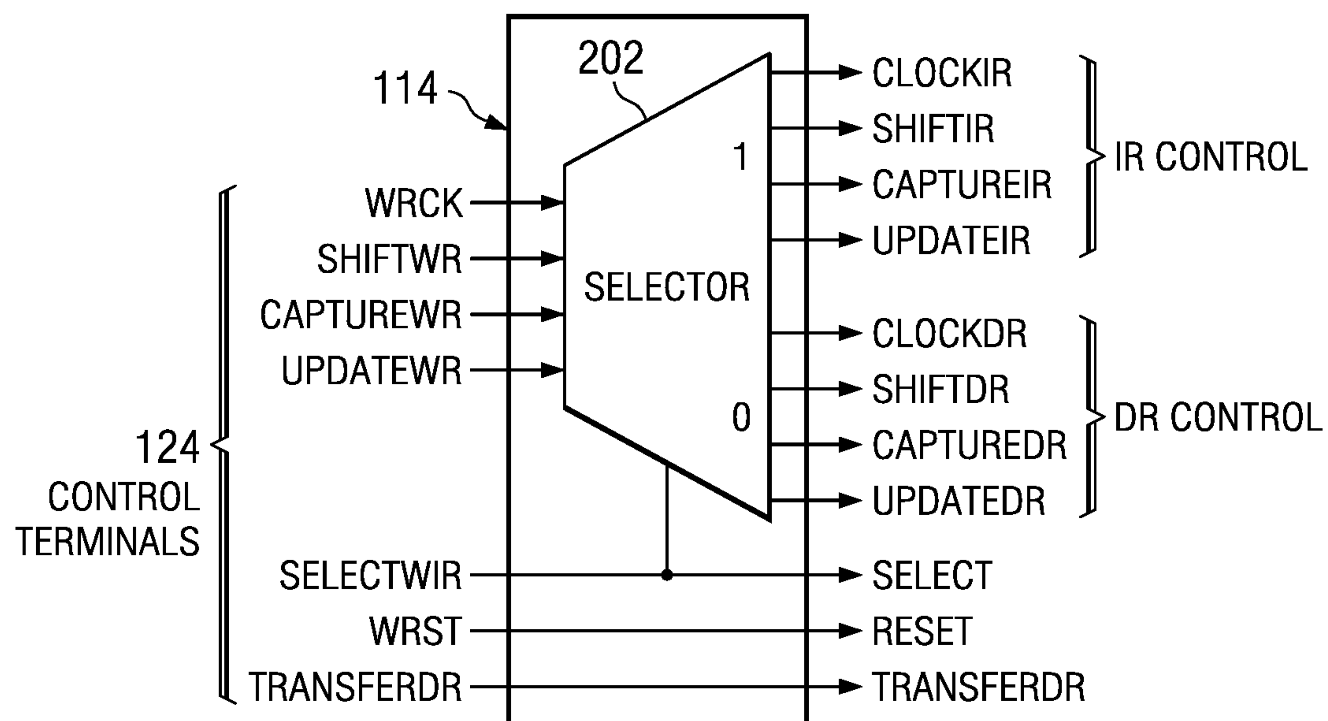
FIG. 2 (PRIOR ART)
