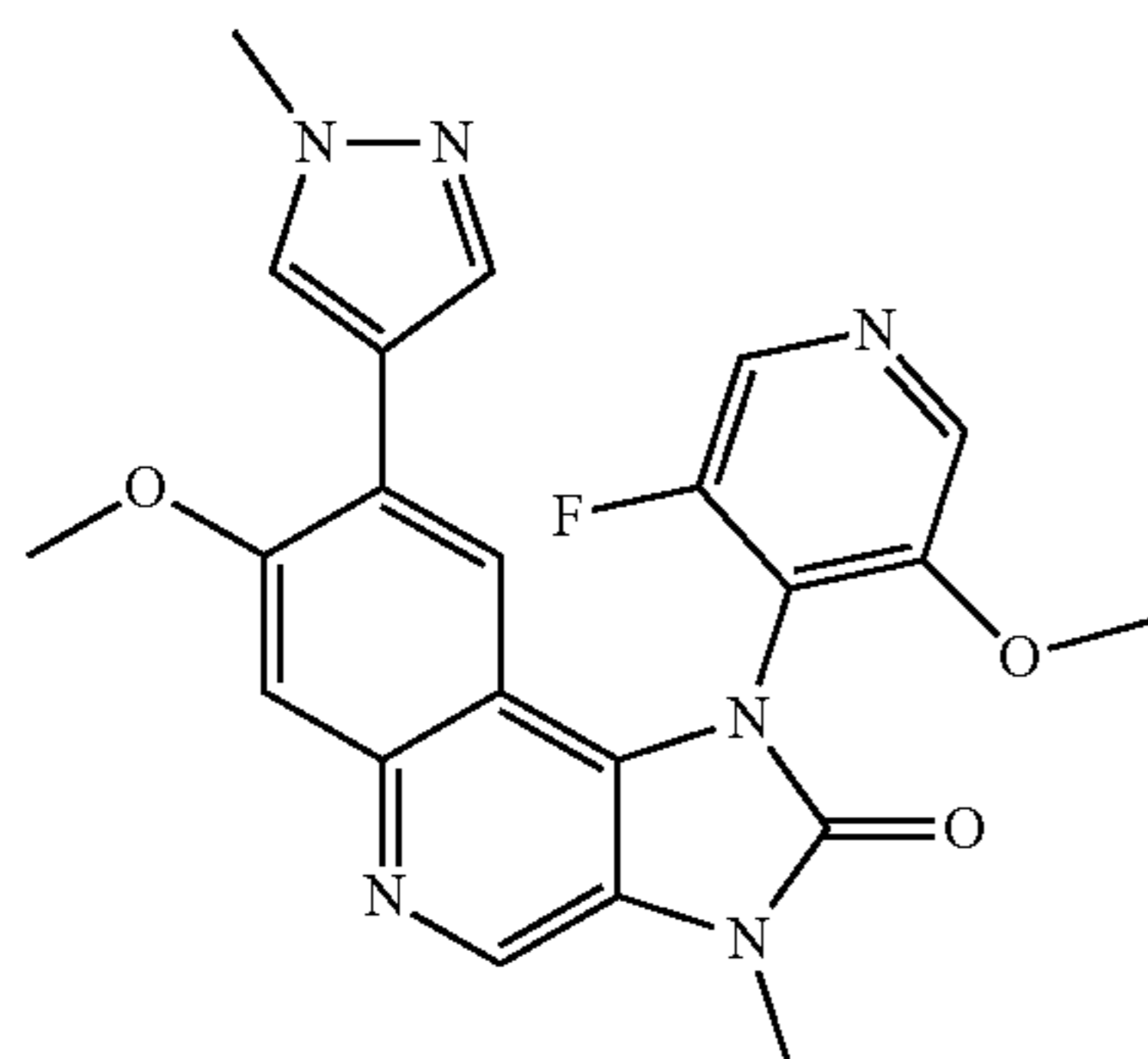
1-(3-Fluoro-5-methoxypyridin-4-yl)-7-methoxy-3-methyl-8-(1-methyl-1H-pyrazol-4-yl)-1,3-dihydroimidazo[4,5-c]quinolin-2-one
