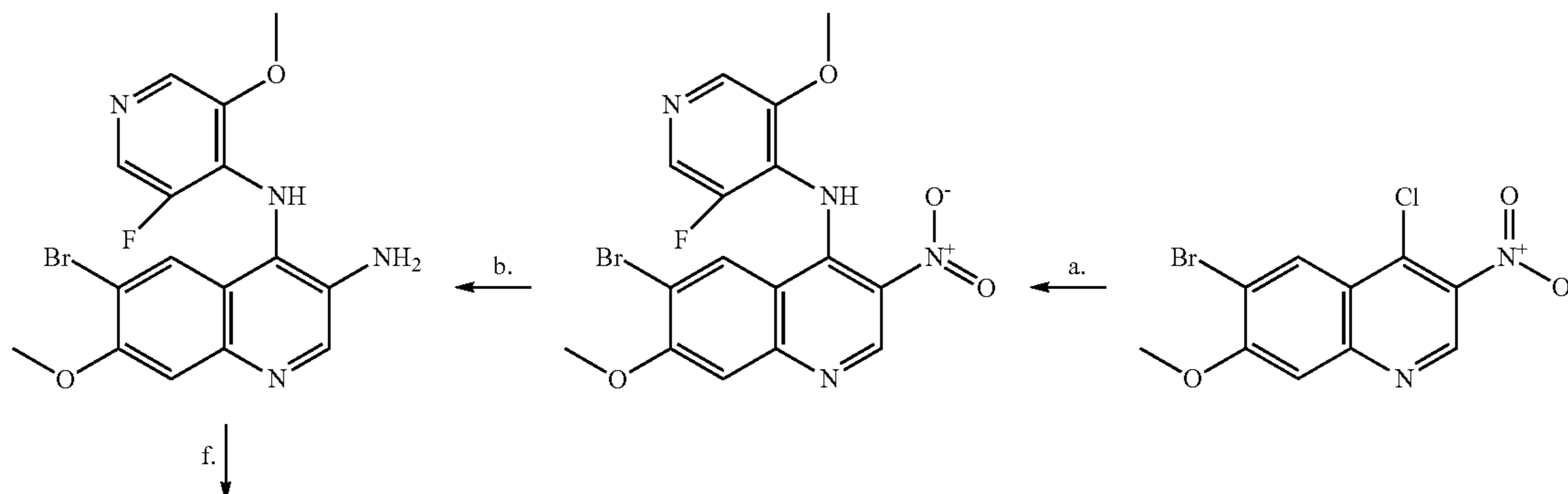
Scheme 3: Synthesis of Compound Example 4
