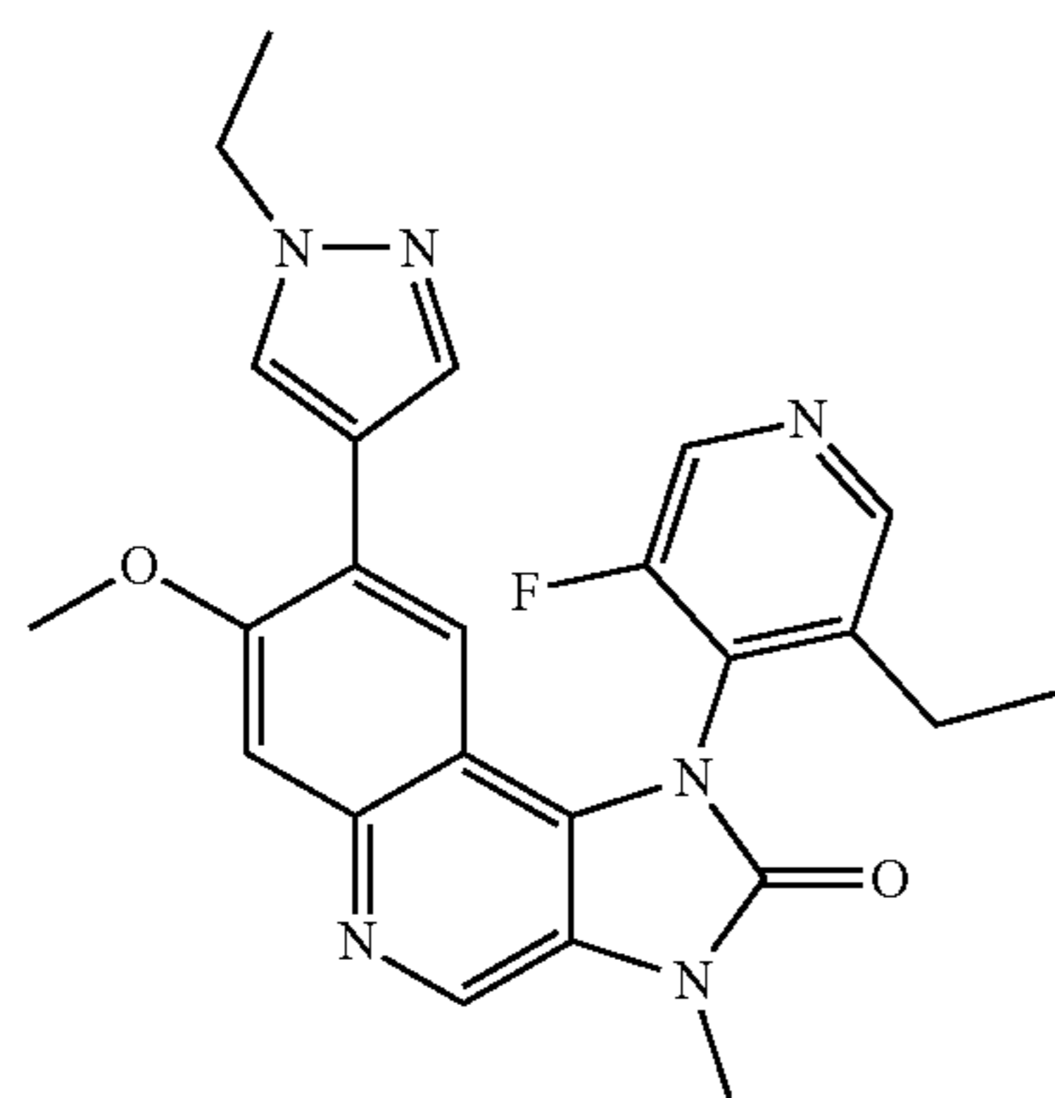
1-(3-Ethyl-5-fluoropyridin-4-yl)-8-(1-ethyl-1H-pyrazol-4-yl)-7-methoxy-3-methyl-1,3-dihydroimidazo[4,5-c]quinolin-2-one
