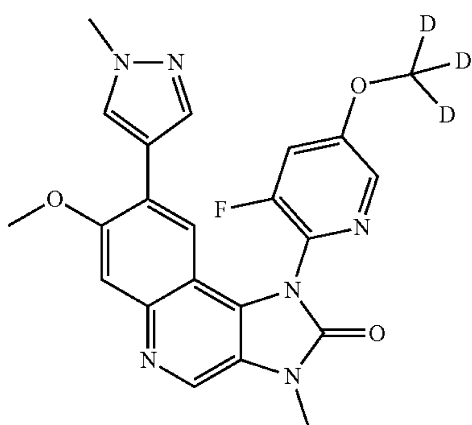
1-[3-Fluoro-5-(trideuteriomethoxy)-2-pyridyl]-7-methoxy-3-methyl-8-(1-methylpyrazol-4-yl)imidazo[4,5-c]quinolin-2-one
