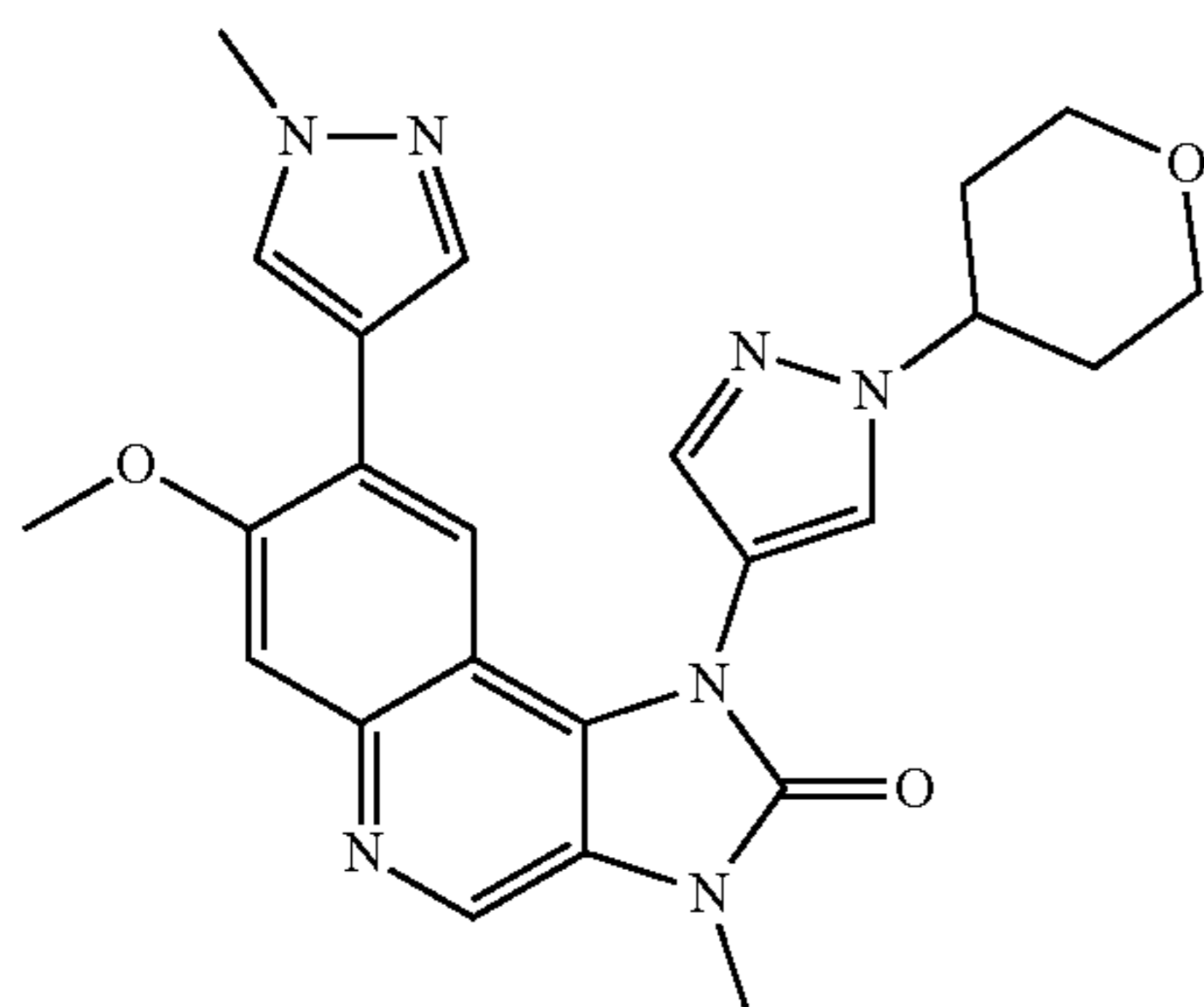
7-Methoxy-3-methyl-8-(1-methyl-1H-pyrazol-4-yl)-1-[1-(tetrahydropyran-4-yl)-1H-pyrazol-4-yl]-1,3-dihydroimidazo[4,5-c]quinolin-2-one
