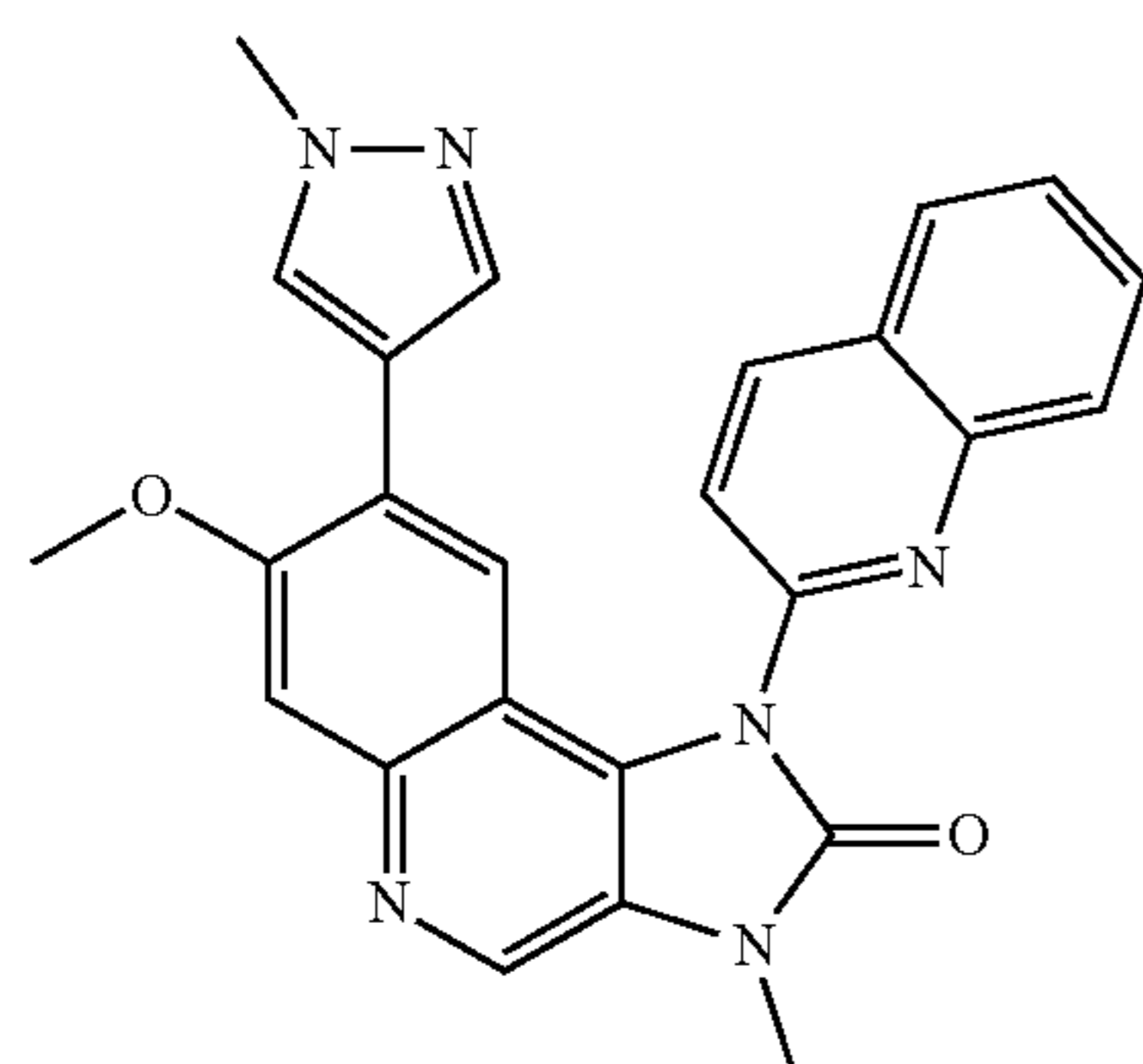
7-Methoxy-3-methyl-8-(1-methyl-1H-pyrazol-4-yl)-1-quinolin-2-yl-1,3-dihydroimidazo[4,5-c]quinolin-2-one
