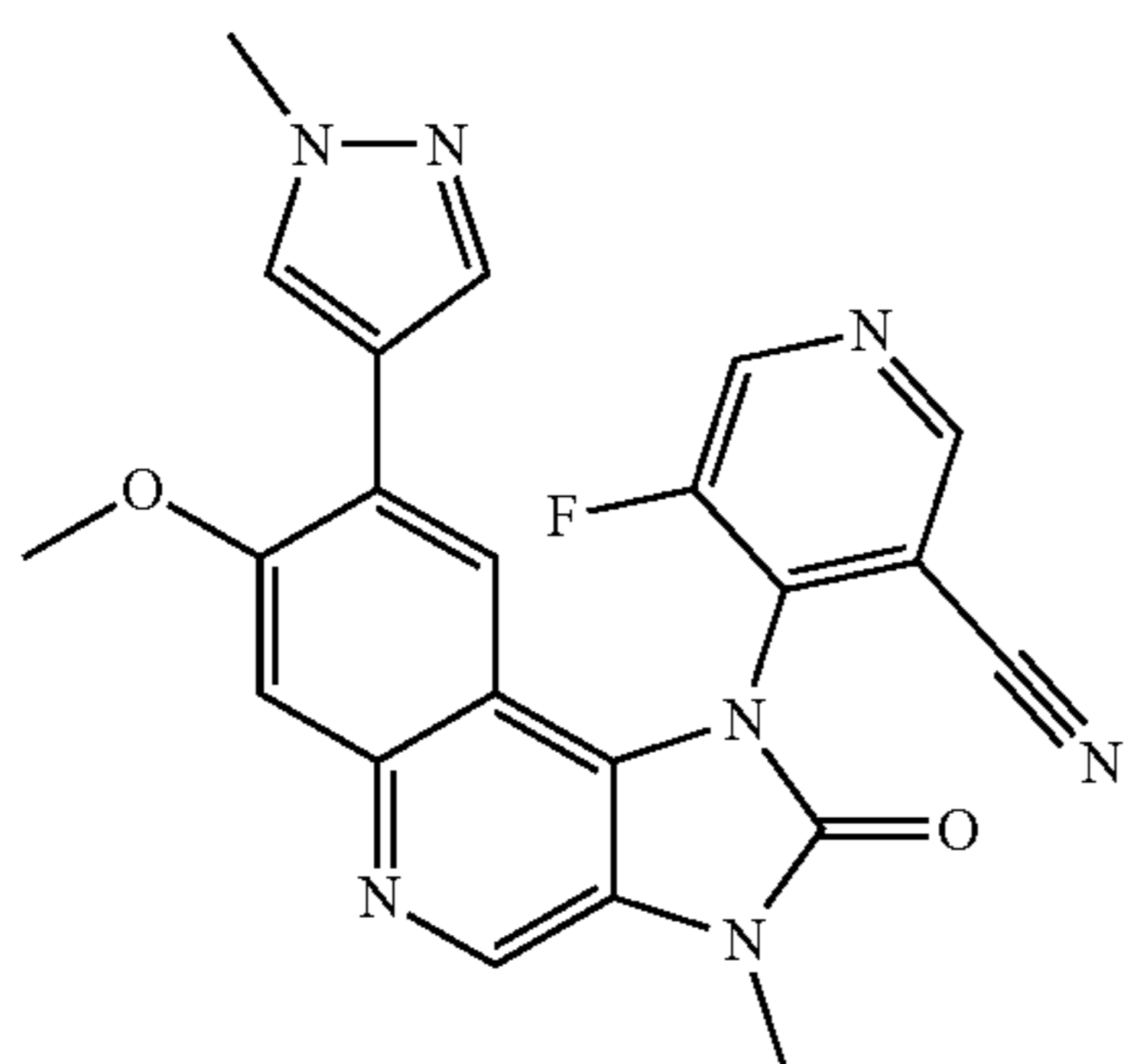
5-Fluoro-4-[7-methoxy-3-methyl-8-(1-methyl-1H-pyrazol-4-yl)-2-oxo-2,3-dihydroimidazo[4,5-c]quinolin-1-yl]nicotinonitrile
