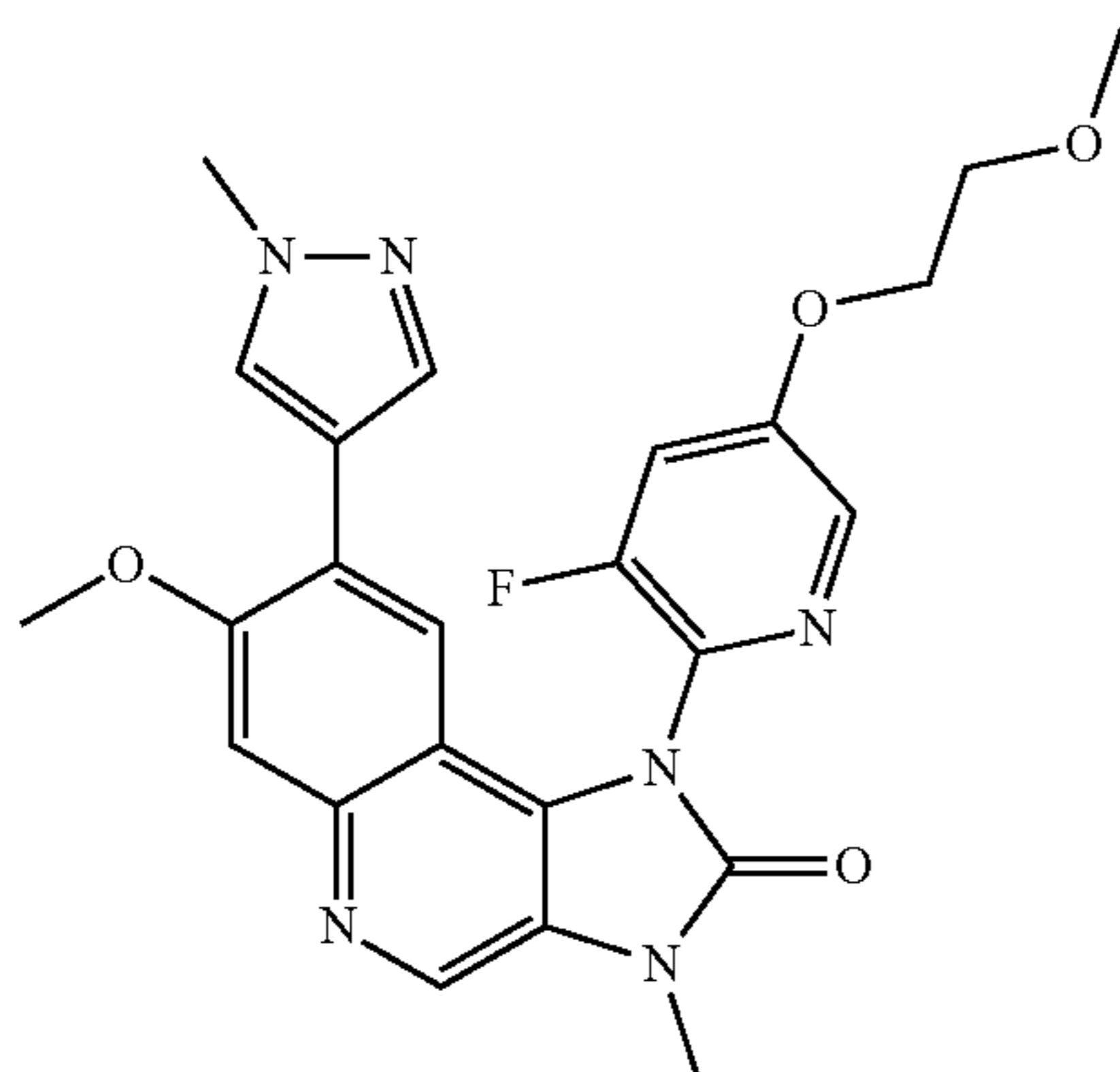
1-[3-Fluoro-5-(2-methoxyethoxy)-2-pyridyl]-7-methoxy-3-methyl-8-(1-methylpyrazol-4-yl)imidazo[4,5-c]quinolin-2-one
