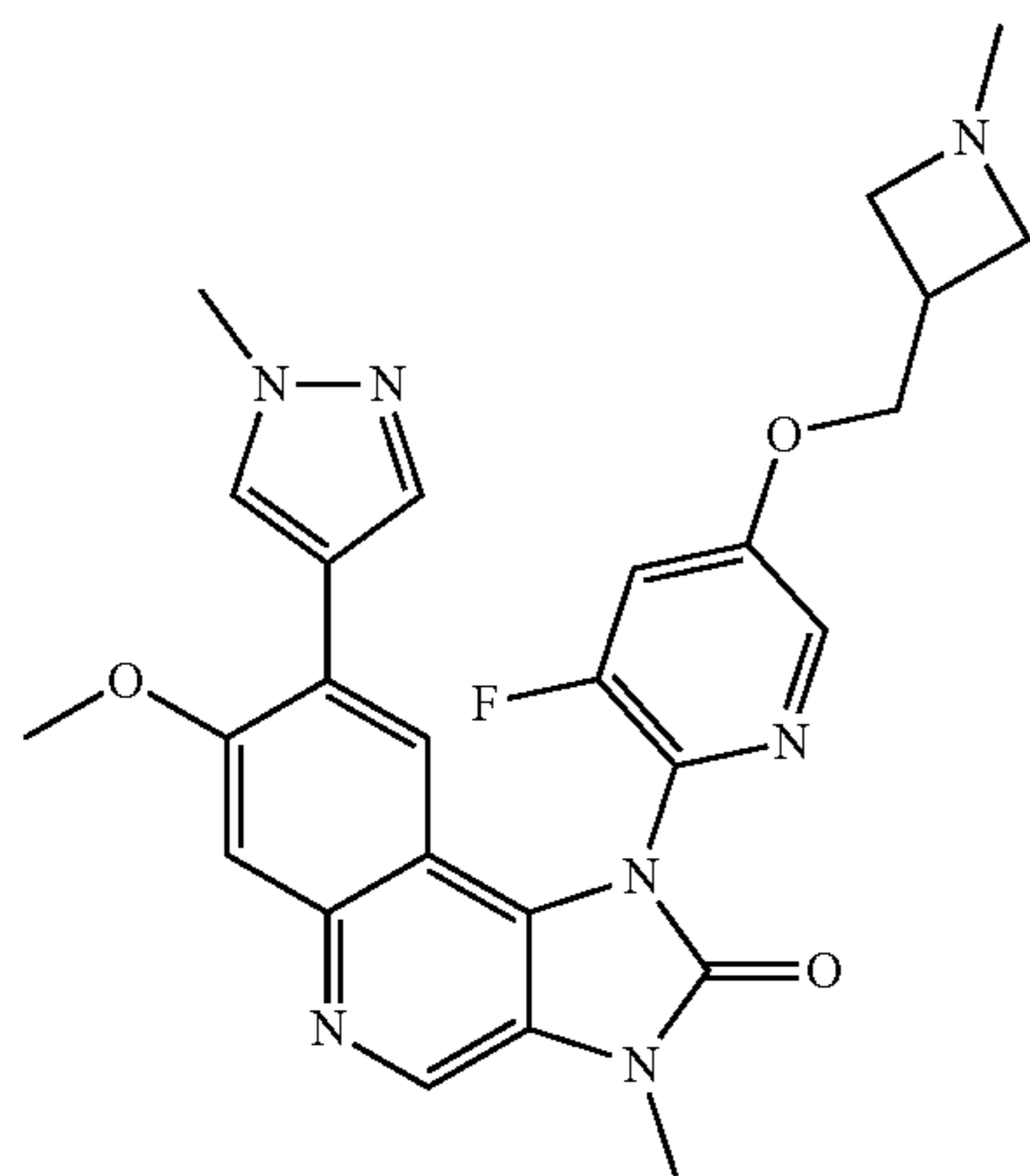
1-[3-Fluoro-5-(1-methylazetidin-3-ylmethoxy)pyridin-2-yl]-7-methoxy-3-methyl-8-(1-methyl-1H-pyrazol-4-yl)-1,3-dihydroimidazo[4,5-c]quinolin-2-one
