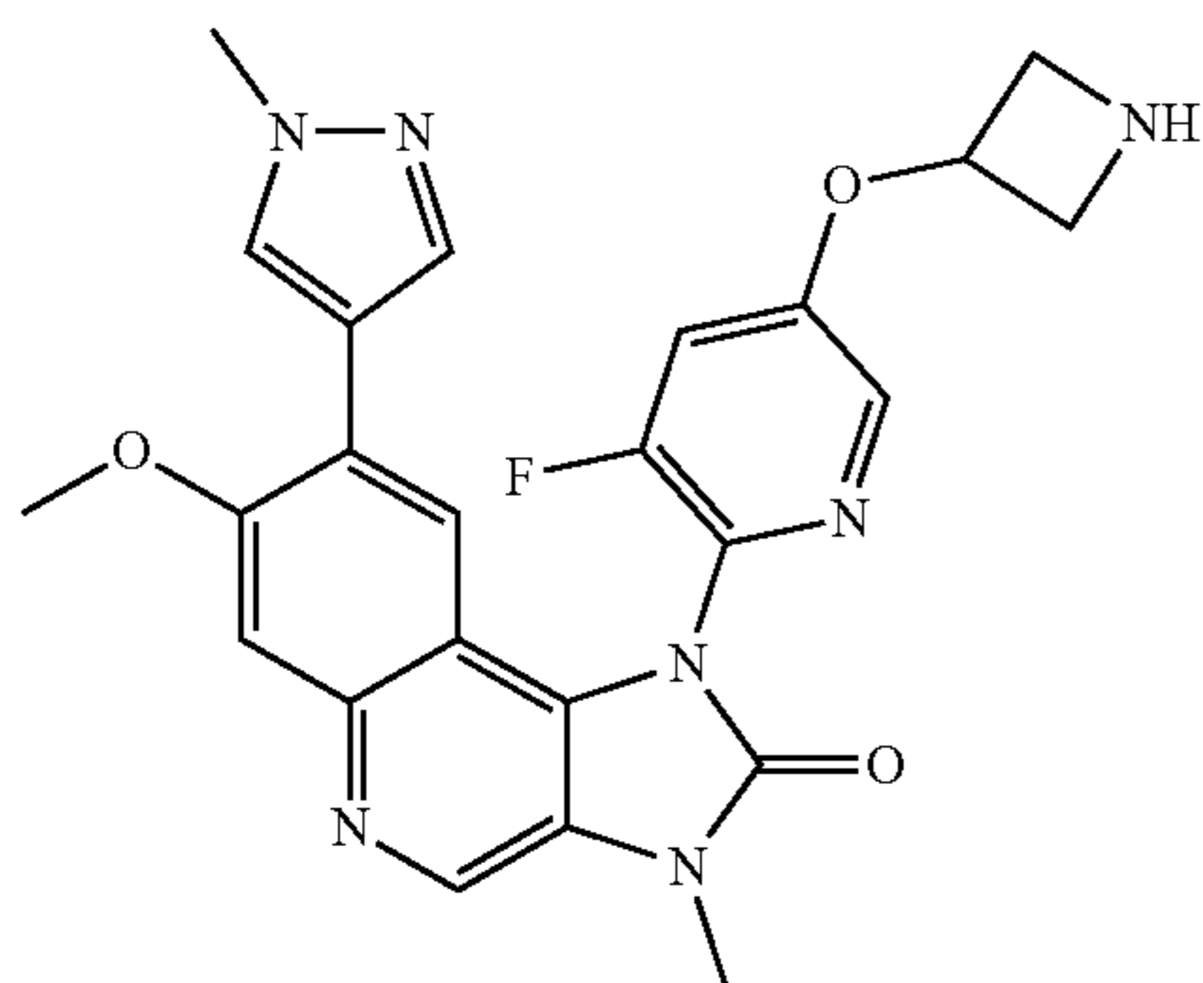
1-[5-(Azetidin-3-yloxy)-3-fluoropyridin-2-yl]-7-methoxy-3-methyl-8-(1-methyl-1H-pyrazol-4-yl)-1,3-dihydroimidazo[4,5-c]quinolin-2-one
