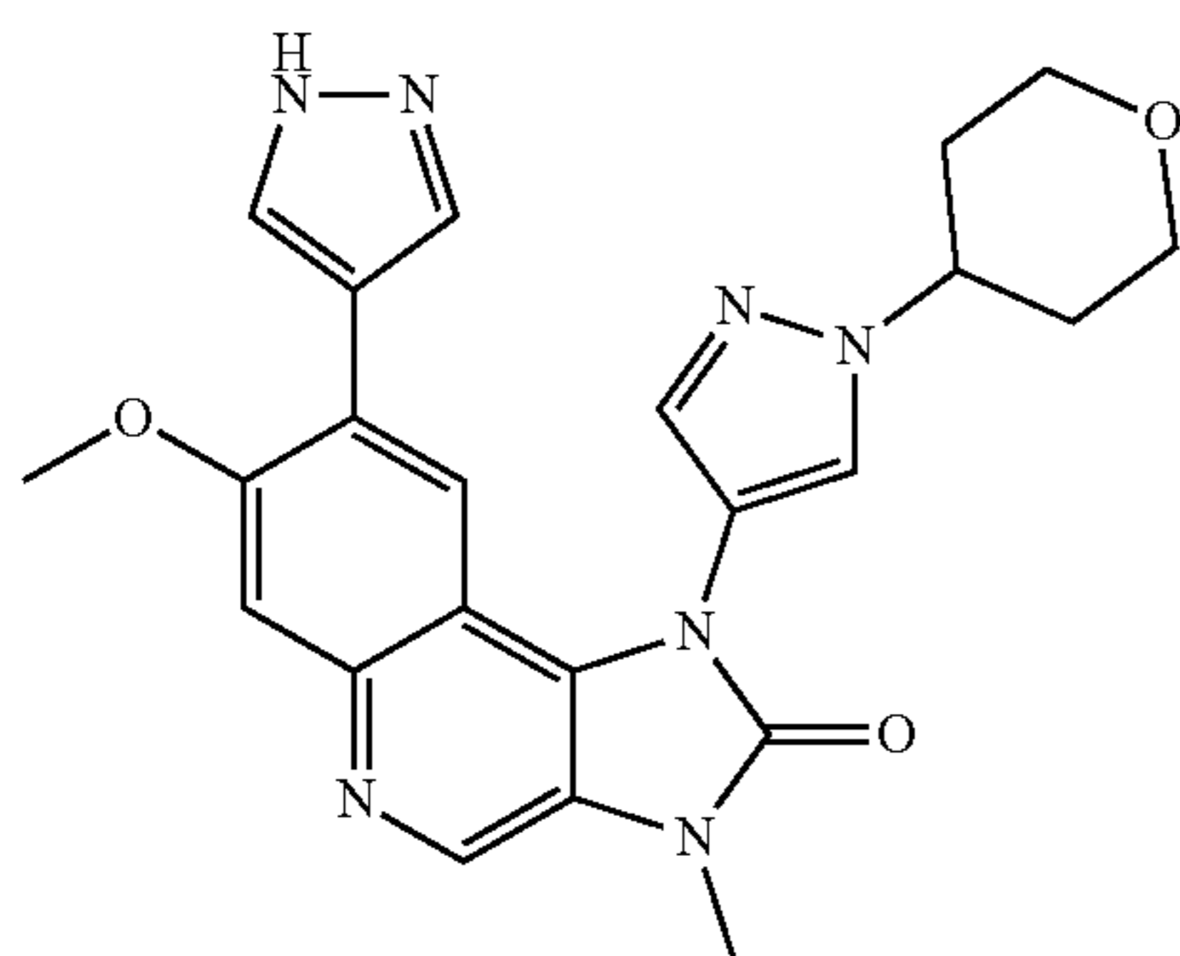
7-Methoxy-3-methyl-8-(1H-pyrazol-4-yl)-1-[1-(tetrahydropyran-4-yl)-1H-pyrazol-4-yl]-1,3-dihydroimidazo[4,5-c]quinolin-2-one
