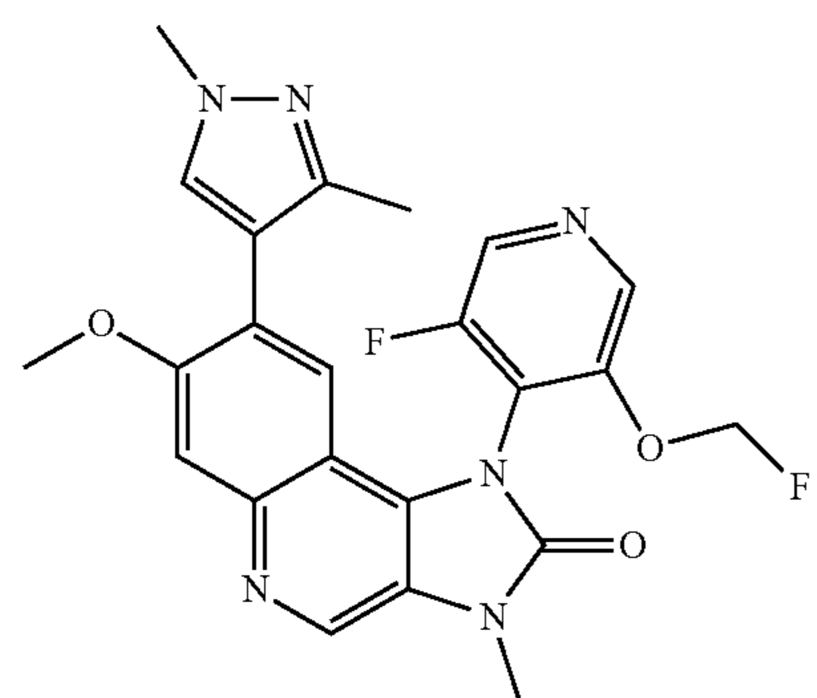
8-(1,3-Dimethyl-1H-pyrazol-4-yl)-1-(3-fluoro-5-fluoromethoxypyridin-4-yl)-7-methoxy-3-methyl-1,3-dihydroimidazo[4,5-c]quinolin-2-one
