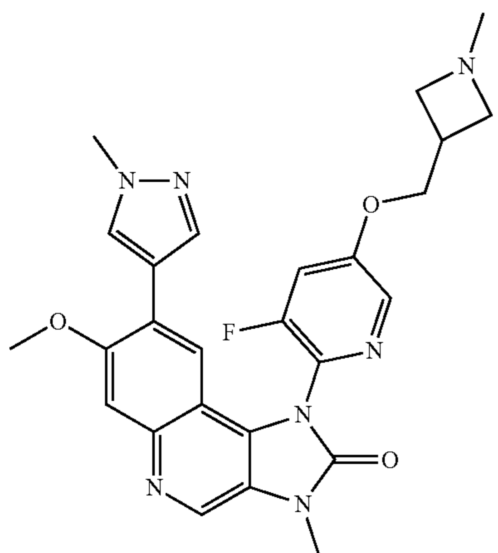
1-[3-Fluoro-5-(1-methylazetidin-3-ylmethoxy)pyridin-2-yl]-7-methoxy-3-methyl-8-(1-methyl-1H-pyrazol-4-yl)-1,3-dihydroimidazo[4,5-c]quinolin-2-one
