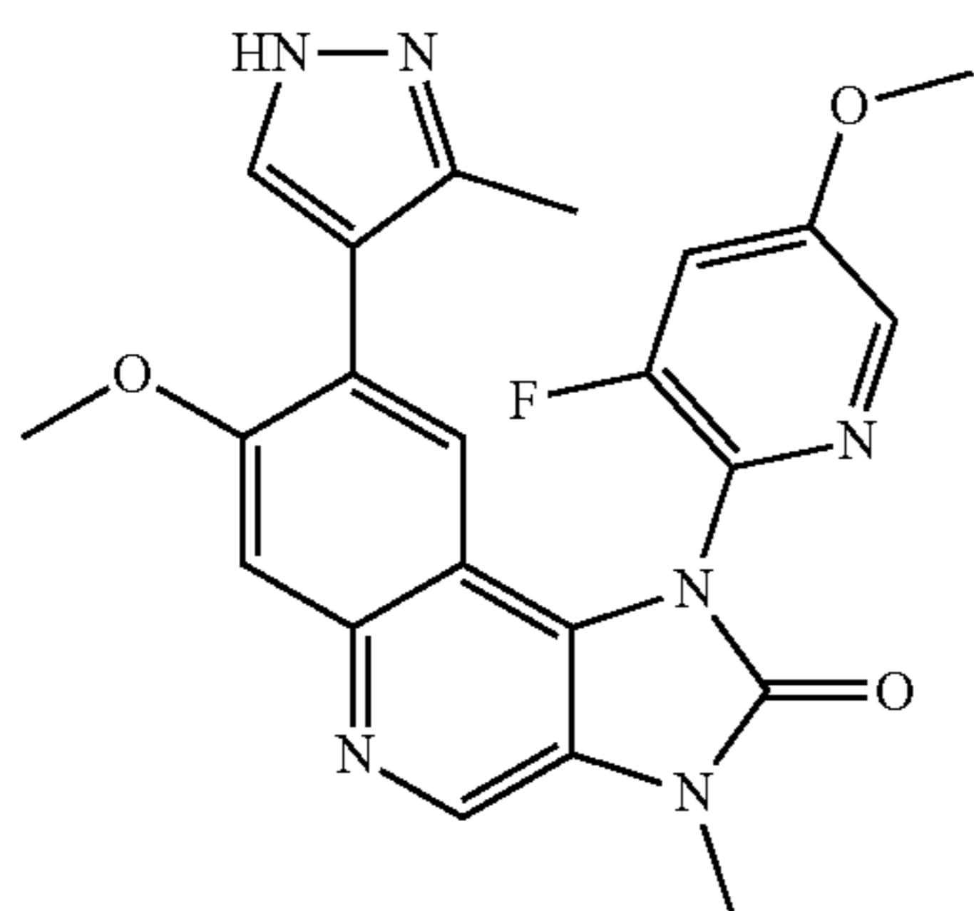
1-(3-Fluoro-5-methoxypyridin-2-yl)-7-methoxy-3-methyl-8-(3-methyl-1H-pyrazol-4-yl)-1,3-dihydroimidazo[4,5-c]quinolin-2-one
