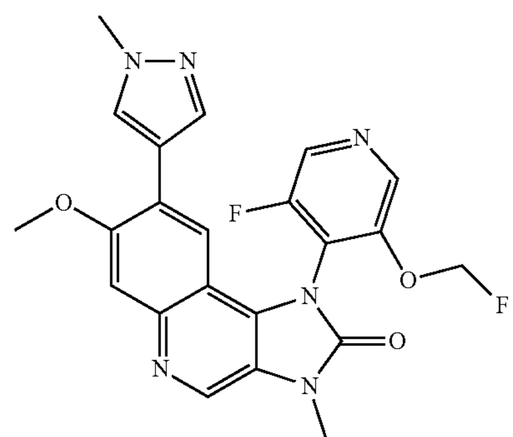
1-(3-Fluoro-5-fluoromethoxypyridin-4-yl)-7-methoxy-3-methyl-8-(1-methyl-1H-pyrazol-4-yl)-1,3-dihydroimidazo[4,5-c]quinolin-2-one
