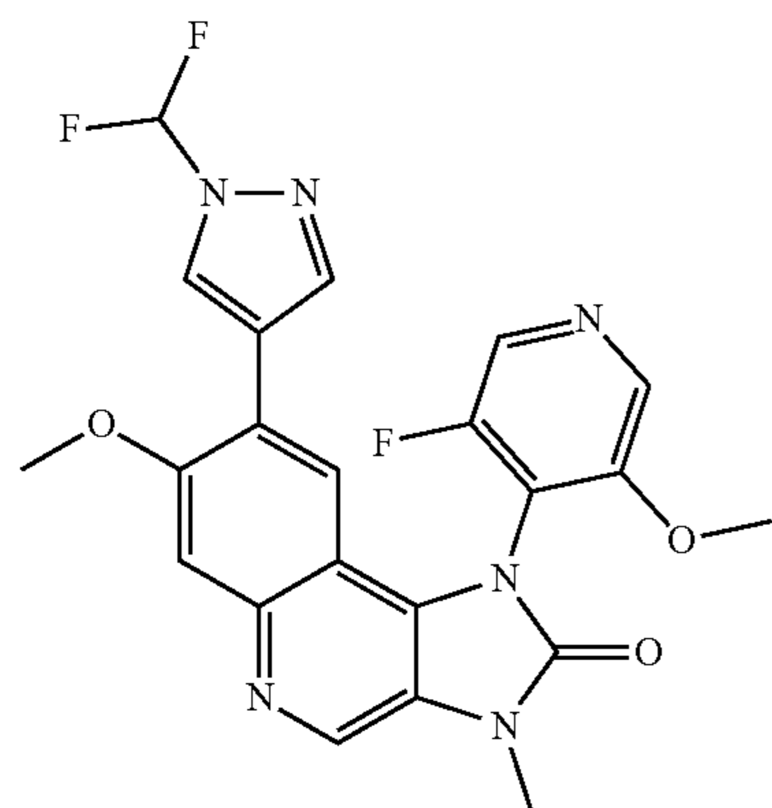
8-(1-Difluoromethyl-1H-pyrazol-4-yl)-1-(3-fluoro-5-methoxy-pyridin-4-yl)-7-methoxy-3-methyl-1,3-dihydroimidazo[4,5-c]quinolin-2-one
