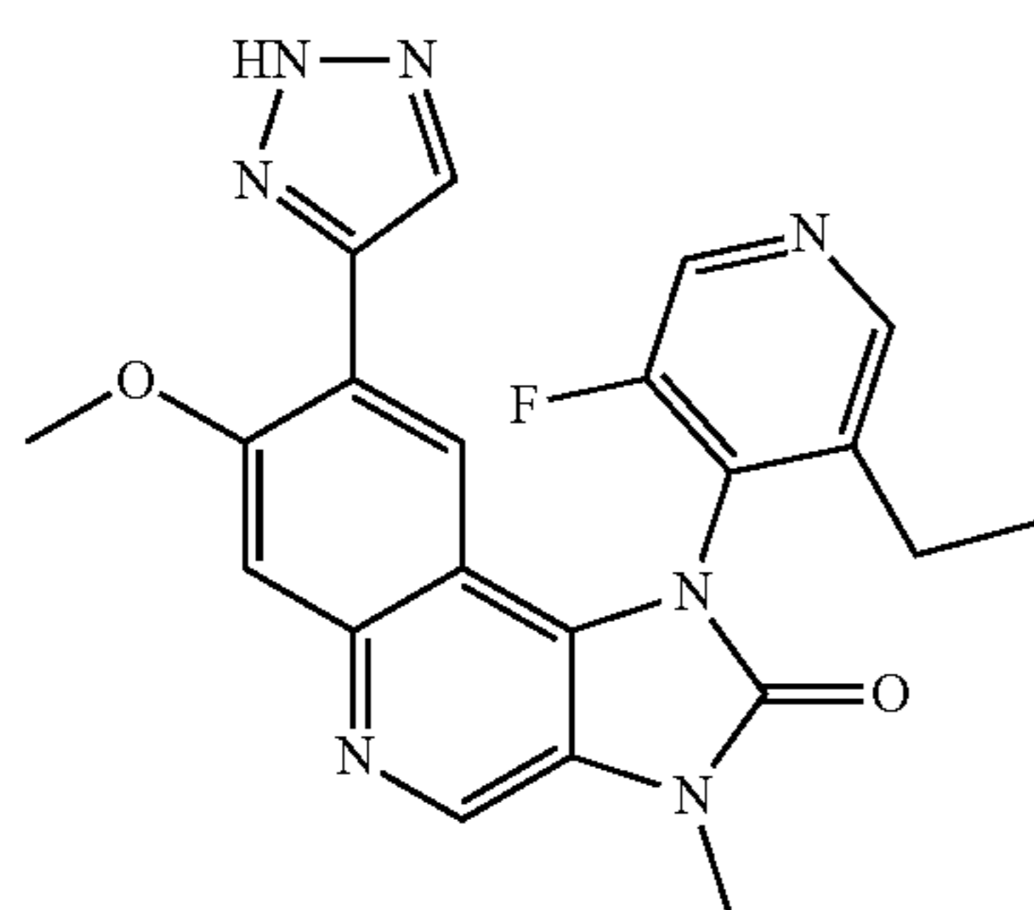
1-(3-Ethyl-5-fluoropyridin-4-yl)-7-methoxy-3-methyl-8-(2H-1,2,3-triazol-4-yl)-1,3-dihydroimidazo[4,5-c]quinolin-2-one
