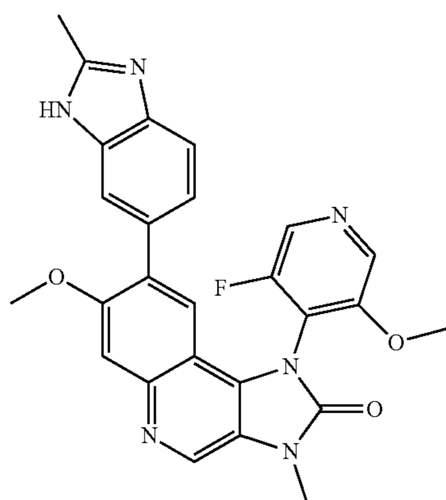
1-(3-Fluoro-5-methoxypyridin-4-yl)-7-methoxy-3-methyl-8-(2-methyl-3H-benzimidazol-5-yl)-1,3-dihydroimidazo[4,5-c]quinolin-2-one
