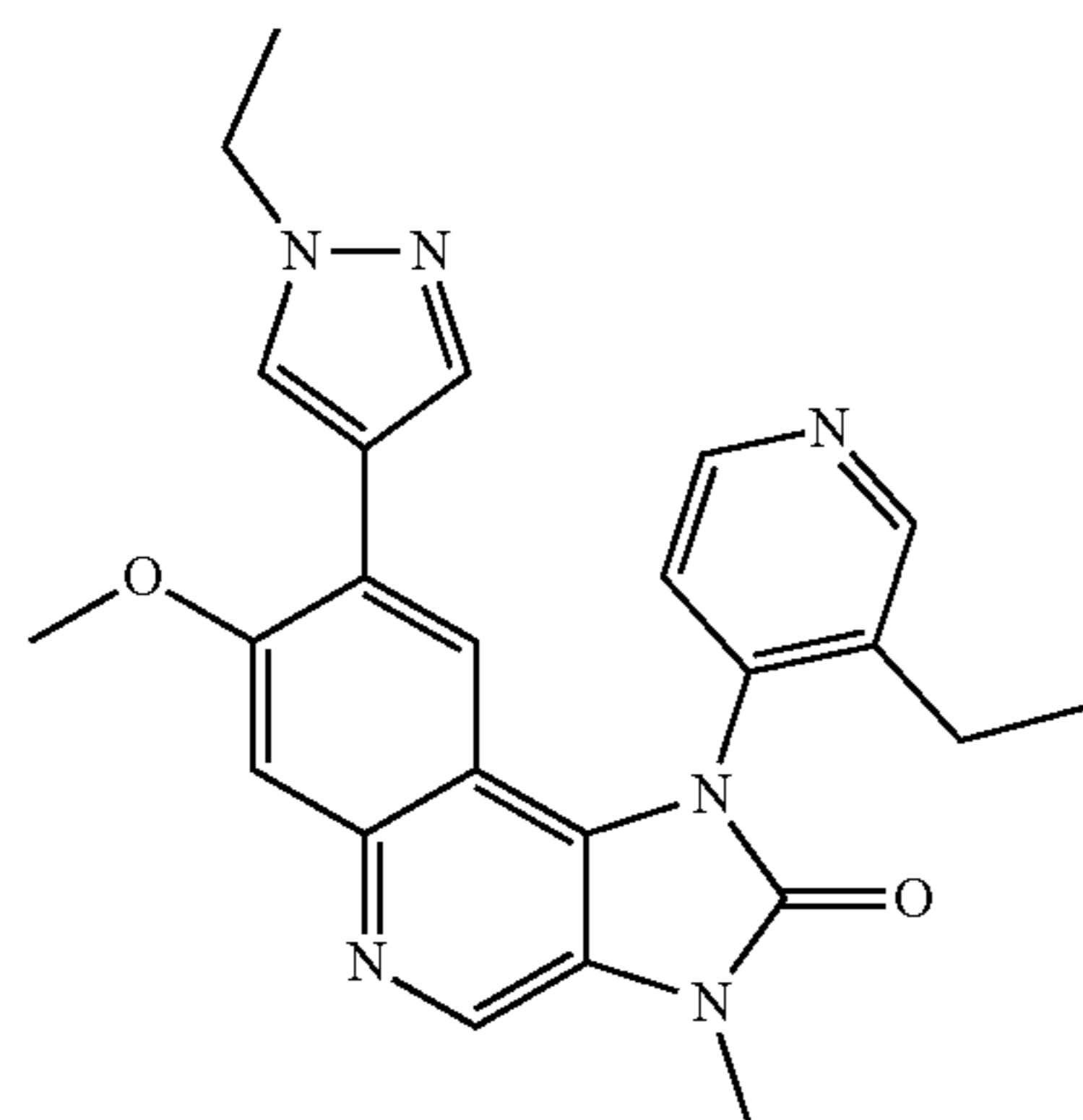
8-(1-Ethyl-1H-pyrazol-4-yl)-1-(3-ethylpyridin-4-yl)-7-methoxy-3-methyl-1,3-dihydroimidazo[4,5-c]quinolin-2-one
