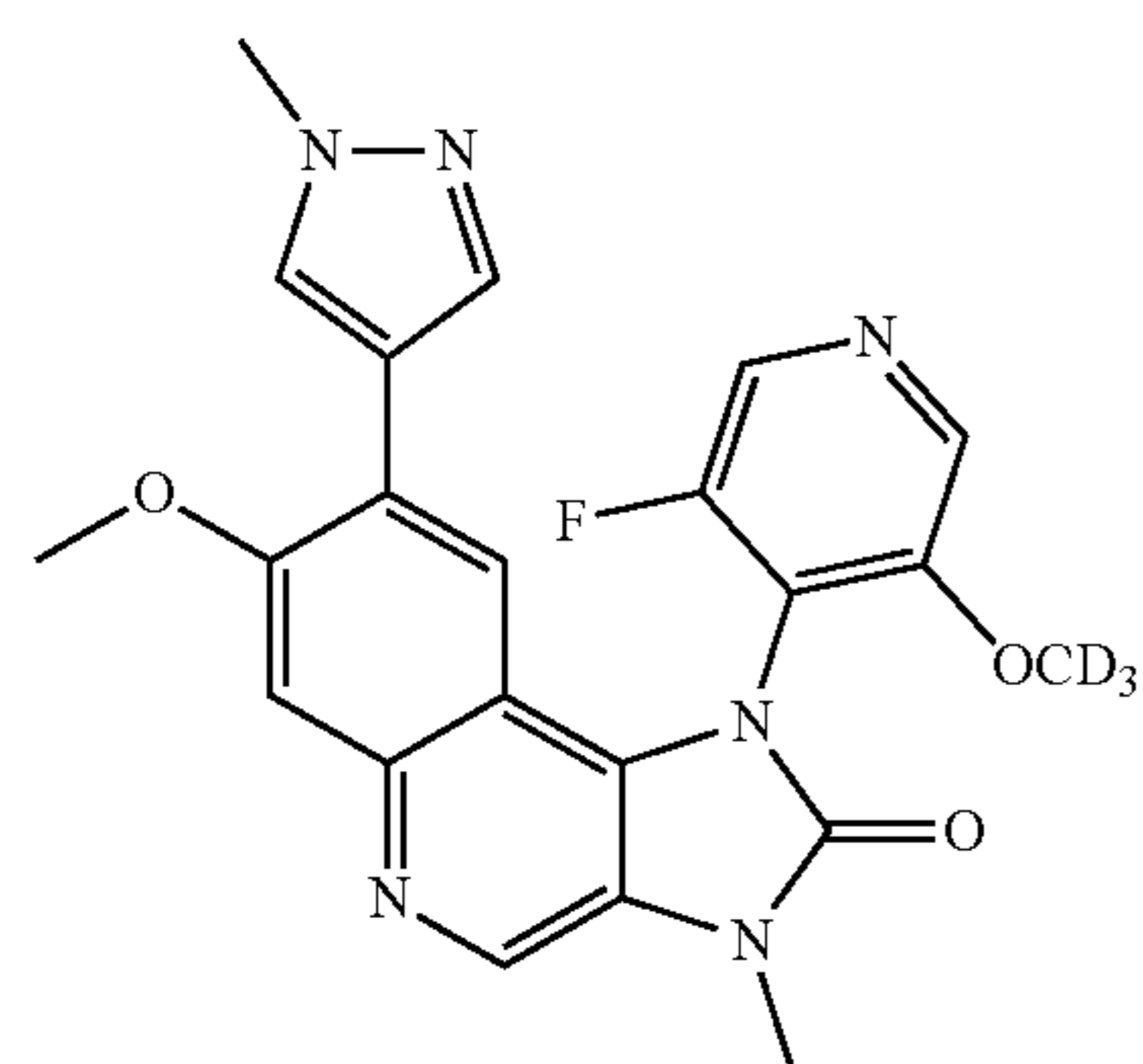
1-[3-Fluoro-5-(trideuteriomethoxy)-4-pyridyl]-7-methoxy-3-methyl-8-(1-methylpyrazol-4-yl)imidazo[4,5-c]quinolin-2-one
