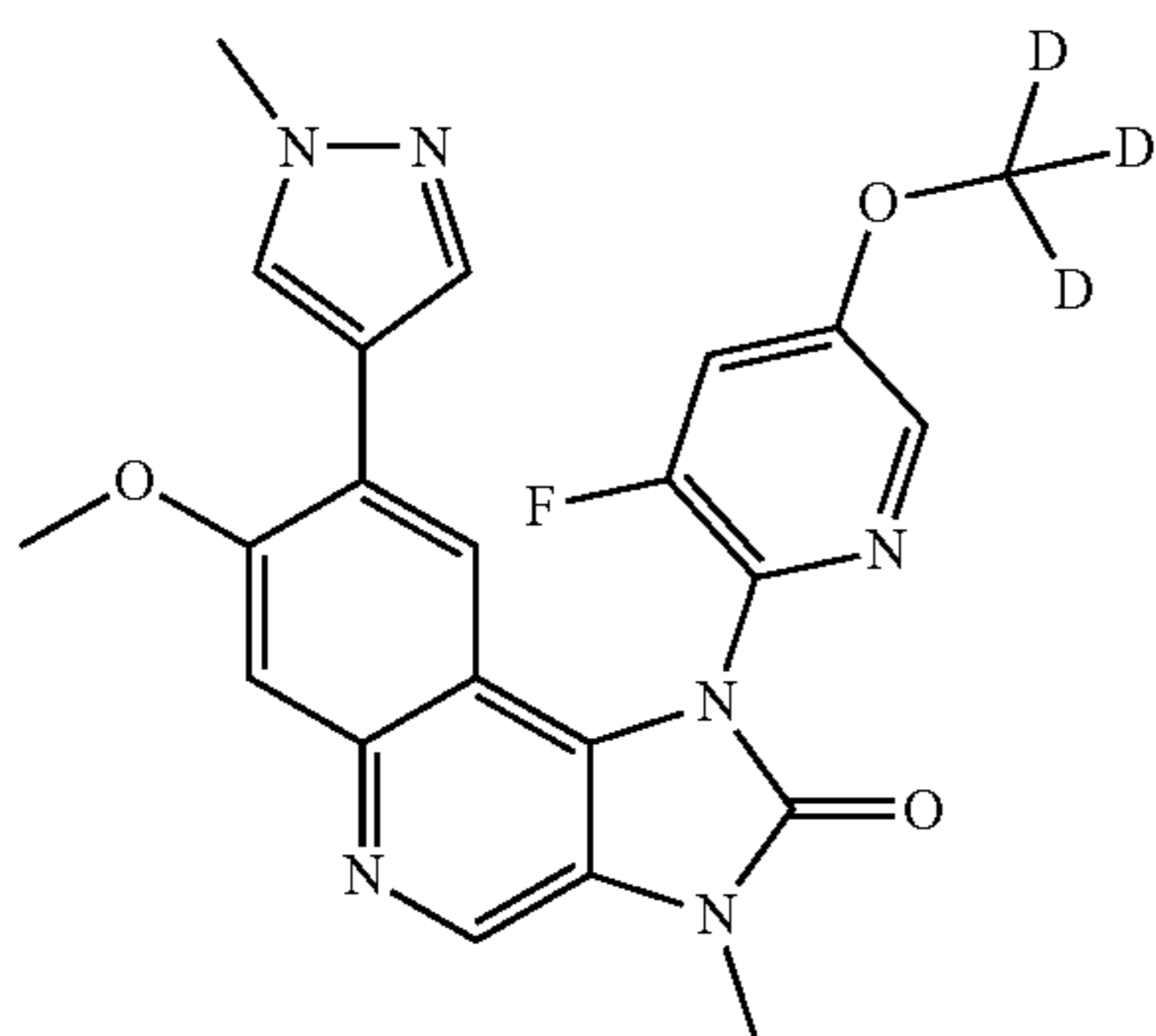
1-[3-Fluoro-5-(trideuteriomethoxy)-2-pyridyl]-7-methoxy-3-methyl-8-(1-methylpyrazol-4-yl)imidazo[4,5-c]quinolin-2-one
