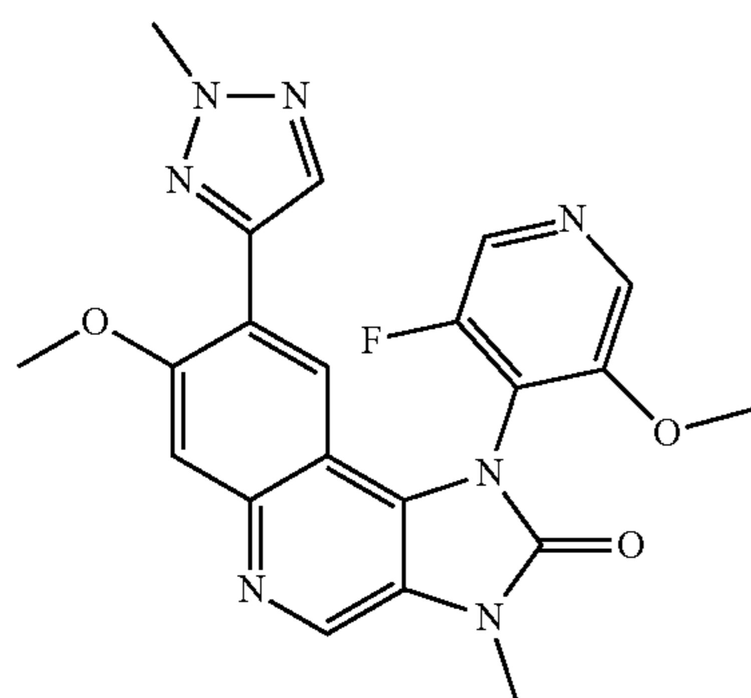
1-(3-Fluoro-5-methoxypyridin-4-yl)-7-methoxy-3-methyl-8-(2-methyl-2H-1,2,3-triazol-4-yl)-1,3-dihydroimidazo[4,5-c]quinolin-2-one
