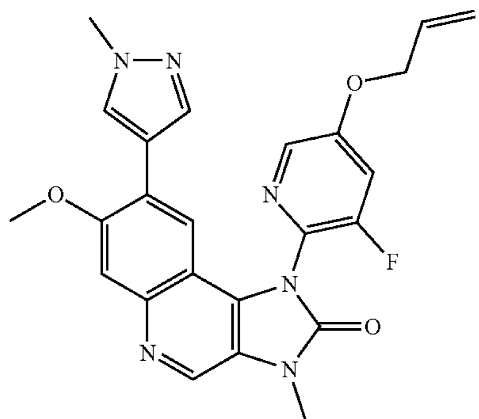
1-(5-Allyloxy-3-fluoropyridin-2-yl)-7-methoxy-3-methyl-8-(1-methyl-1H-pyrazol-4-yl)-1,3-dihydroimidazo[4,5-c]quinolin-2-one
