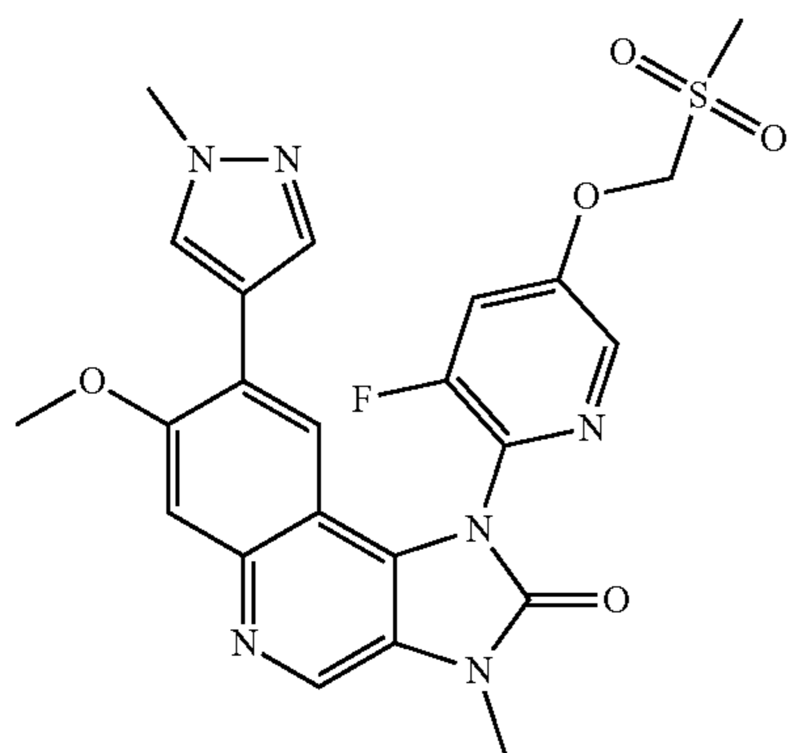
1-(3-Fluoro-5-methylsulfonylmethoxypyridin-2-yl)-7-methoxy-3-methyl-8-(1-methyl-1H-pyrazol-4-yl)-1,3-dihydroimidazo[4,5-c]quinolin-2-one
