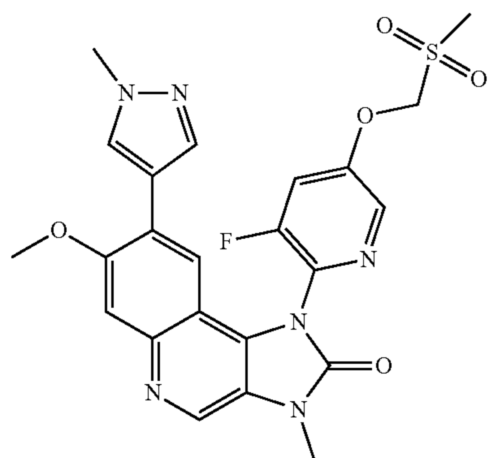
1-(3-Fluoro-5-methylsulfonylmethoxypyridin-2-yl)-7-methoxy-3-methyl-8-(1-methyl-1H-pyrazol-4-yl)-1,3-dihydroimidazo[4,5-c]quinolin-2-one
