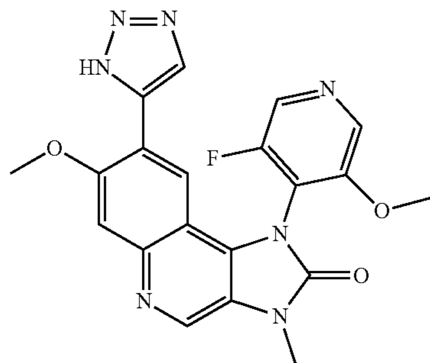
1-(3-Fluoro-5-methoxypyridin-4-yl)-7-methoxy-3-methyl-8-(3H-1,2,3-triazol-4-yl)-1,3-dihydroimidazo[4,5-c]quinolin-2-one
