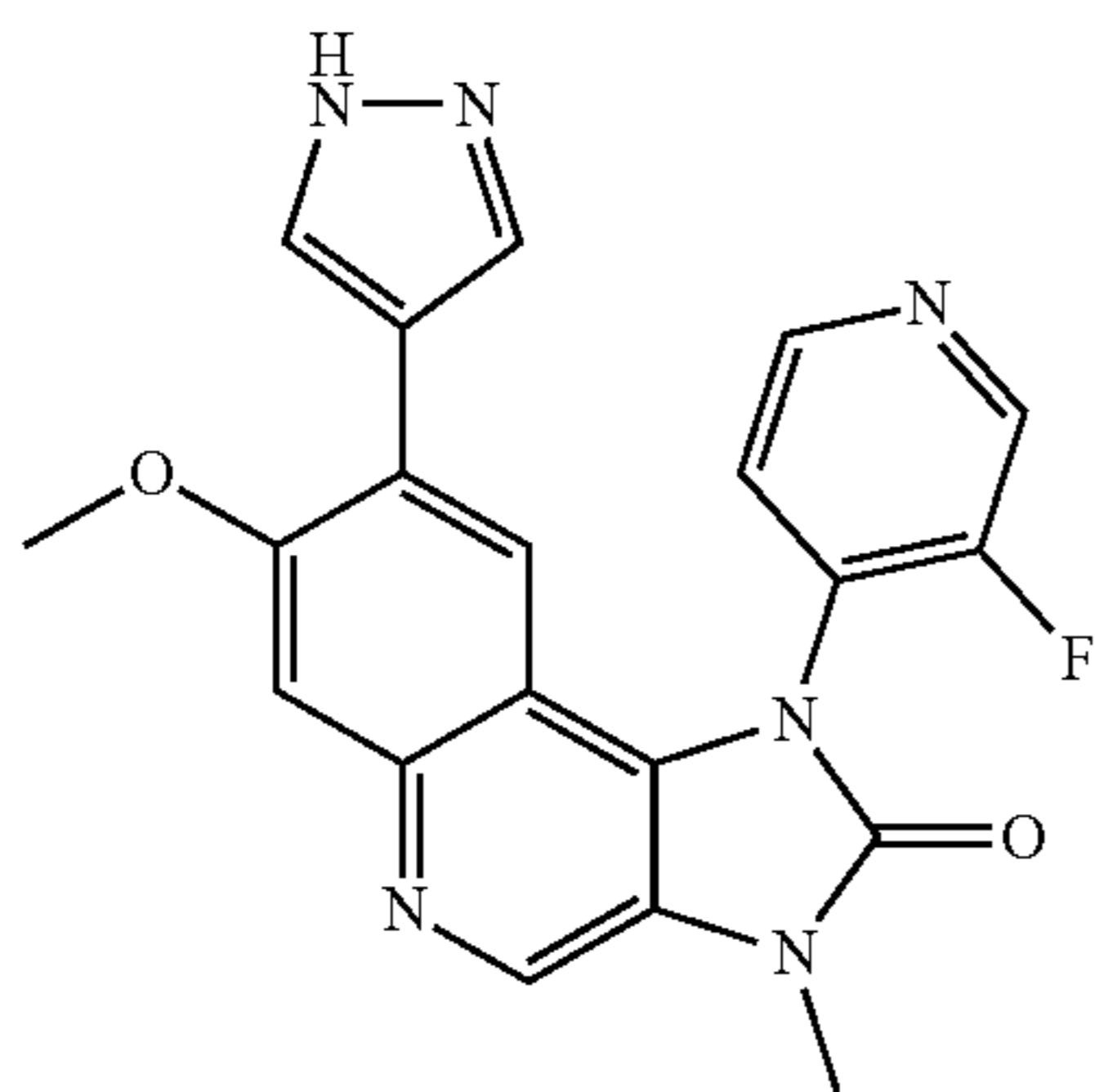
1-(3-Fluoropyridin-4-yl)-7-methoxy-3-methyl-8-(1H-pyrazol-4-yl)-1,3-dihydroimidazo[4,5-c]quinolin-2-one
