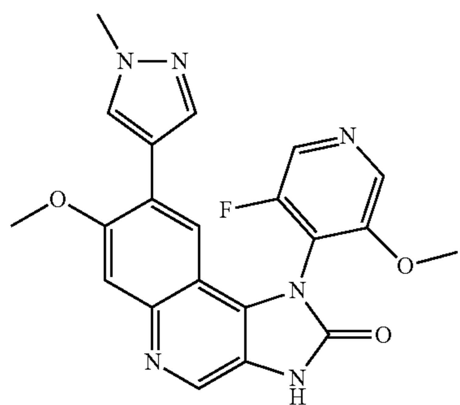
1-(3-Fluoro-5-methoxypyridin-4-yl)-7-methoxy-8-(1-methyl-1H-pyrazol-4-yl)-1,3-dihydroimidazo[4,5-c]quinolin-2-one
