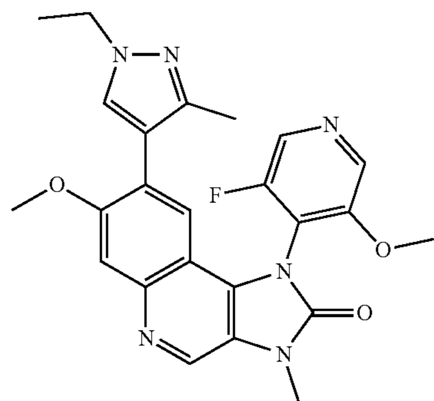
8-(1-Ethyl-3-methyl-1H-pyrazol-4-yl)-1-(3-fluoro-5-methoxy-pyridin-4-yl)-7-methoxy-3-methyl-1,3-dihydroimidazo[4,5-c]quinolin-2-one
