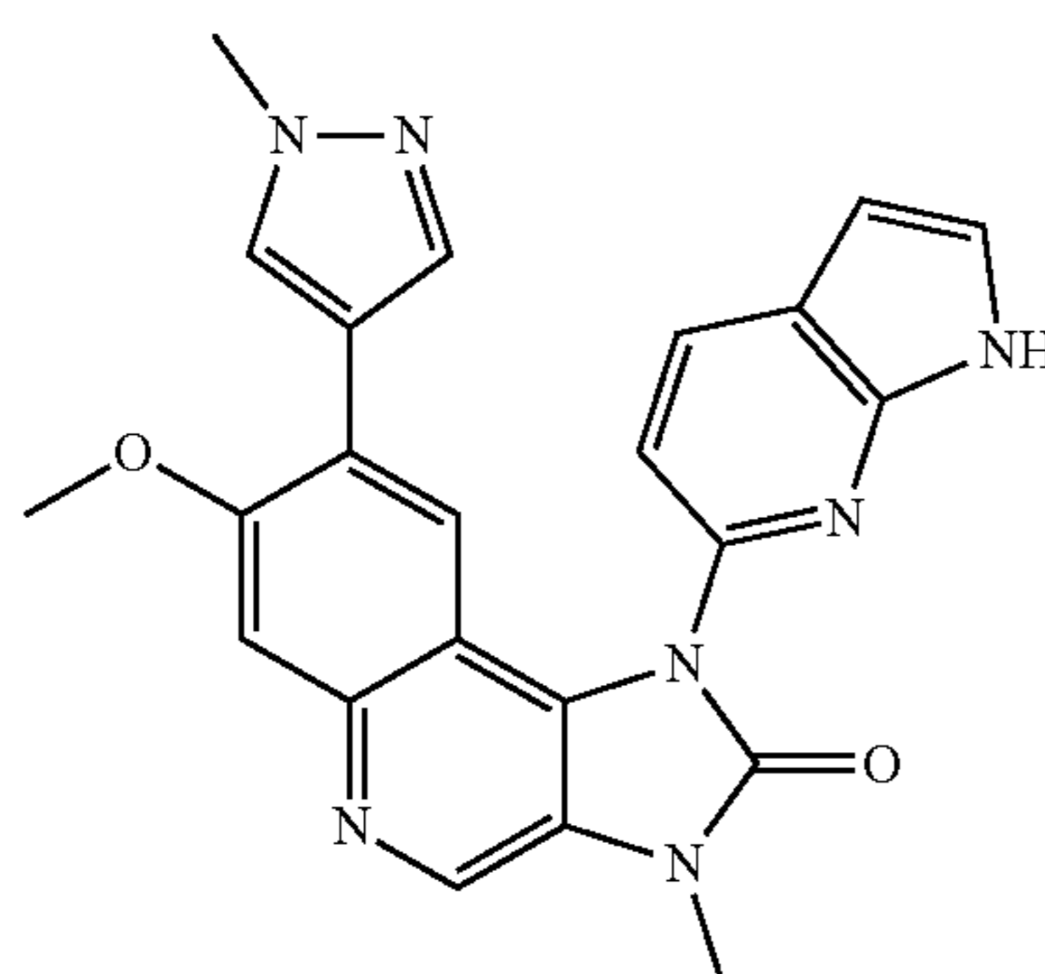
7-Methoxy-3-methyl-8-(1-methyl-1H-pyrazol-4-yl)-1-(1H-pyrrolo[2,3-b]pyridin-6-yl)-1,3-dihydroimidazo[4,5-c]quinolin-2-one
