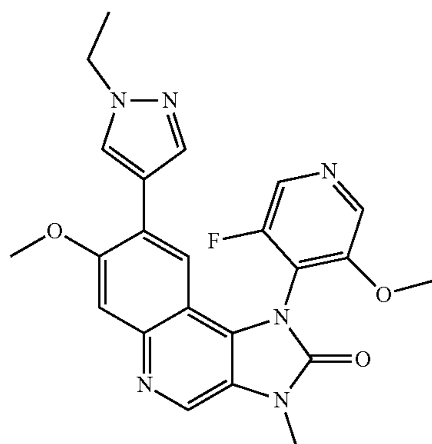
8-(1-Ethyl-1H-pyrazol-4-yl)-1-(3-fluoro-5-methoxypyridin-4-yl)-7-methoxy-3-methyl-1,3-dihydroimidazo[4,5-c]quinolin-2-one
