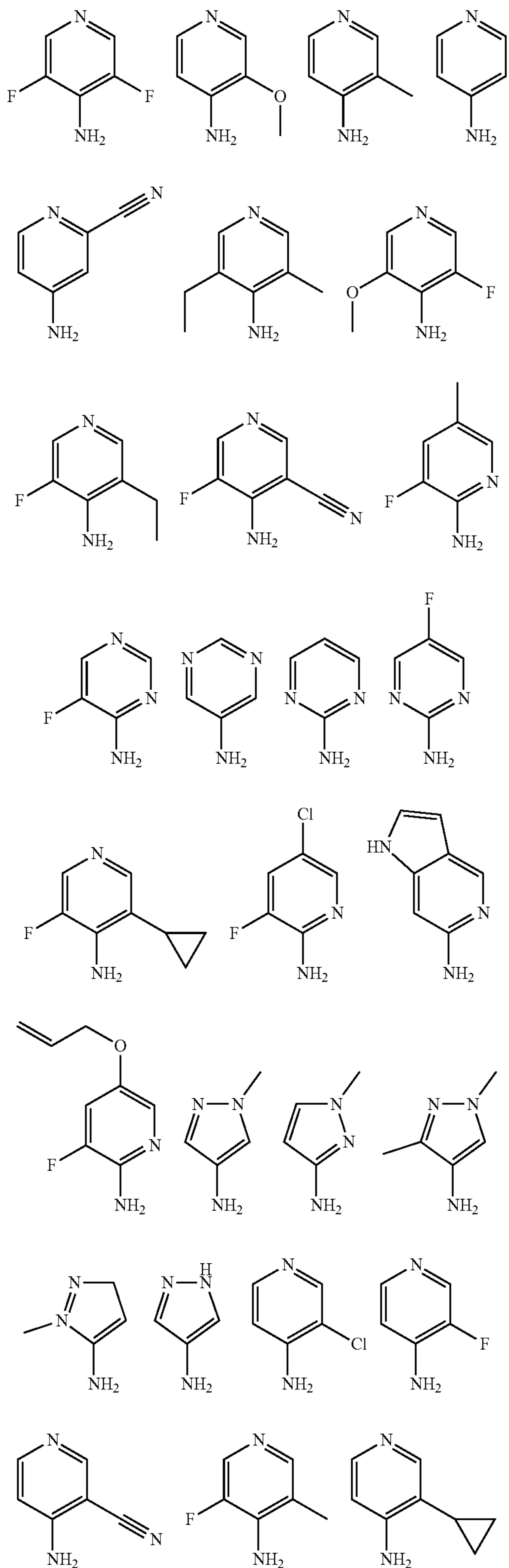
Schema 4: Amine derivatives, boronic acid esters or analogues
