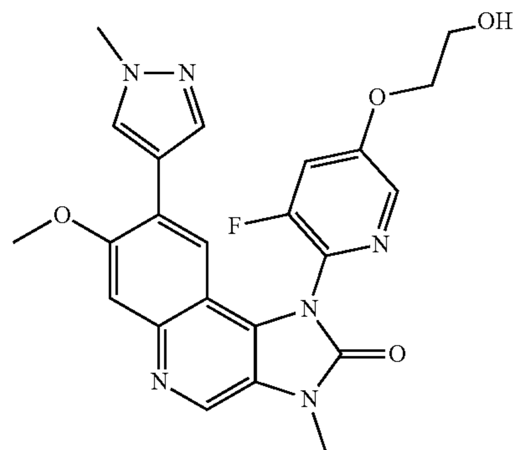
1-[3-Fluoro-5-(2-hydroxyethoxy)-2-pyridyl]-7-methoxy-3-methyl-8-(1-methylpyrazol-4-yl)imidazo[4,5-c]quinolin-2-one
