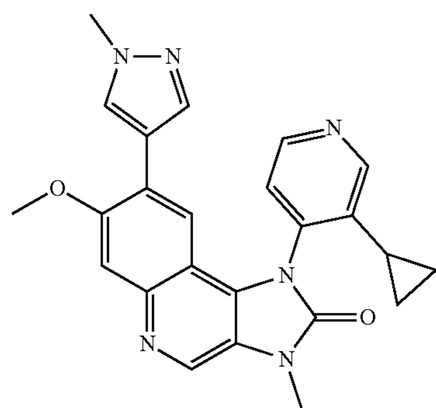
1-(3-Cyclopropylpyridin-4-yl)-7-methoxy-3-methyl-8-(1-methyl-1H-pyrazol-4-yl)-1,3-dihydroimidazo[4,5-c]quinolin-2-one
