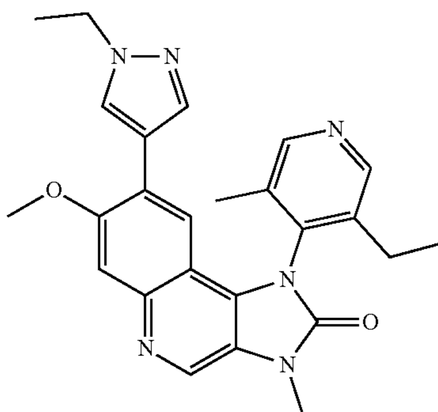
1-(3-Ethyl-5-methylpyridin-4-yl)-8-(1-ethyl-1H-pyrazol-4-yl)-7-methoxy-3-methyl-1,3-dihydroimidazo[4,5-c]quinolin-2-one
