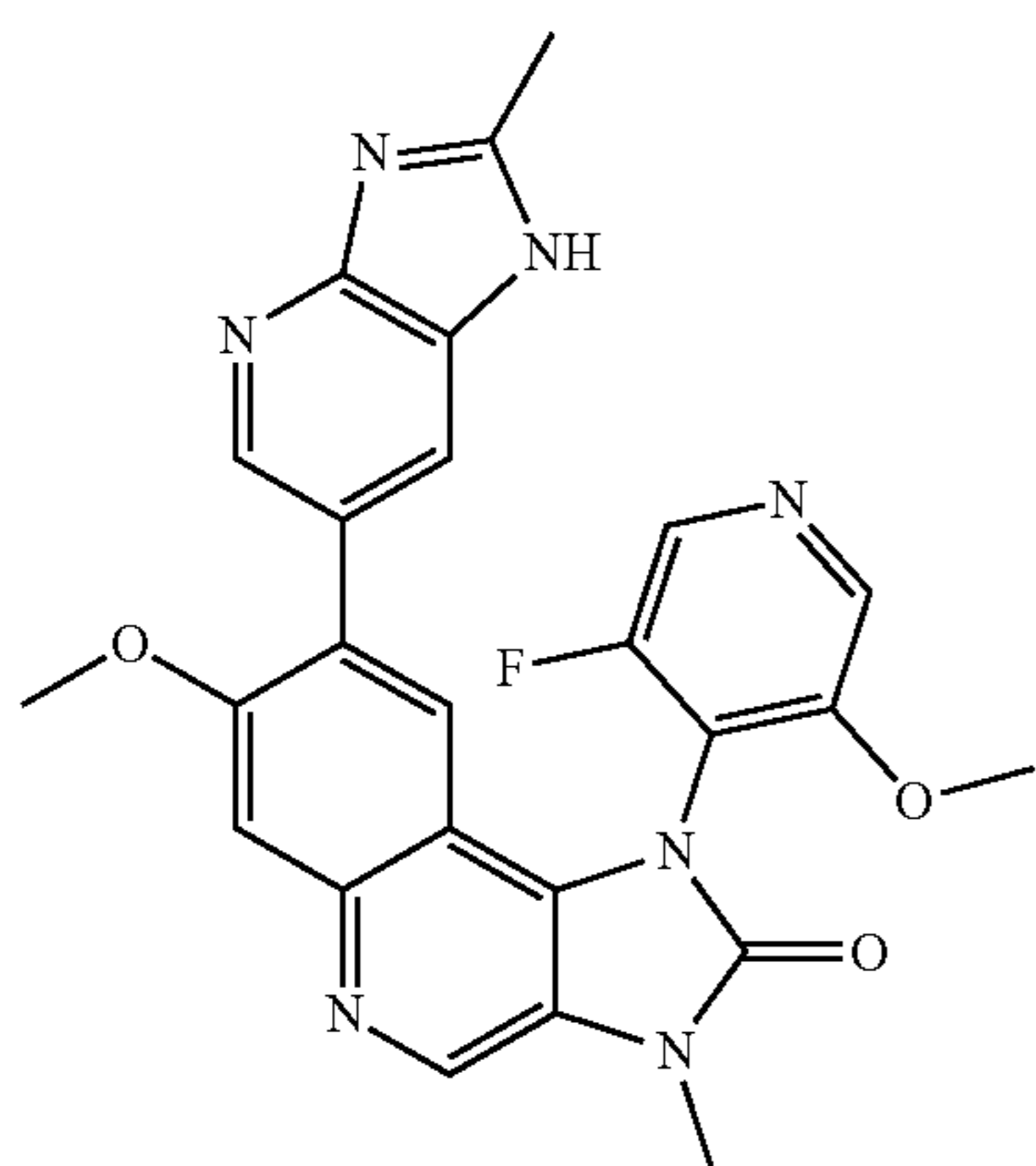
1-(3-Fluoro-5-methoxypyridin-4-yl)-7-methoxy-3-methyl-8-(2-methyl-1H-imidazo[4,5-b]pyridin-6-yl)-1,3-dihydroimidazo[4,5-c]quinolin-2-one
