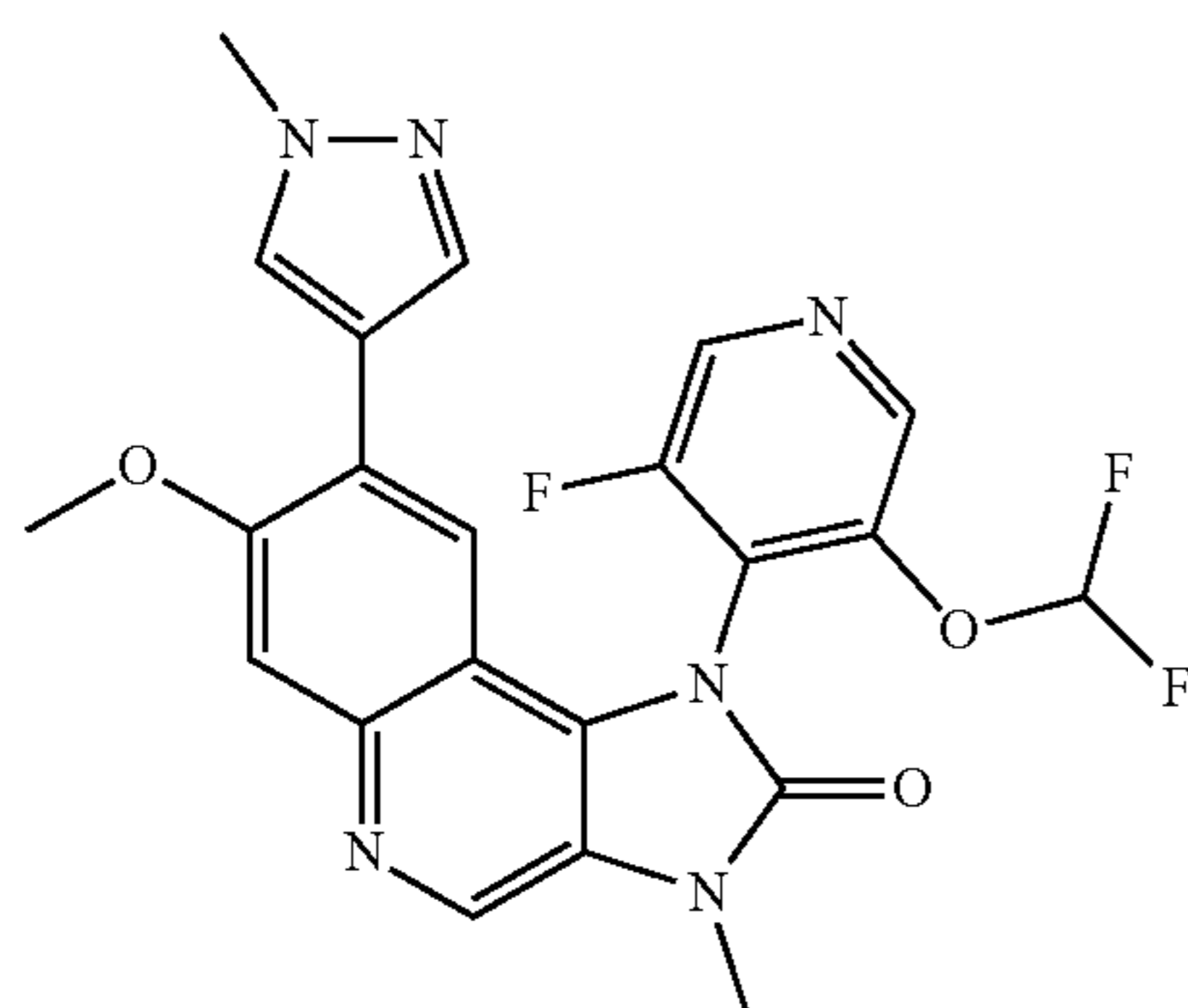
1-(3-Difluoromethoxy-5-fluoropyridin-4-yl)-7-methoxy-3-methyl-8-(1-methyl-1H-pyrazol-4-yl)-1,3-dihydroimidazo[4,5-c]quinolin-2-one
