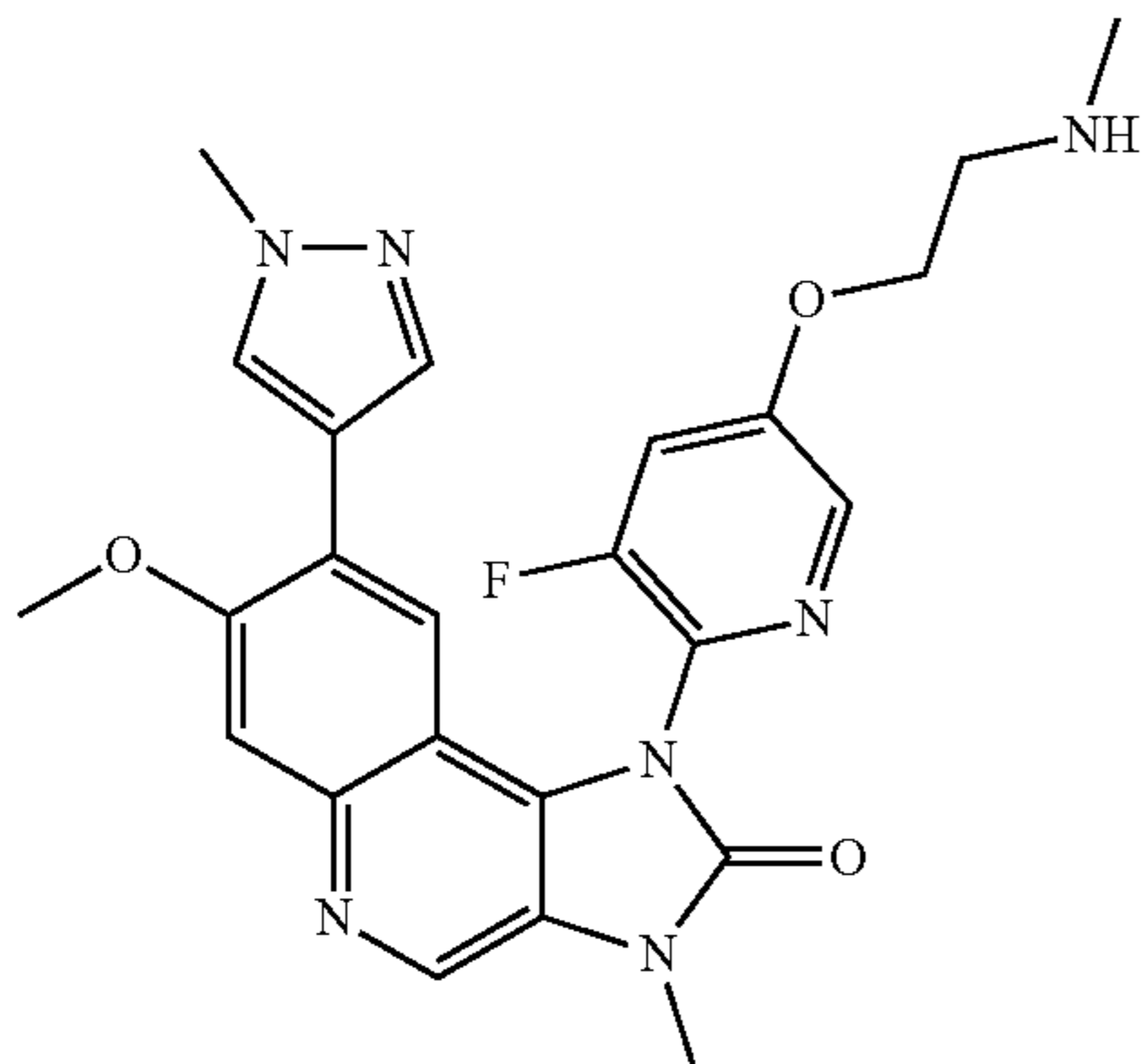
1-[3-Fluoro-5-(2-methylamino-ethoxy)pyridin-2-yl]-7-methoxy-3-methyl-8-(1-methyl-1H-pyrazol-4-yl)-1,3-dihydroimidazo[4,5-c]quinolin-2-one
