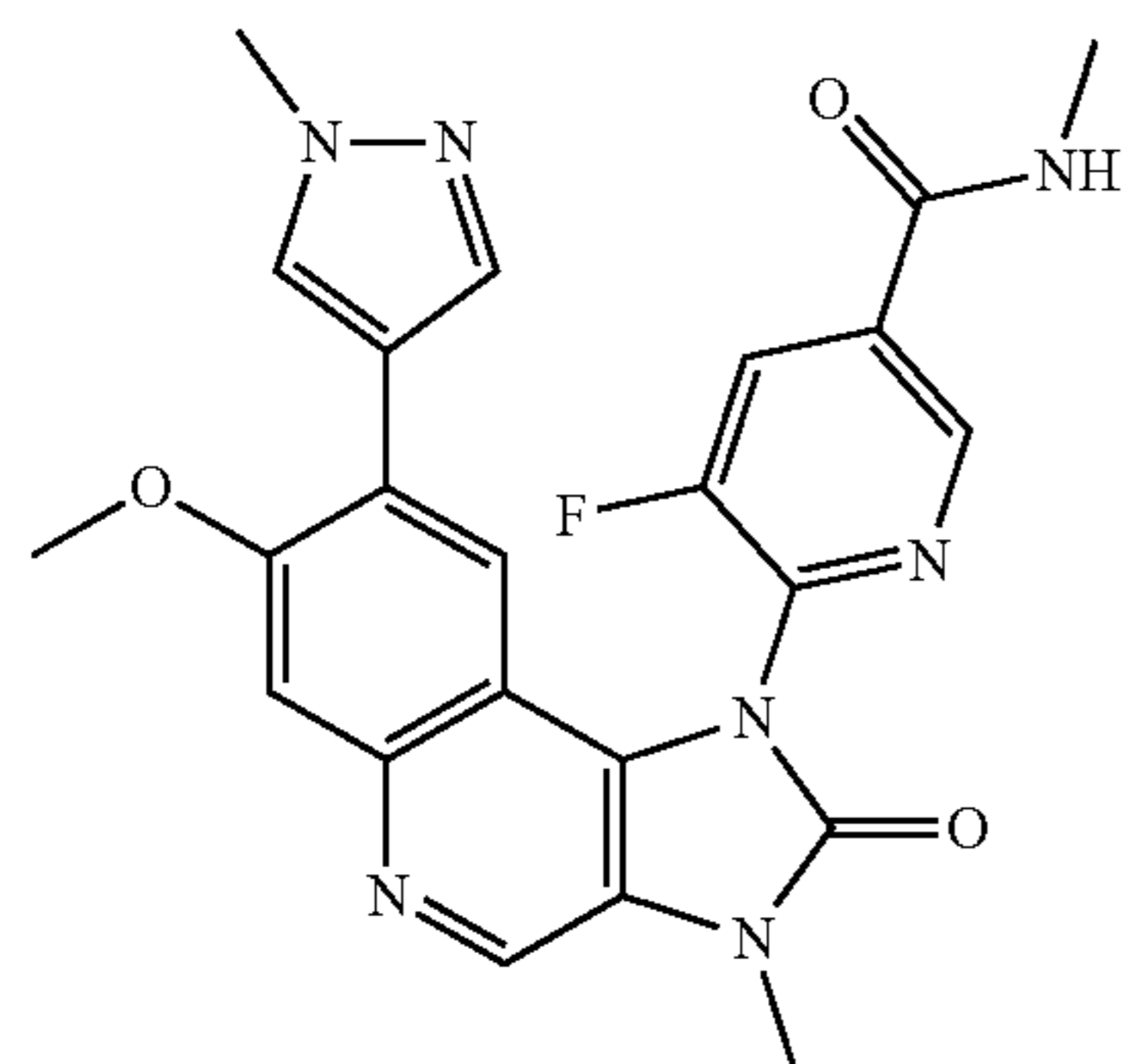
5-Fluoro-6-[7-methoxy-3-methyl-8-(1-methyl-1H-pyrazol-4-yl)-2-oxo-2,3-dihydroimidazo[4,5-c]quinolin-1-yl]-N-methylnicotinamide
