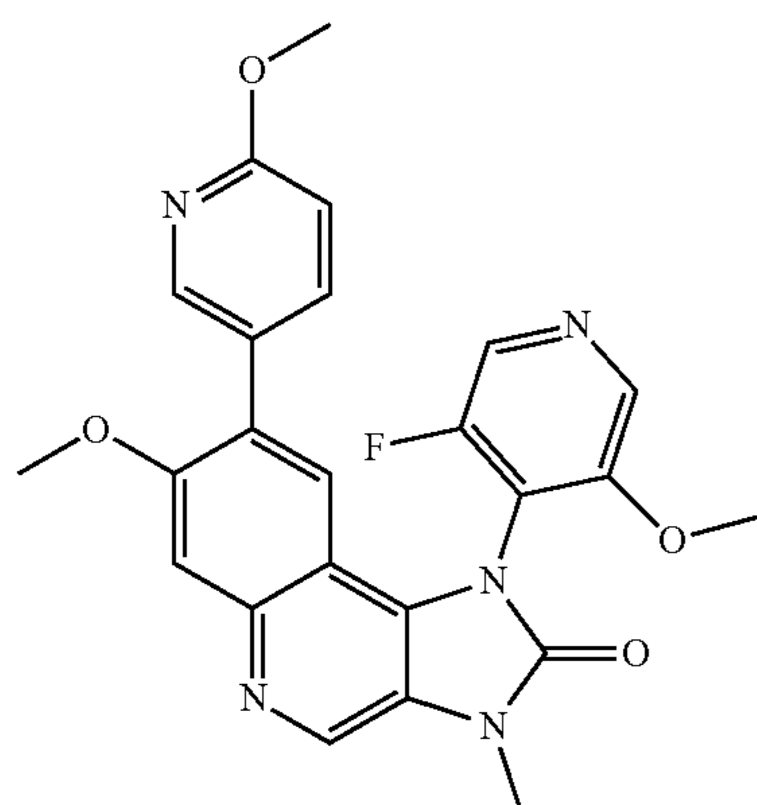
1-(3-Fluoro-5-methoxypyridin-4-yl)-7-methoxy-8-(6-methoxypyridin-3-yl)-3-methyl-1,3-dihydroimidazo[4,5-c]quinolin-2-one
