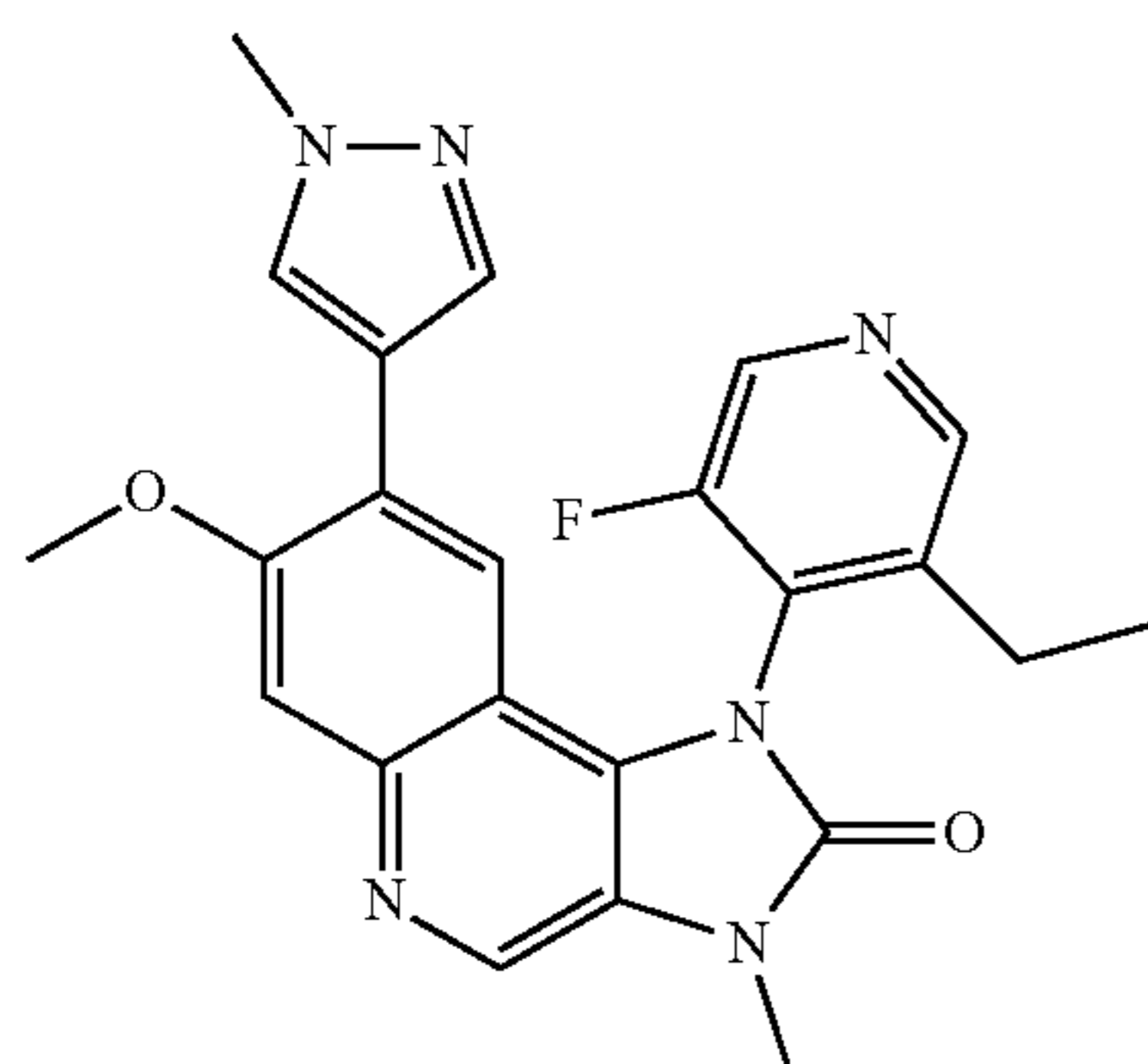
1-(3-Ethyl-5-fluoropyridin-4-yl)-7-methoxy-3-methyl-8-(1-methyl-1H-pyrazol-4-yl)-1,3-dihydroimidazo[4,5-c]quinolin-2-one
