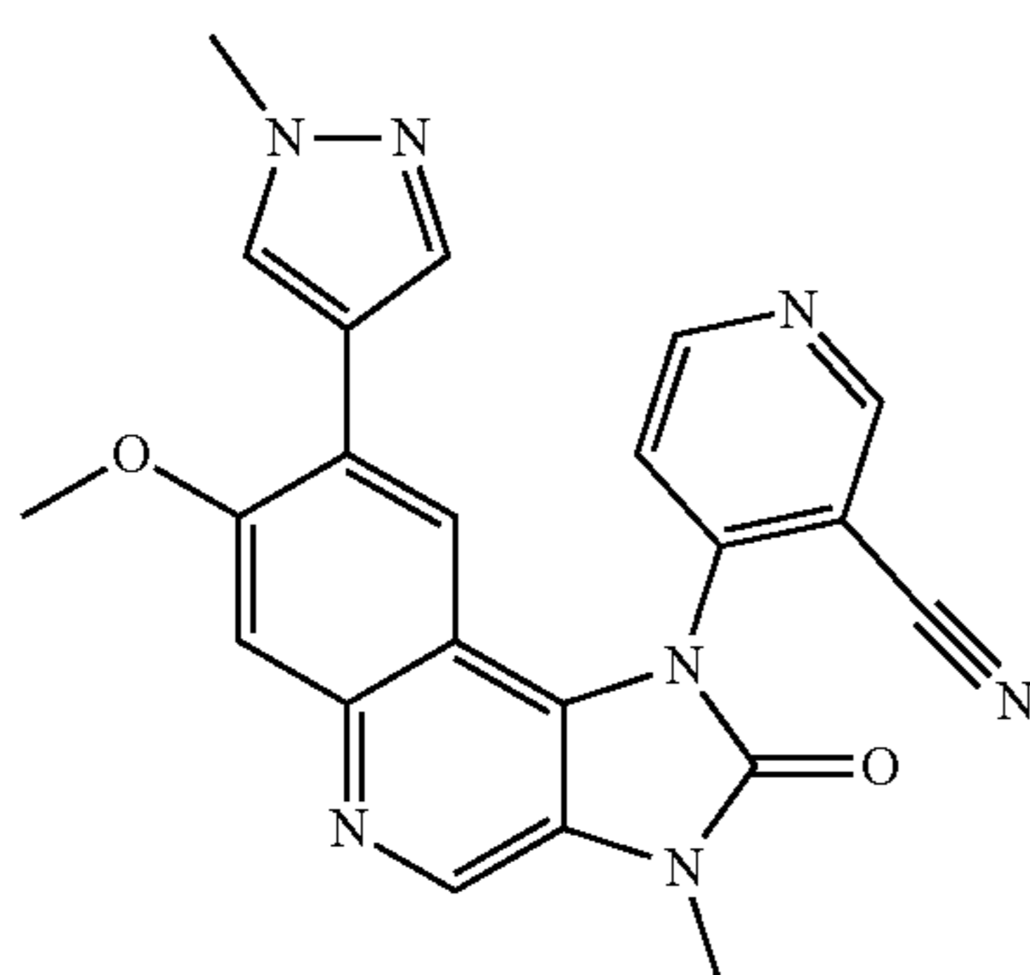
4-[7-Methoxy-3-methyl-8-(1-methyl-1H-pyrazol-4-yl)-2-oxo-2,3-dihydroimidazo[4,5-c]quinolin-1-yl]nicotinonitrile
