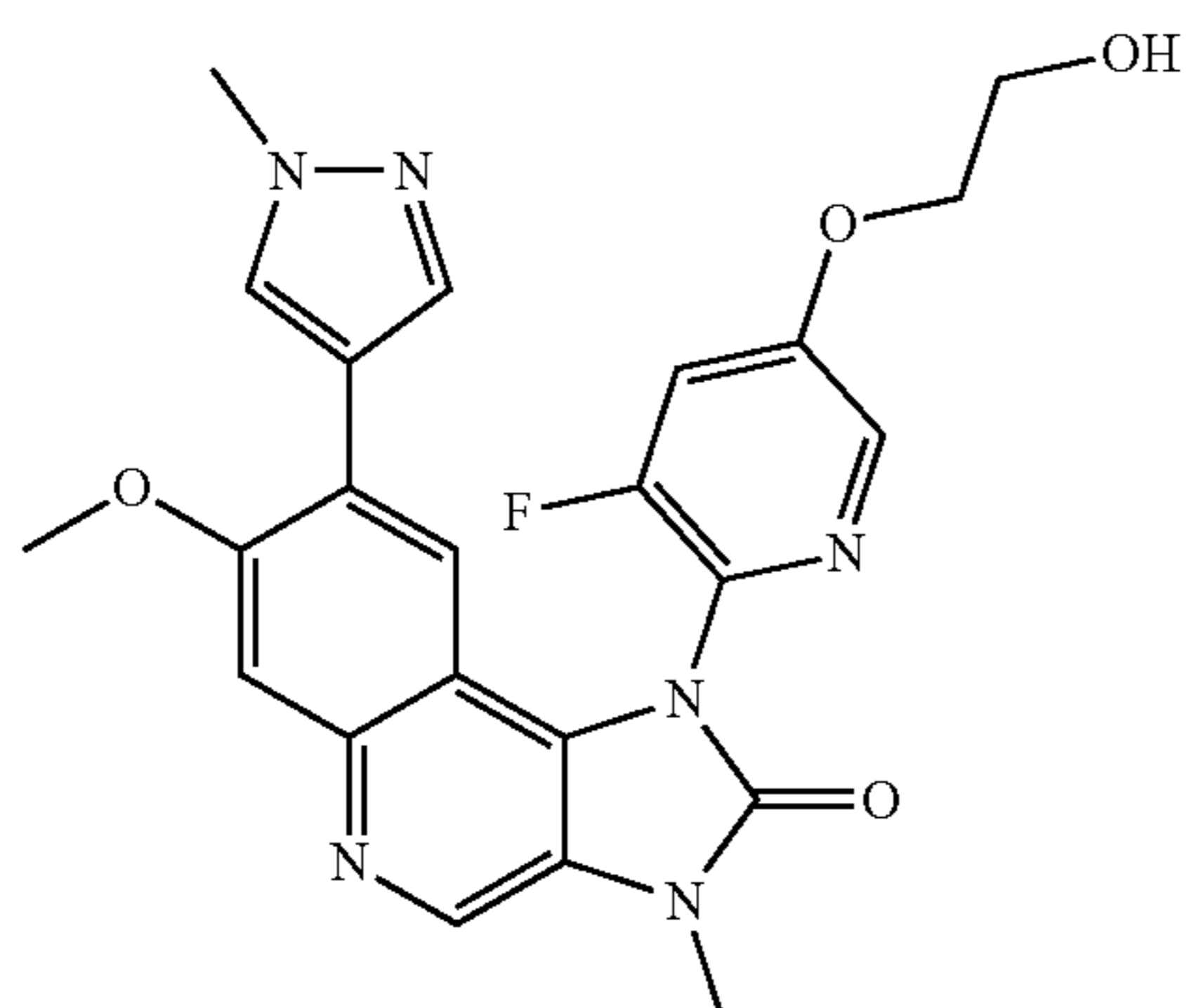
1-[3-Fluoro-5-(2-hydroxyethoxy)-2-pyridyl]-7-methoxy-3-methyl-8-(1-methylpyrazol-4-yl)imidazo[4,5-c]quinolin-2-one
