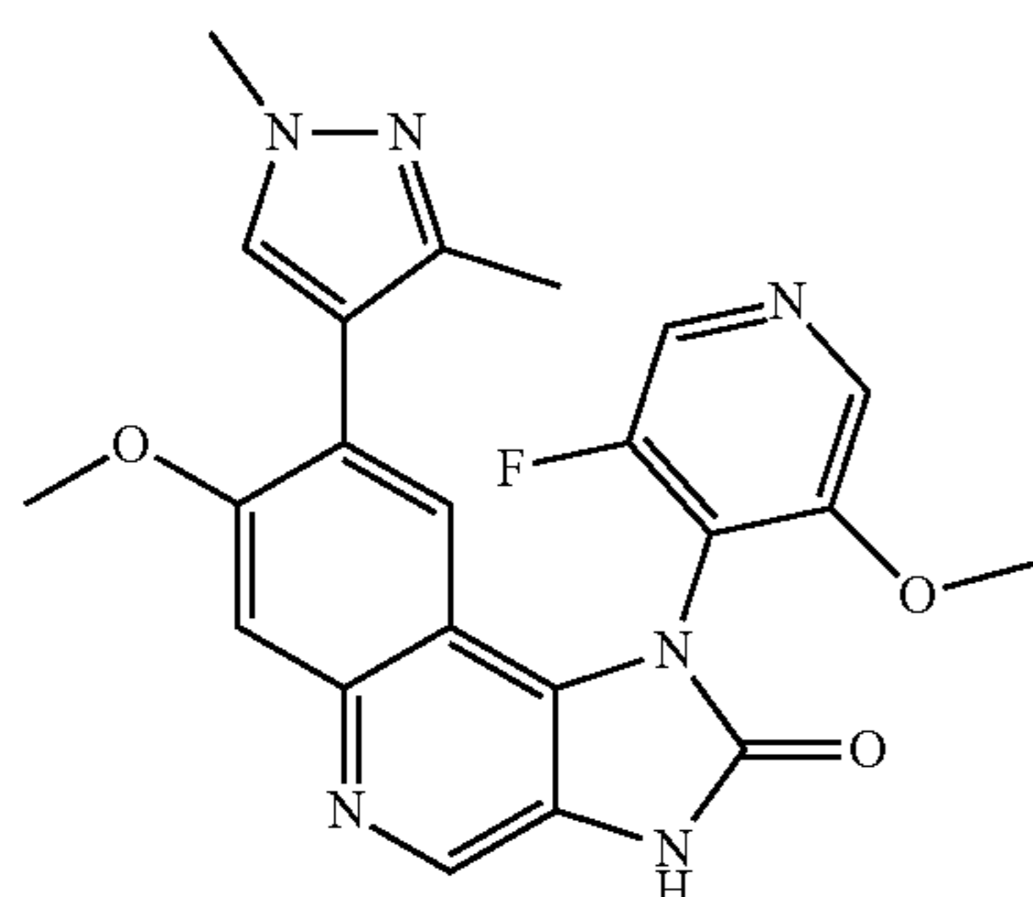
8-(1,3-Dimethyl-1H-pyrazol-4-yl)-1-(3-fluoro-5-methoxypyridin-4-yl)-7-methoxy-1,3-dihydroimidazo[4,5-c]quinolin-2-one
