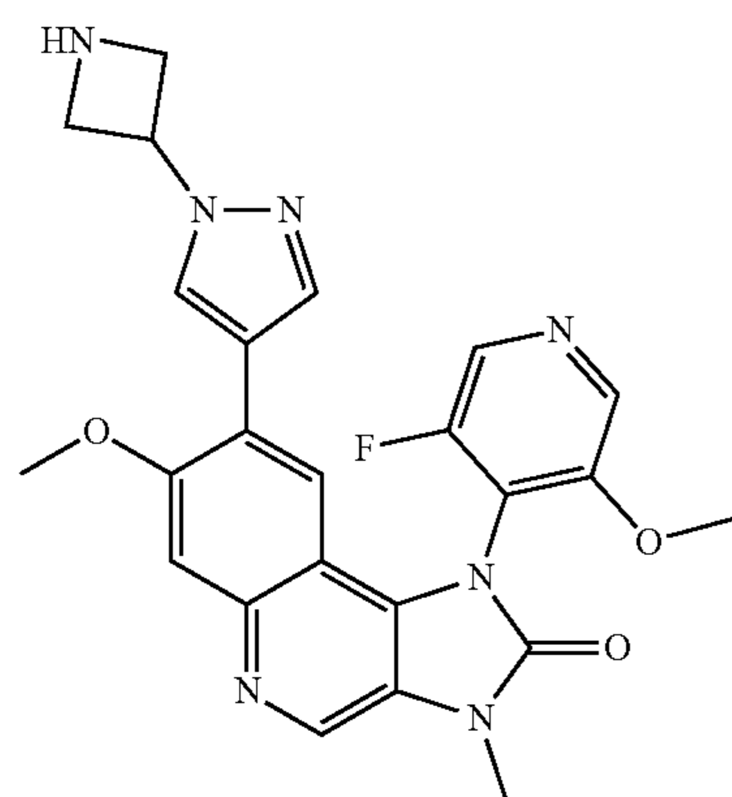
8-[1-(Azetidin-3-yl)-1H-pyrazol-4-yl]-1-(3-fluoro-5-methoxy-pyridin-4-yl)-7-methoxy-3-methyl-1H,2H,3H-imidazo[4,5-c]quinolin-2-one
