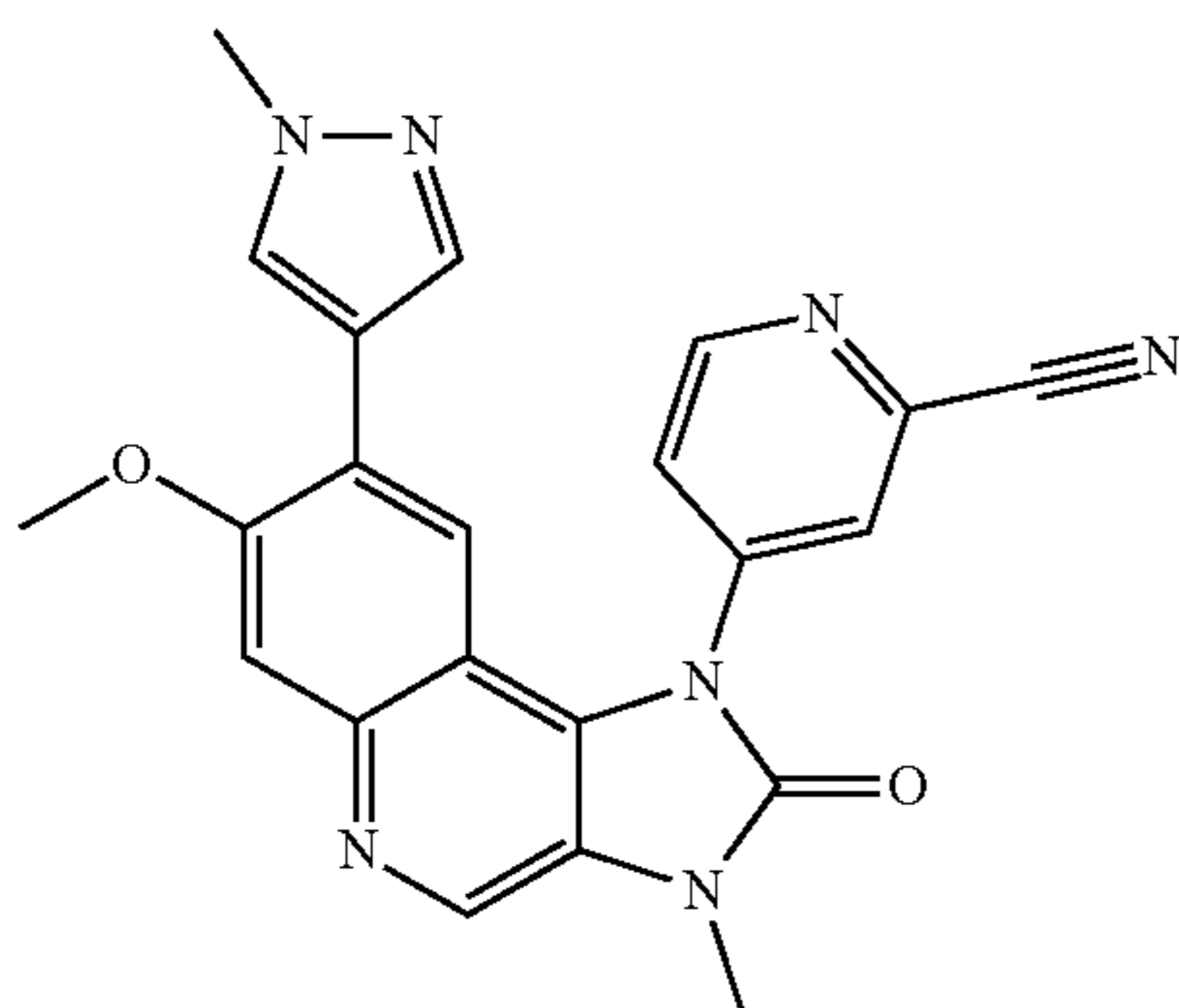
4-[7-Methoxy-3-methyl-8-(1-methyl-1H-pyrazol-4-yl)-2-oxo-2,3-dihydroimidazo[4,5-c]quinolin-1-yl]pyridine-2-carbonitrile
