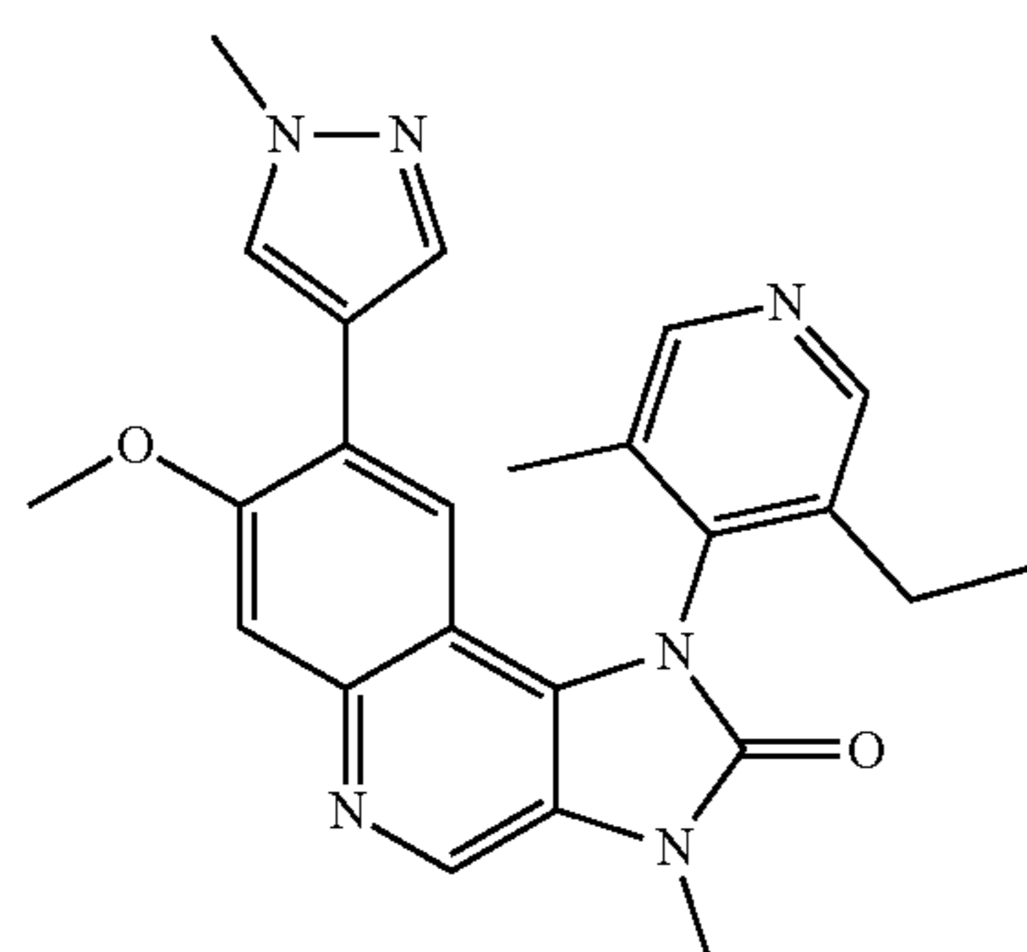
1-(3-Ethyl-5-methylpyridin-4-yl)-7-methoxy-3-methyl-8-(1-methyl-1H-pyrazol-4-yl)-1,3-dihydroimidazo[4,5-c]quinolin-2-one
