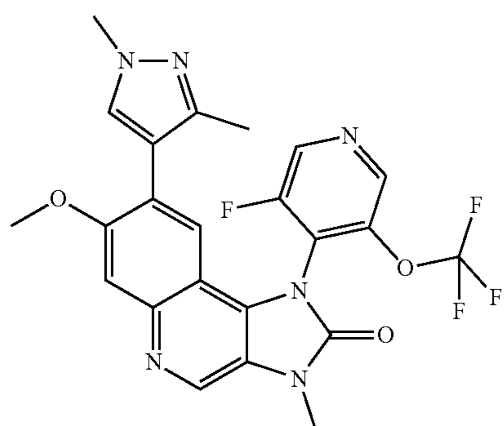
1-[3-Fluoro-5-(trifluoromethoxy)-4-pyridyl]-7-methoxy-3-methyl-8-(1,3-dimethylpyrazol-4-yl)-1,3-dihydroimidazo[4,5-c]quinolin-2-one
