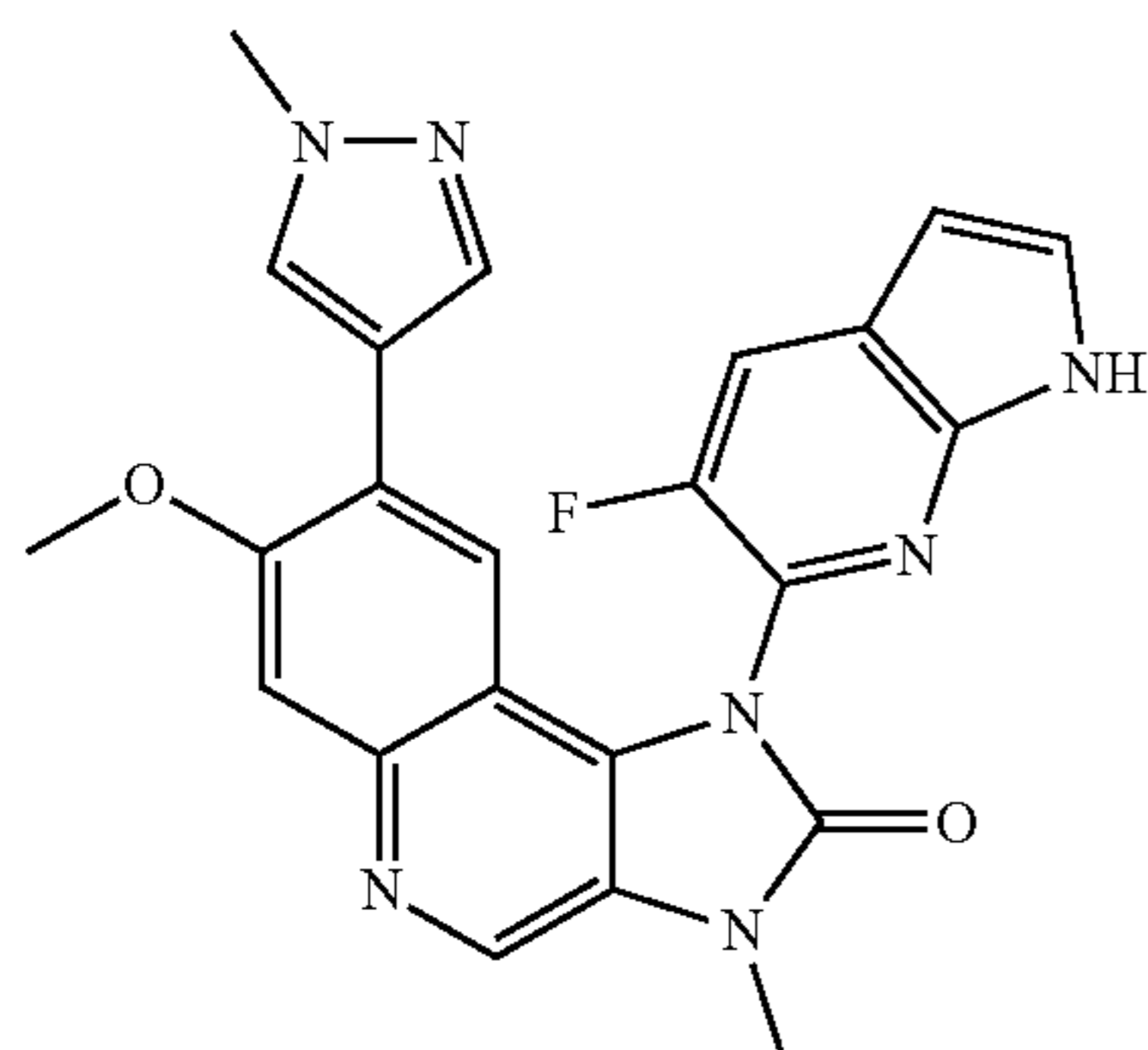
1-(5-Fluoro-1H-pyrrolo[2,3-b]pyridin-6-yl)-7-methoxy-3-methyl-8-(1-methyl-1H-pyrazol-4-yl)-1,3-dihydroimidazo[4,5-c]quinolin-2-one
