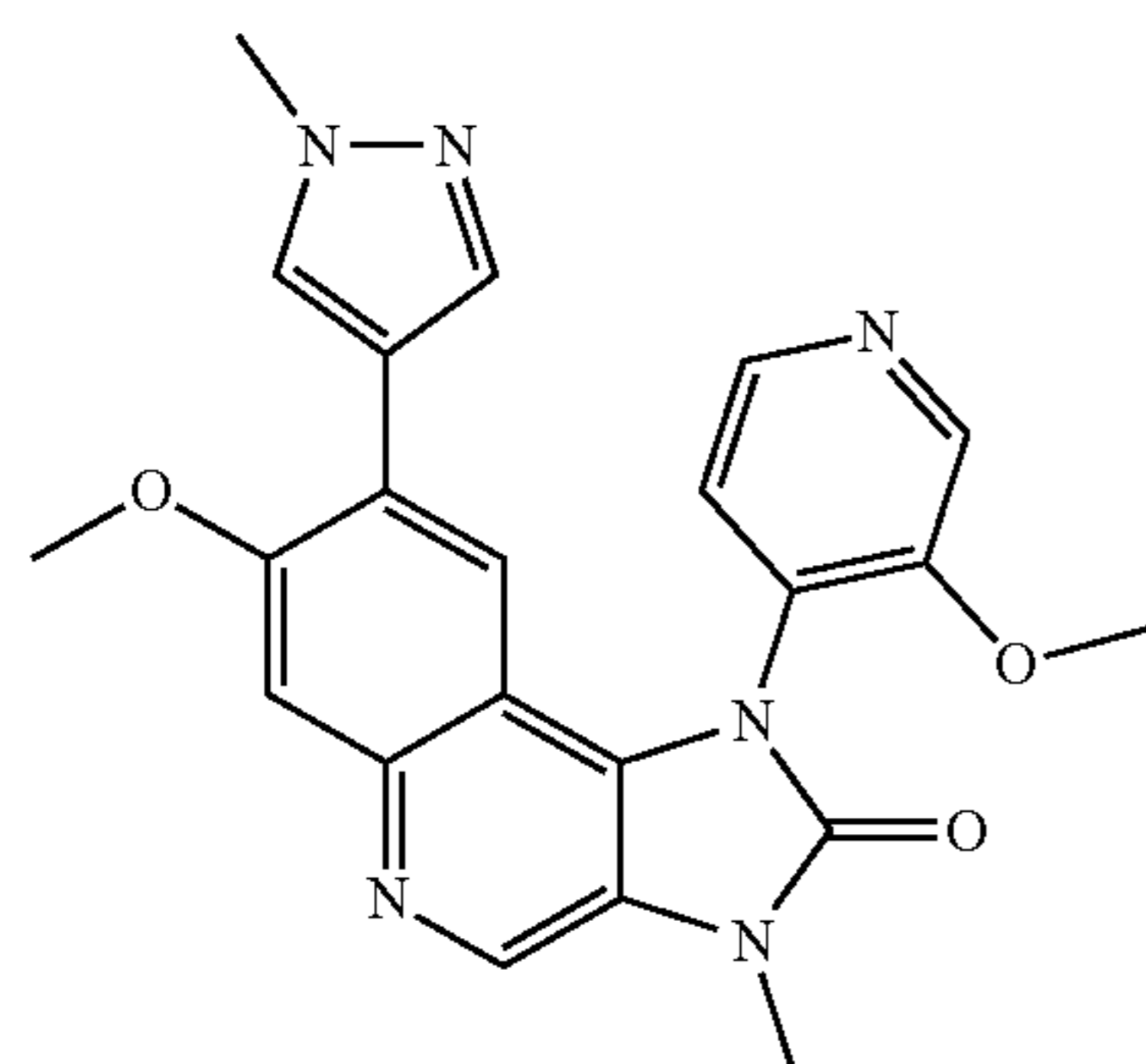
7-Methoxy-1-(3-methoxypyridin-4-yl)-3-methyl-8-(1-methyl-1H-pyrazol-4-yl)-1,3-dihydroimidazo[4,5-c]quinolin-2-one
