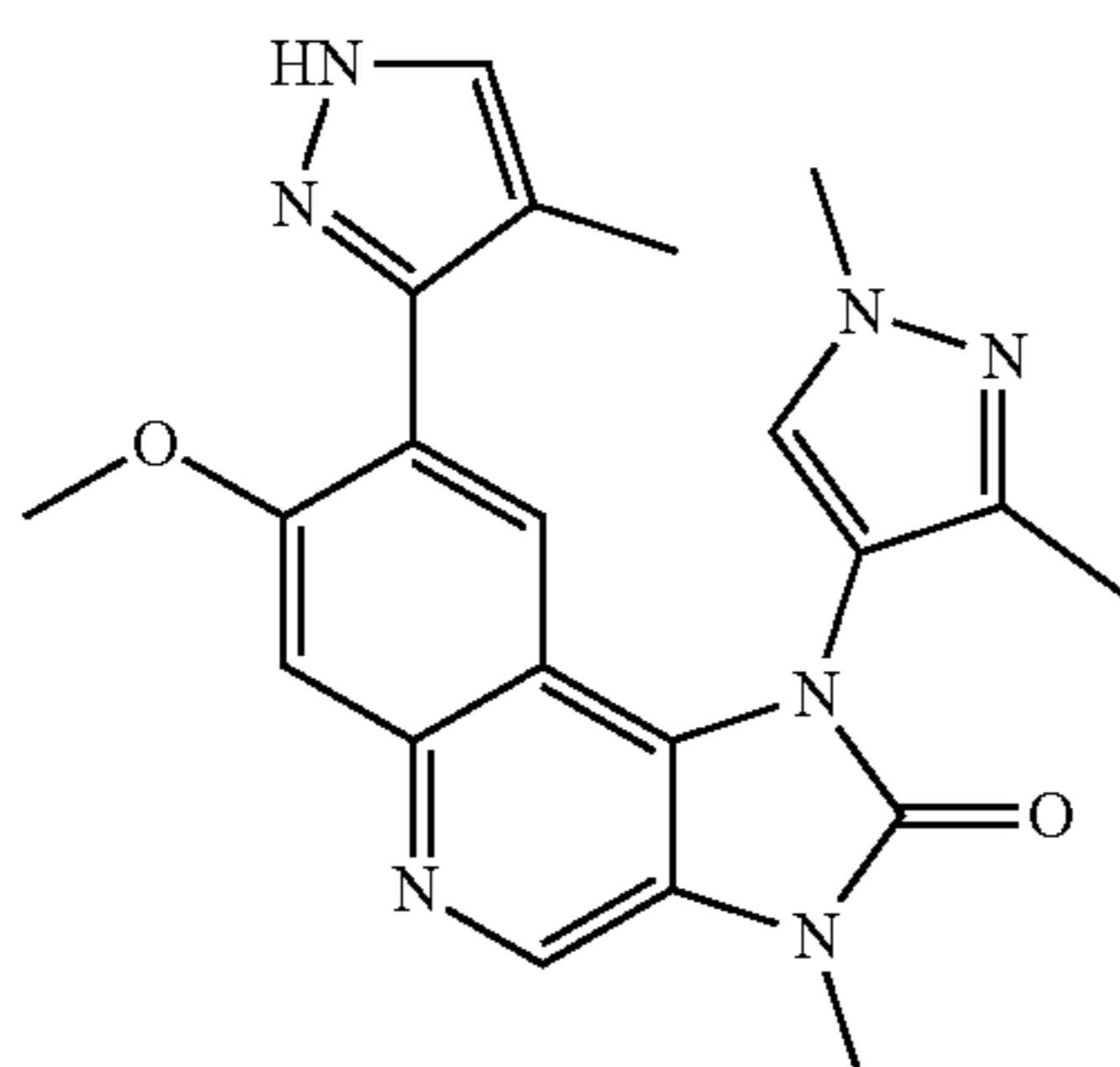
1-(1,3-Dimethyl-1H-pyrazol-4-yl)-7-methoxy-3-methyl-8-(4-methyl-1H-pyrazol-3-yl)-1,3-dihydroimidazo[4,5-c]quinolin-2-one
