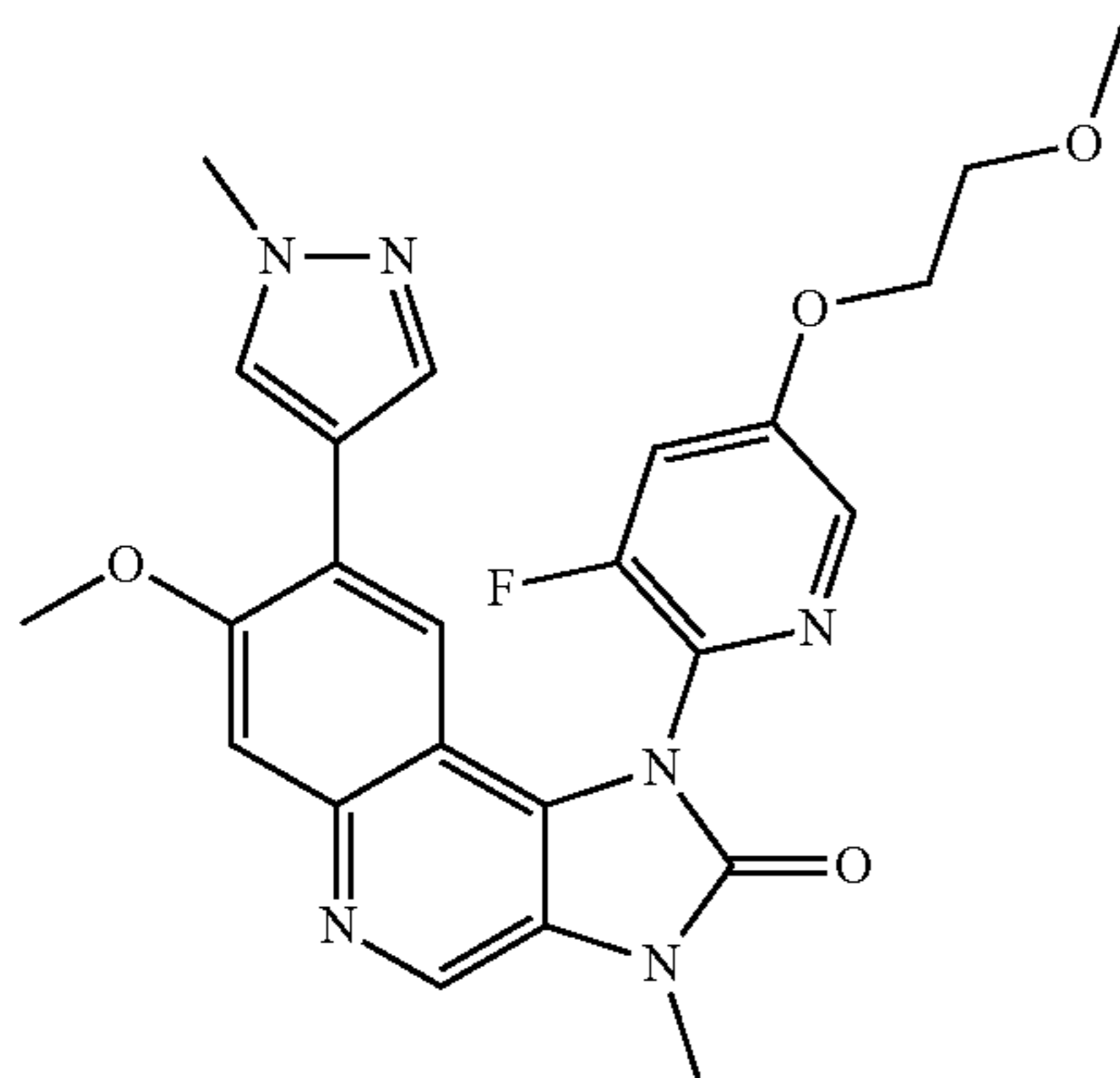
1-[3-Fluoro-5-(2-methoxyethoxy)-2-pyridyl]-7-methoxy-3-methyl-8-(1-methylpyrazol-4-yl)imidazo[4,5-c]quinolin-2-one
