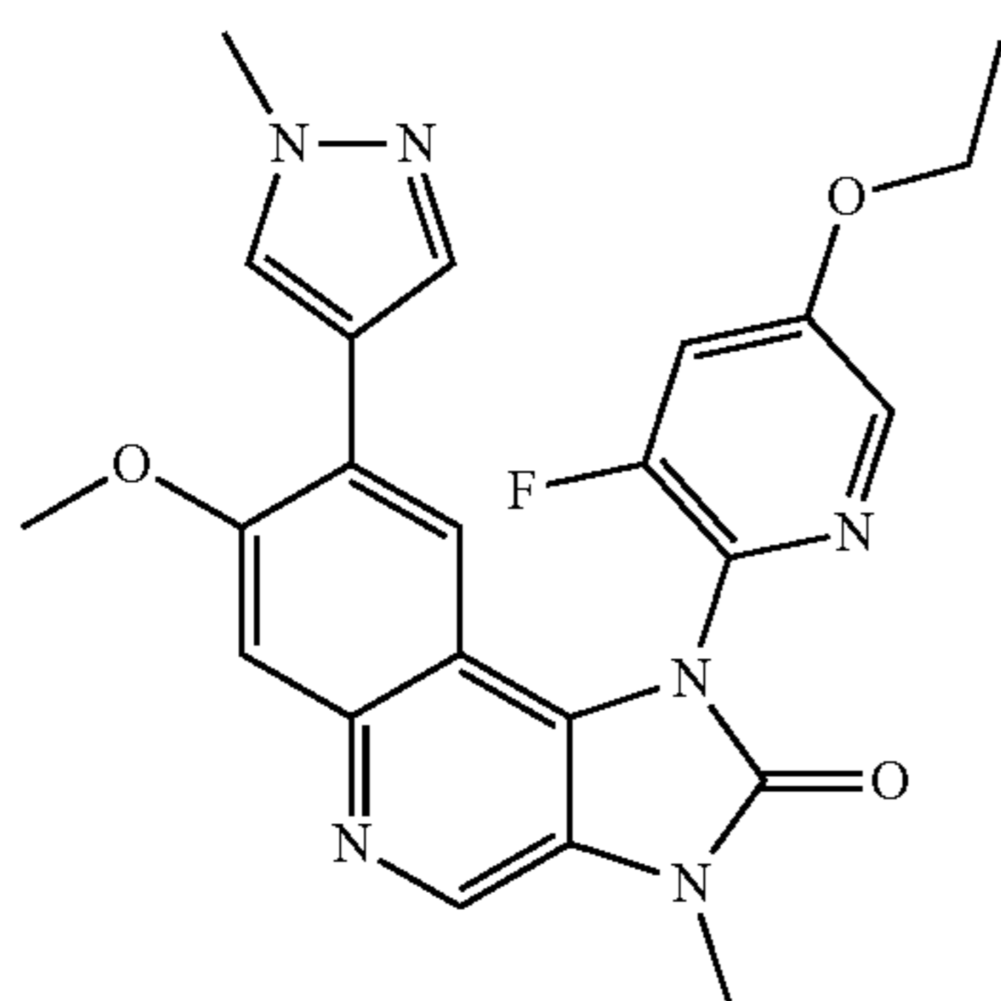
1-(5-Ethoxy-3-fluoropyridin-2-yl)-7-methoxy-3-methyl-8-(1-methyl-1H-pyrazol-4-yl)-1,3-dihydroimidazo[4,5-c]quinolin-2-one
