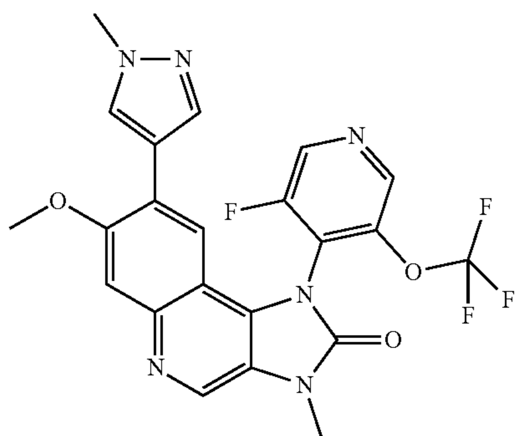
1-[3-Fluoro-5-(trifluoromethoxy)-4-pyridyl]-7-methoxy-3-methyl-8-(1-methyl-1H-pyrazol-4-yl)-1,3-dihydroimidazo[4,5-c]quinolin-2-one
