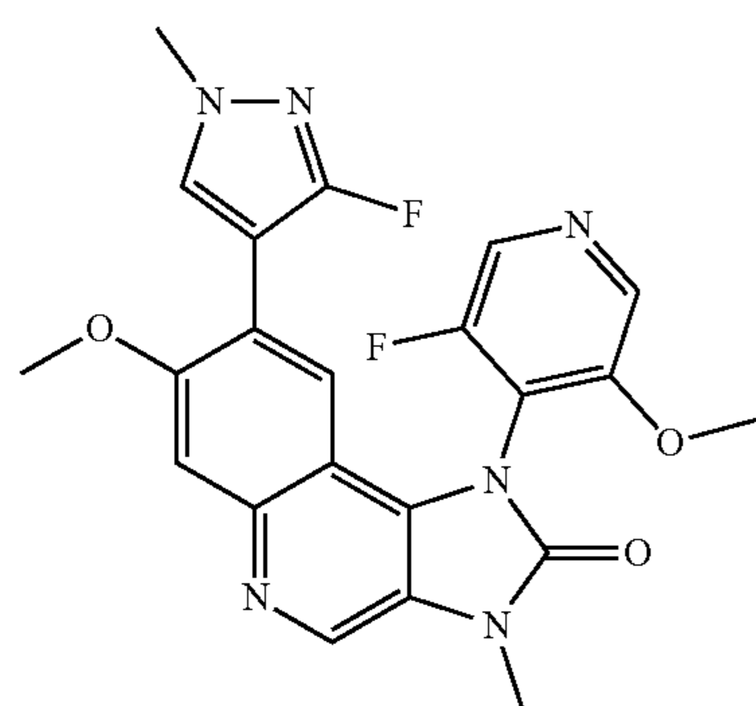
1-(3-Fluoro-5-methoxypyridin-4-yl)-7-methoxy-3-methyl-8-(3-fluoro-1-methyl-1H-pyrazol-4-yl)-1,3-dihydroimidazo[4,5-c]quinolin-2-one
