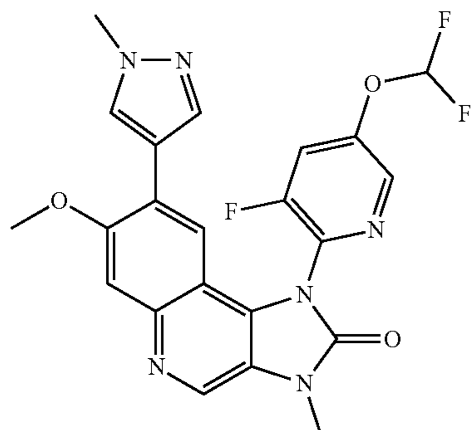
1-(5-Difluoromethoxy-3-fluoropyridin-2-yl)-7-methoxy-3-methyl-8-(1-methyl-1H-pyrazol-4-yl)-1,3-dihydroimidazo[4,5-c]quinolin-2-one
