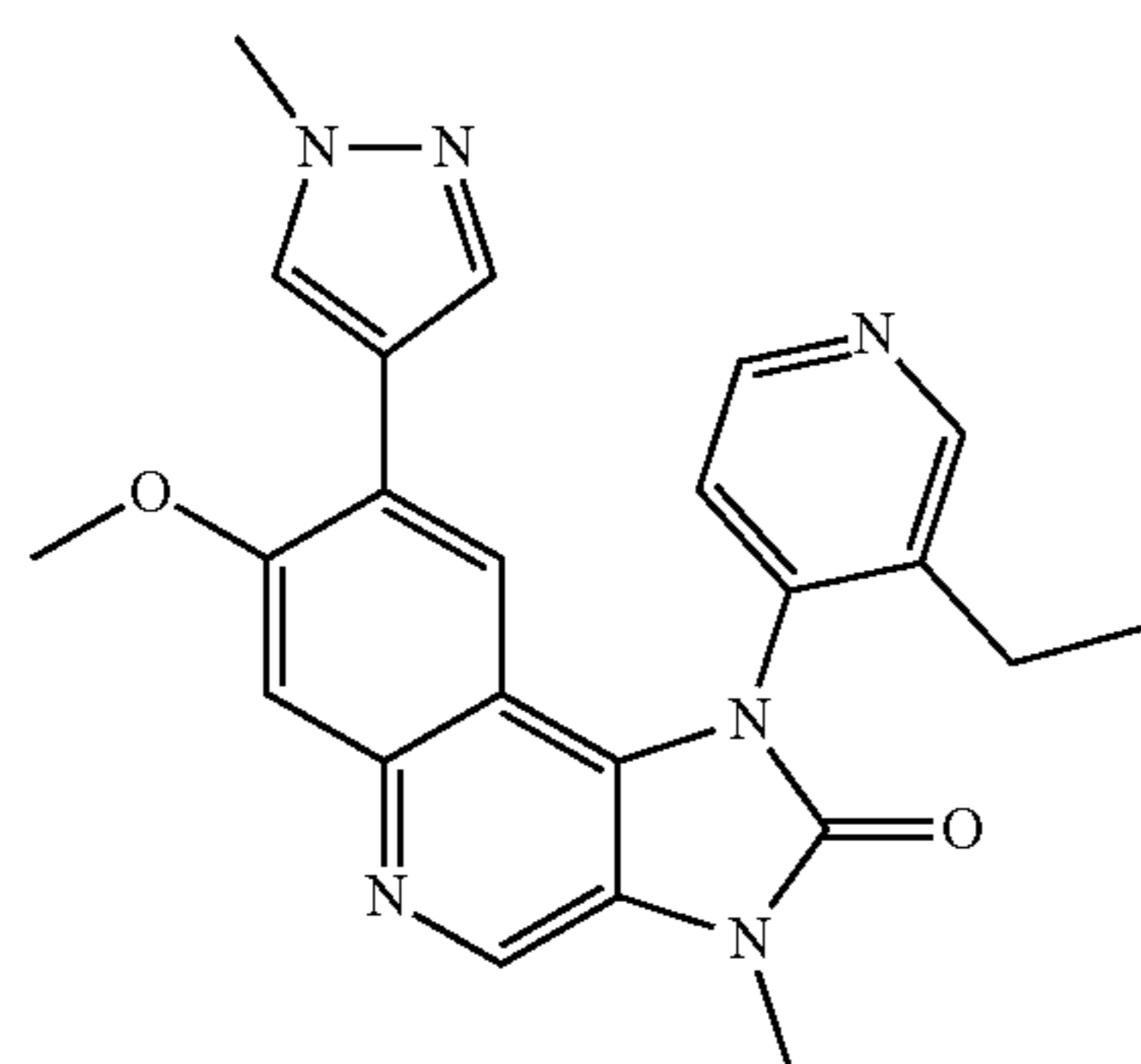
1-(3-Ethylpyridin-4-yl)-7-methoxy-3-methyl-8-(1-methyl-1H-pyrazol-4-yl)-1,3-dihydroimidazo[4,5-c]quinolin-2-one
