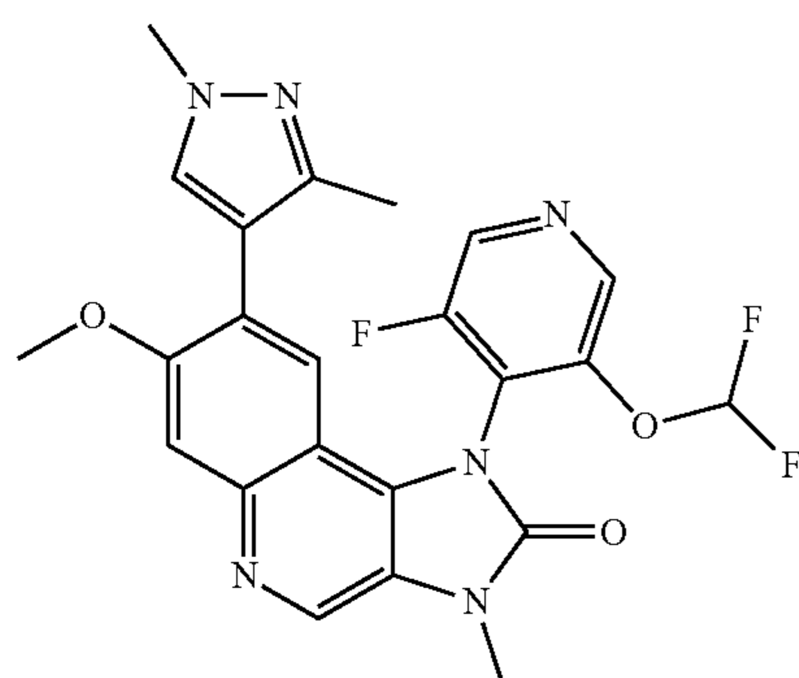
1-(3-Difluoromethoxy-5-fluoropyridin-4-yl)-8-(1,3-dimethyl-1H-pyrazol-4-yl)-7-methoxy-3-methyl-1,3-dihydroimidazo[4,5-c]quinolin-2-one
