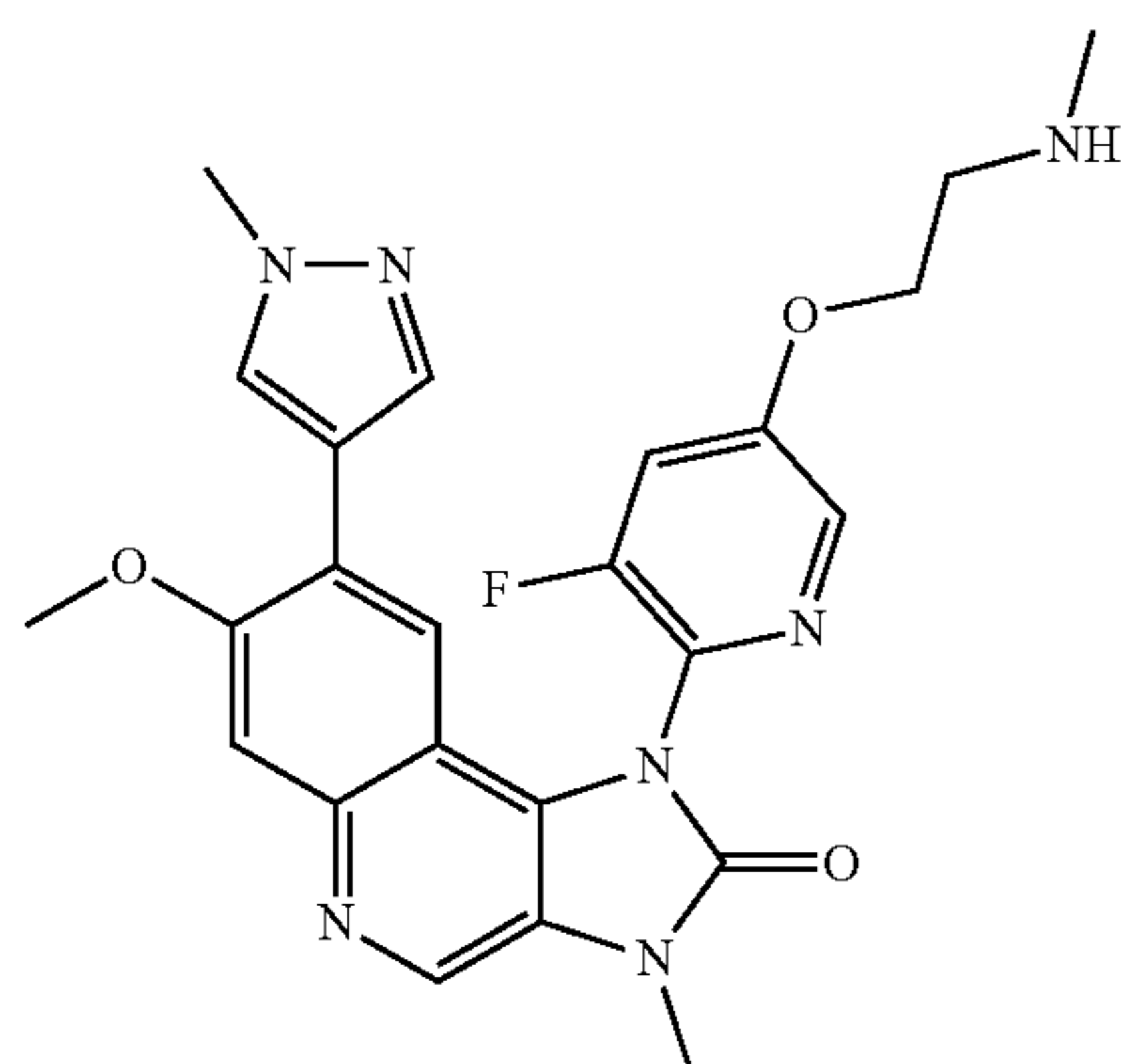
1-[3-Fluoro-5-(2-methylaminoethoxy)-pyridin-2-yl]-7-methoxy-3-methyl-8-(1-methyl-1H-pyrazol-4-yl)-1,3-dihydroimidazo[4,5-c]quinolin-2-one
