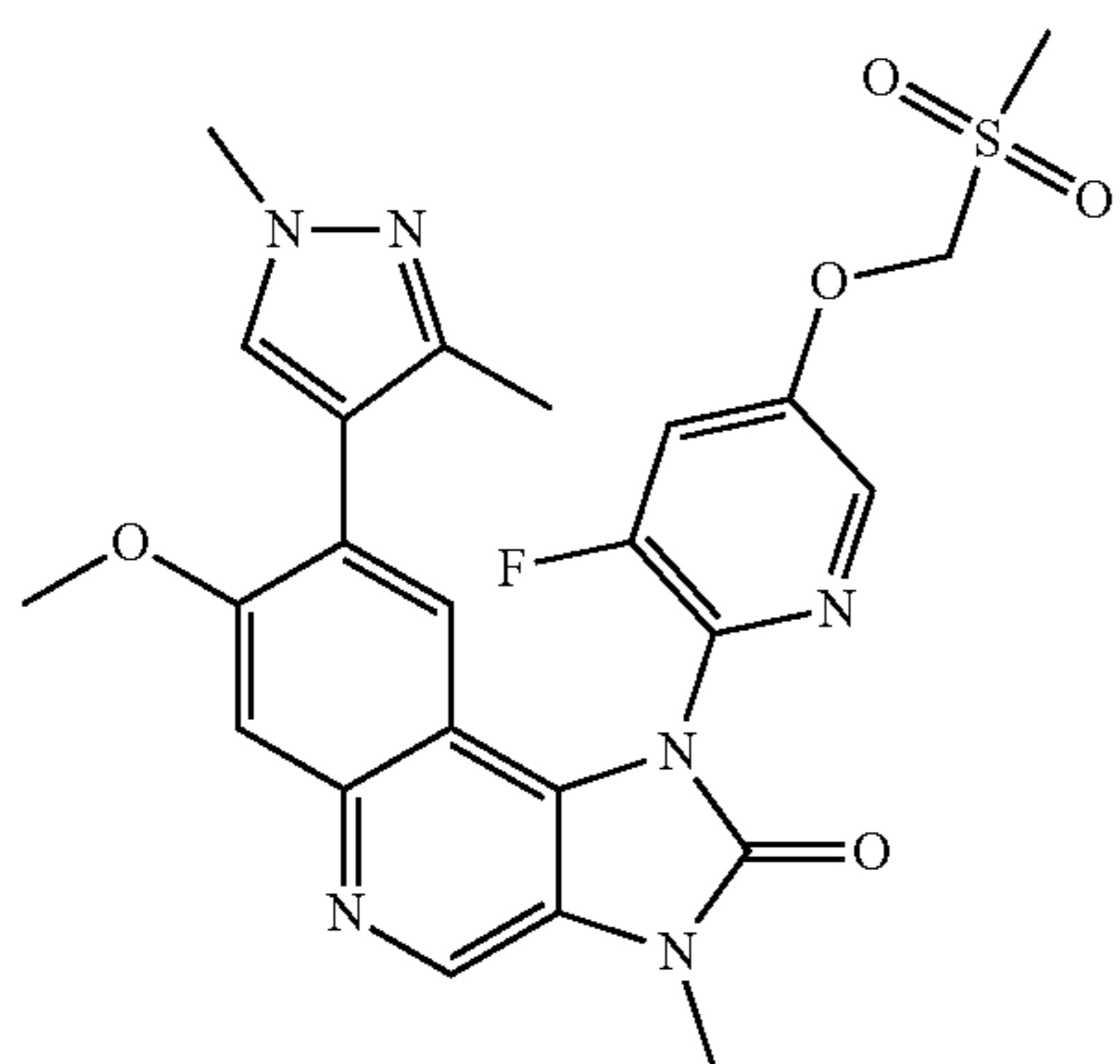
8-(1,3-Dimethyl-1H-pyrazol-4-yl)-1-(3-fluoro-5-methyl-sulfonylmethoxypyridin-2-yl)-7-methoxy-3-methyl-1,3-dihydroimidazo[4,5-c]quinolin-2-one
