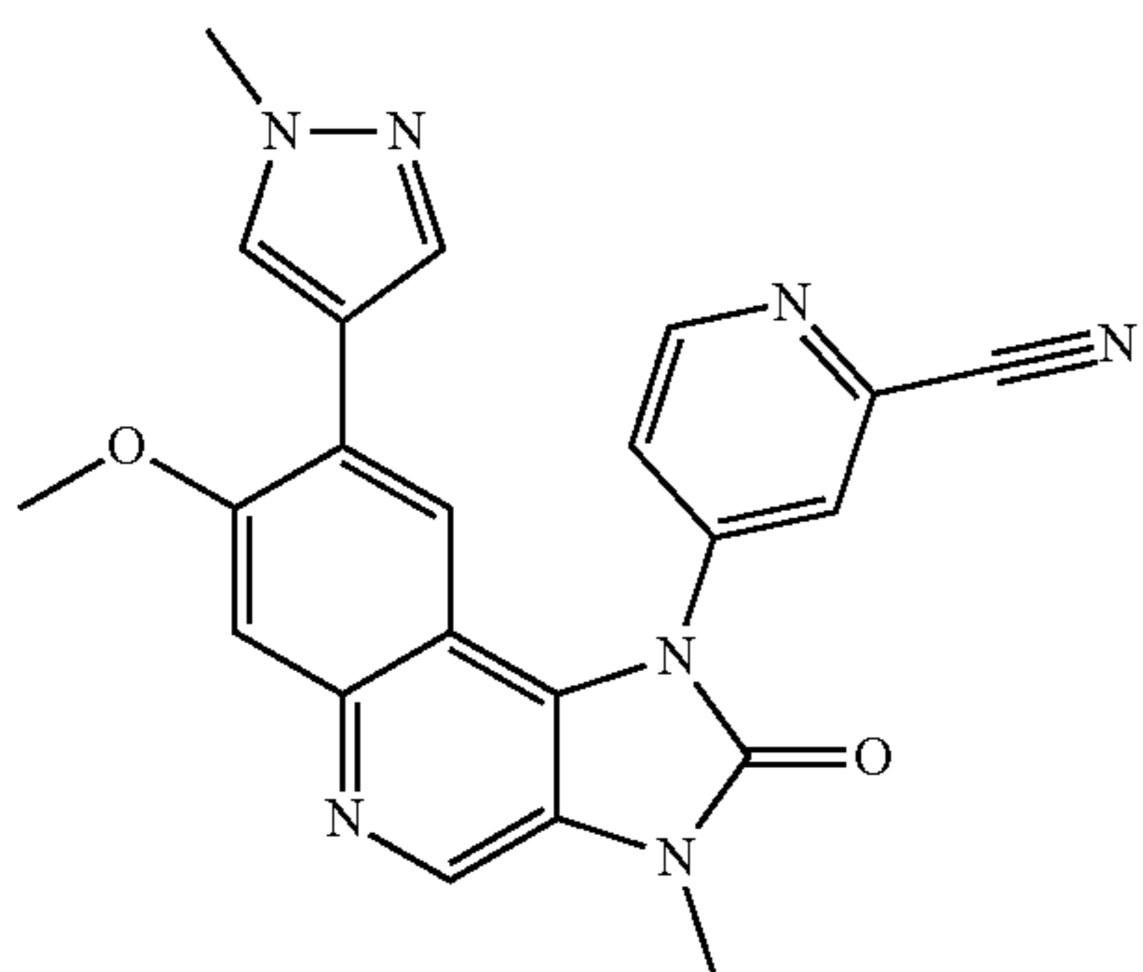
4-[7-Methoxy-3-methyl-8-(1-methyl-1H-pyrazol-4-yl)-2-oxo-2,3-dihydroimidazo[4,5-c]quinolin-1-yl]pyridine-2-carbonitrile
