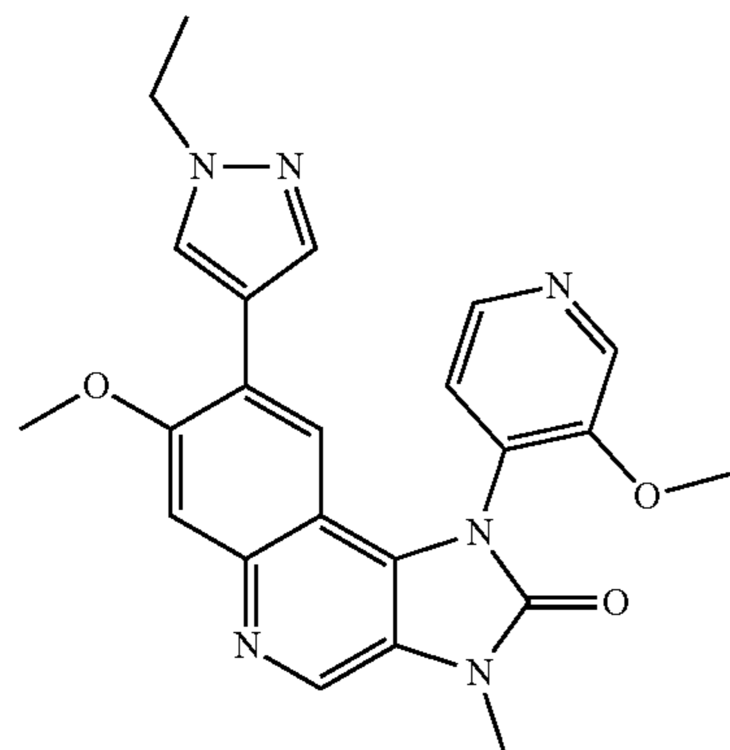
8-(1-Ethyl-1H-pyrazol-4-yl)-7-methoxy-1-(3-methoxypyridin-4-yl)-3-methyl-1,3-dihydroimidazo[4,5-c]quinolin-2-one
