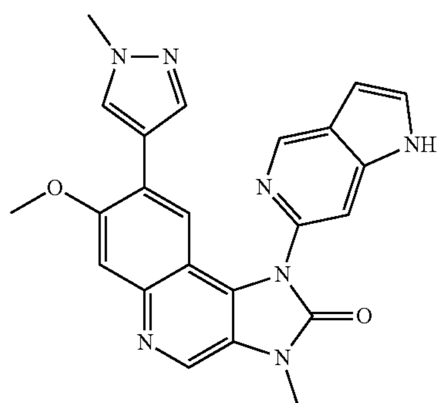
7-Methoxy-3-methyl-8-(1-methyl-1H-pyrazol-4-yl)-1-(1H-pyrrolo[3,2-c]pyridin-6-yl)-1,3-dihydroimidazo[4,5-c]quinolin-2-one
