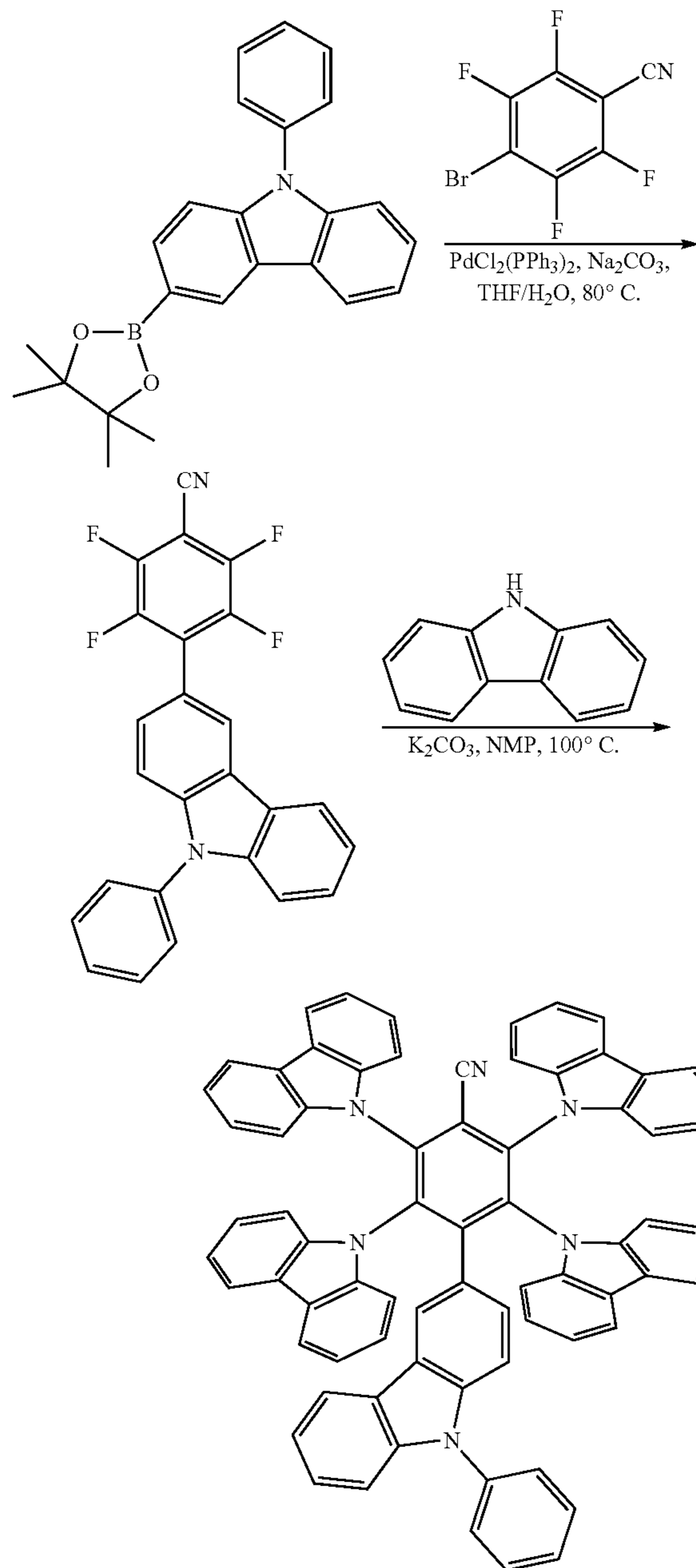
Synthesis of 2,3,5,6-tetrafluoro-4-(9-phenyl-9H-carbazol-3-yl)benzonitrile
