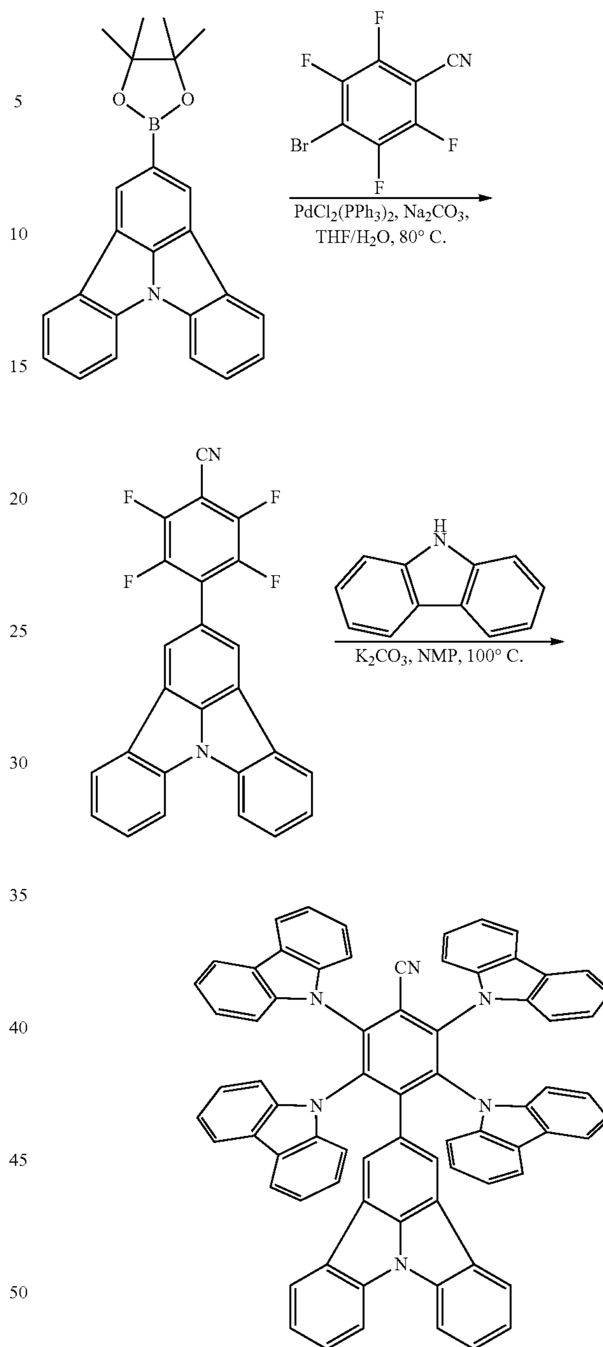
Synthesis of 2,3,5,6-tetrafluoro-4-(indolo[3,2,1-jk]carbazol-2-yl)benzonitrile
