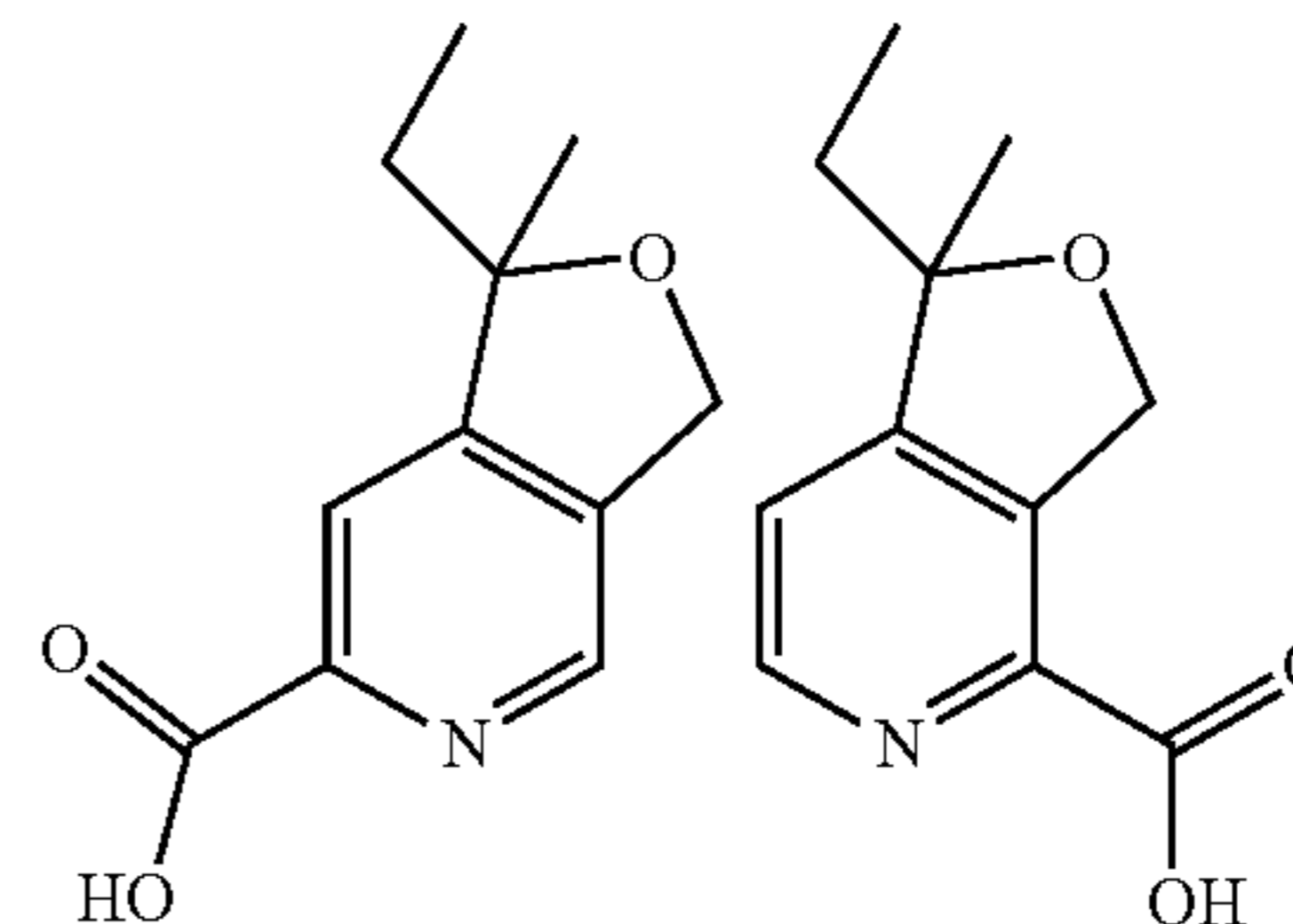
1-ethyl-1-methyl-1,3-dihydrofuro[3,4-c]pyridine-6-carboxylic acid and 1-ethyl-1-methyl-1,3-dihydrofuro[3,4-c]pyridine-4-carboxylic acid
