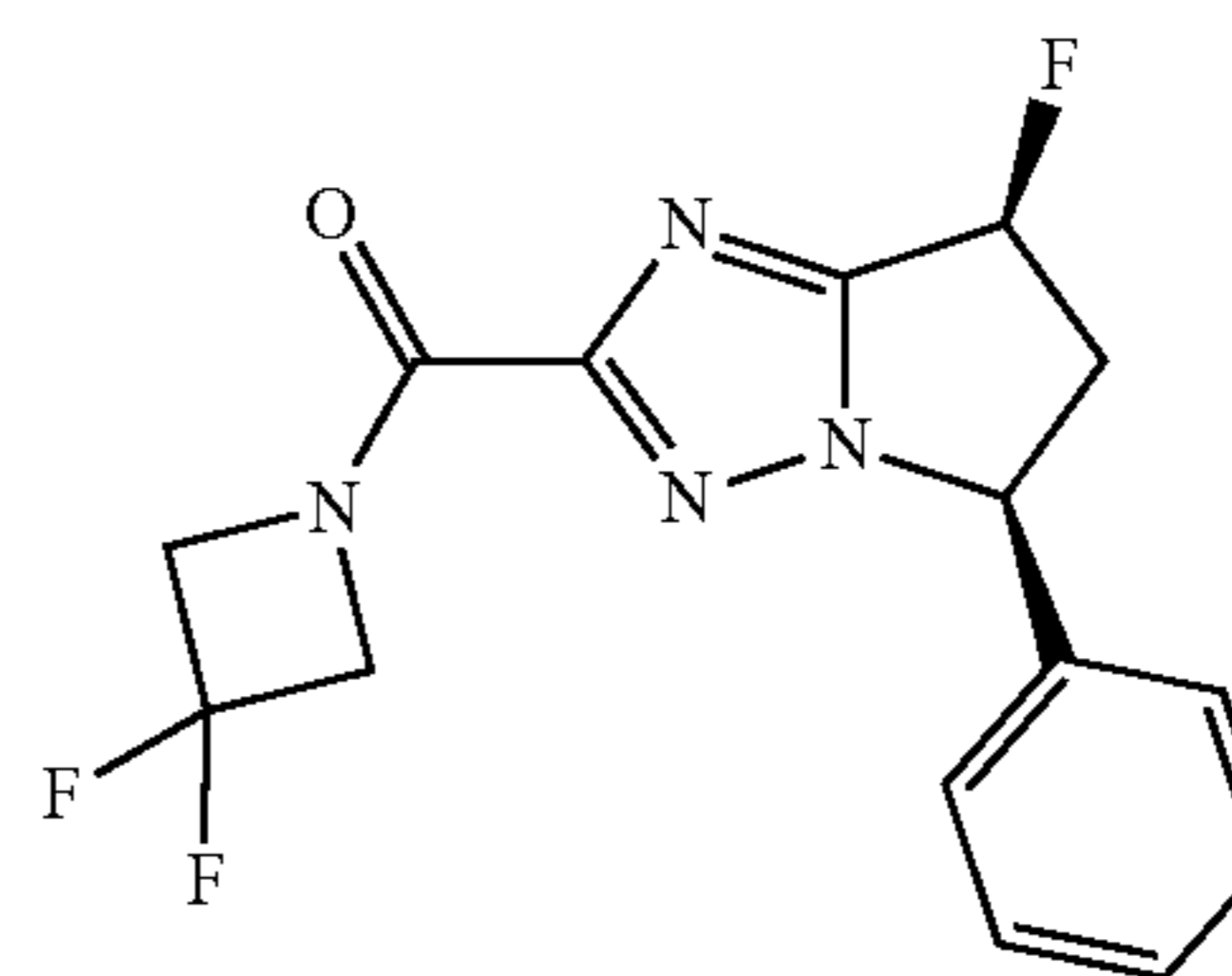
(3,3-difluoroazetid-1-yl)-[(5S,7S)-7-fluoro-5-phenyl-6,7-dihydro-5H-pyrrolo[1,2-b][1,2,4]triazol-2-yl]methanone (cis mixture)
