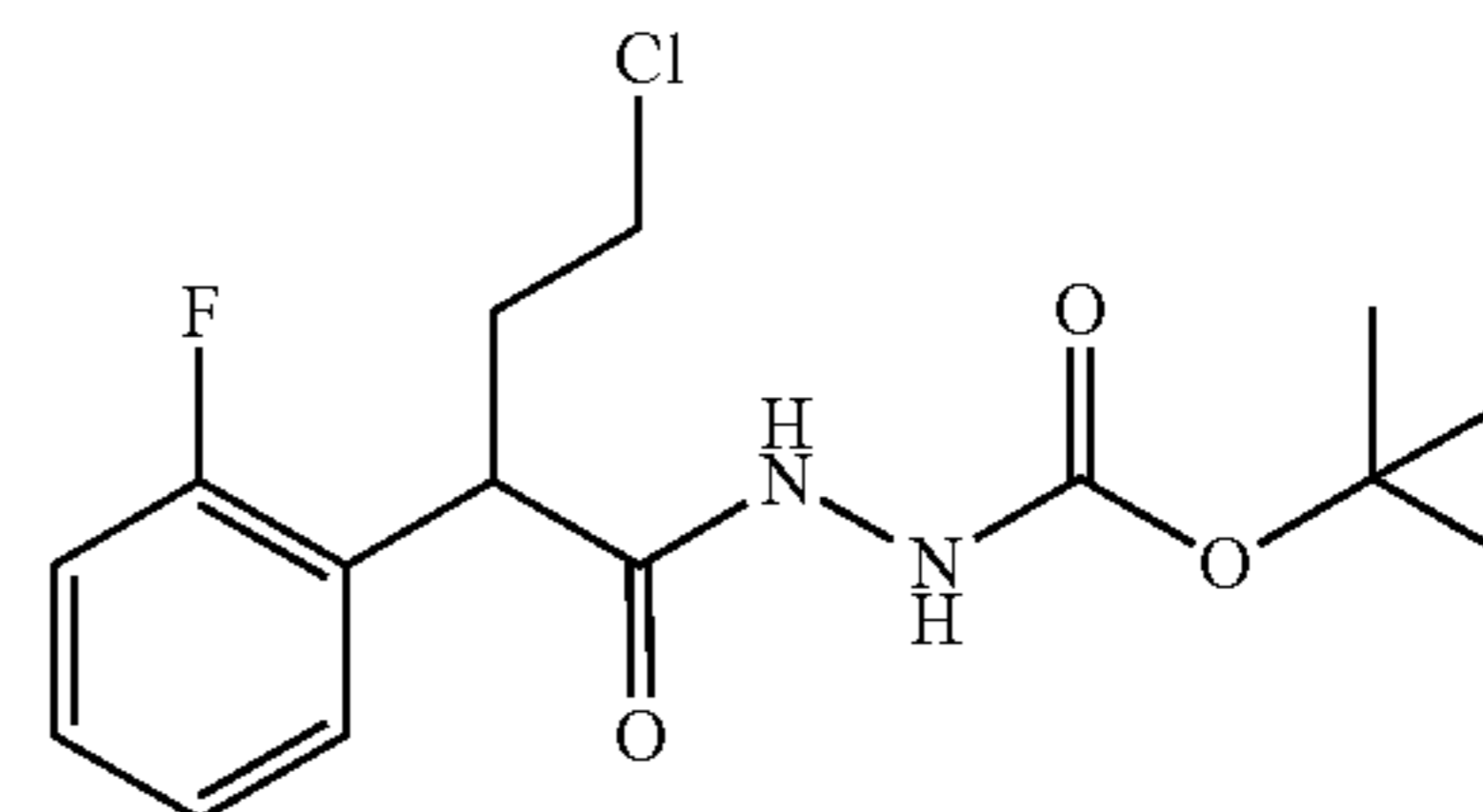
Step 3: tert-butyl 2-(4-chloro-2-(2-fluorophenyl)butanoyl)hydrazinecarboxylate
