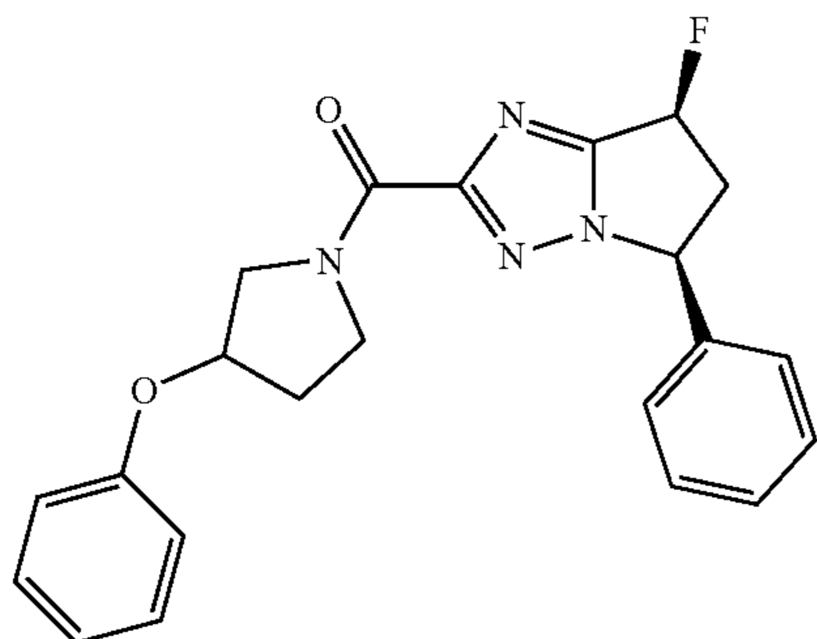
(3-phenoxy)pyrrolidin-1-yl-[rac-(5S,7S)-7-fluoro-5-phenyl-6,7-dihydro-5H-pyrrolo[1,2-b][1,2,4]triazol-2-yl]methanone (arbitrarily assigned 5S, 7S configuration)
