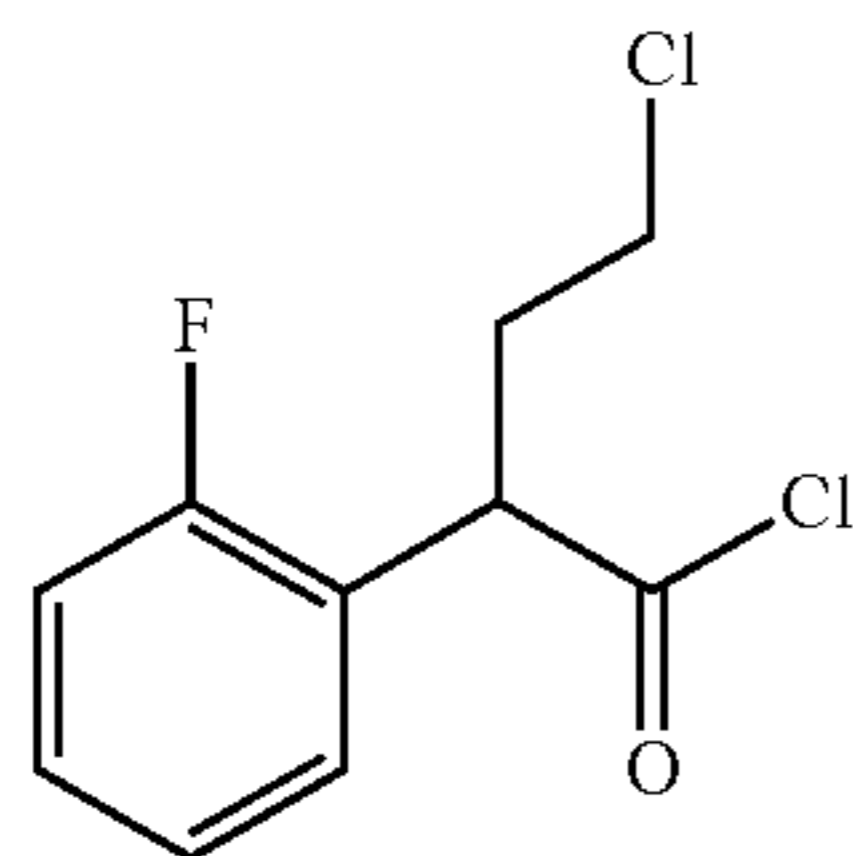
Step 2: 4-chloro-2-(2-fluorophenyl)butanoyl chloride
