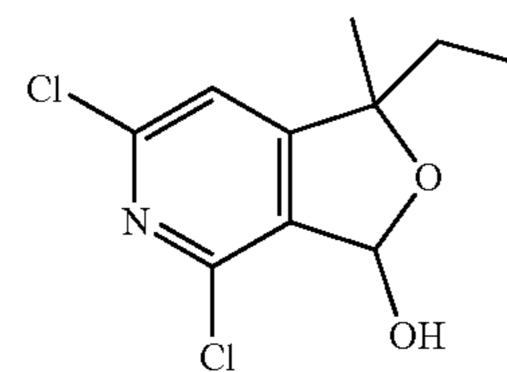
4,6-dichloro-1-ethyl-1-methyl-1,3-dihydrofuro[3,4-c]pyridin-3-ol
