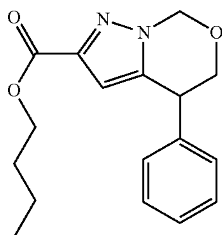
Step 4: butyl 4-phenyl-6,7-dihydro-4H-pyrazolo[5, 1-c][1,4]oxazine-2-carboxylate
