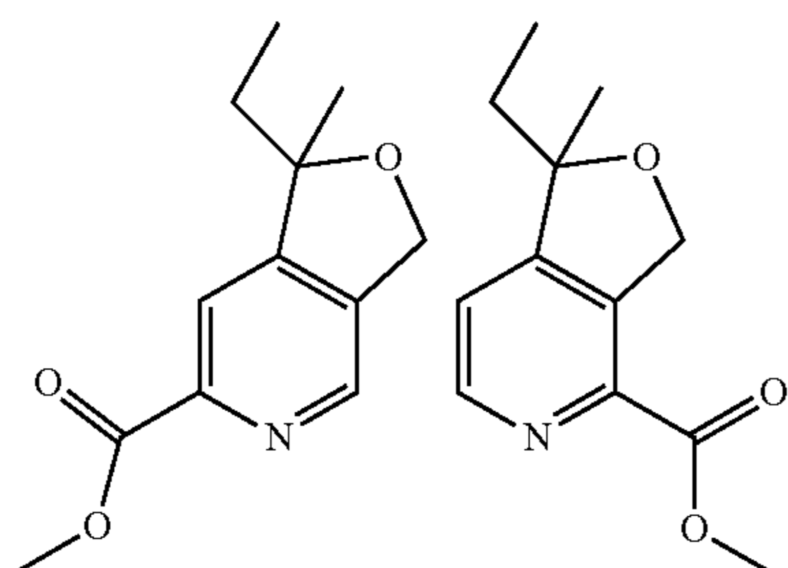
Methyl 1-ethyl-1-methyl-1,3-dihydrofuro[3,4-c]pyridine-6-carboxylate and methyl 1-ethyl-1-methyl-1,3-dihydrofuro[3,4-c]pyridine-4-carboxylate
