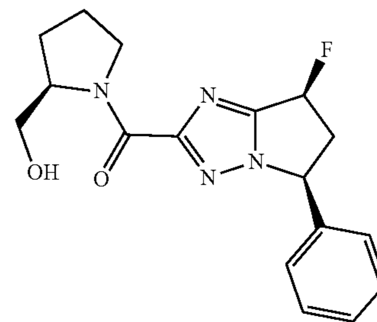
[rac-(5S,7S)-7-fluoro-5-phenyl-6,7-dihydro-5H-pyrrolo[1,2-b][1,2,4]triazol-2-yl]-[rac-(2R)-2-(hydroxymethyl)pyrrolidin-1-yl]methanone (arbitrarily assigned 2R, 5S, 7S) configuration)
