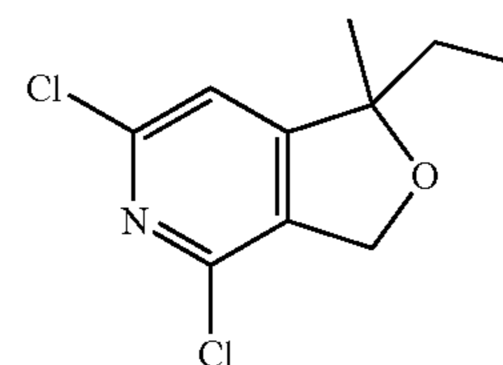
4,6-dichloro-1-ethyl-1-methyl-1,3-dihydrofuro[3,4-c]pyridine
