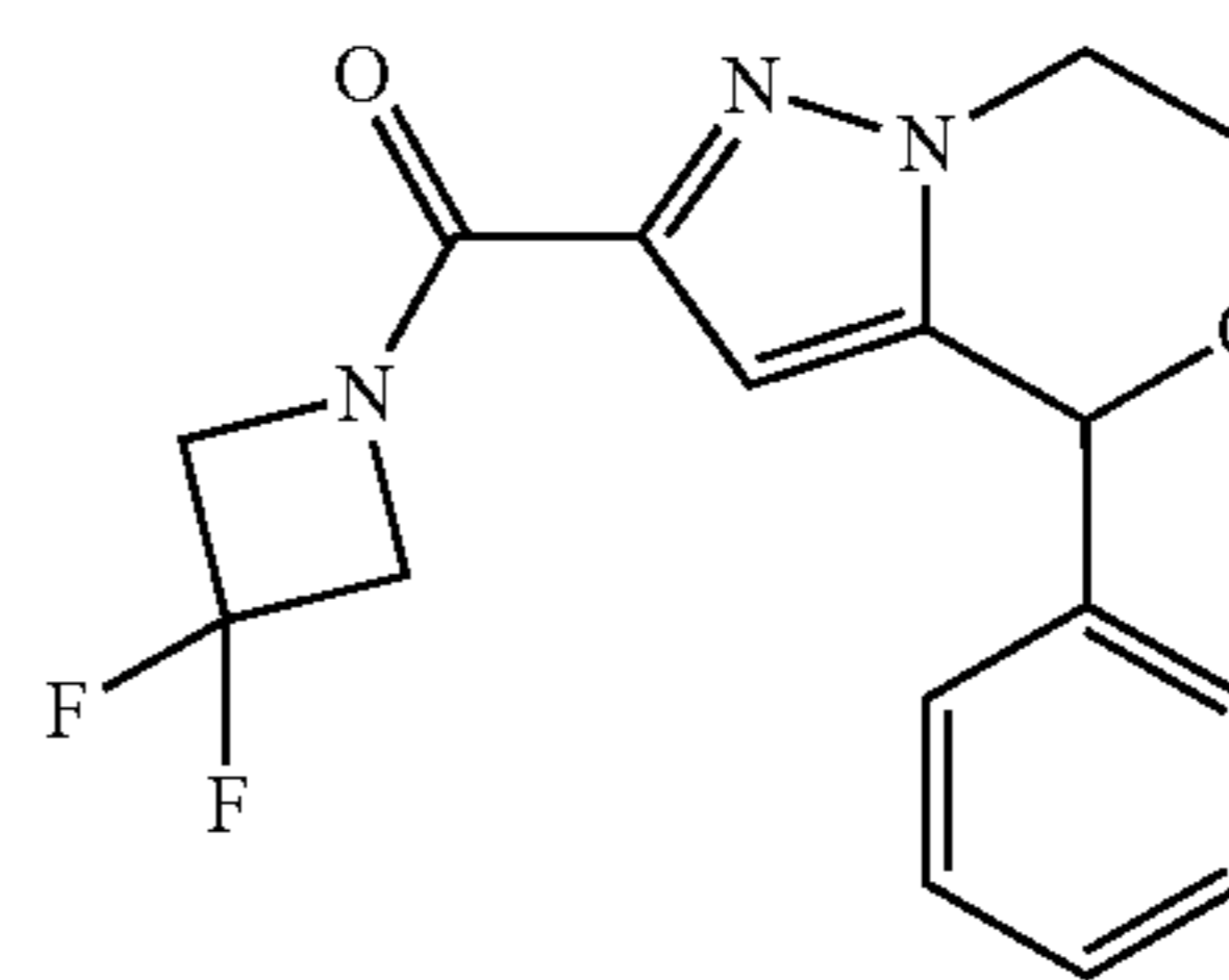
Step 6: (3,3-difluoroazetididin-1-yl)-(4-phenyl-6,7- dihydro-4H-pyrazolo[5,1-c][1,4]oxazin-2-yl)metha- none
