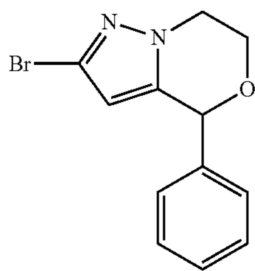
Step 3: 2-bromo-4-phenyl-6,7-dihydro-4H-pyrazolo [5,1-c][1,4]oxazine
