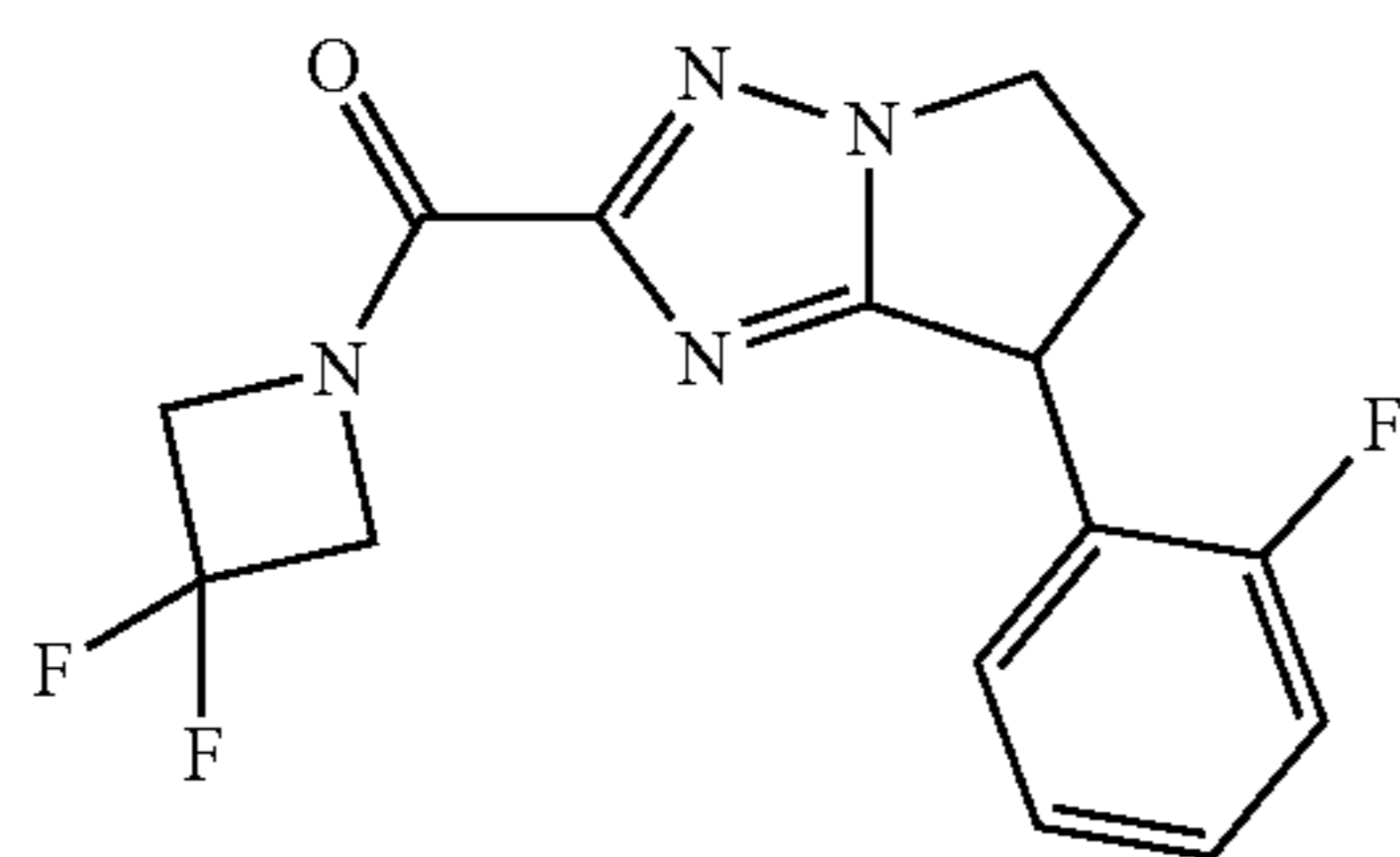
(3,3-difluoroazetidin-1-yl)-[7-(2-fluorophenyl)-6,7-dihydro-5H-pyrrolo[1,2-b][1,2,4]triazol-2-yl]methanone
