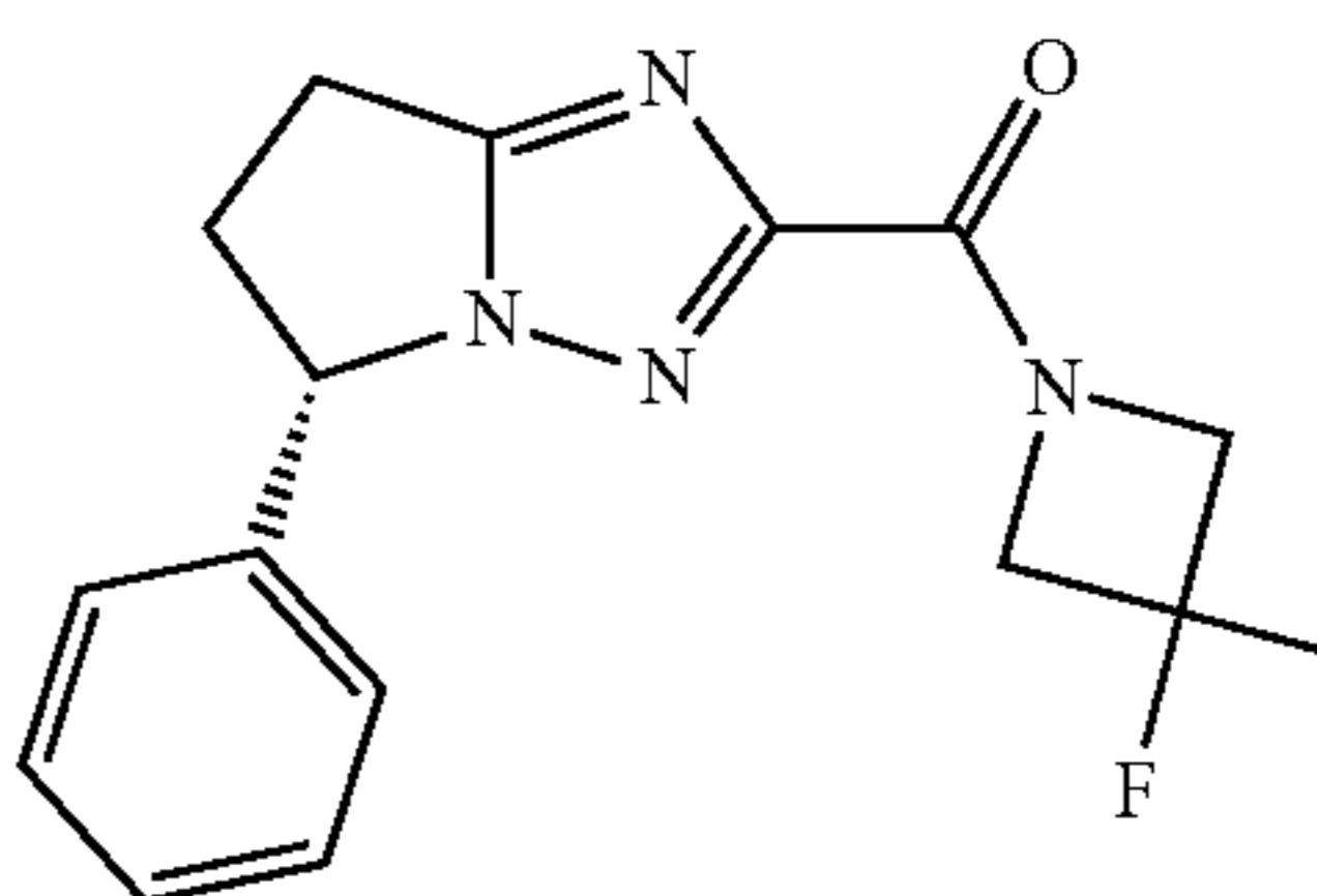
(3,3-difluoroazetidin-1-yl)-[rac-(5S)-5-phenyl-6,7-dihydro-5H-pyrrolo[1,2-b][1,2,4]triazol-2-yl]methanone
