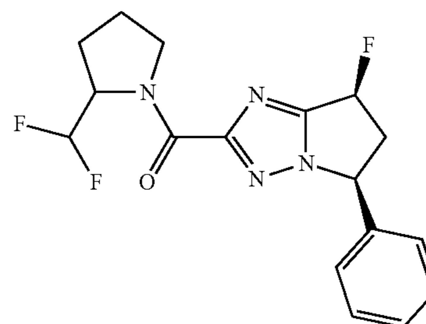
[2-(difluoromethyl)pyrrolidin-1-yl]-[rac-(5S,7S)-7-fluoro-5-phenyl-6,7-dihydro-5H-pyrrolo[1,2-b][1,2,4]triazol-2-yl]methanone (arbitrarily assigned 5S, 7S configuration)
