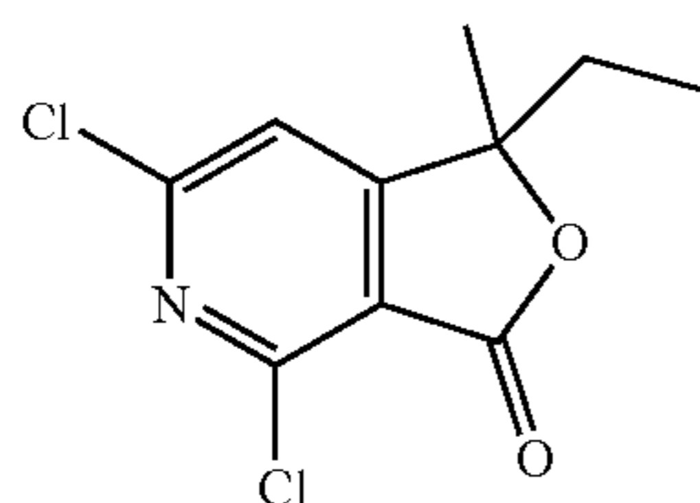
4,6-dichloro-1-ethyl-1-methylfuro[3,4-c]pyridin-3(1H)-one
