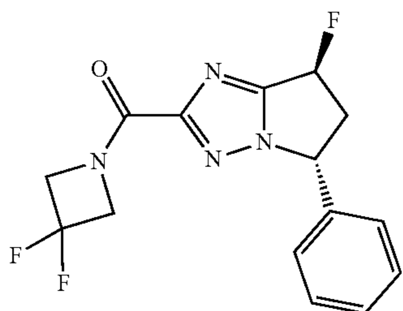
Step 3: (3,3-difluoroazetid-1-yl)-[(5R,7S)-7-fluoro-5-phenyl-6,7-dihydro-5H-pyrrolo [1,2-b][1,2,4]triazol-2-yl]methanone (trans mixture)
