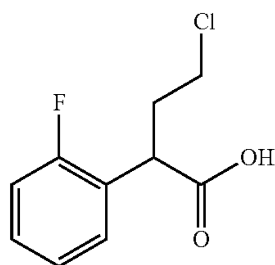
Step 1: 4-chloro-2-(2-fluorophenyl)butanoic acid
