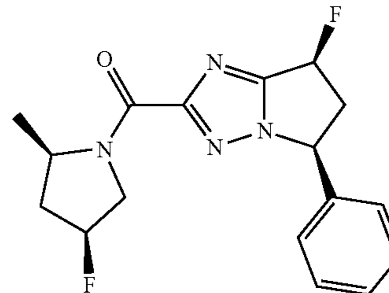
[rac-(2R,4S)-4-fluoro-2-methyl-pyrrolidin-1-yl]-[rac-(5S,7S)-7-fluoro-5-phenyl-6,7-dihydro-5H-pyrrolo[1,2-b][1,2,4]triazol-2-yl]methanone {arbitrarily assigned (2R, 4S), (5S, 7S) configuration}
