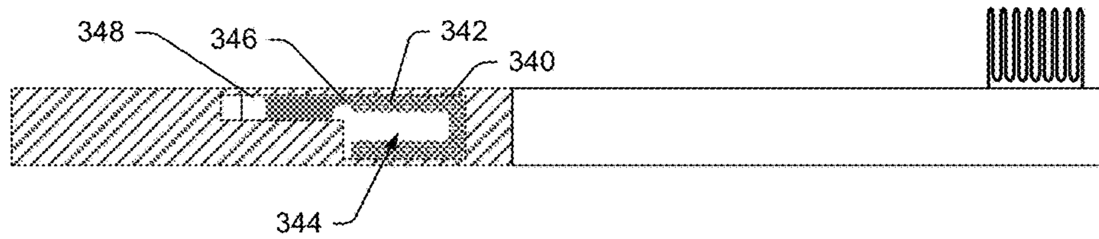
FIG. 3D SECTION D-D
