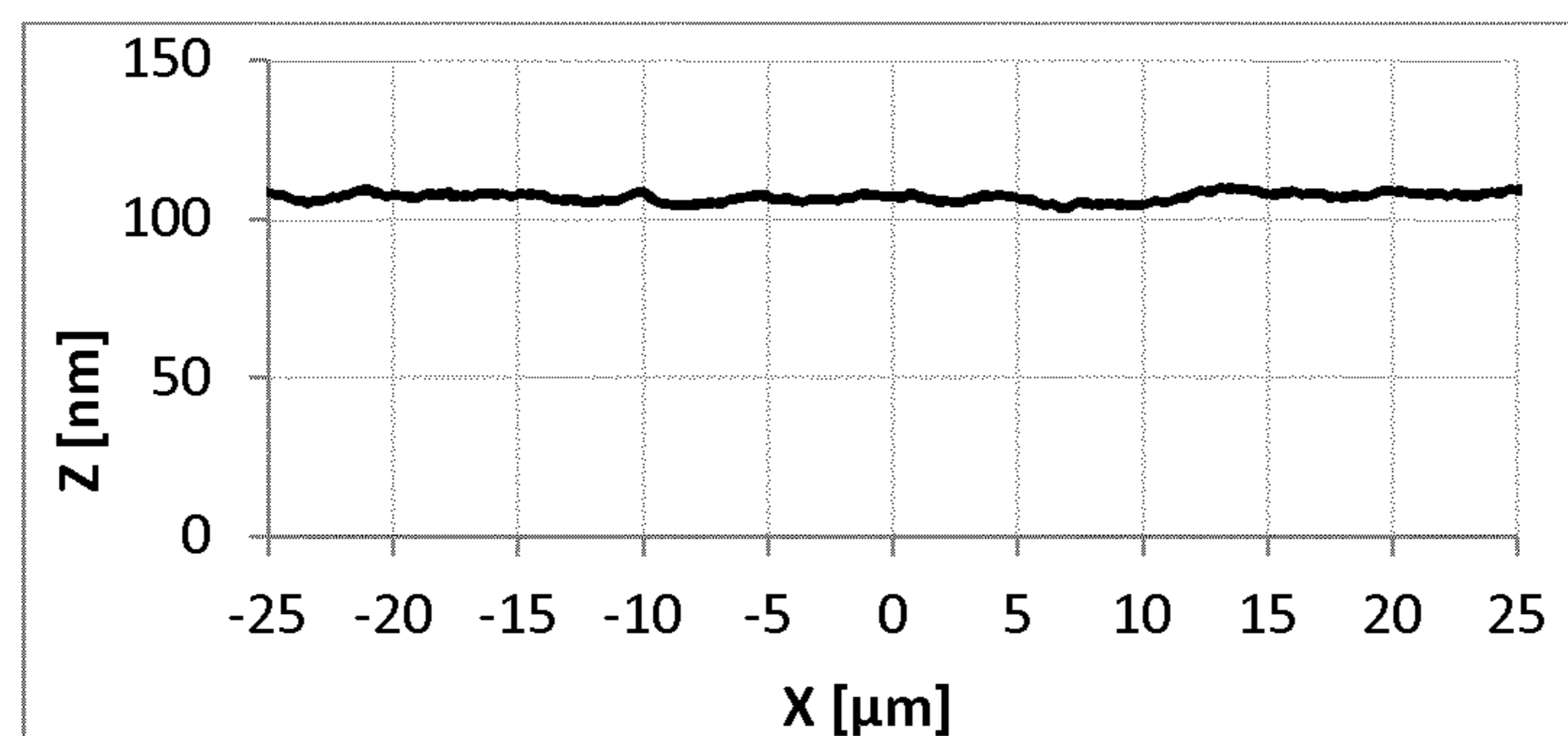
Film profile of the film of Example 8
