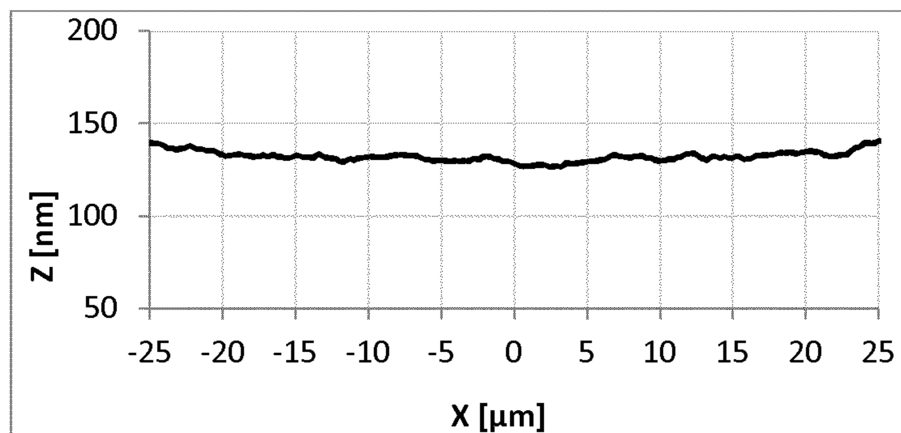
Film profile of the film of Example 3
