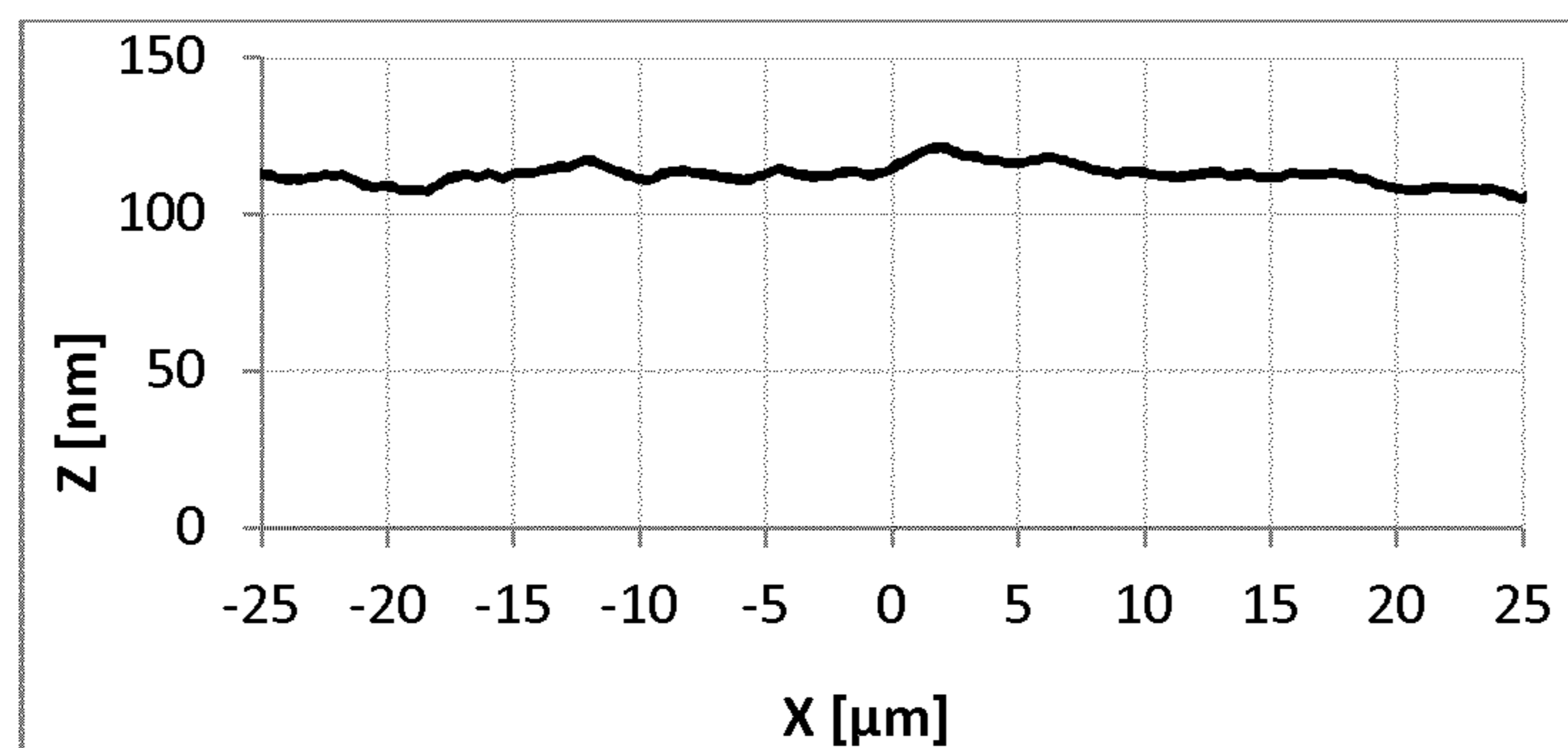
Film profile of the film of Example 6
