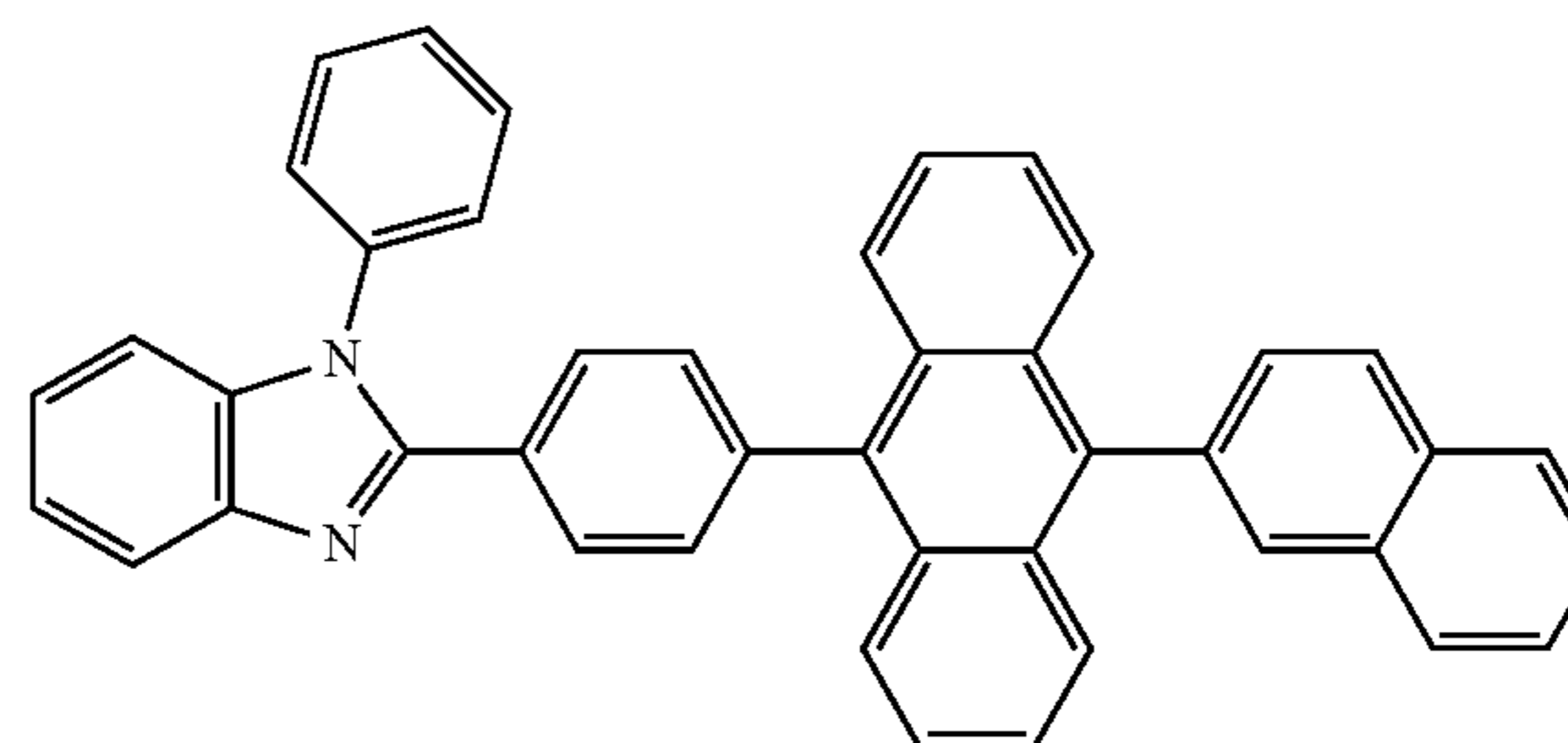
formula ET-13
