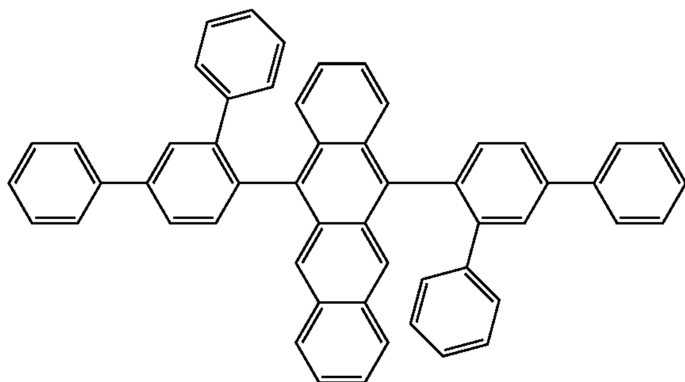
formula H-8
