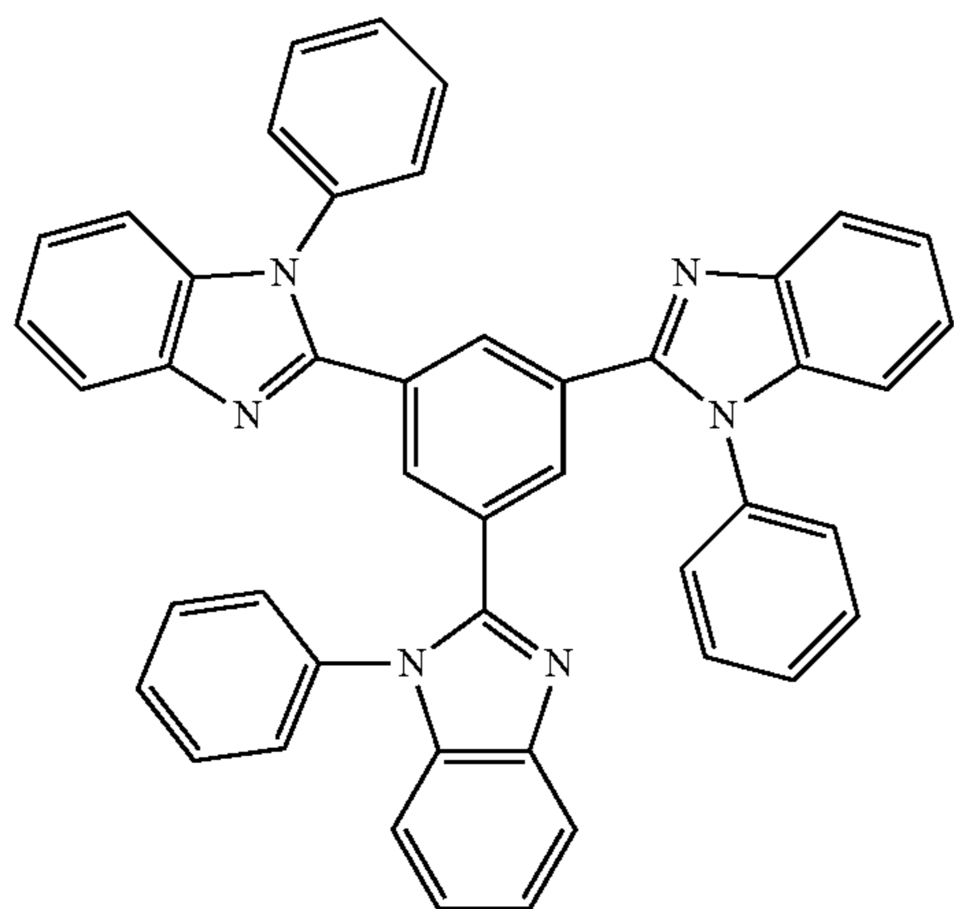
TPBI
