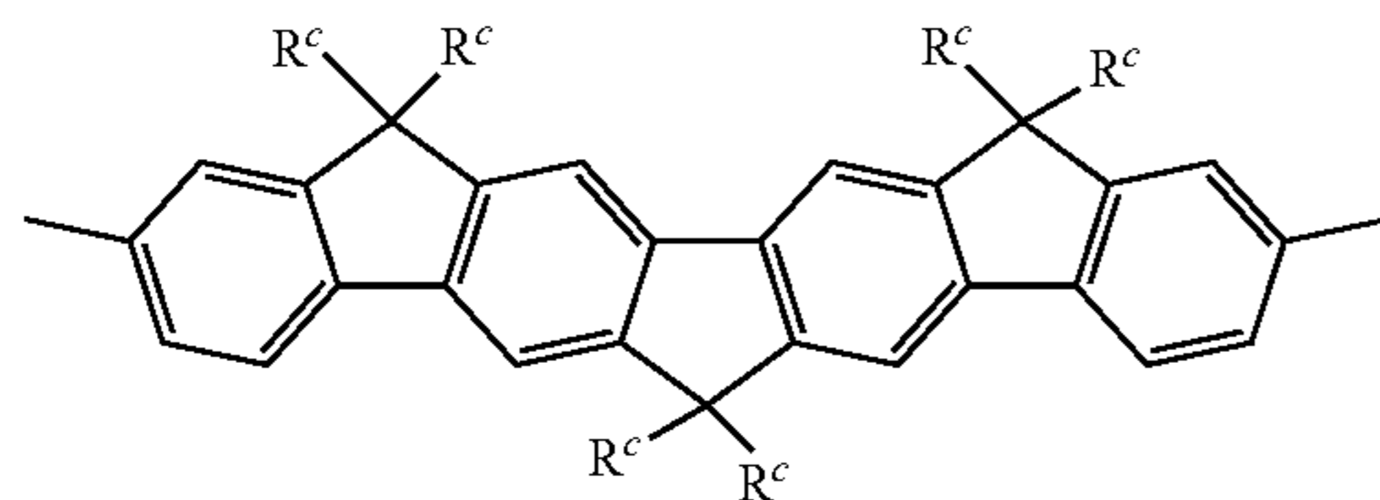
formula PB-1C
