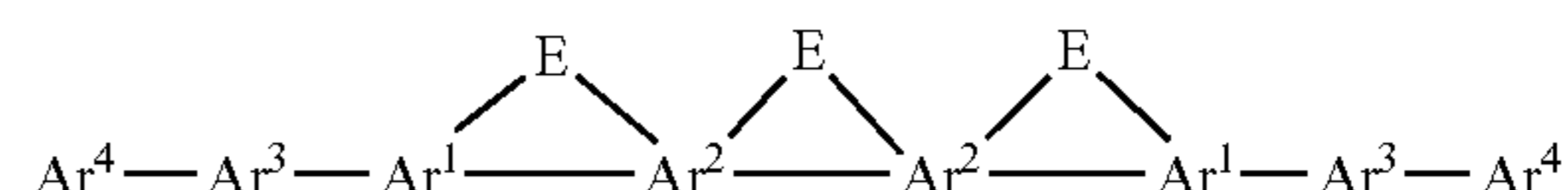
formula (3)
