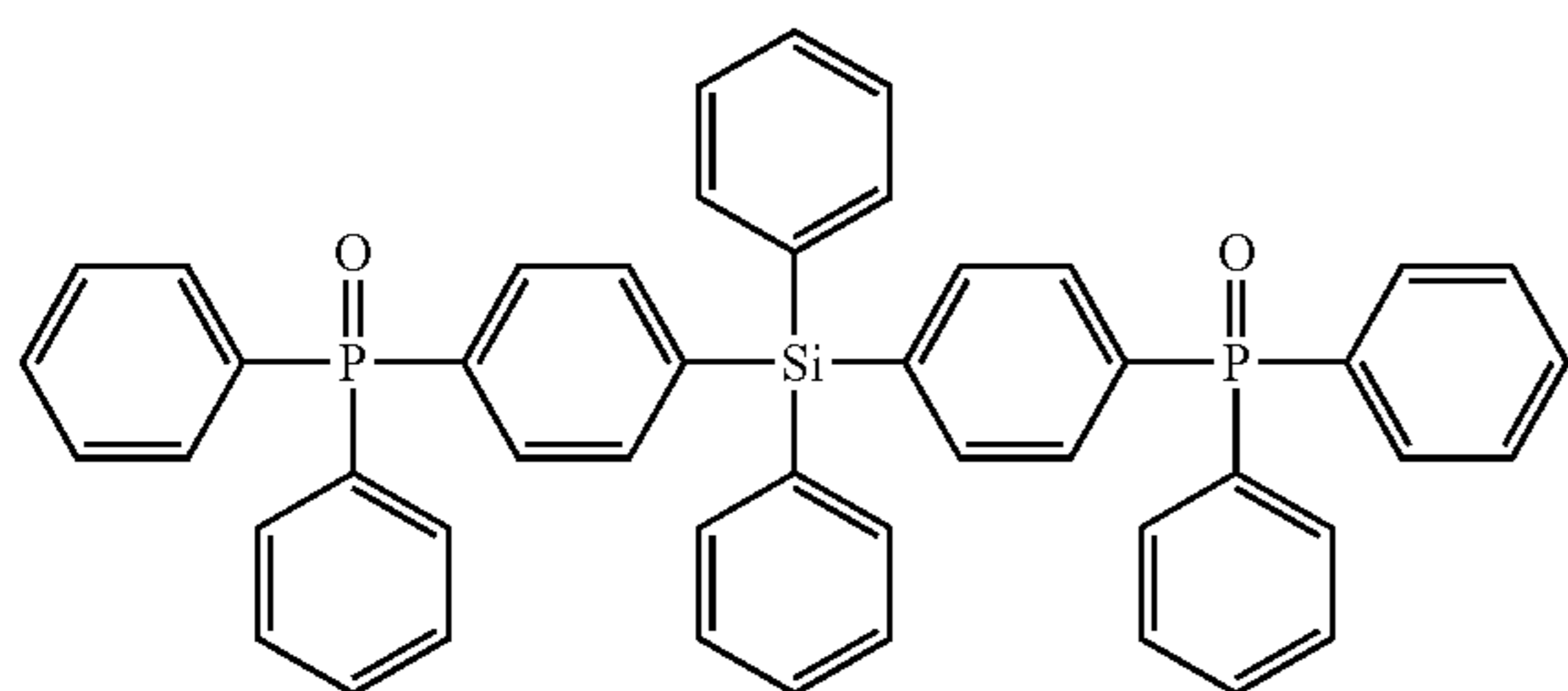
formula H-21
