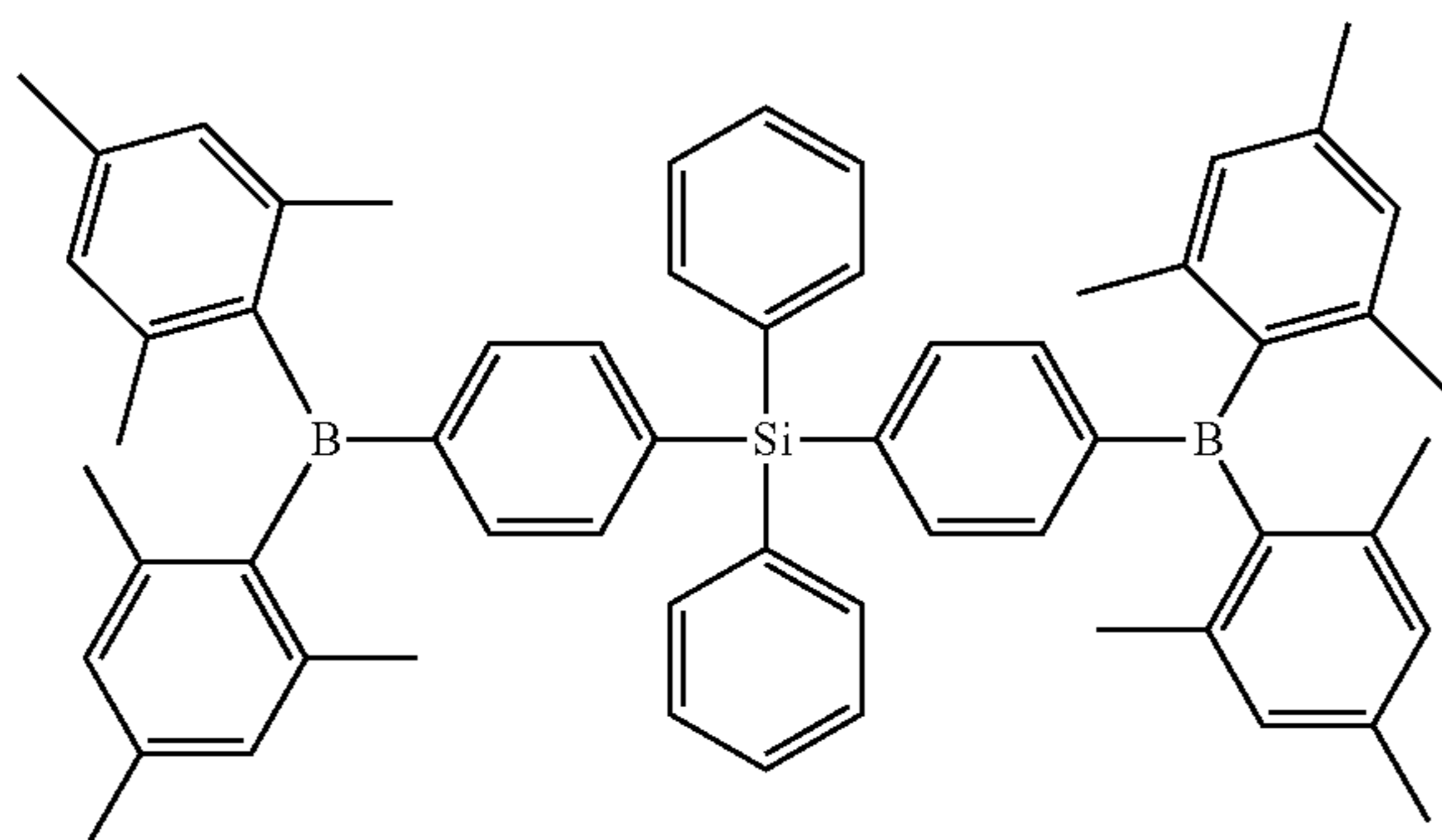
formula H-20
