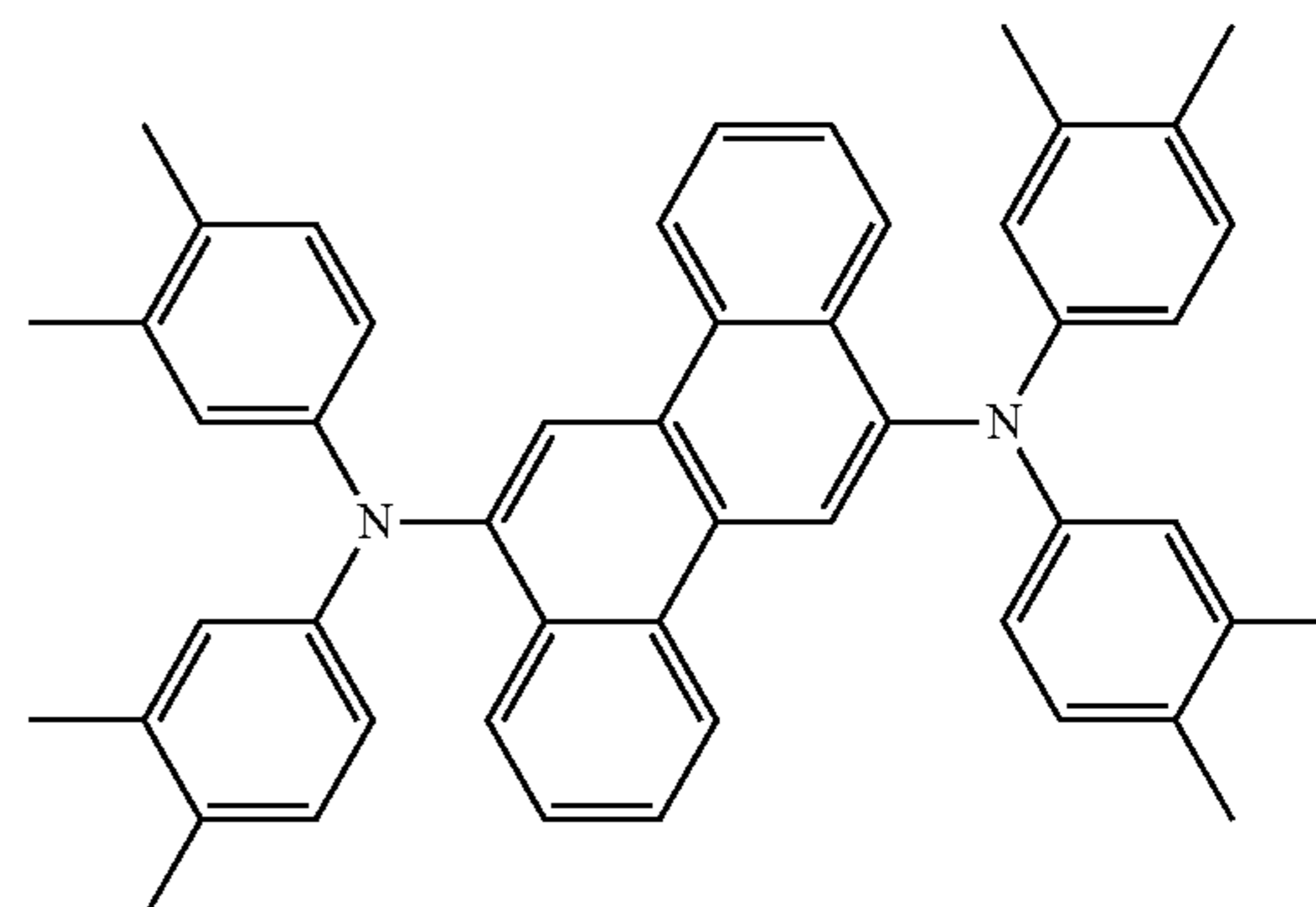
formula EM-7
