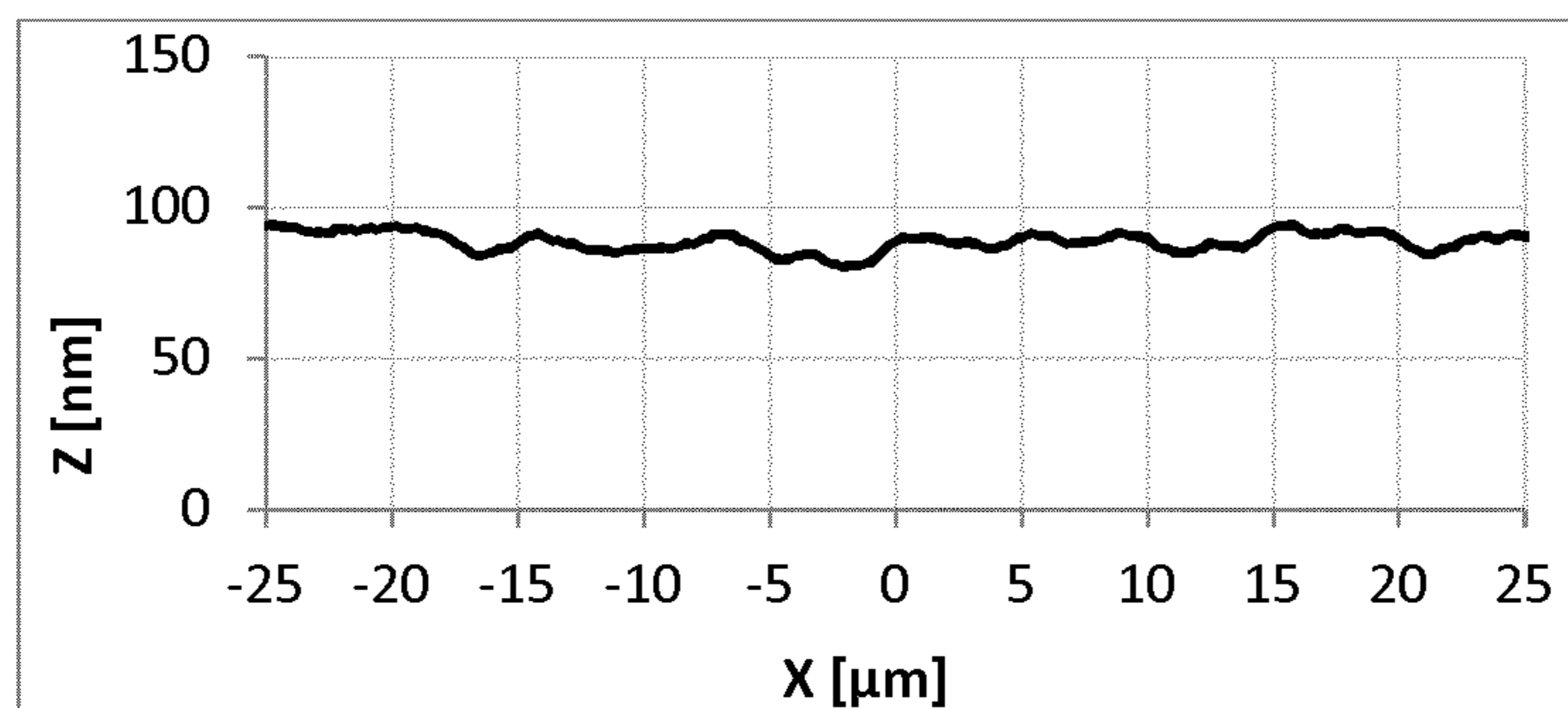
Film profile of the film of Example 9
