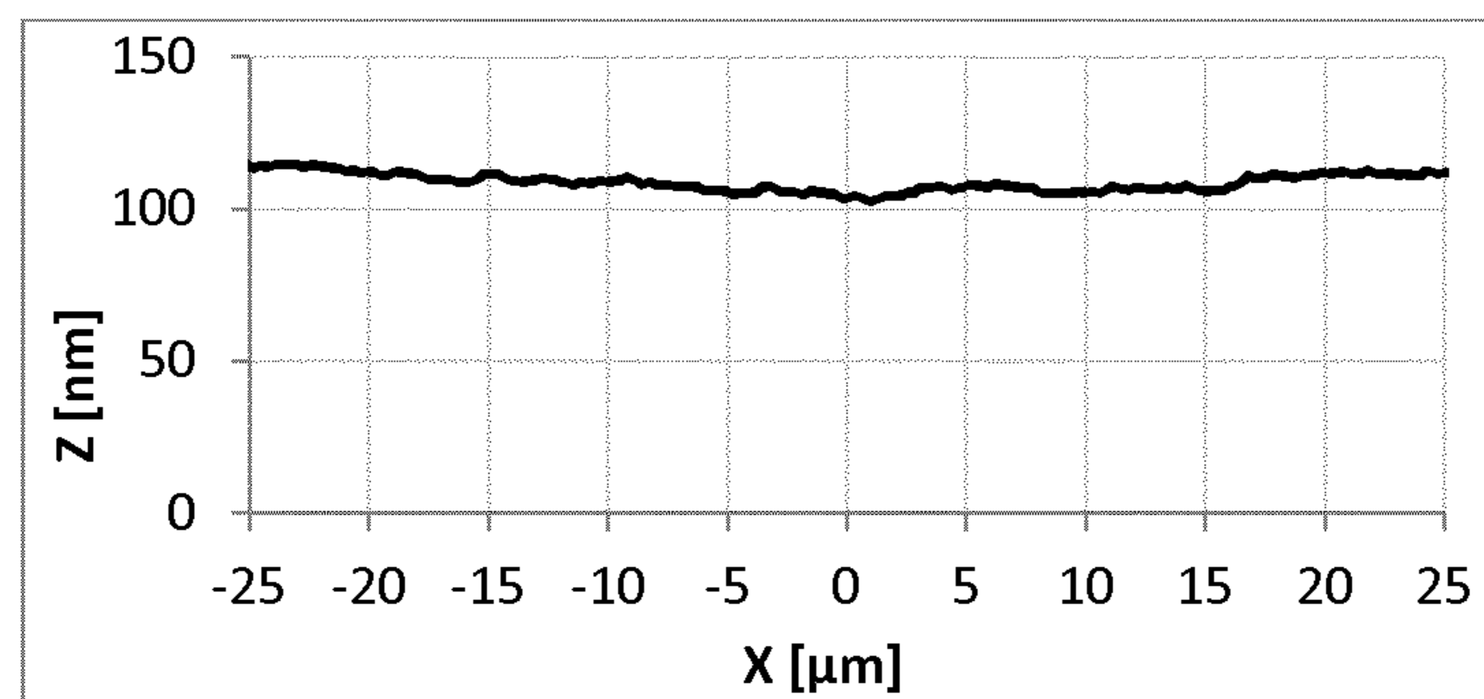
Film profile of the film of Example 5
