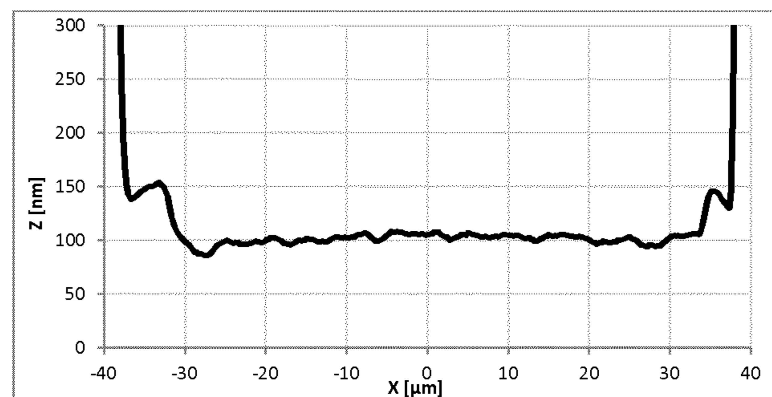
Film profile of the film of Example 14
