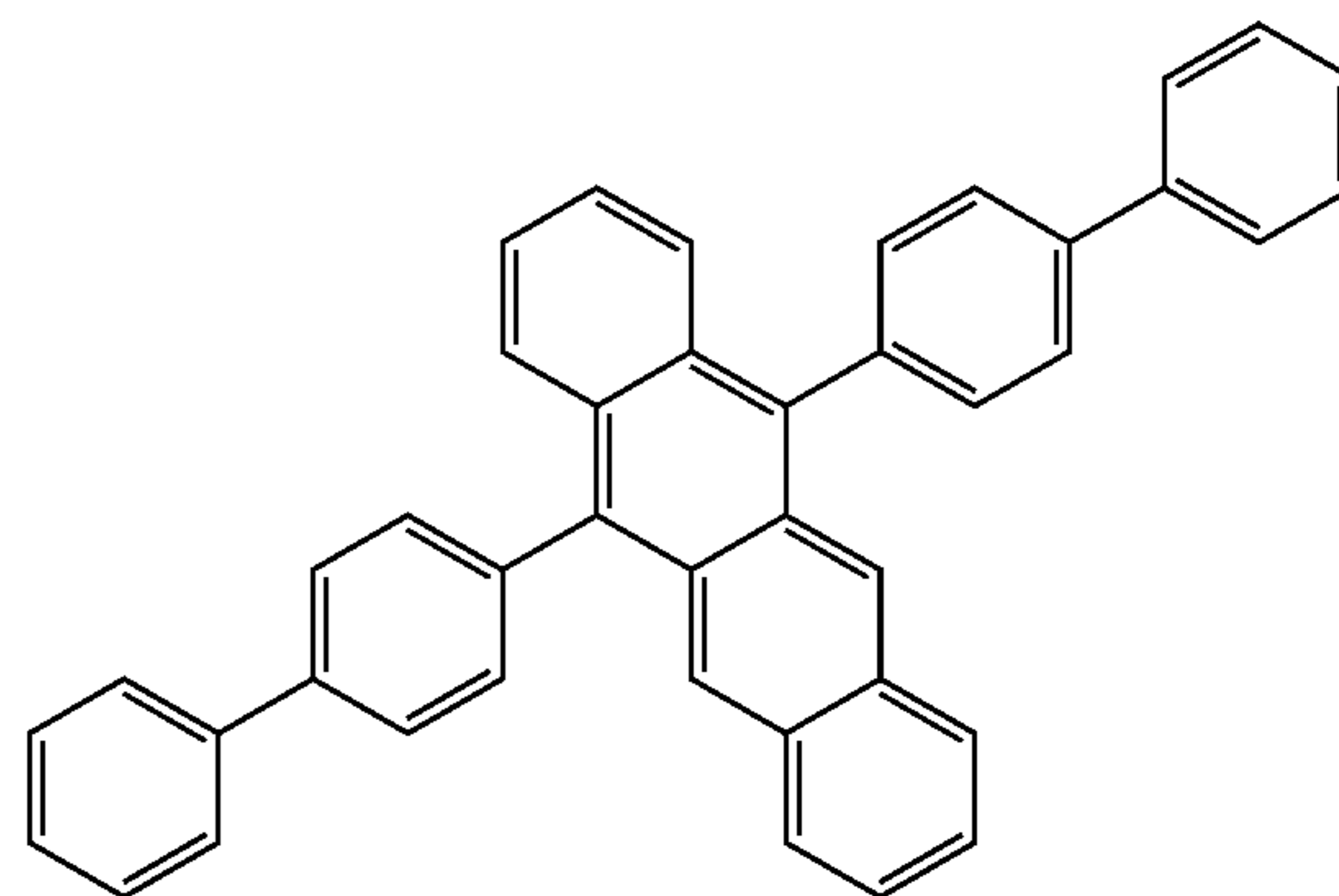
formula H-2
