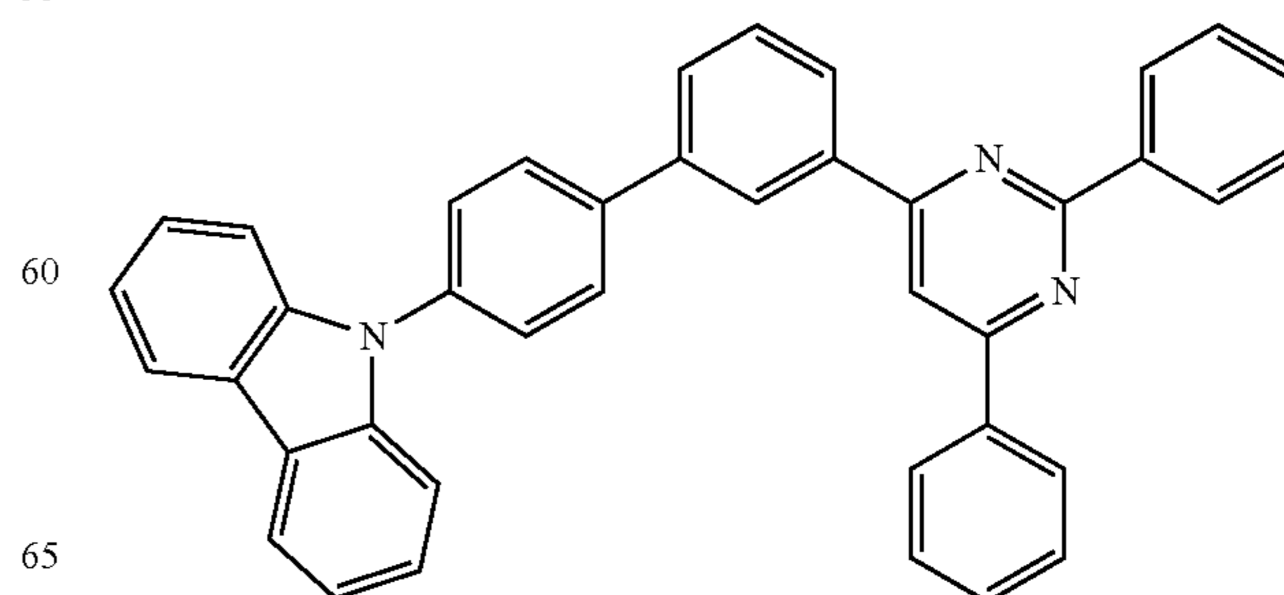
formula H-9
