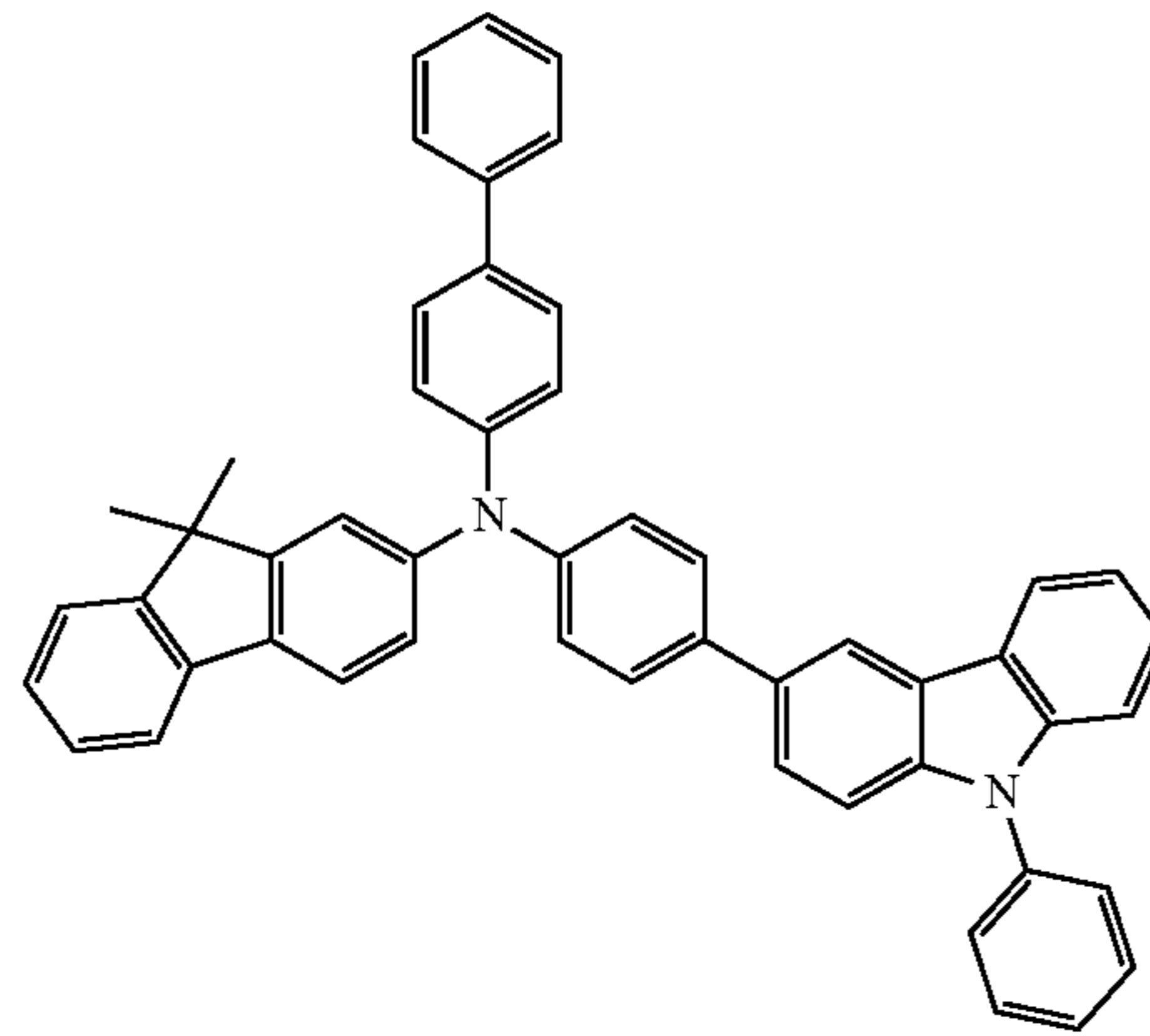
formula TA-7
