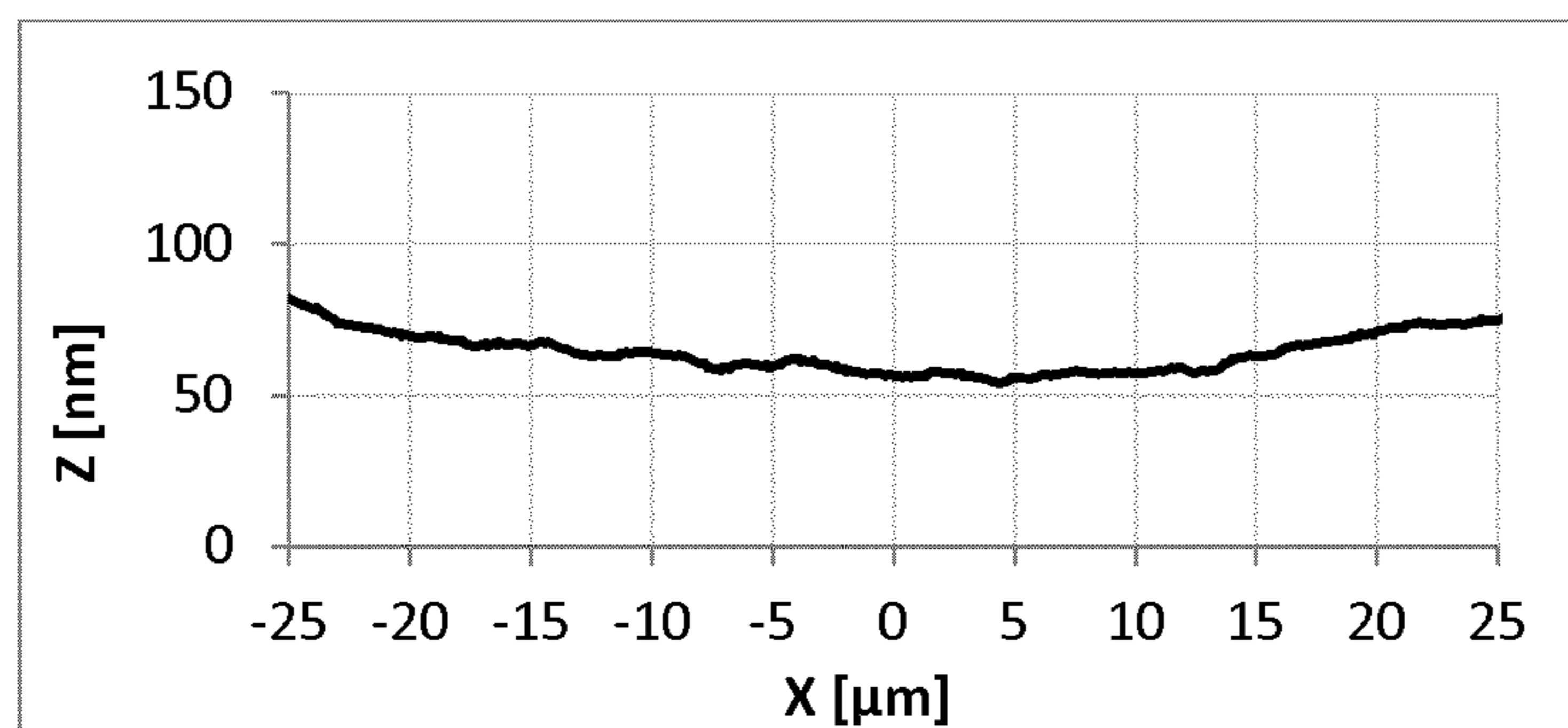
Film profile of the film of the Reference Example
