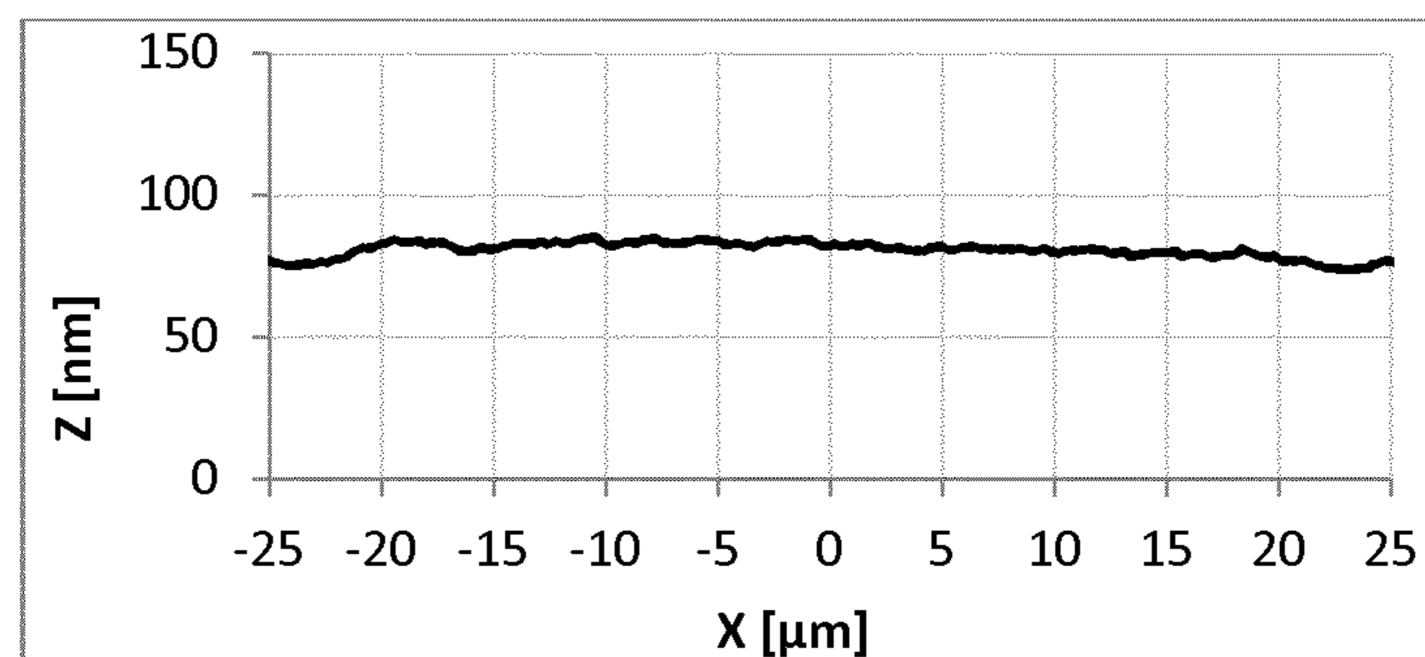
Film profile of the film of Example 11
