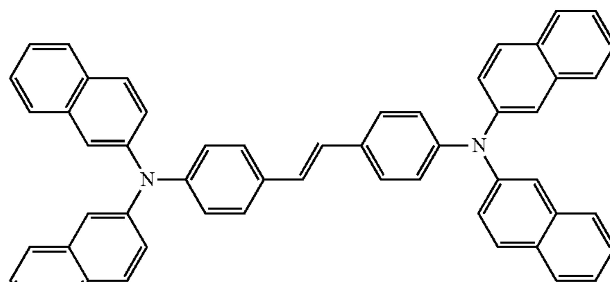
formula EM-2
