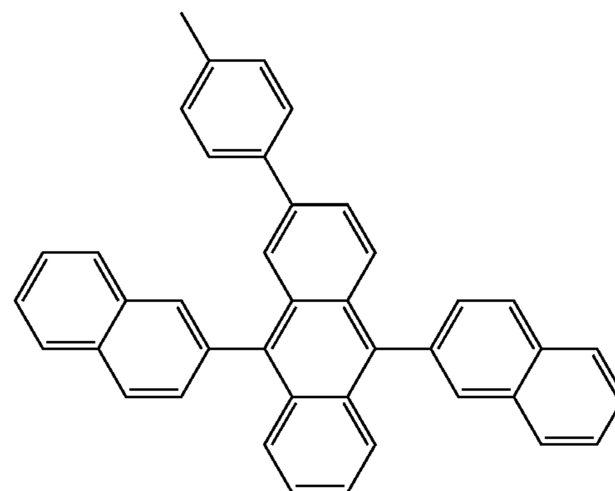
formula H-3
