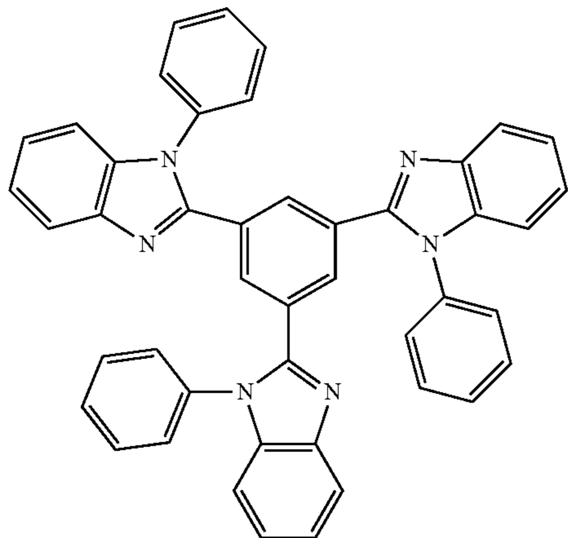
TPBI
