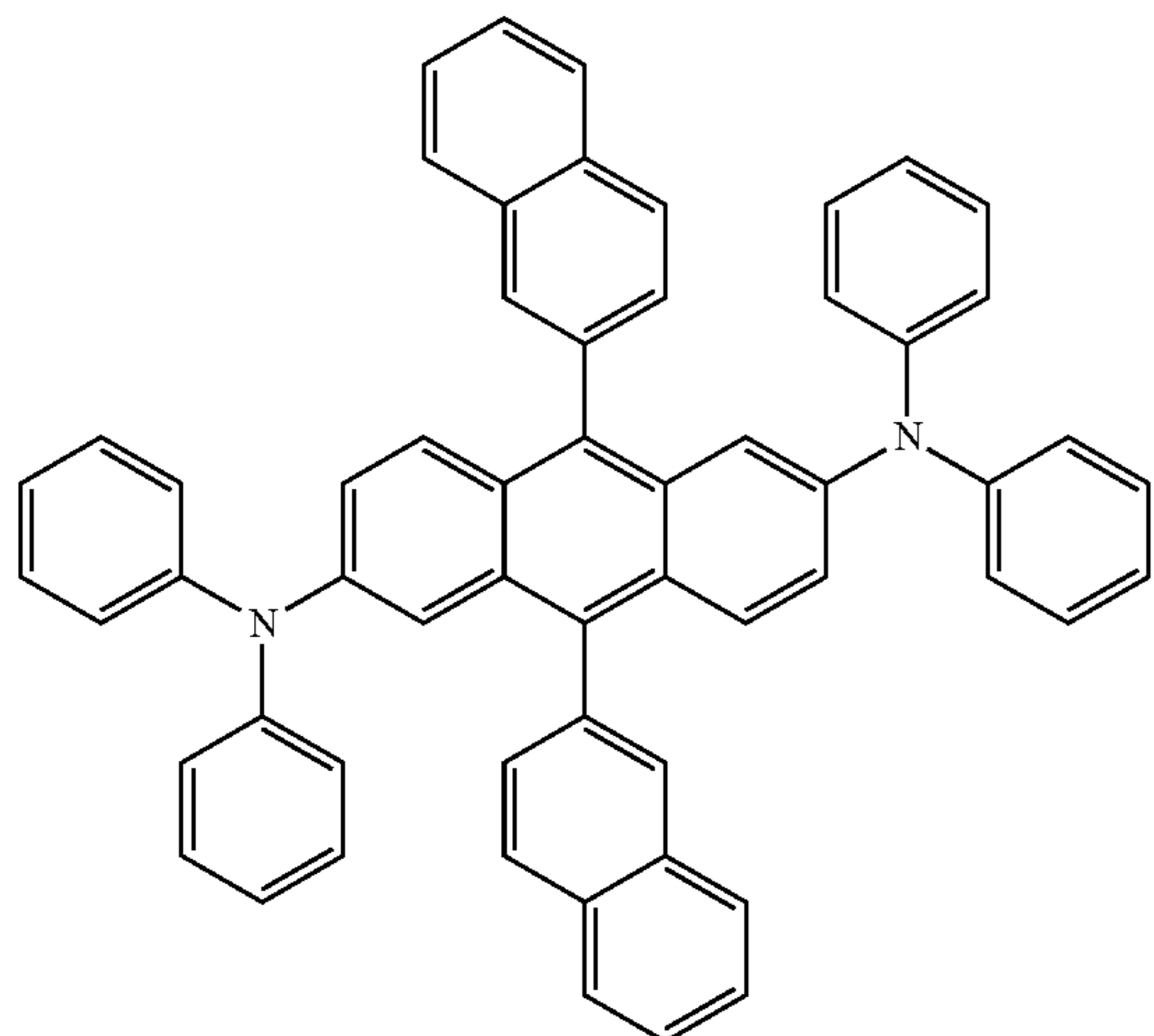
formula EM-4
