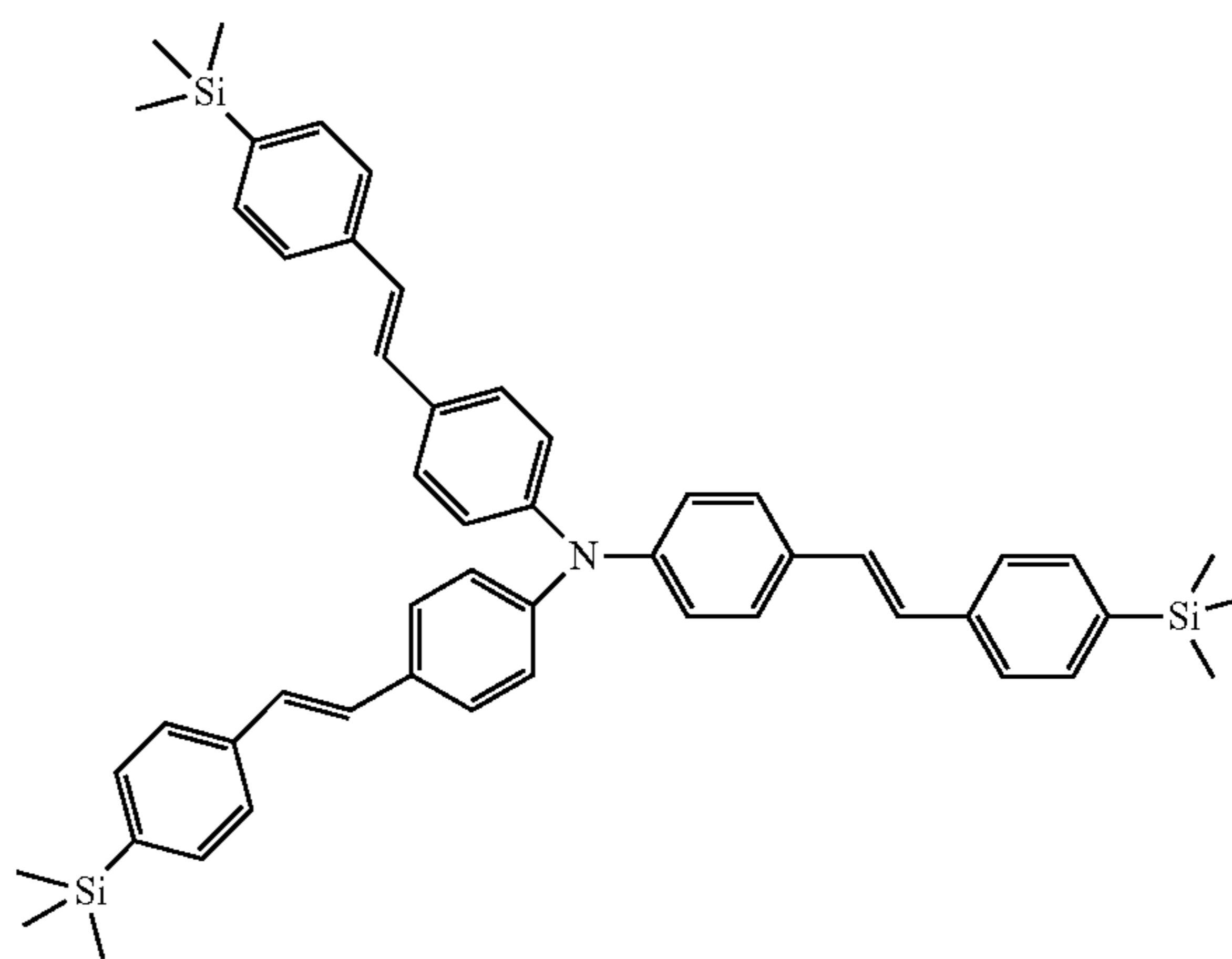
formula EM-2
