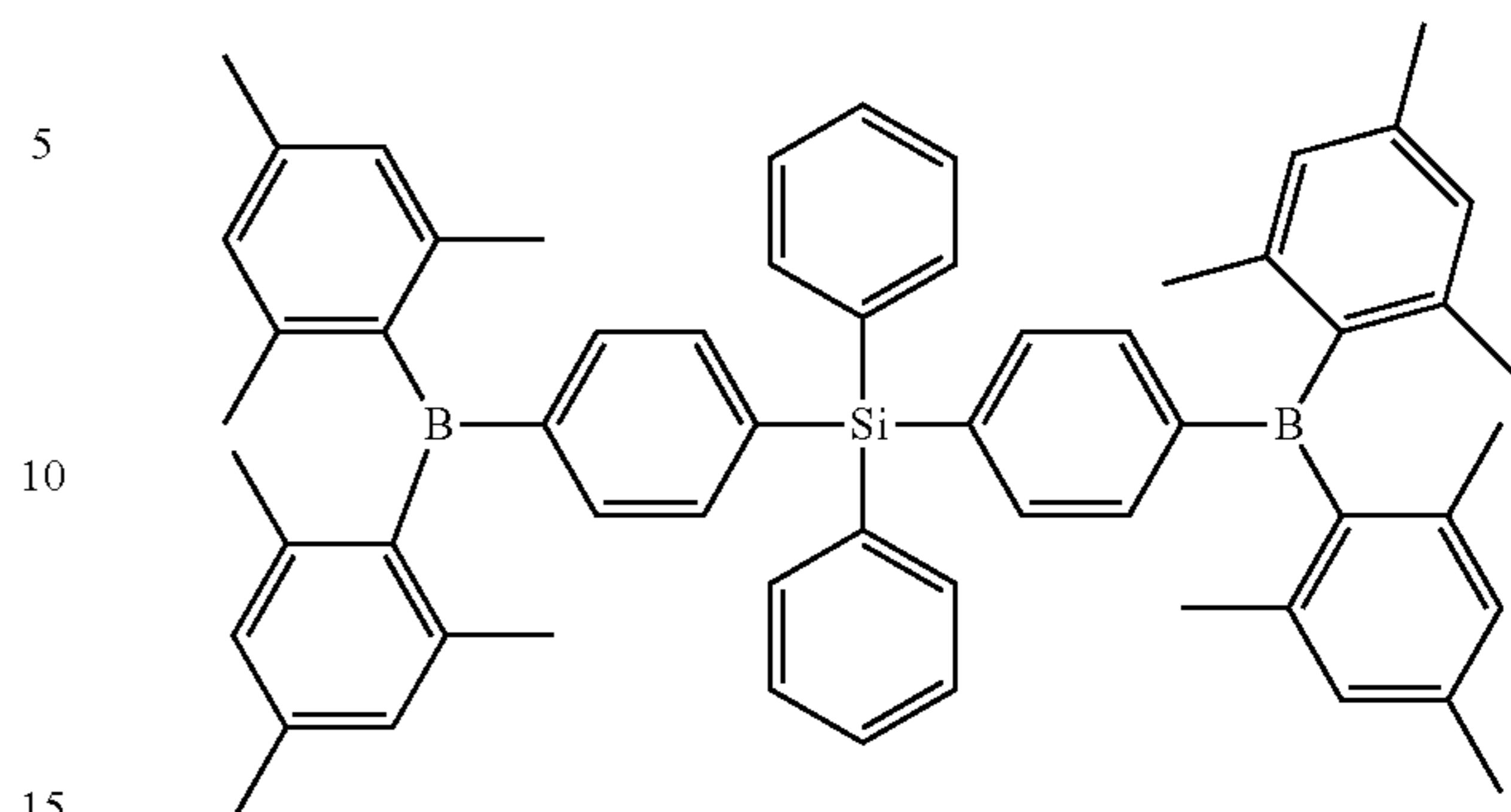
formula ET-4
