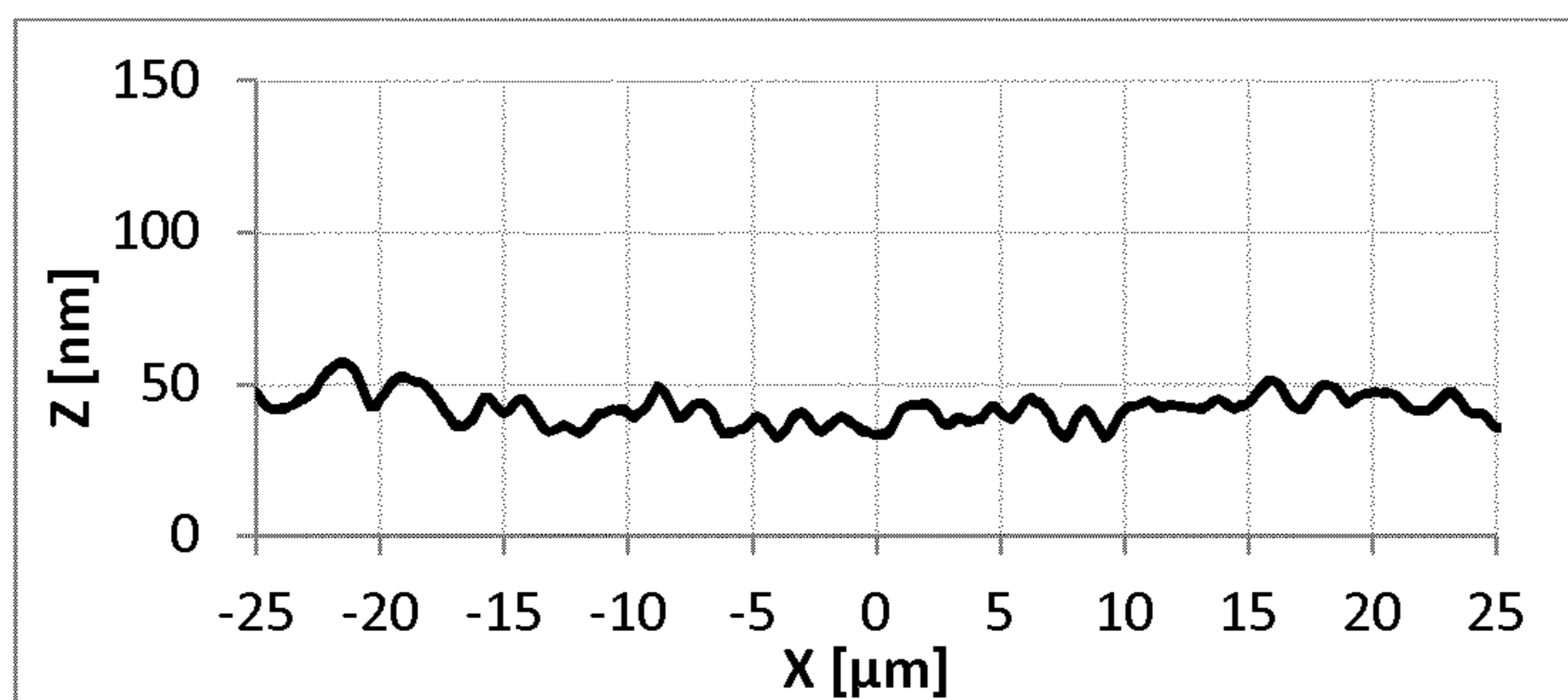
Film profile of the film of Example 1
