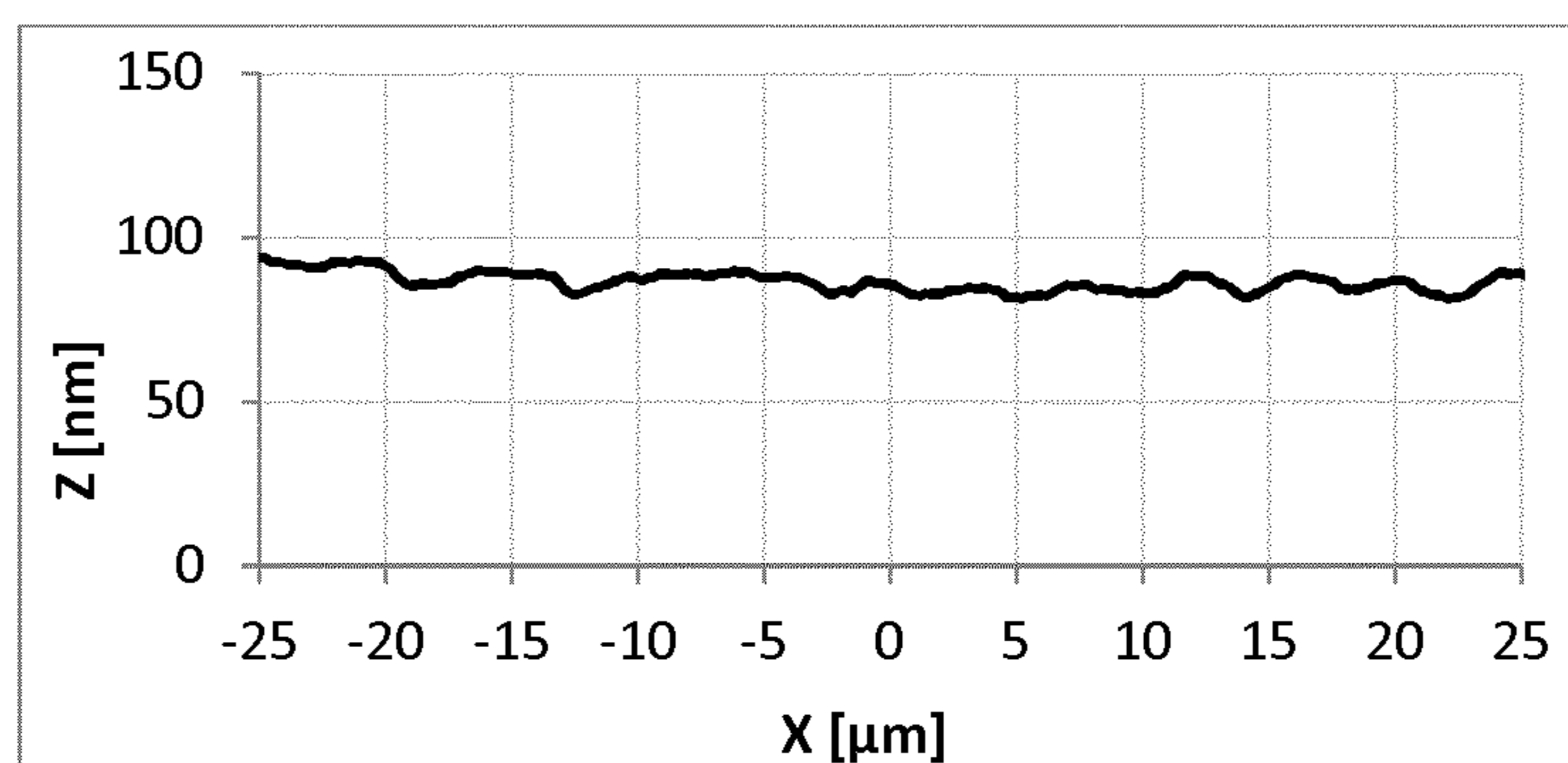
Film profile of the film of Example 4
