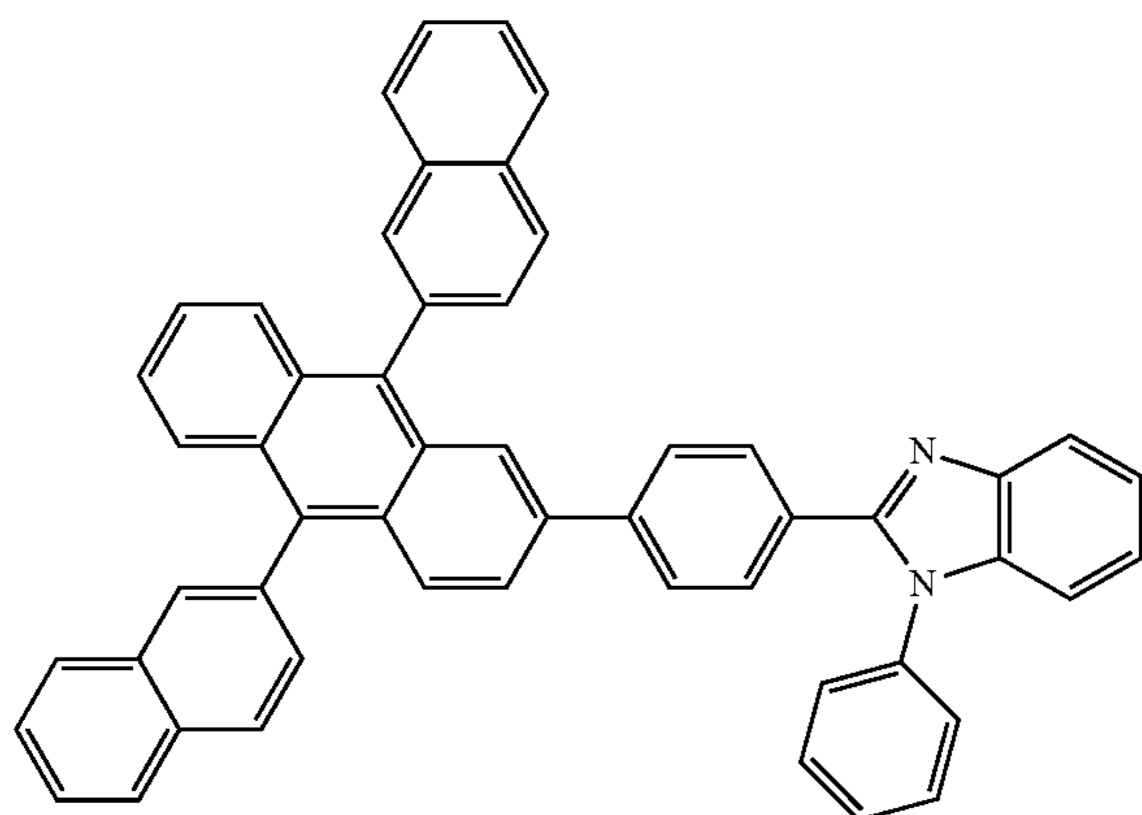
formula ET-11
