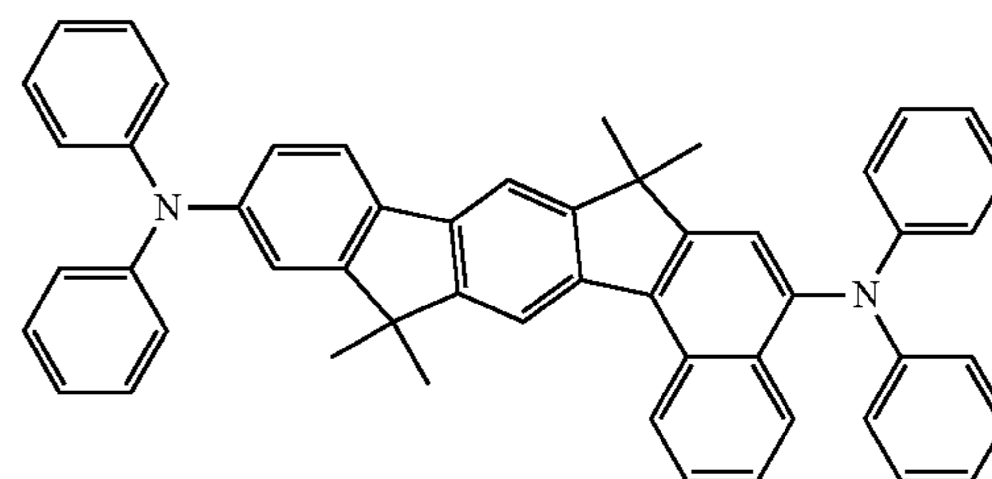
formula EM-9
