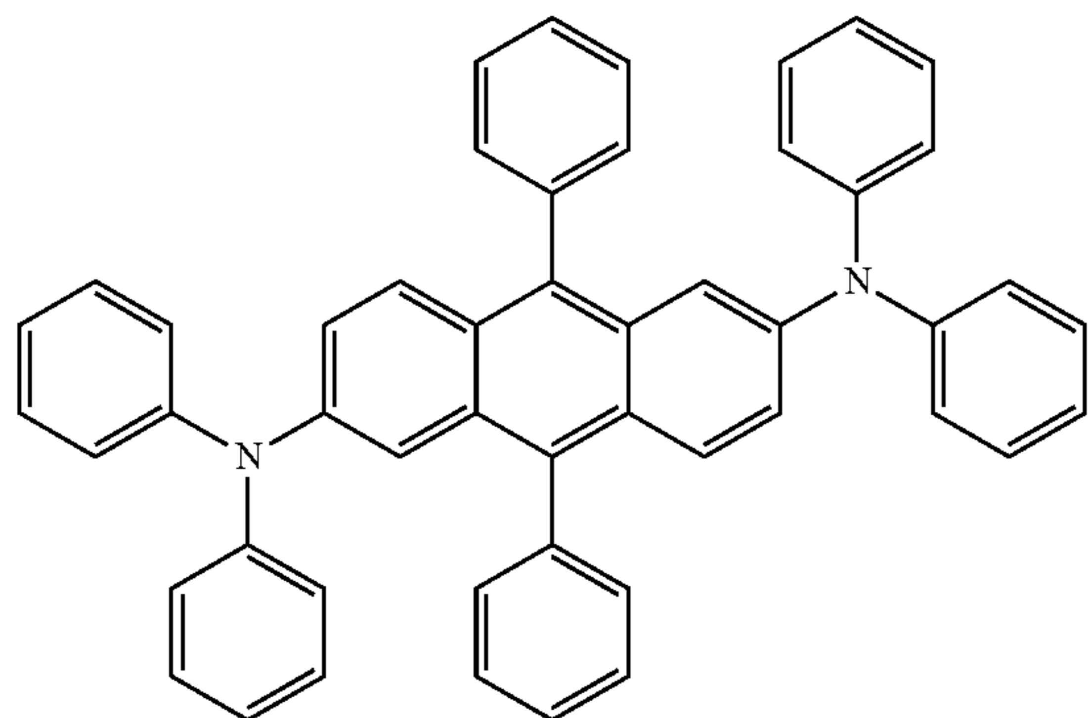
formula EM-3
