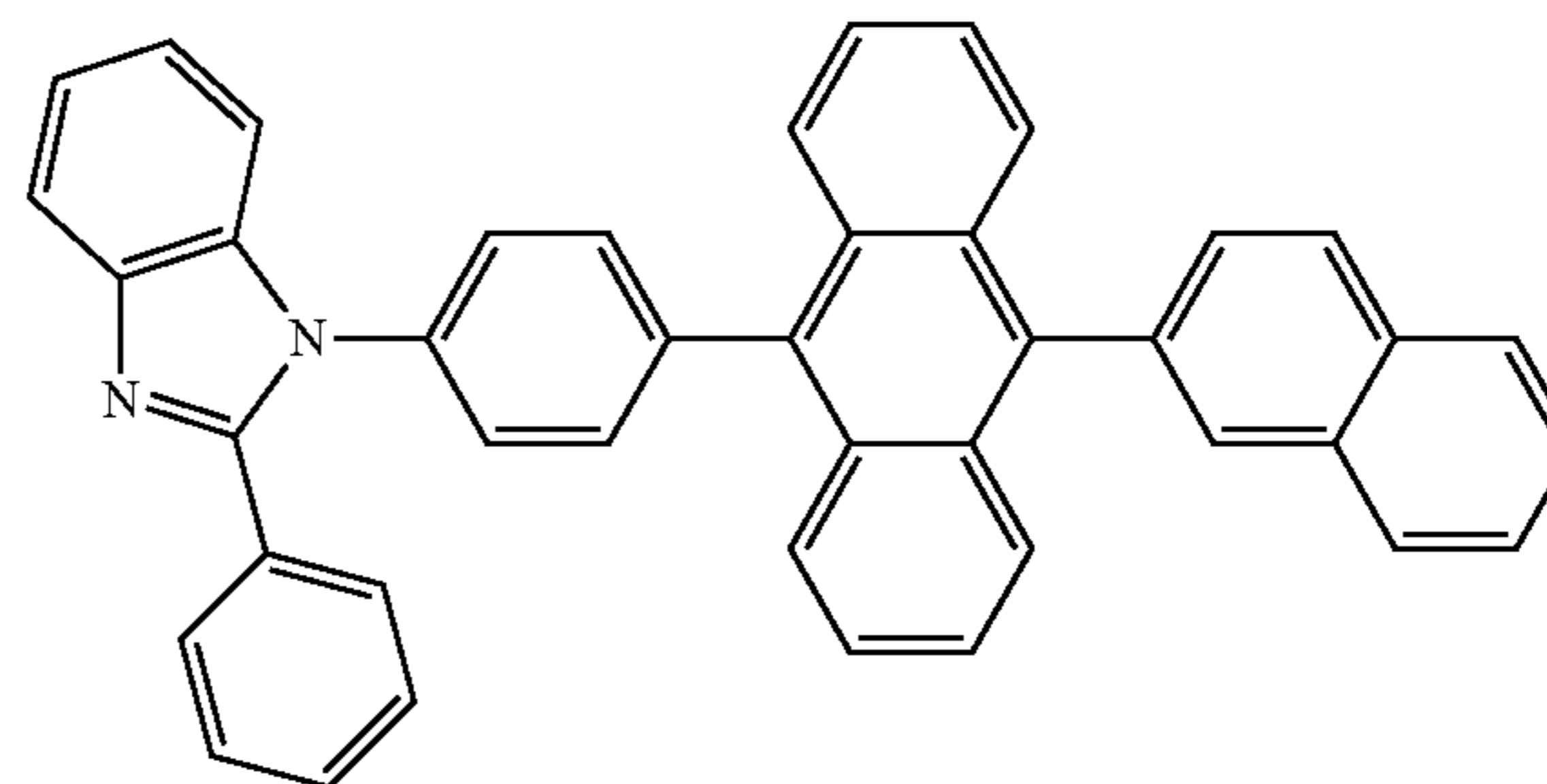
formula ET-13
