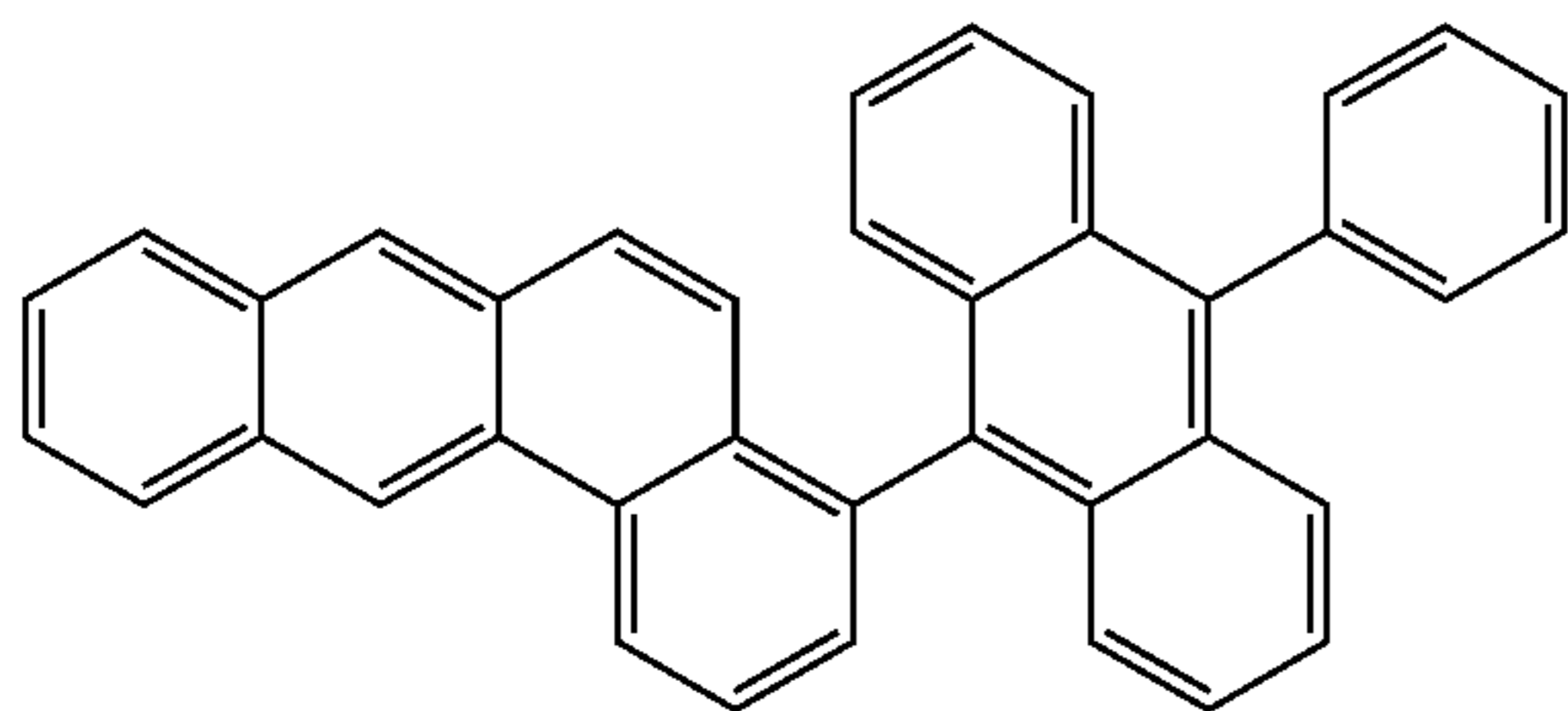
formula H-6
