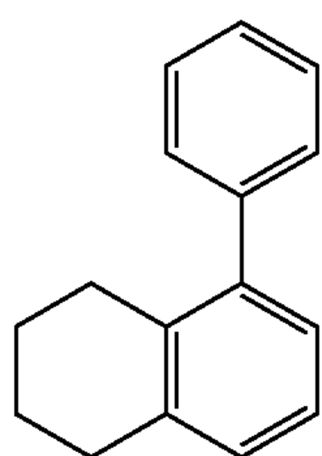
CAS 67064-63-5 1,2,3,4-tetrahydro-5-phenylnaphthalene
