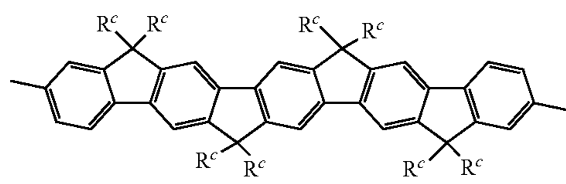
formula PB-1D
