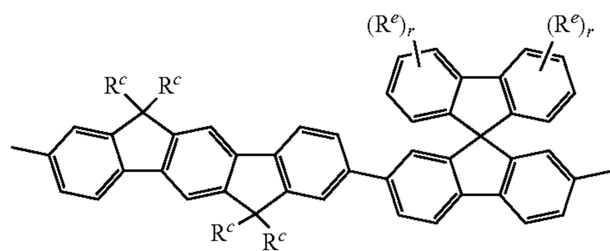
formula PB-1E
