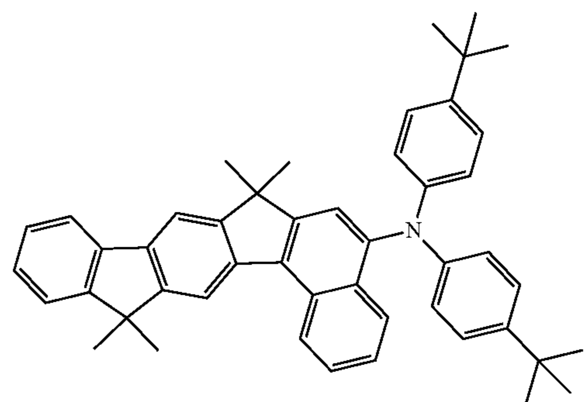
formula EM-9
