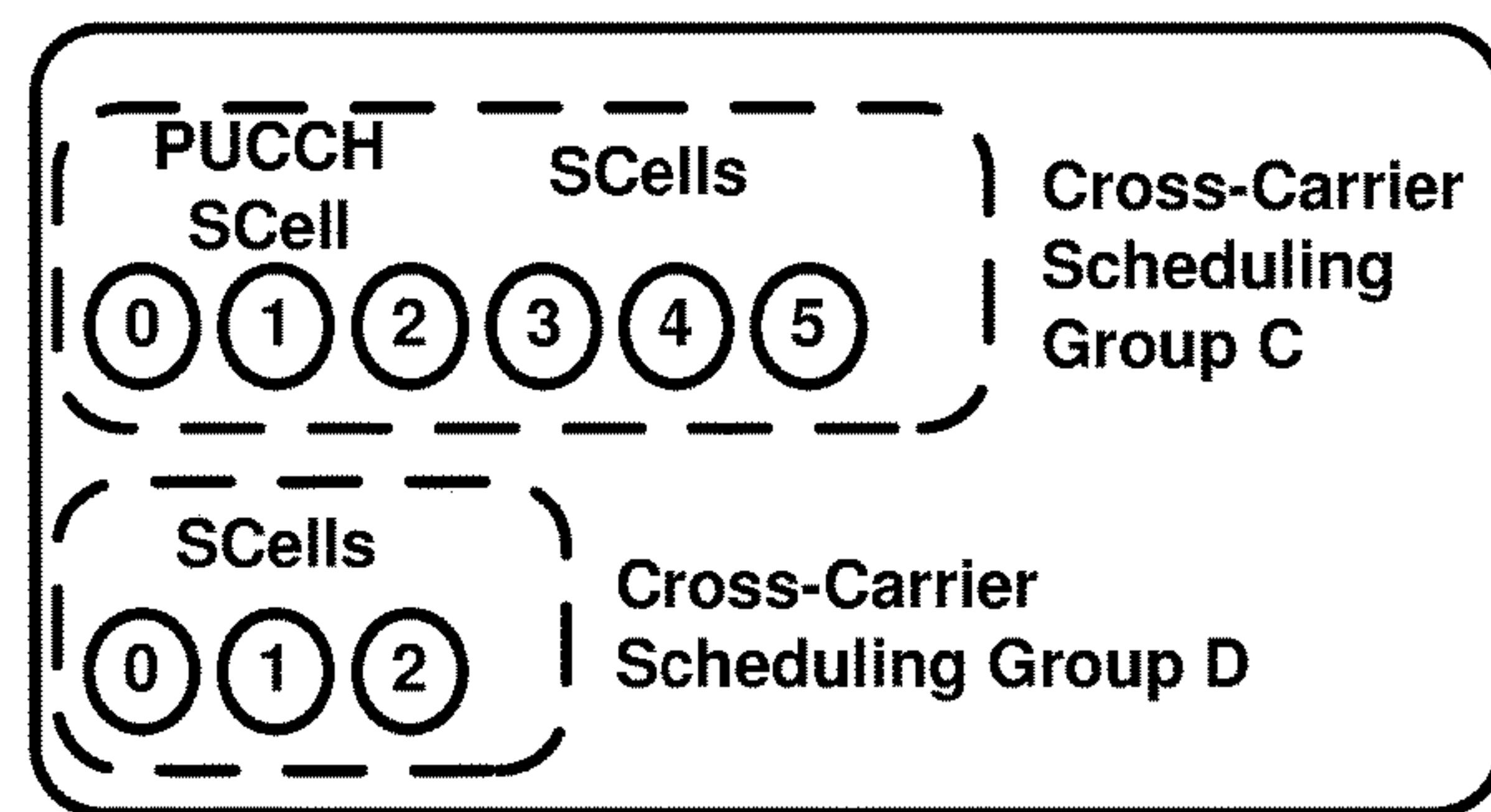
Secondary PUCCH Group
