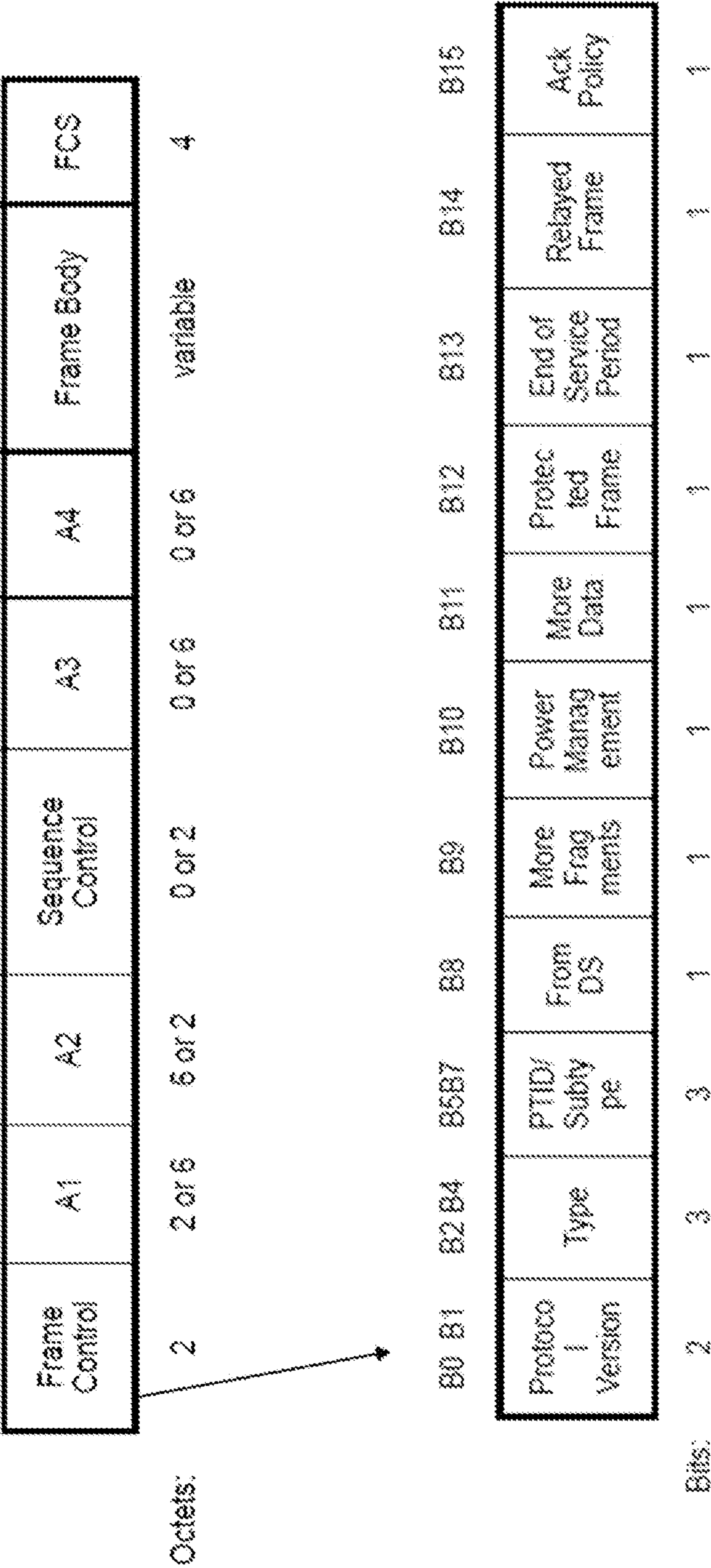
FIG. 22 (PRIOR ART)
