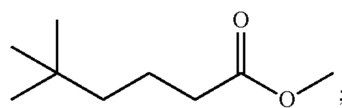
methyl 5,5-dimethylhexanoate
