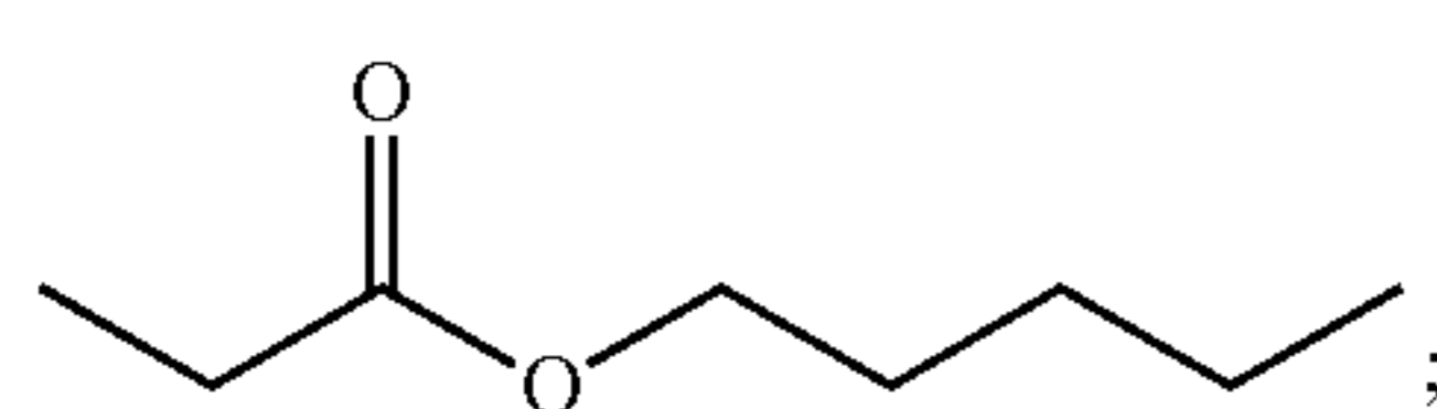
pentyl propionate
