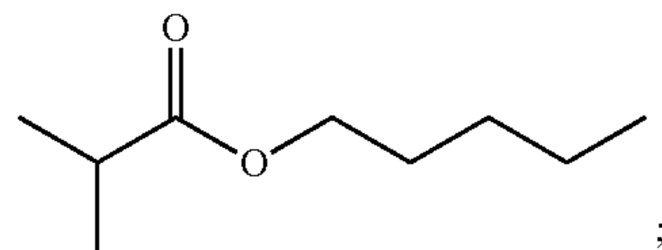
pentyl isobutyrate
