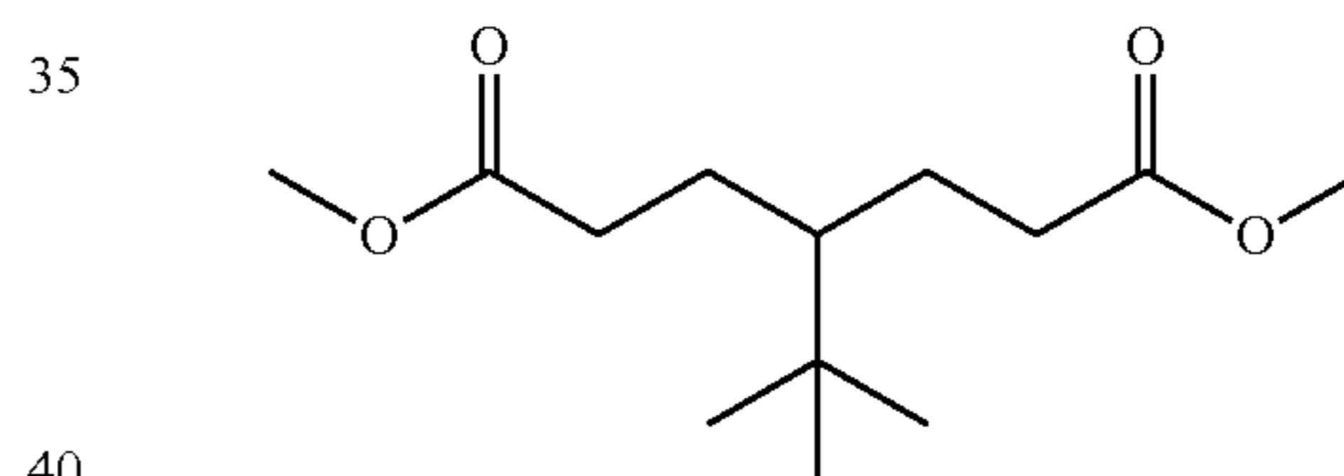
dimethyl 4-(tert-butyl)heptanedioate
