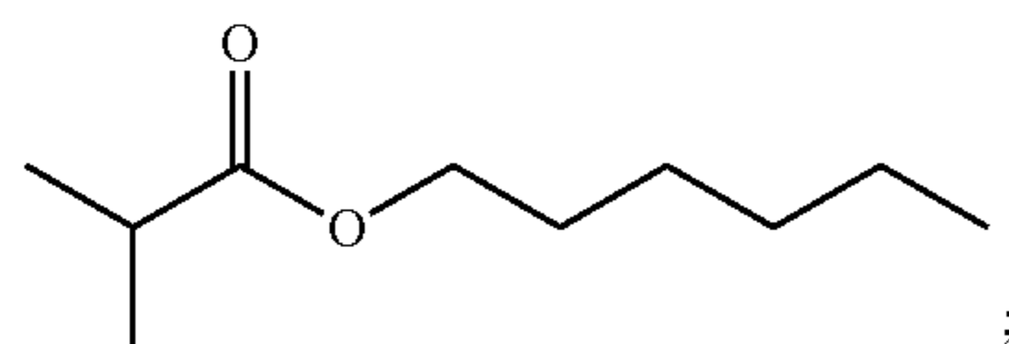
hexyl isobutyrate
