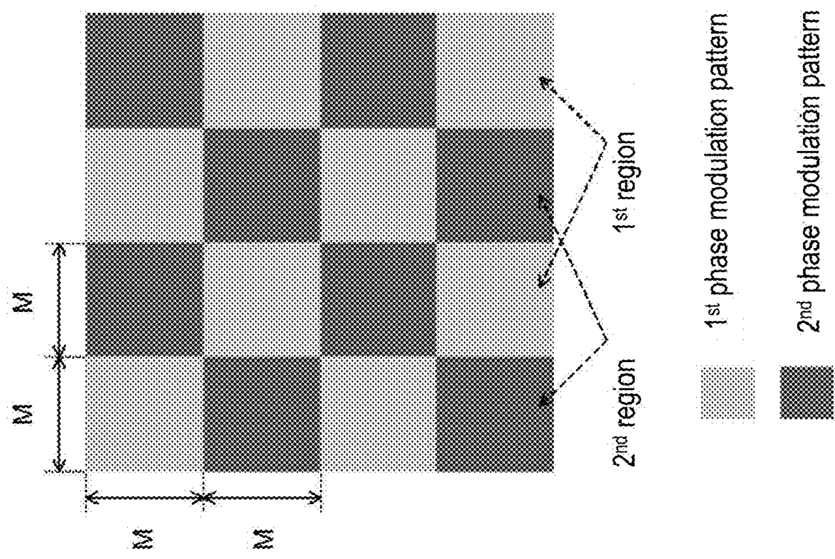
FIG. 14 (a) Phase modulation pattern example 2
