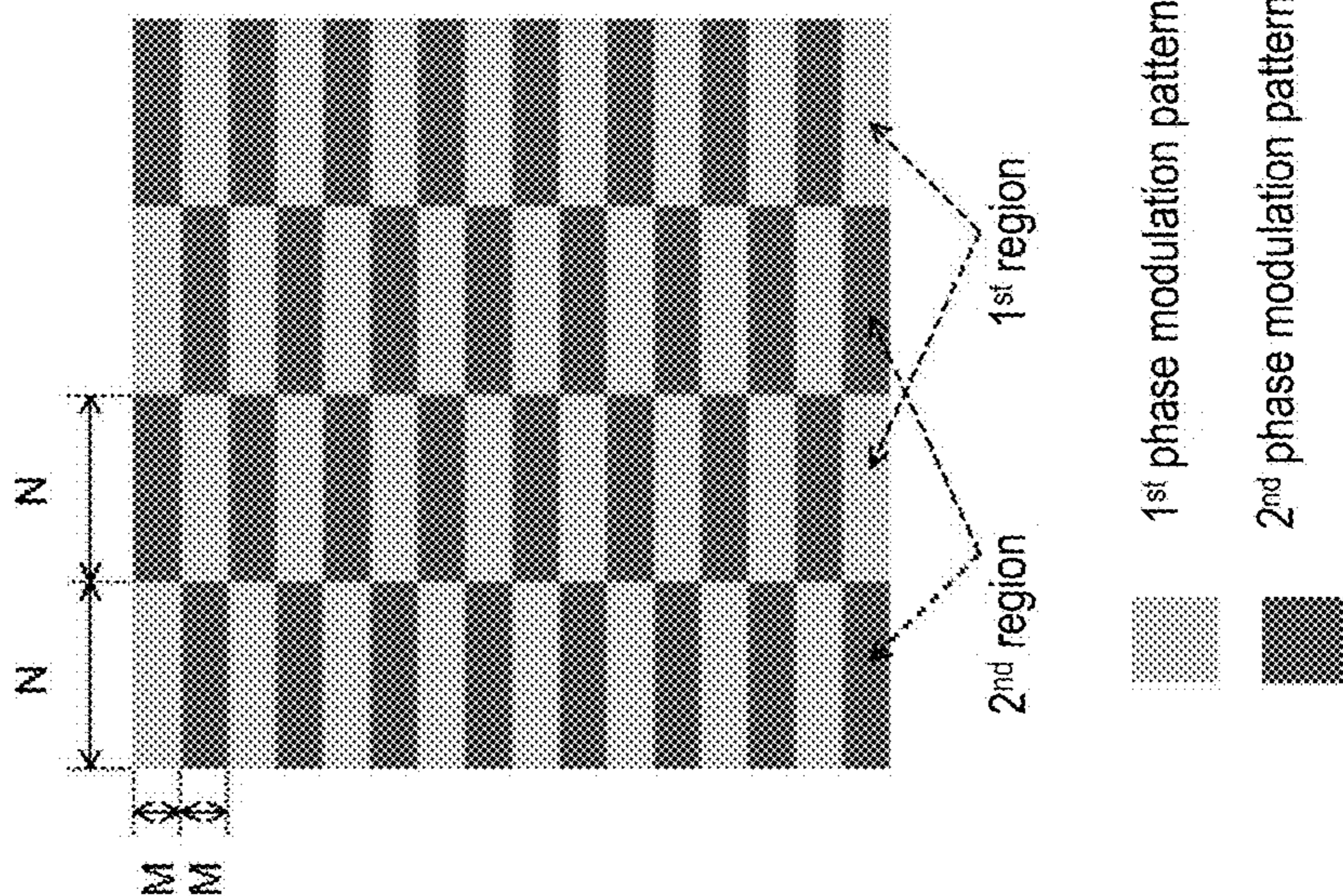
FIG. 17 (a) Phase modulation pattern example 3
