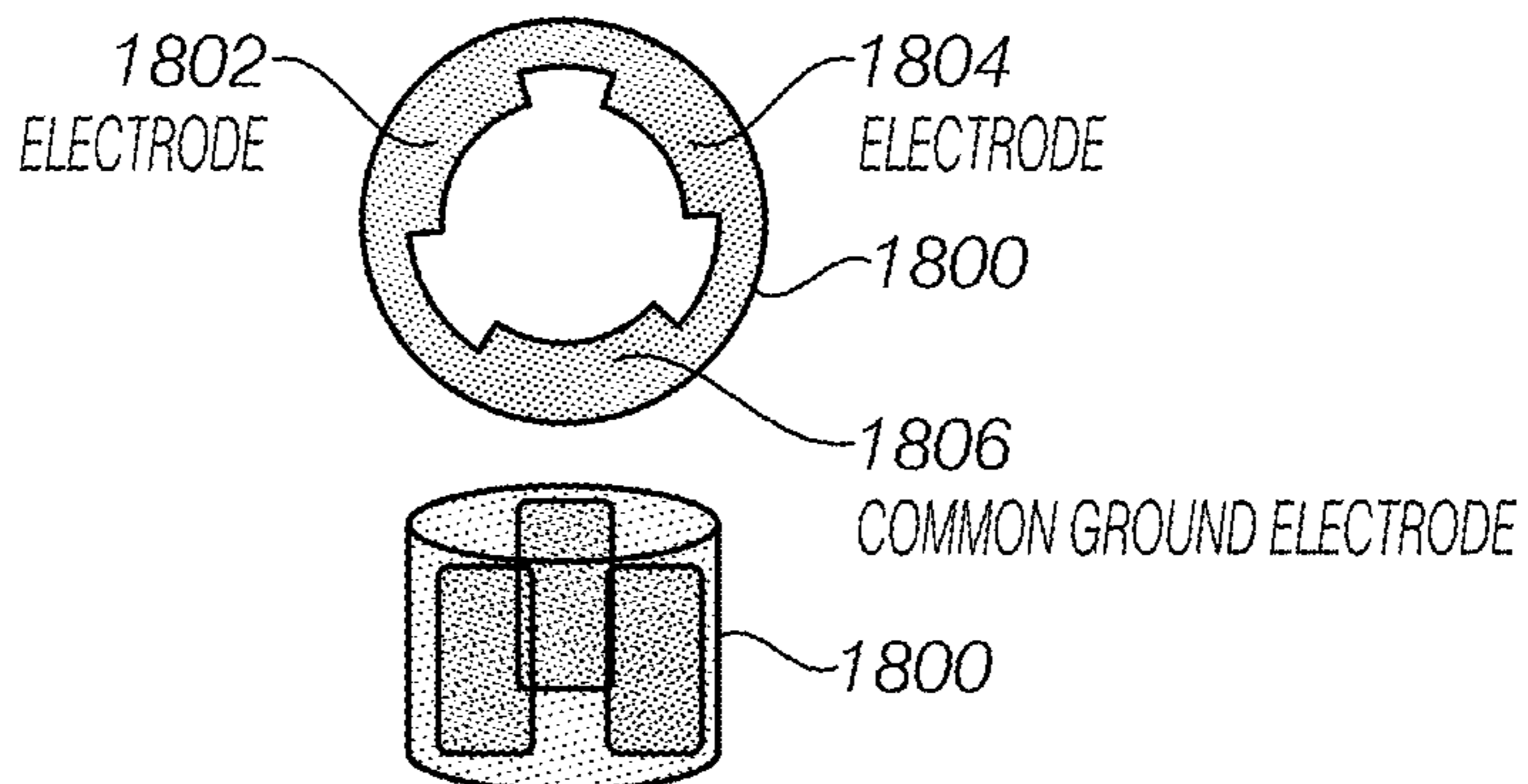
RING WITH 3 ELECTRODES
