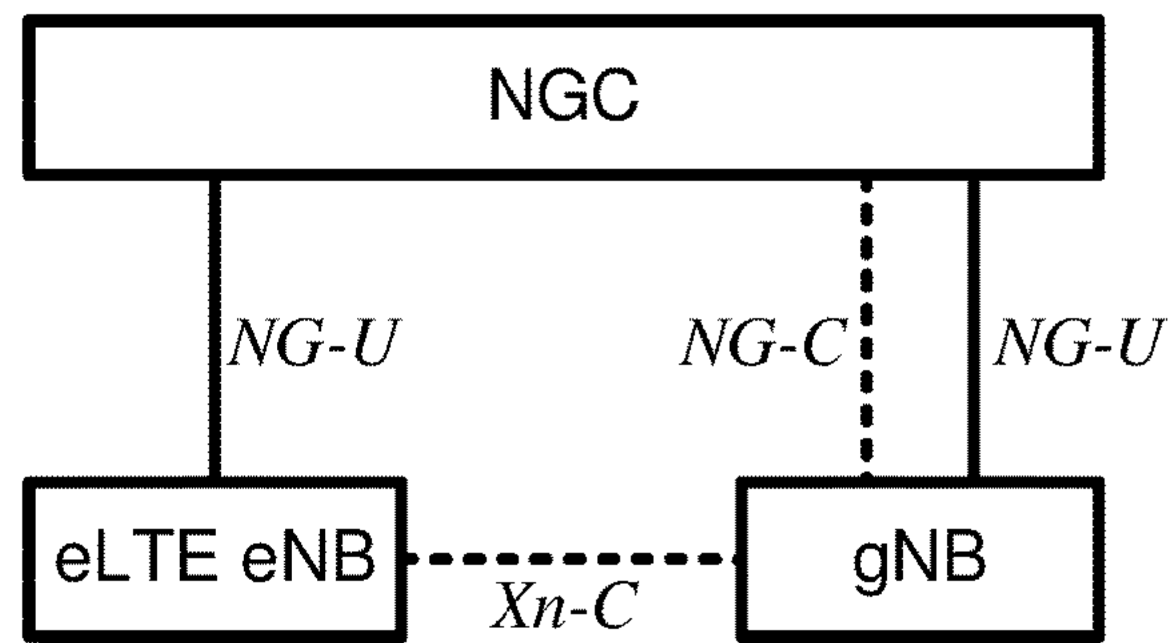
gNB connected to NGC with non-standalone eLTE eNB. eLTE eNB user plane connected to NGC directly.
