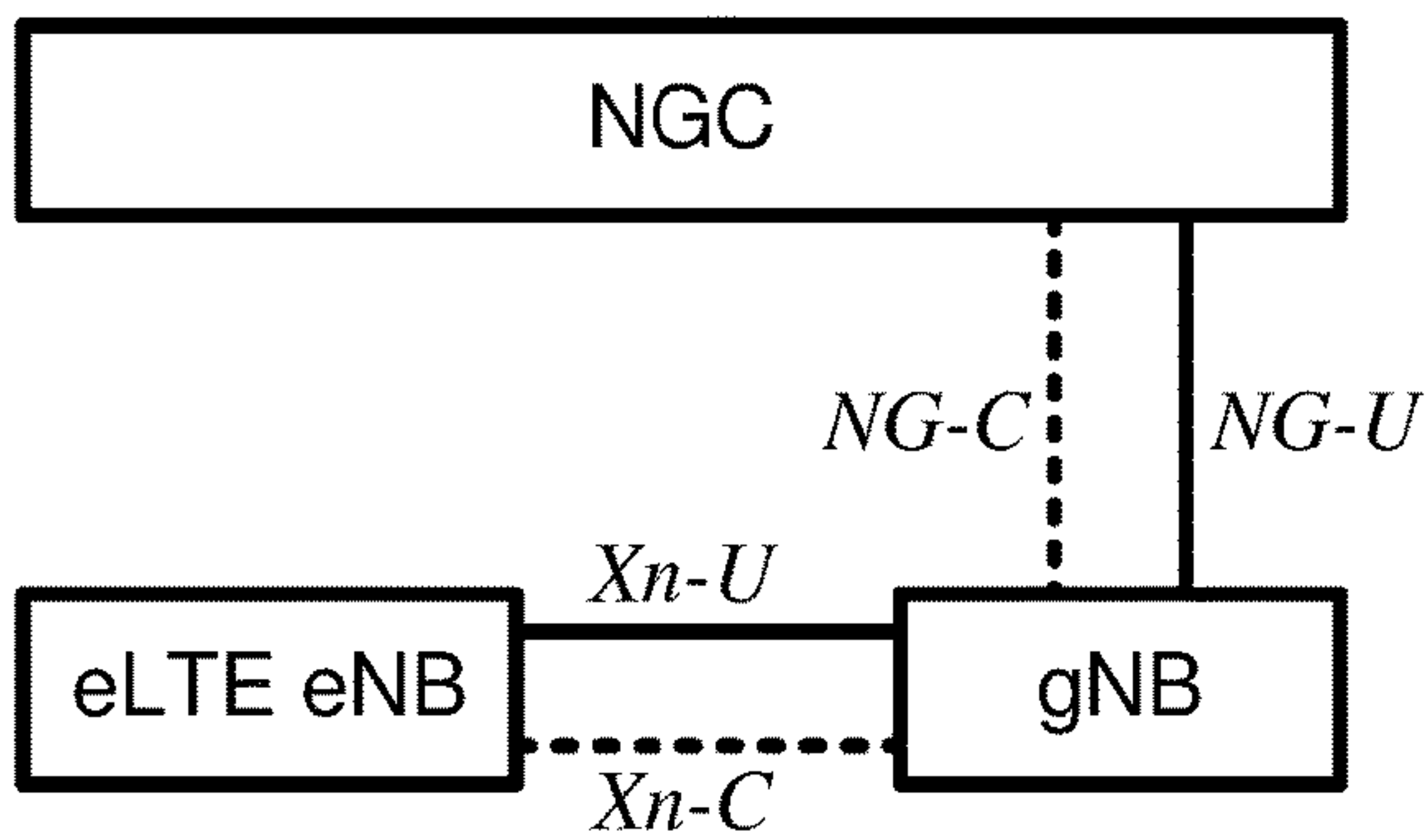
gNB connected to NGC with non-standalone eLTE eNB. eLTE eNB user plane connected to NGC via gNB.
