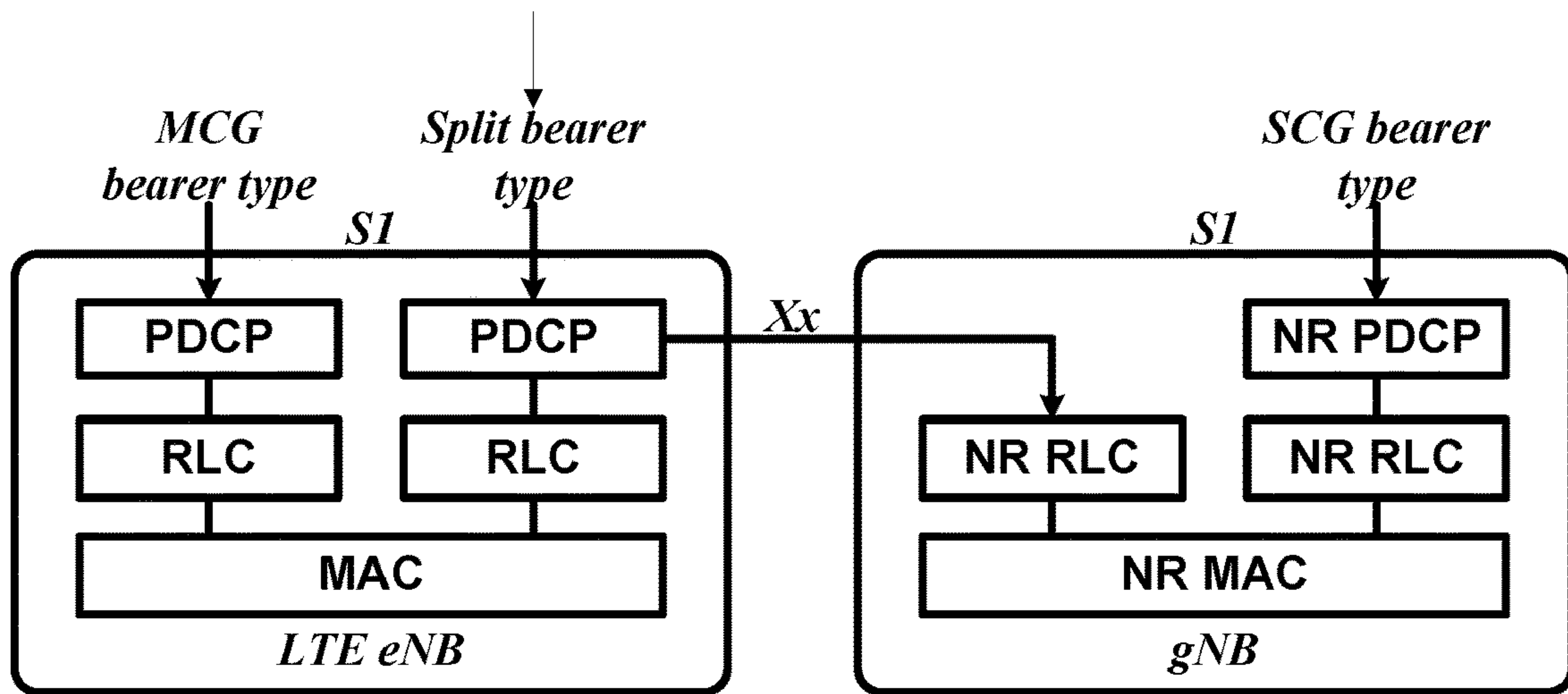
Radio protocol architecture for split bearer and SCG bearer. LTE eNB connected to EPC with non-standalone gNB.
