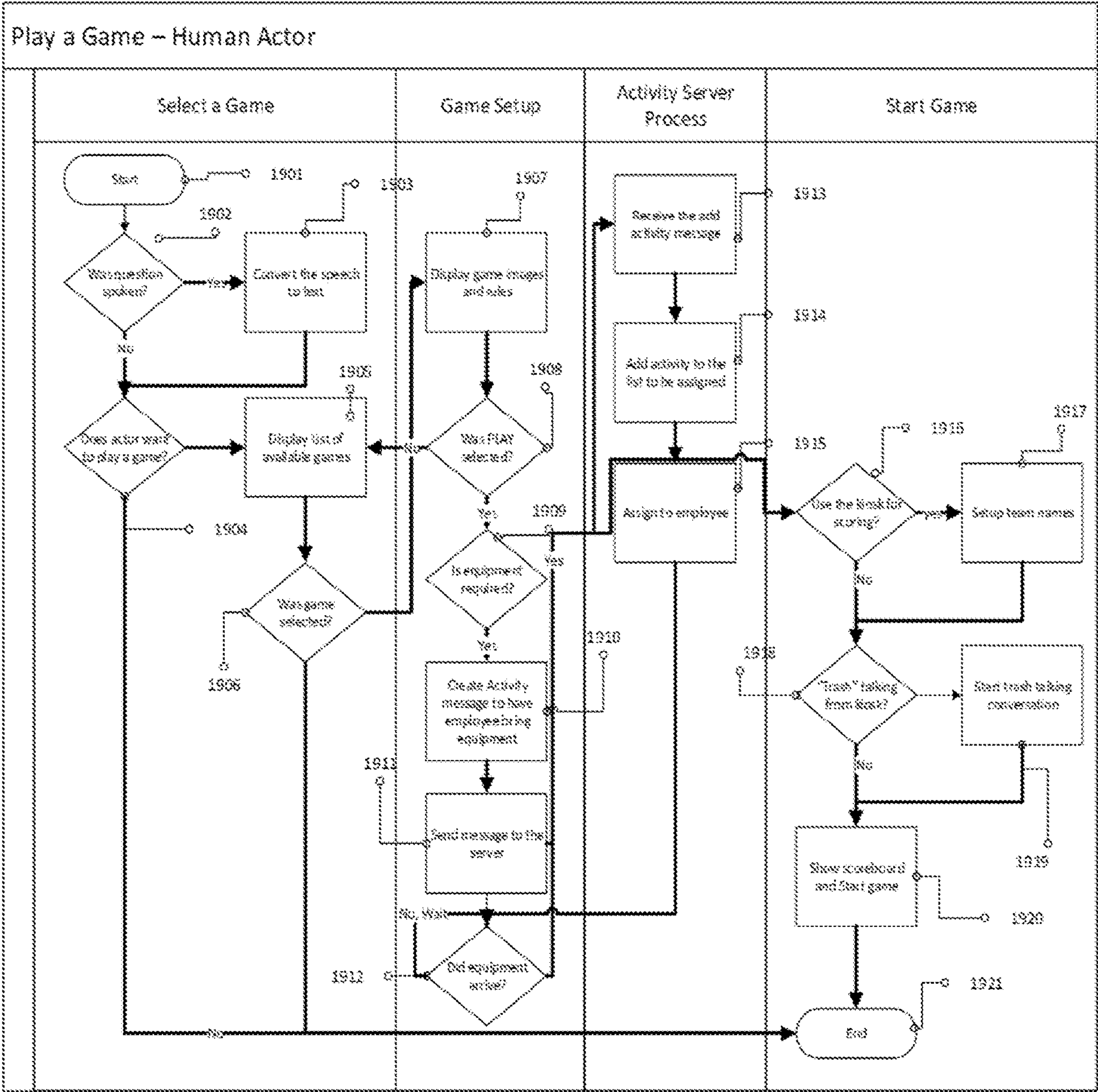
FIG. 19 Play a Game – Human Actor
