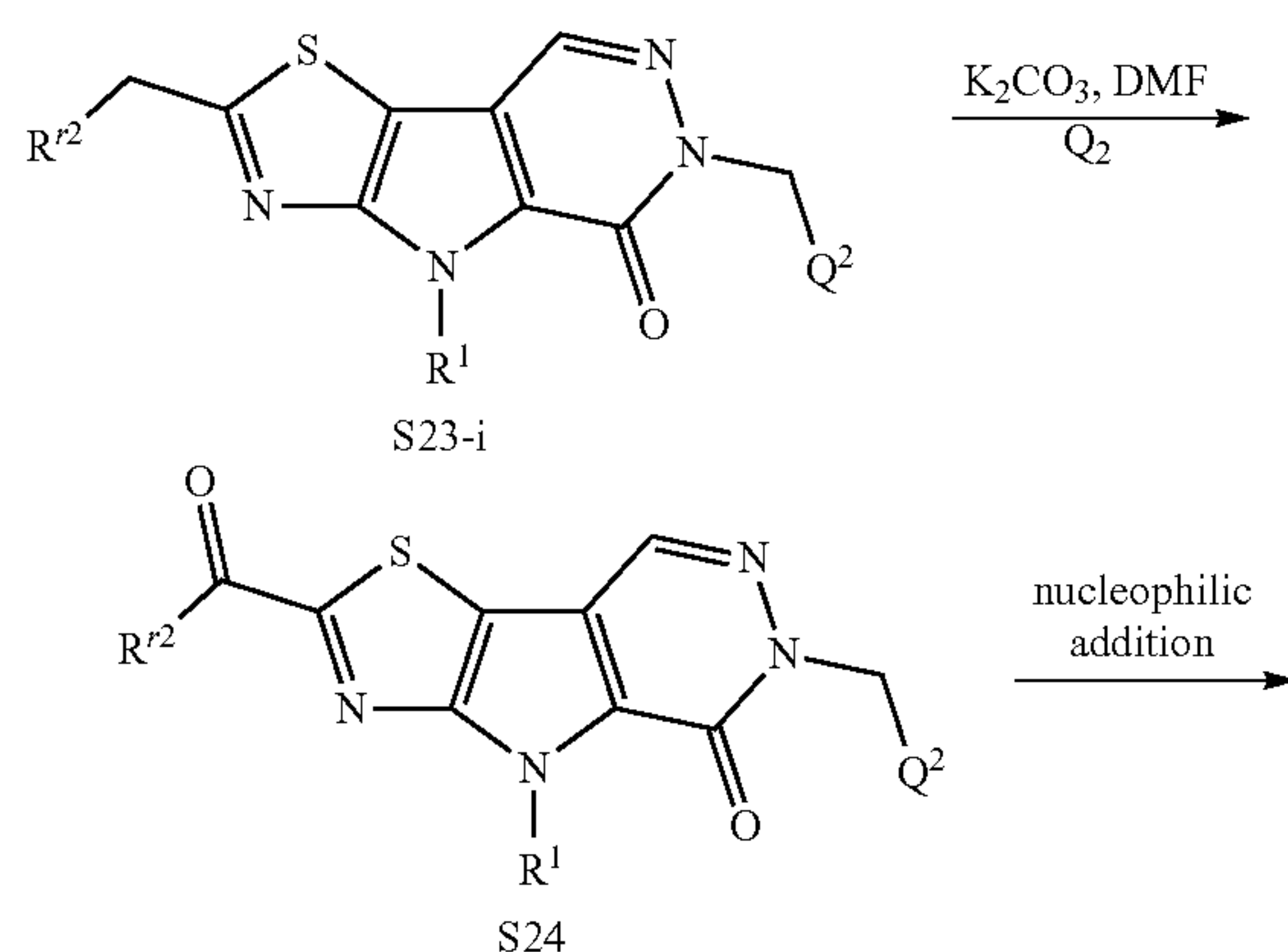
Scheme 3
