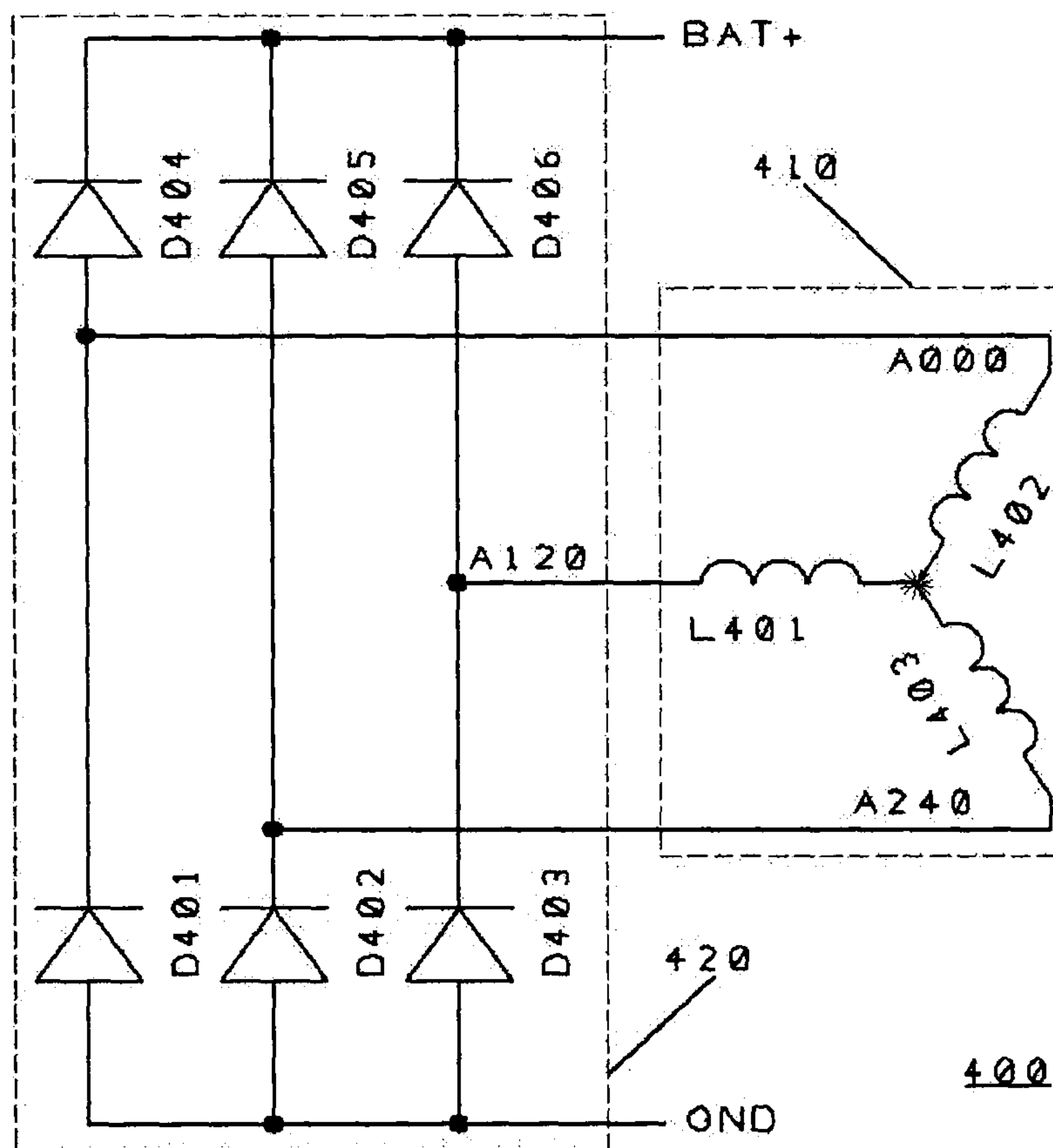
FIG. 4 PRIOR ART
