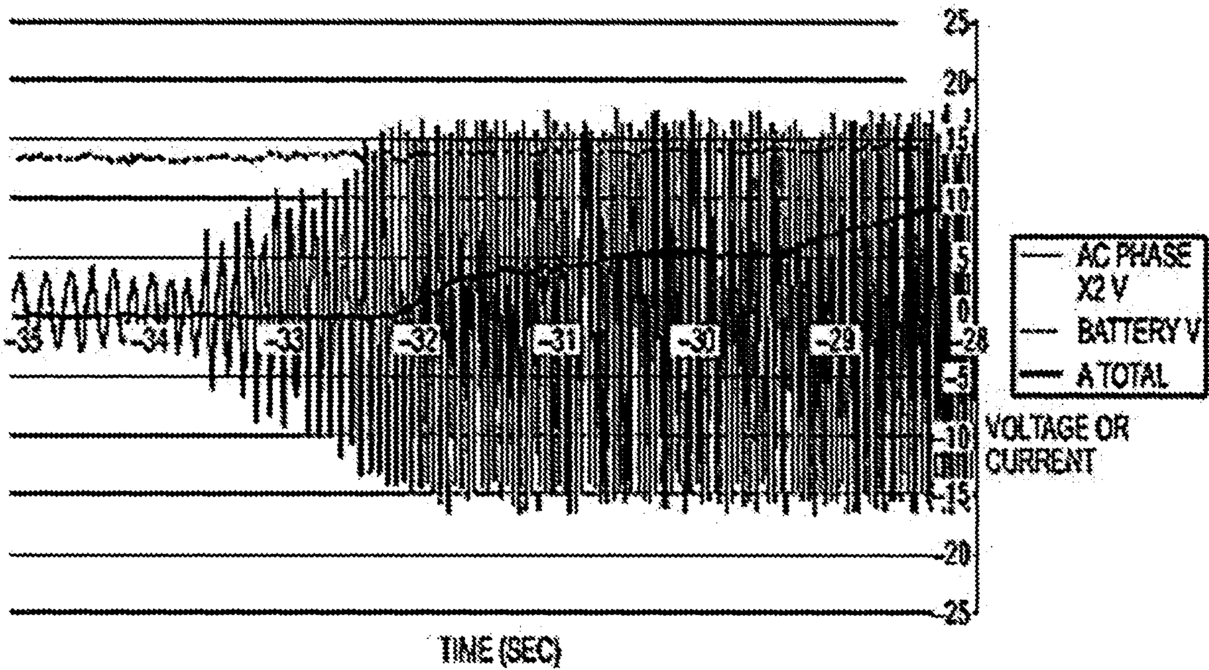
FIG. 2 PRIOR ART
