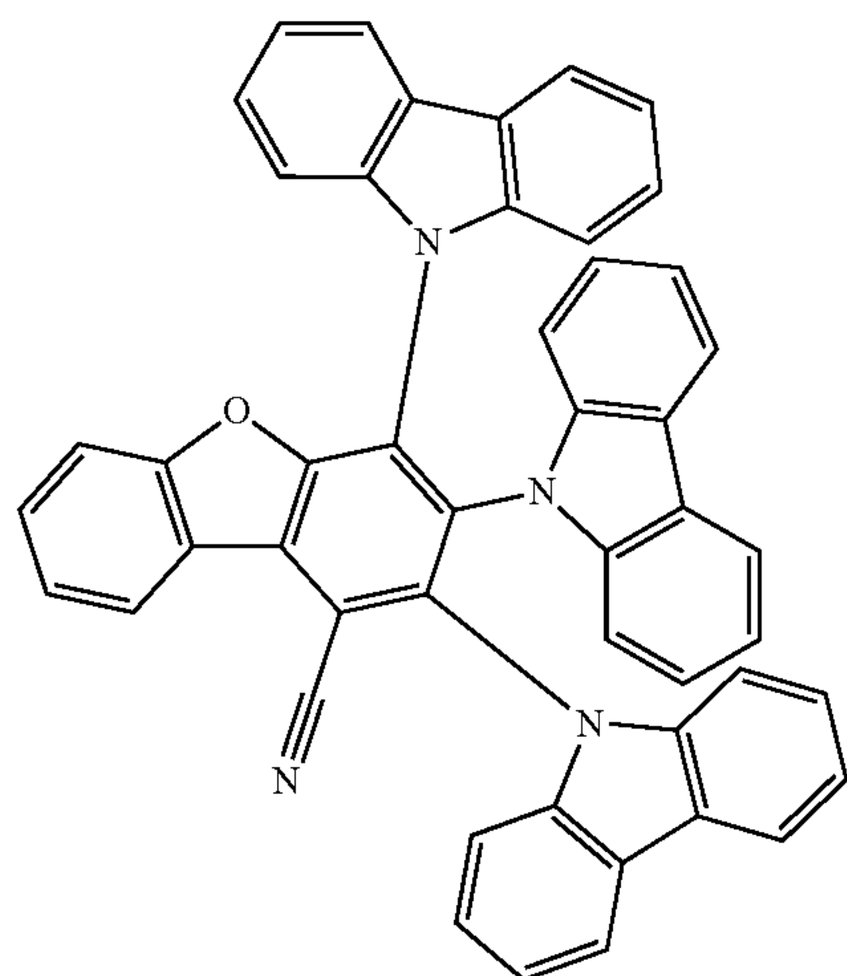
Compound 3
