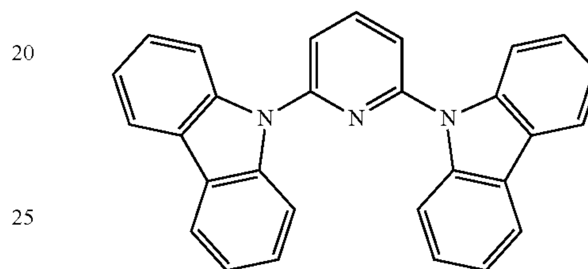
PDY2Cz
