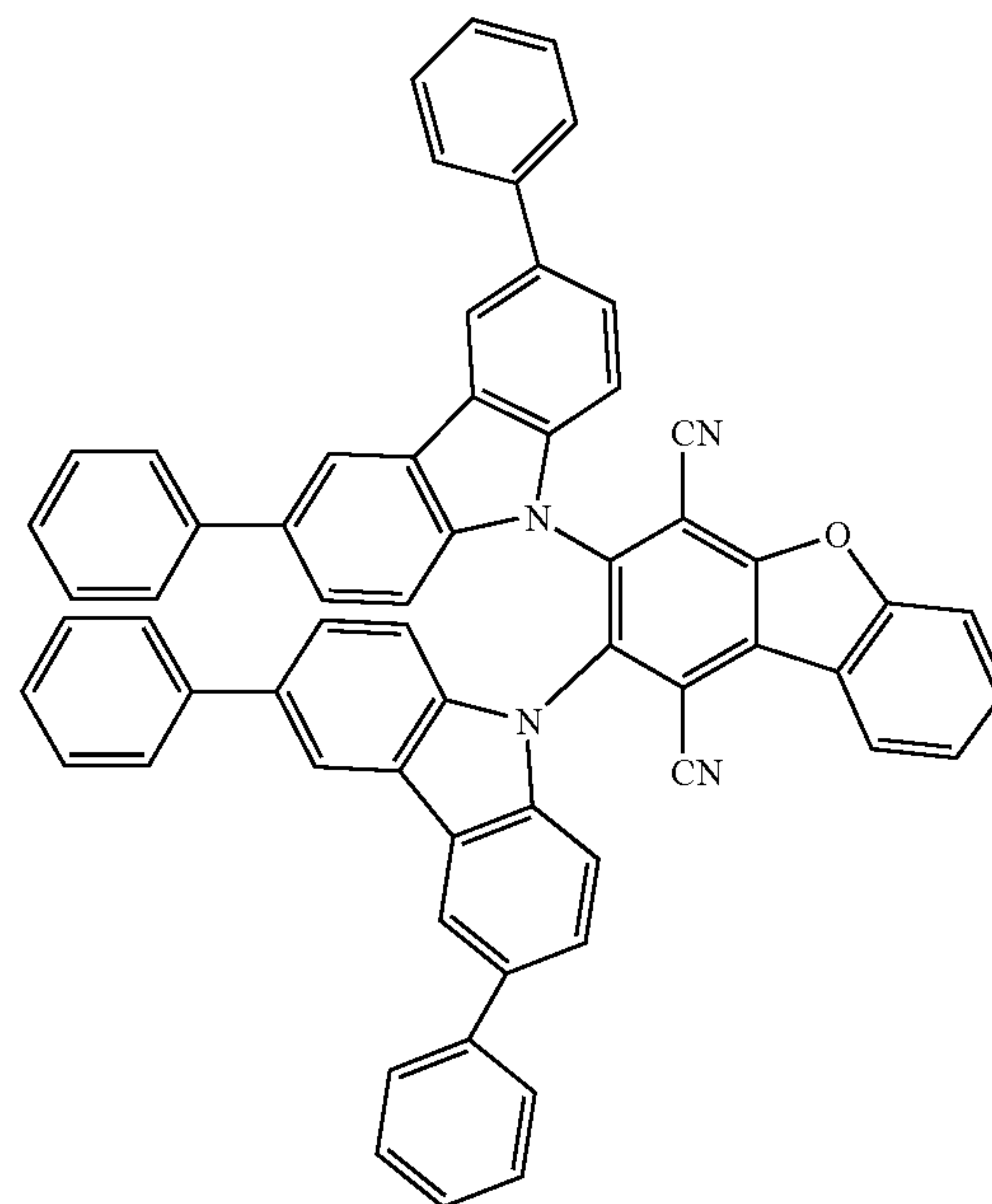
Compound 7
