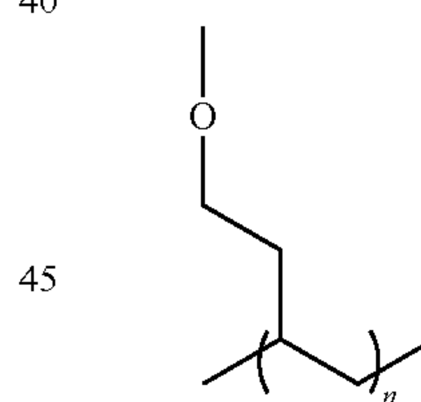
Formula (A)
