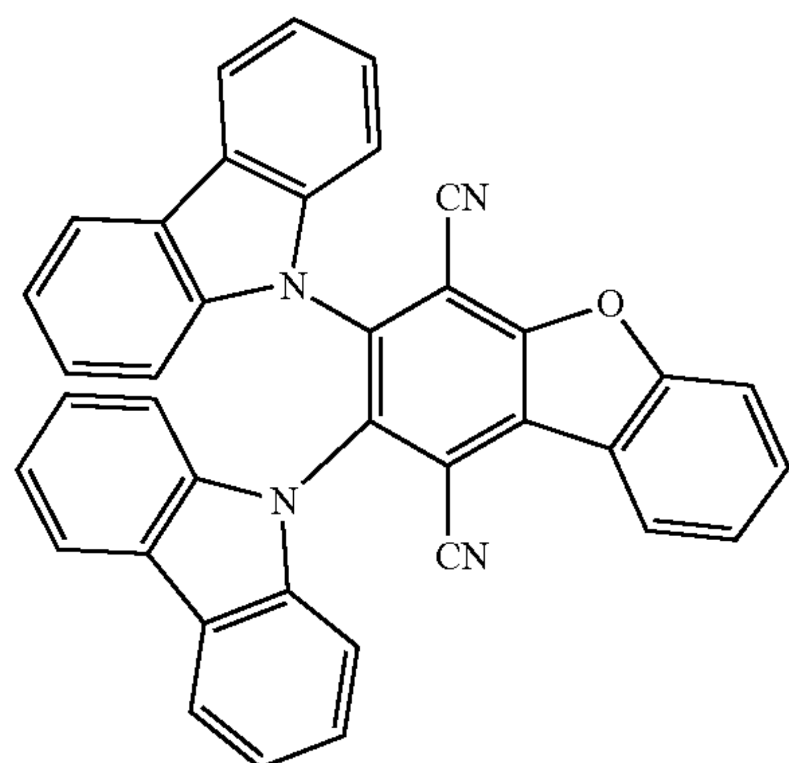
Compound 6
