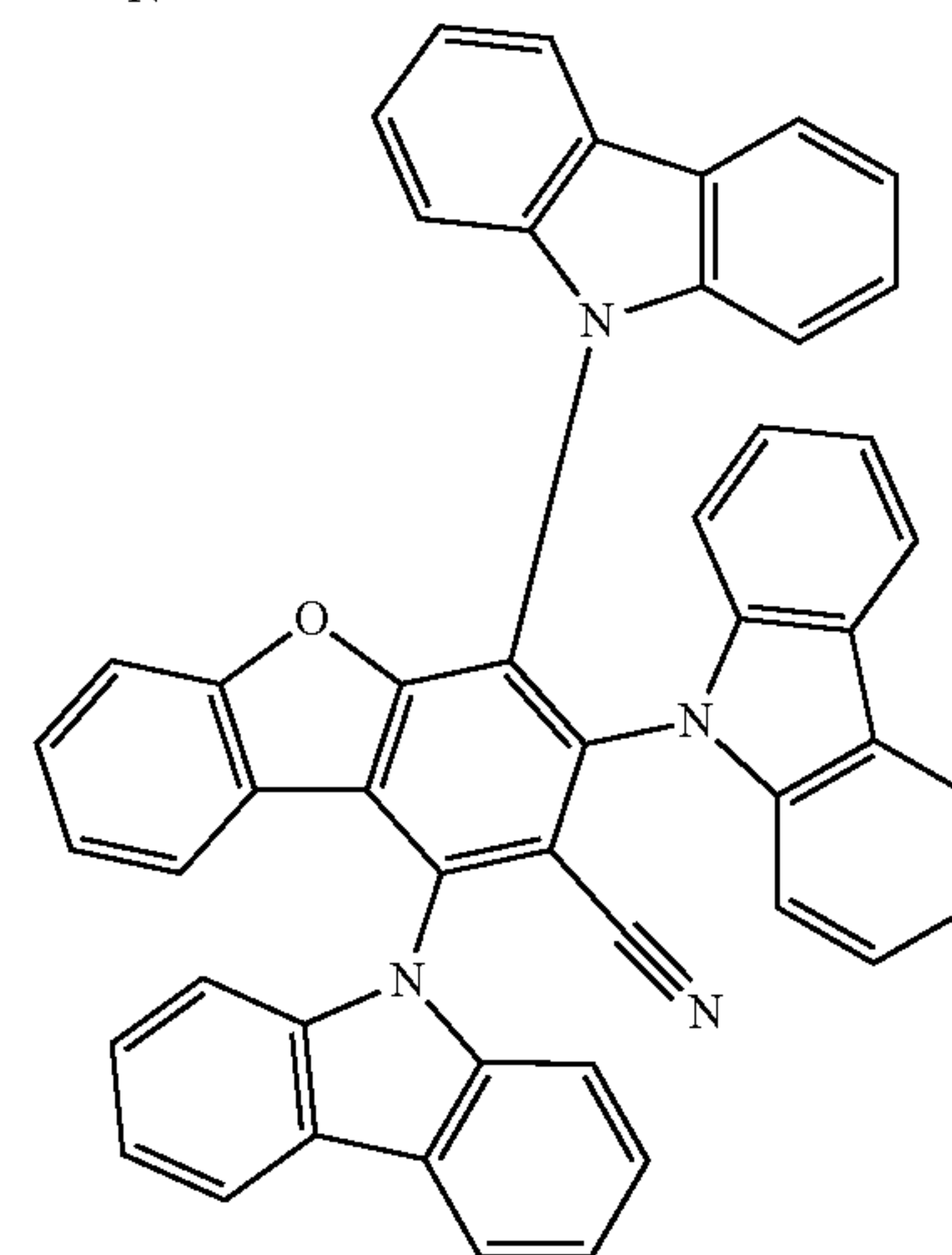
Compound 4
