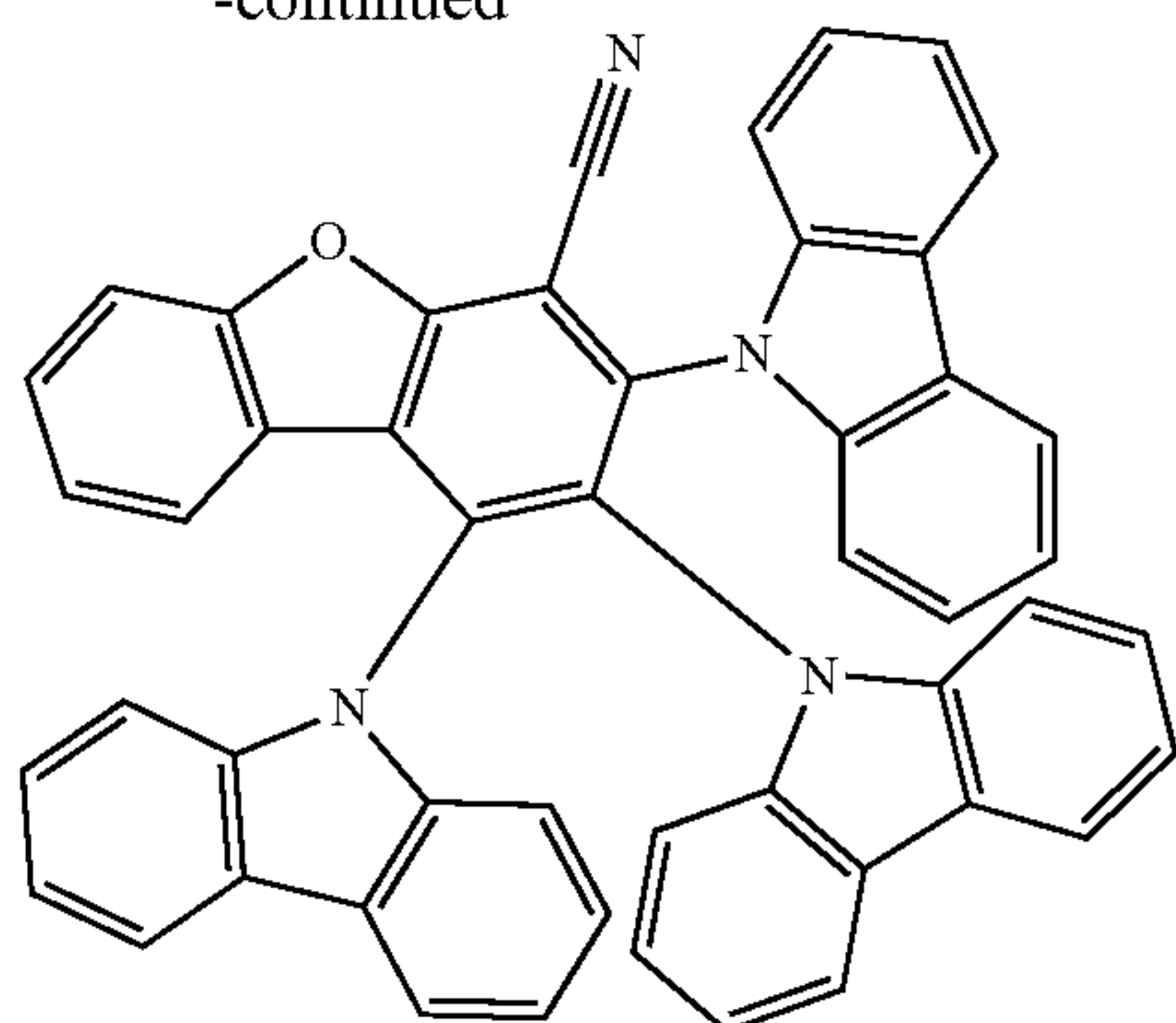
Compound 2
