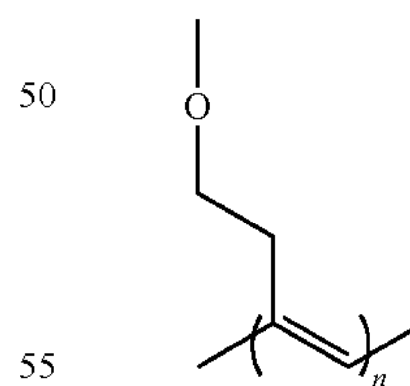
Formula (B)
