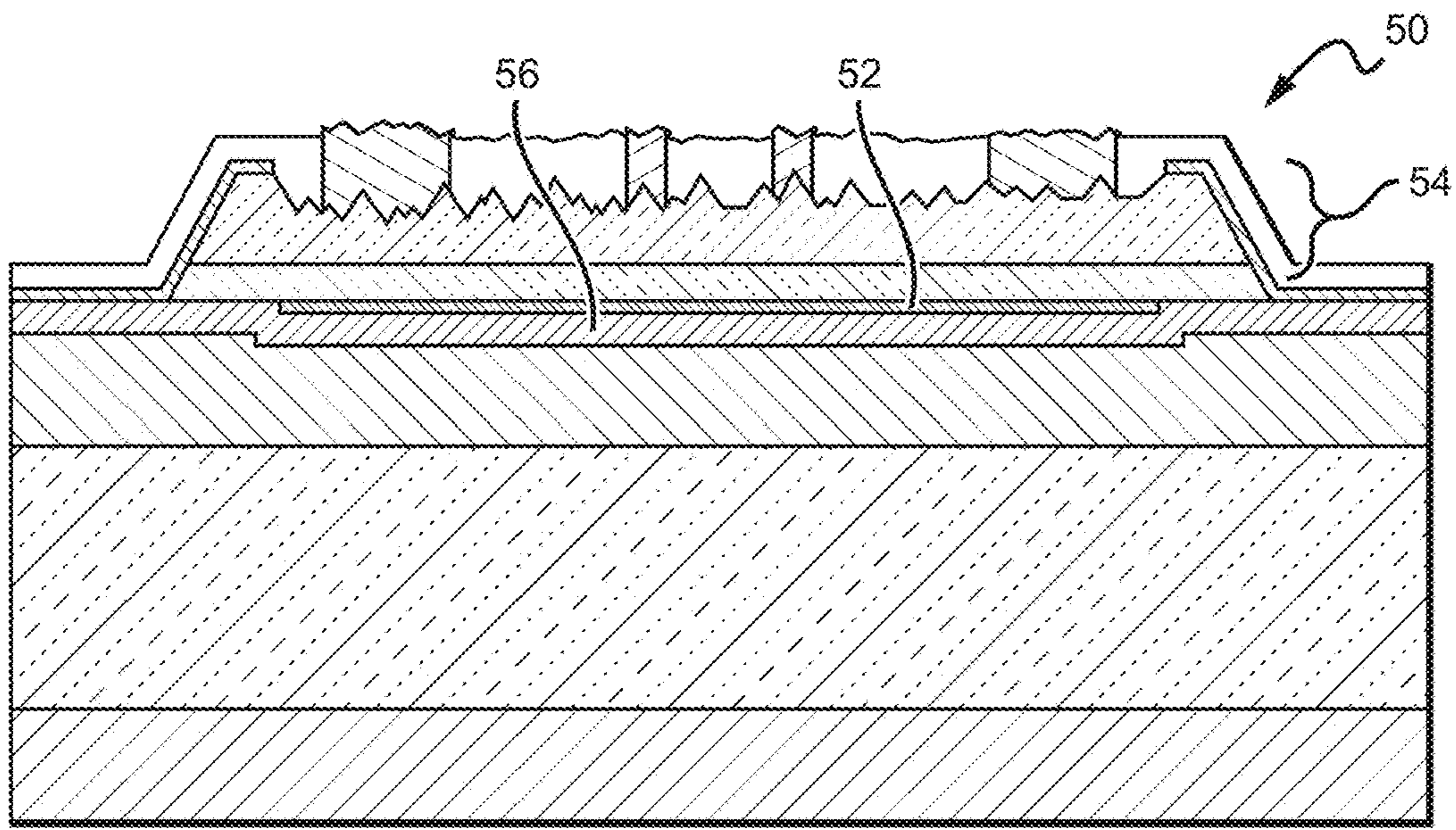
FIG. 5 PRIOR ART
