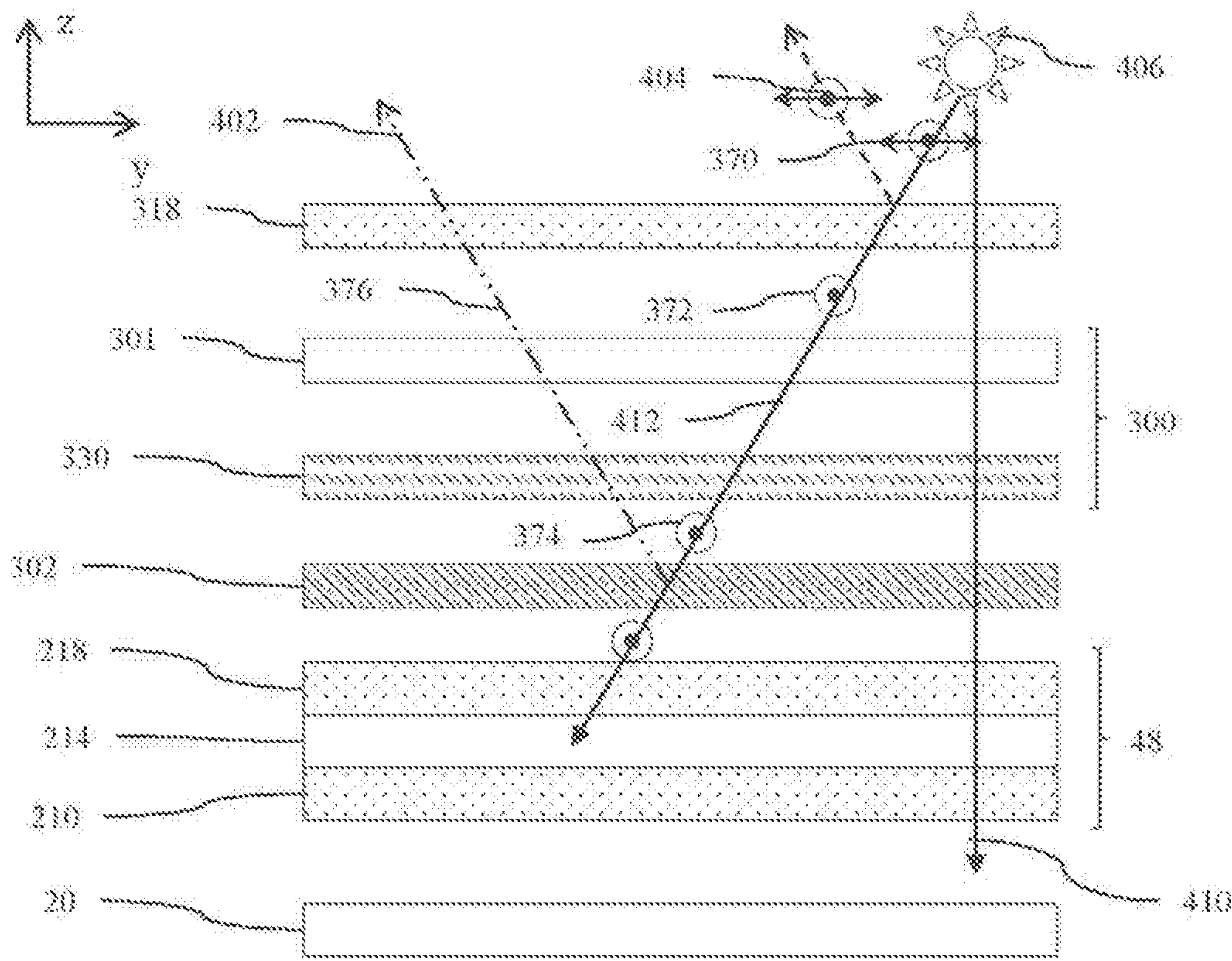
FIG. 17A Reflectivity
