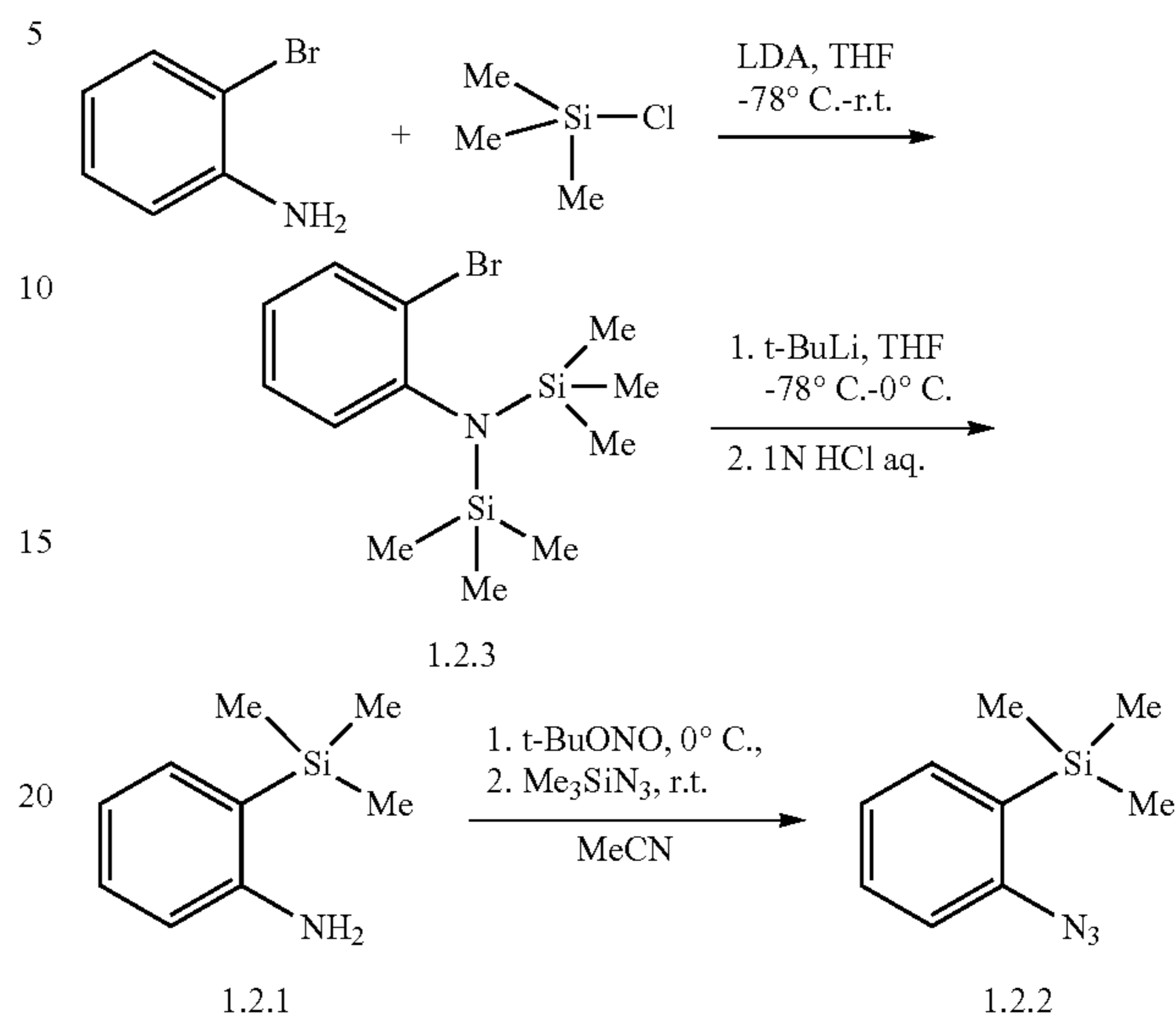
Scheme s2. Synthesis of ortho-silyl substituted aryl azide.
