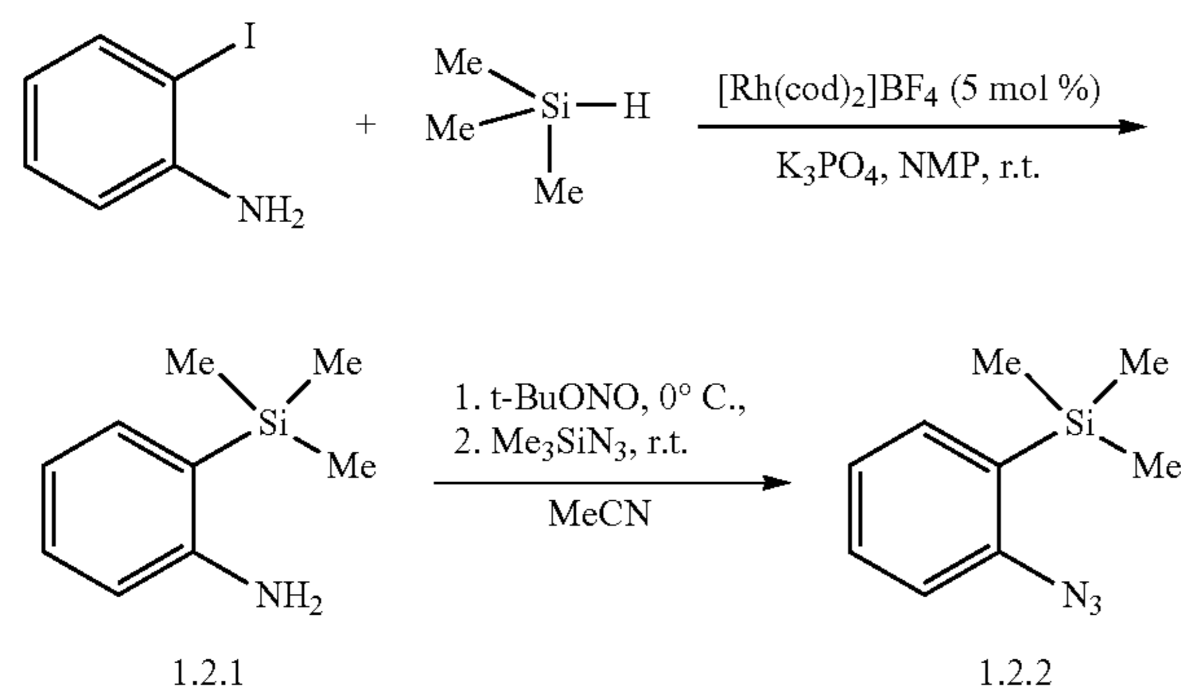
Scheme s1. Synthesis of ortho-silyl substituted aryl azide.
