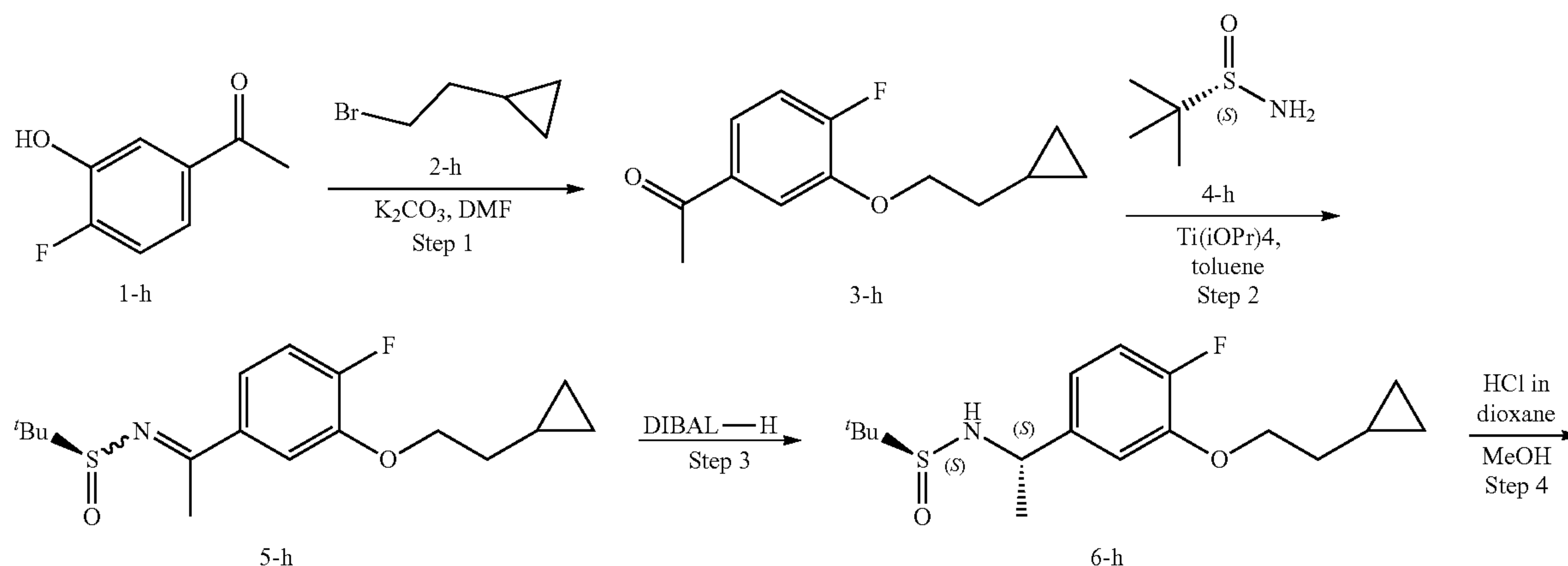
Scheme 8.
