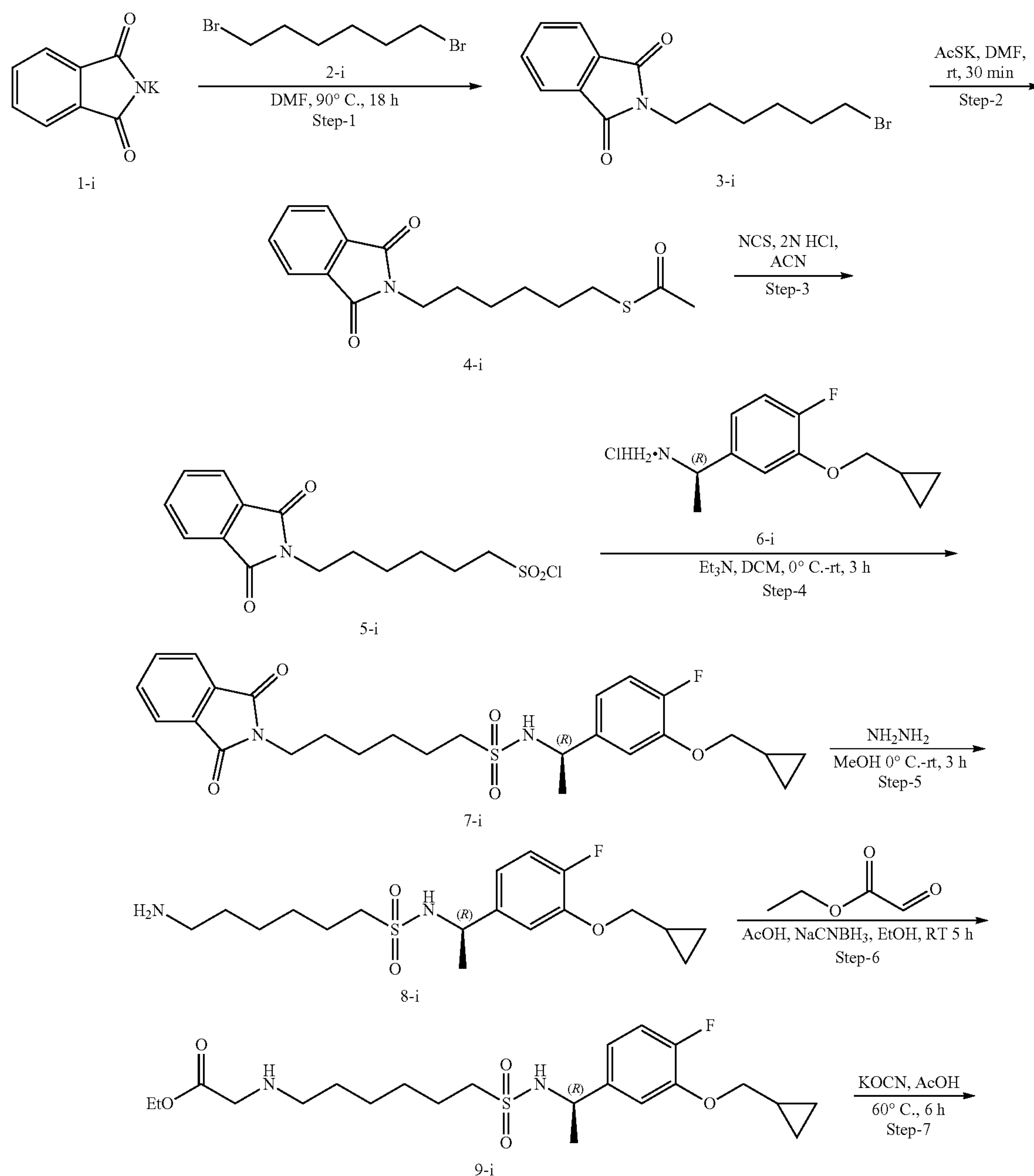
Scheme 10.
