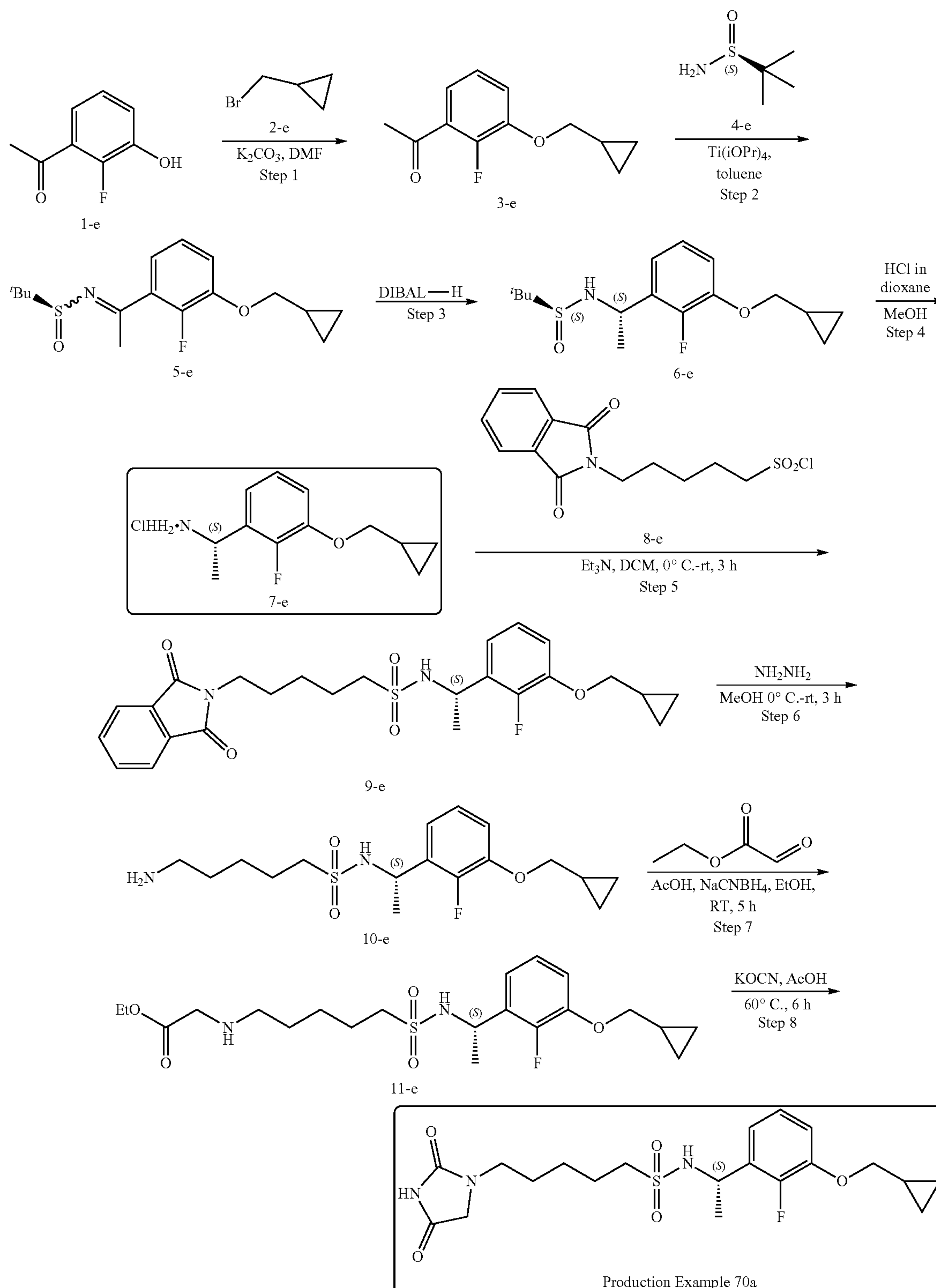
Scheme 5.
