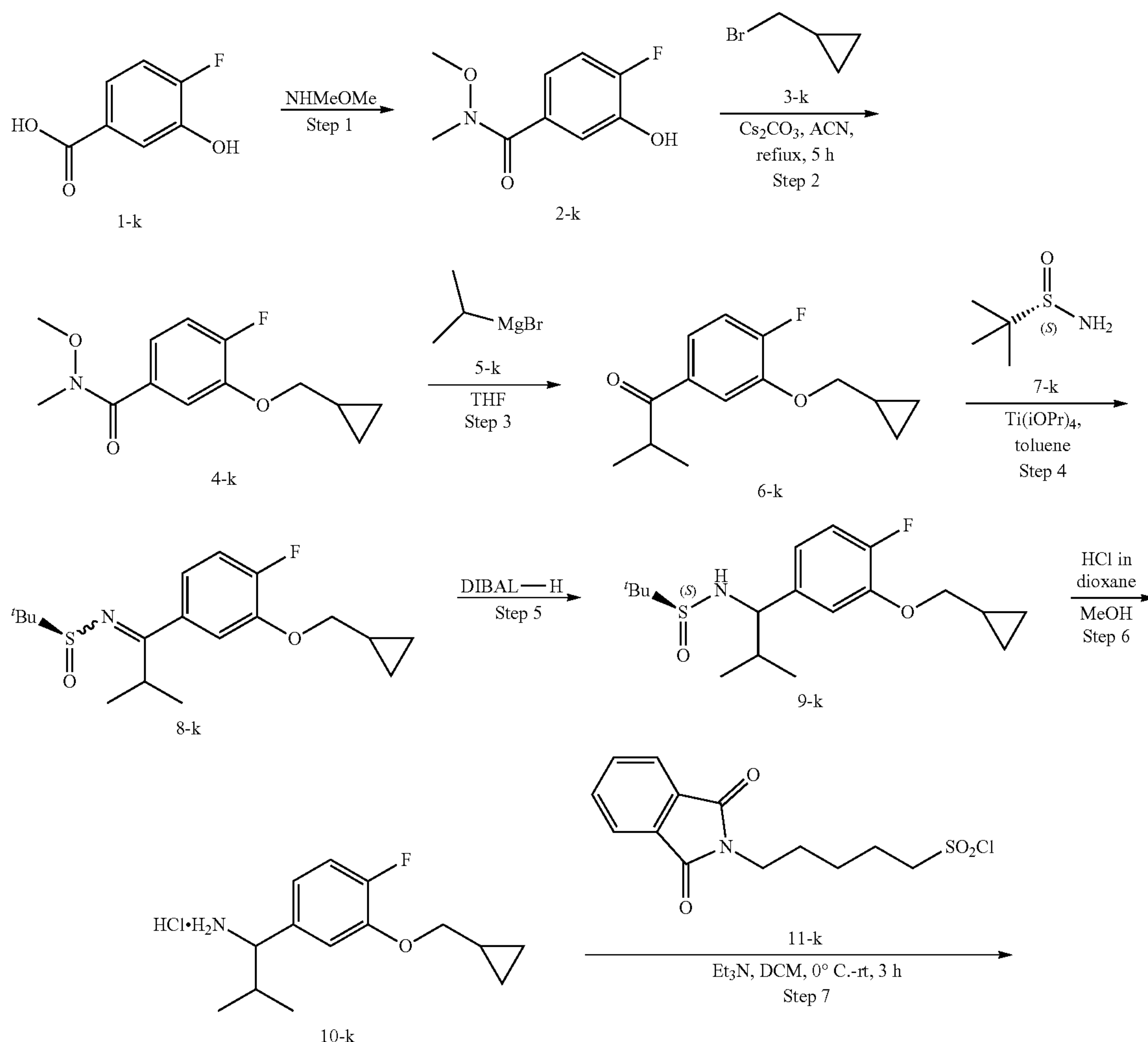
Scheme 12.
