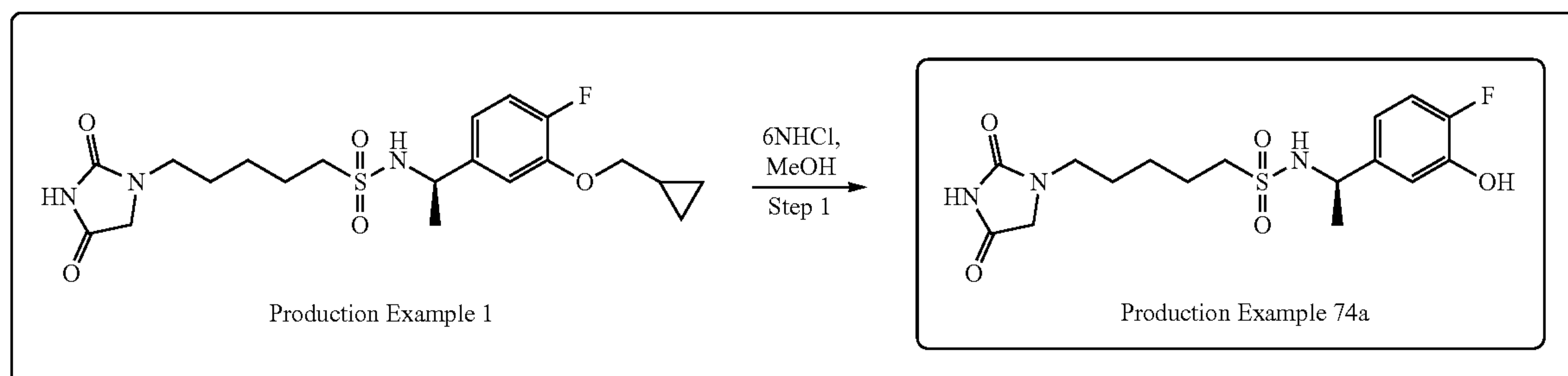
Scheme 9.
