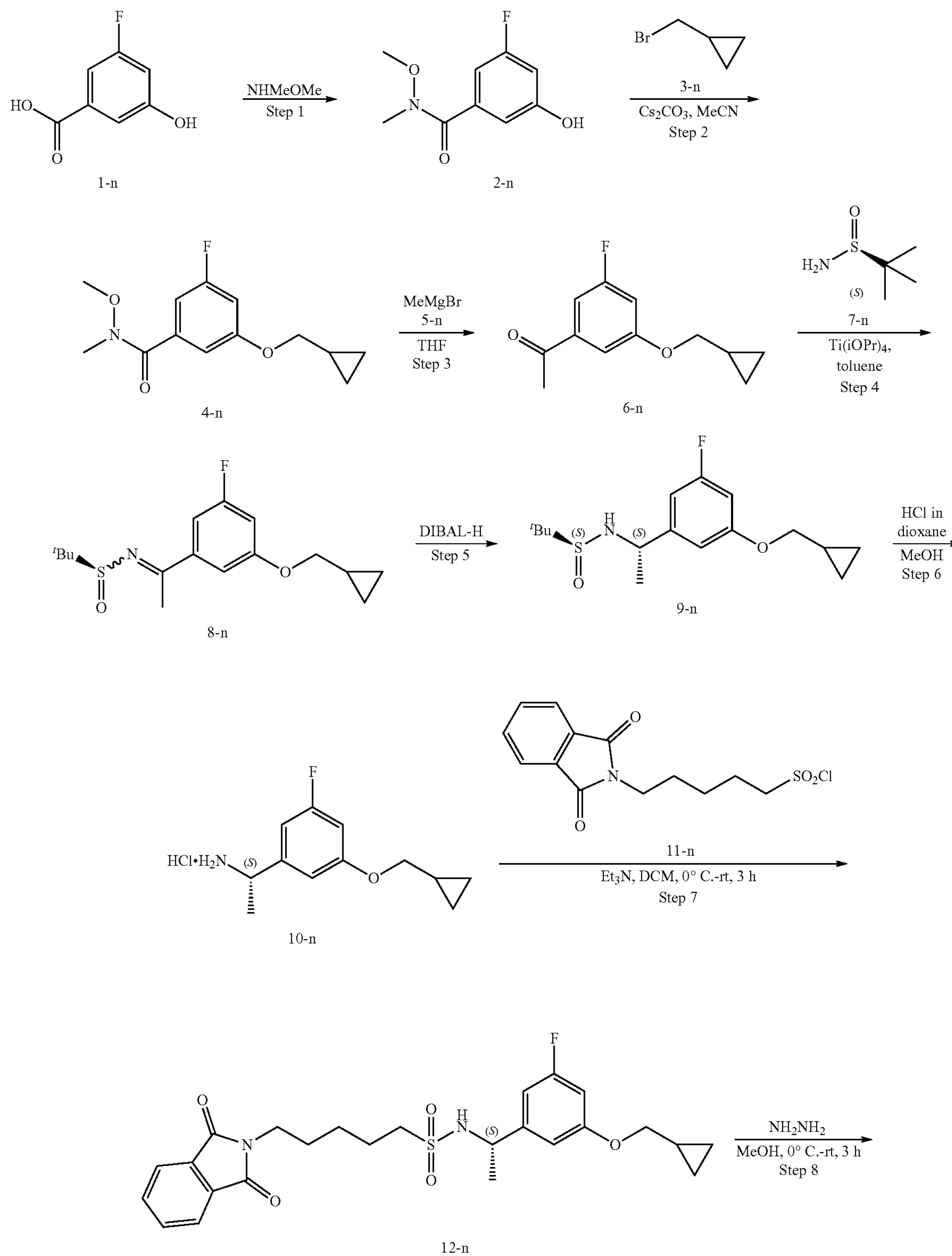
Scheme 15.
