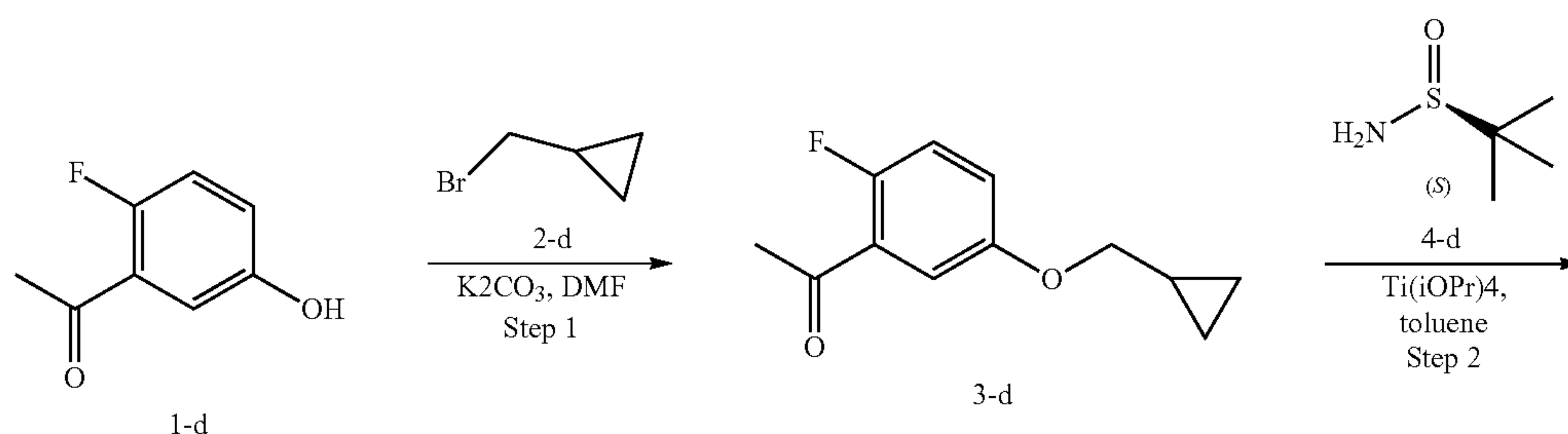
Scheme 4.
