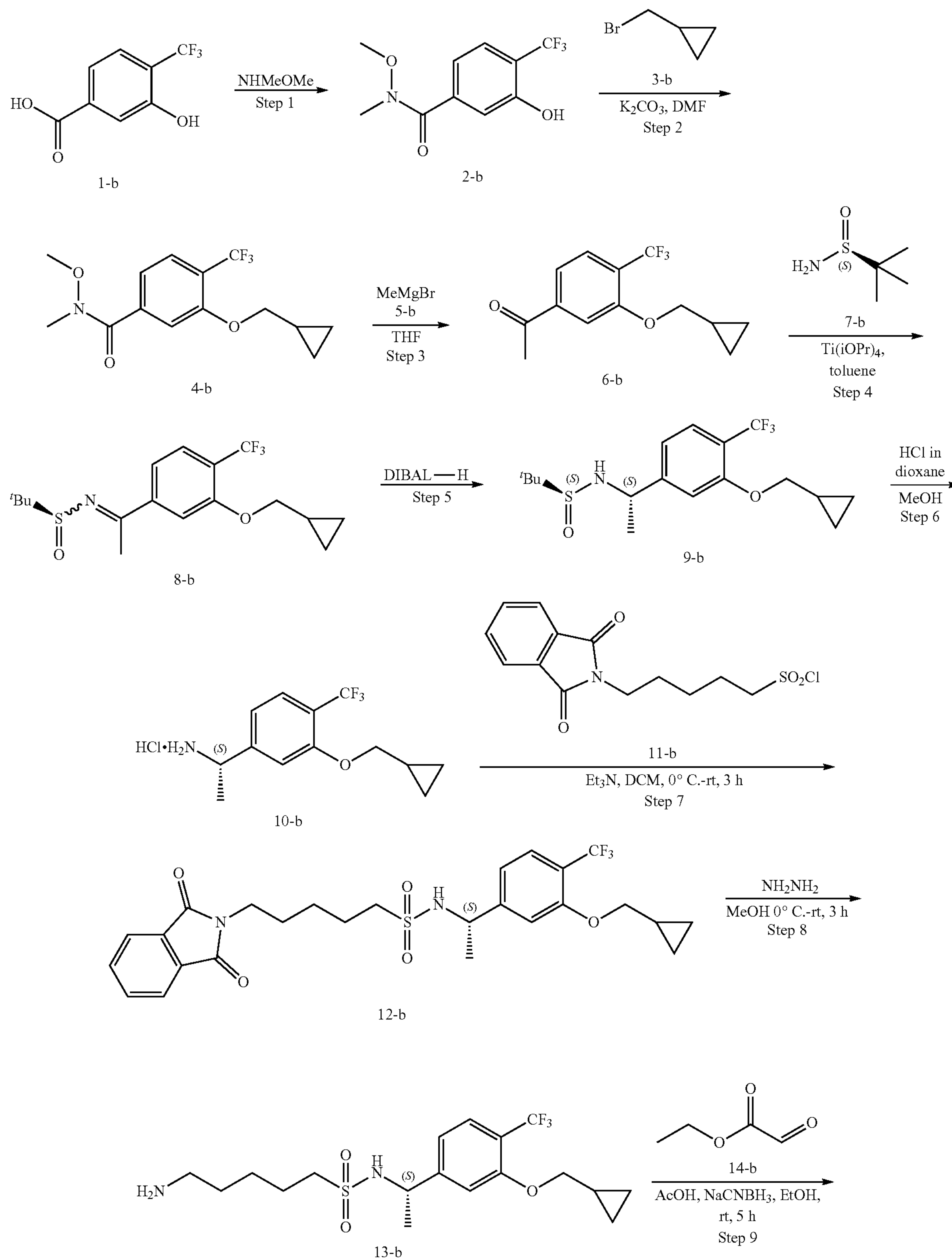
Scheme 2.
