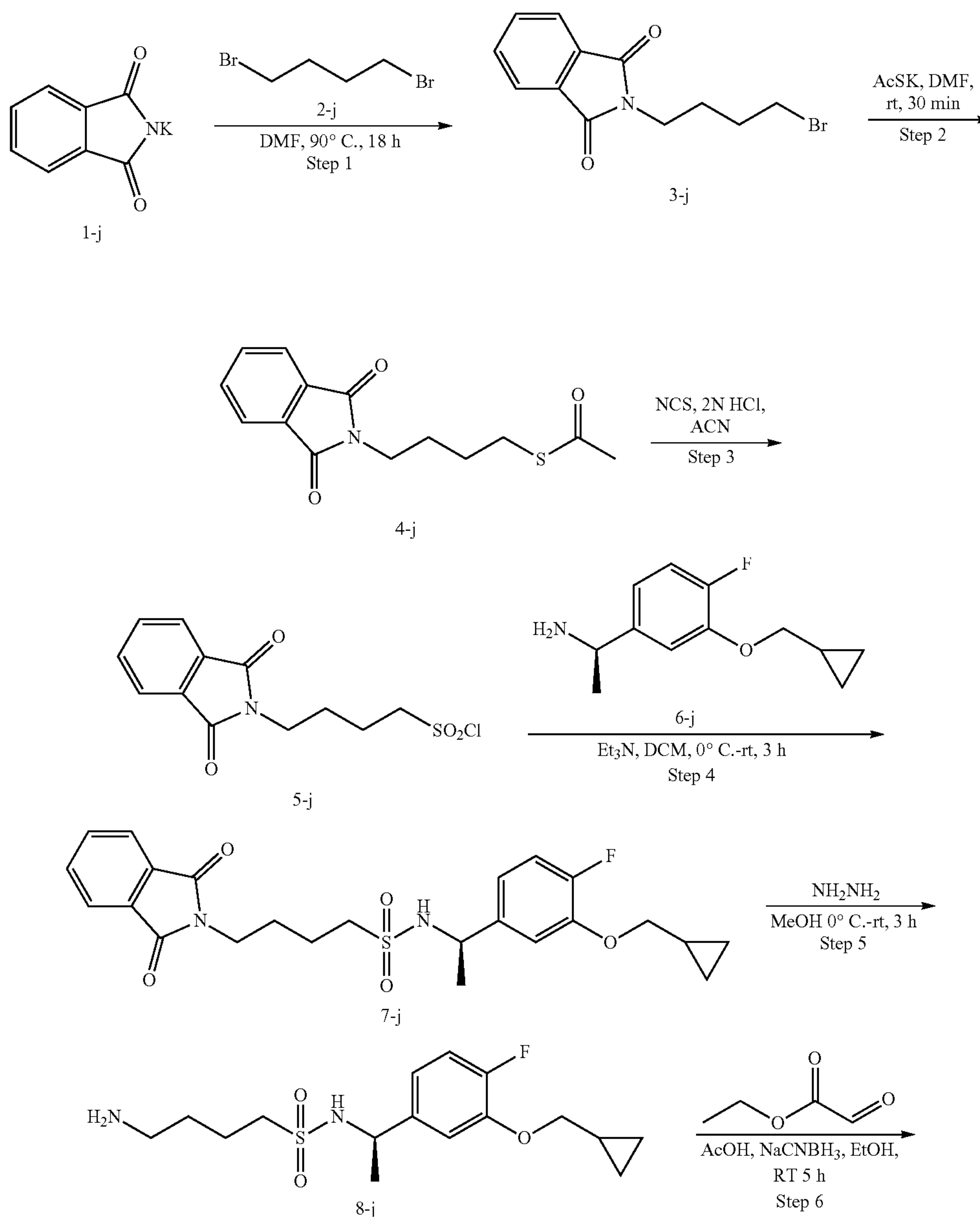
Scheme 11.
