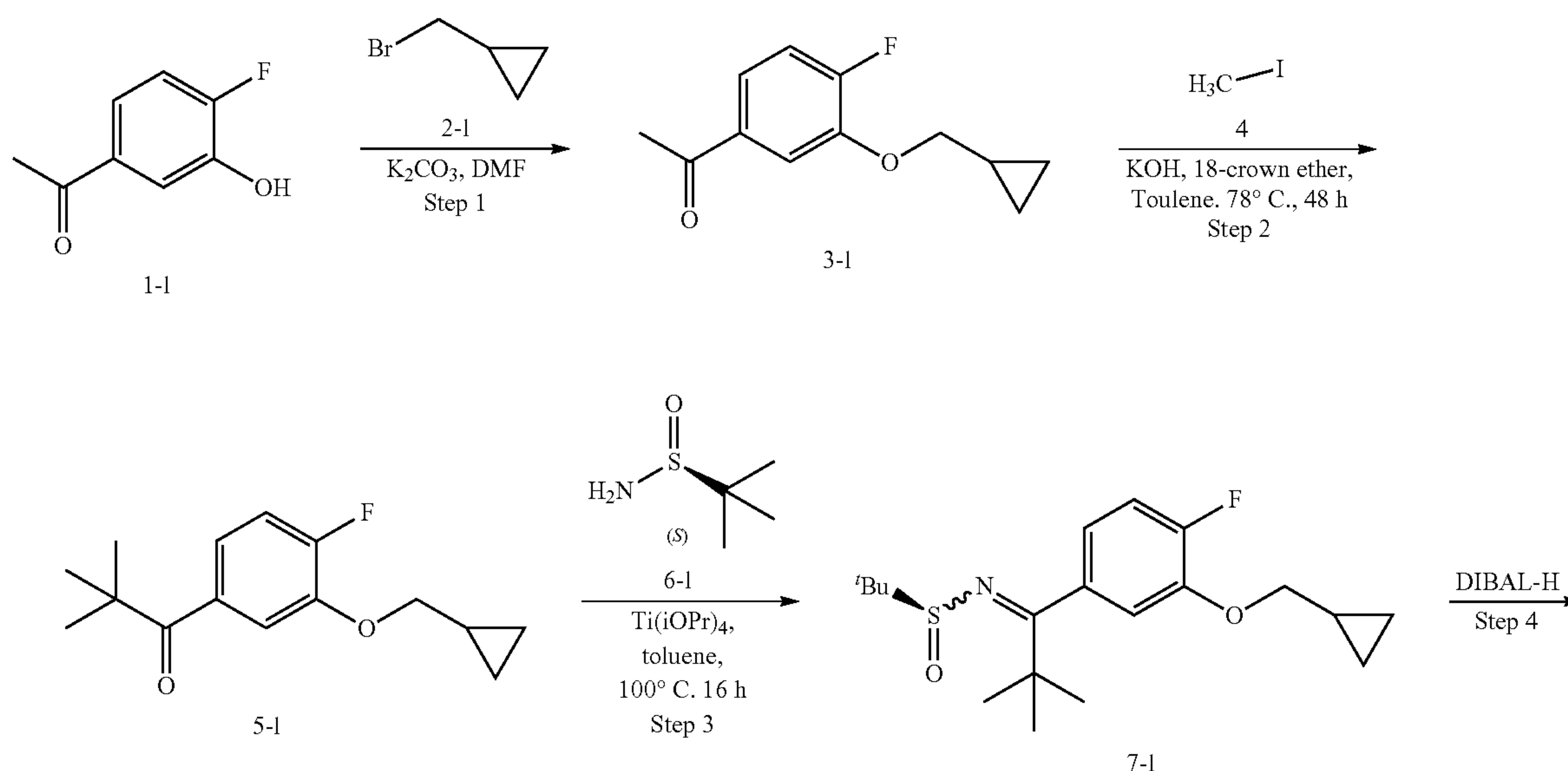
Scheme 13.
