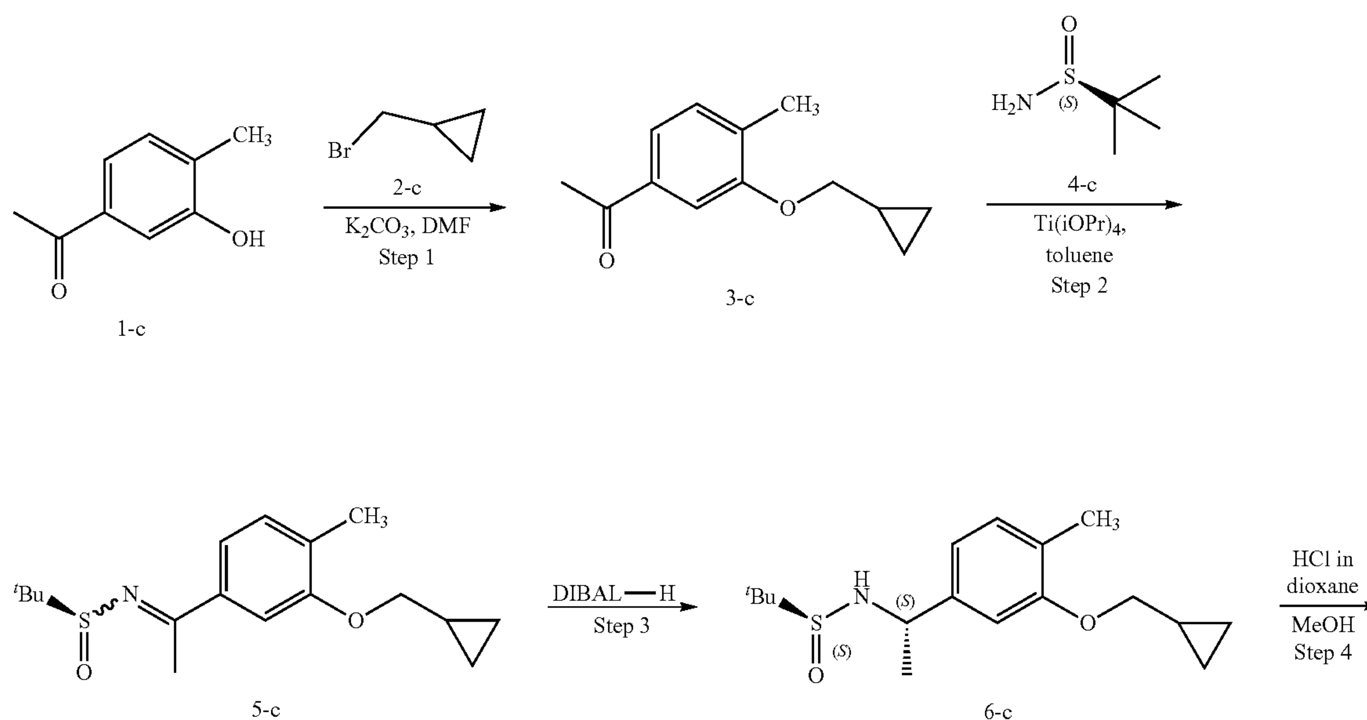
Scheme 3.
