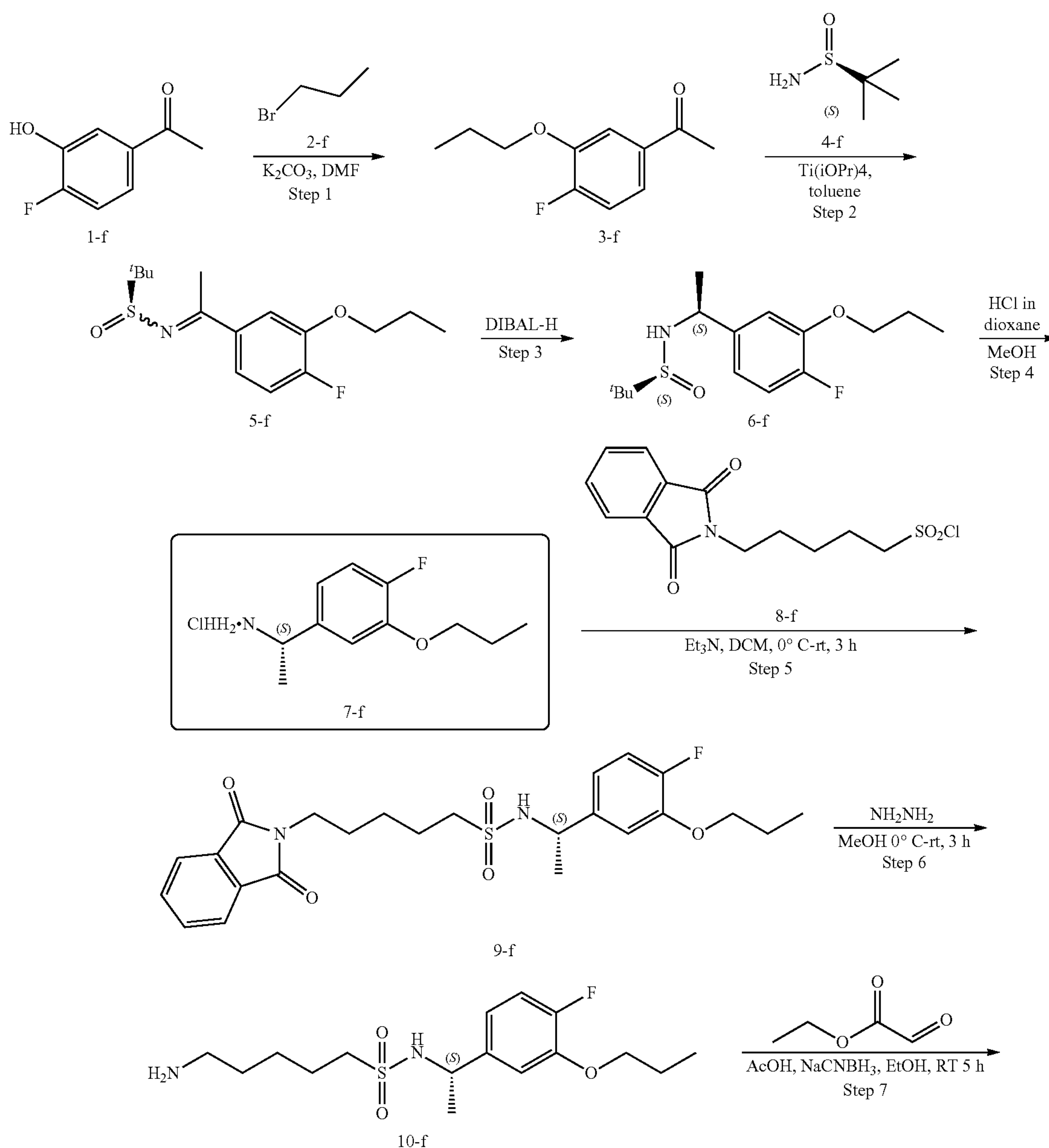
Scheme 6.
