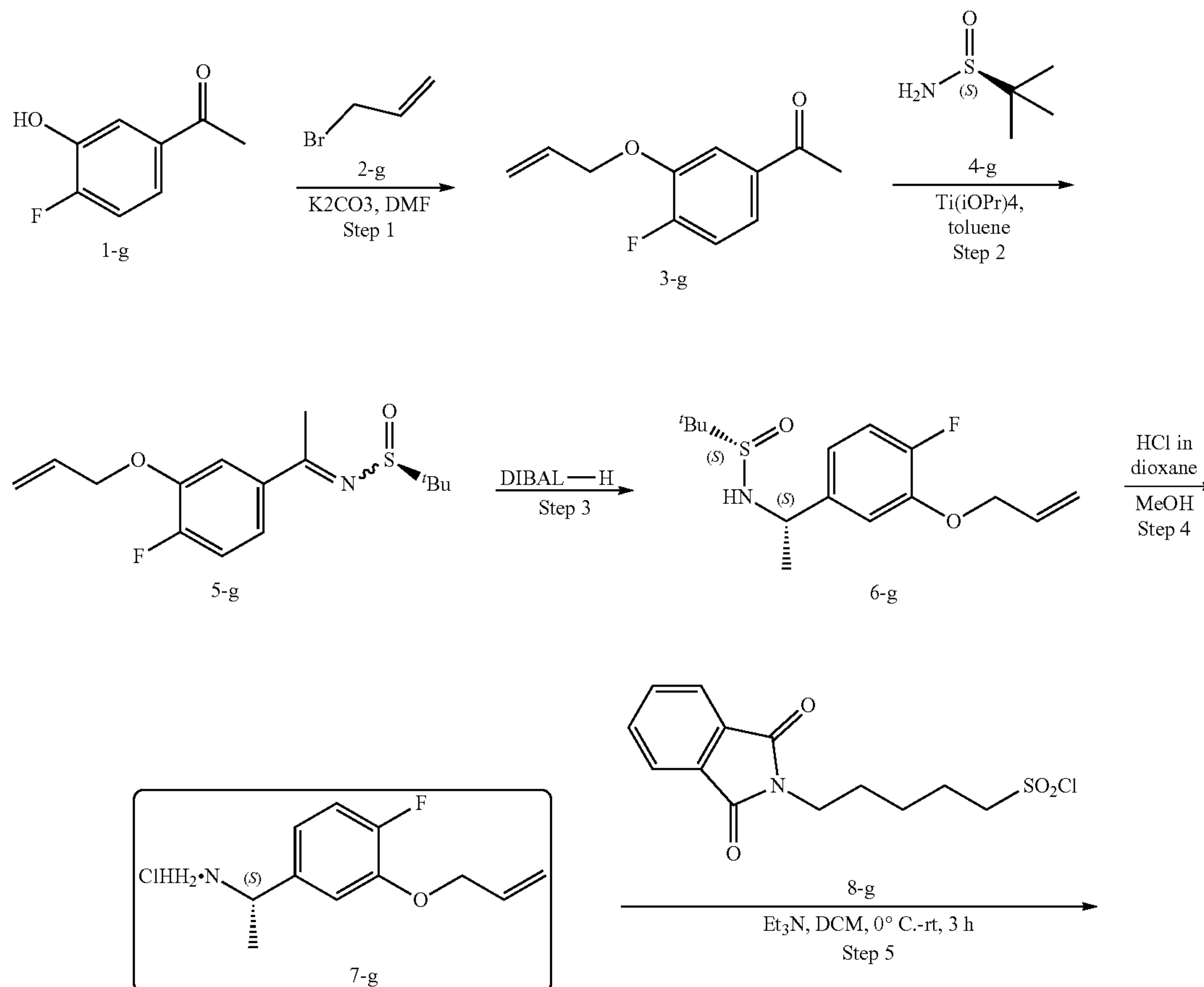
Scheme 7.
