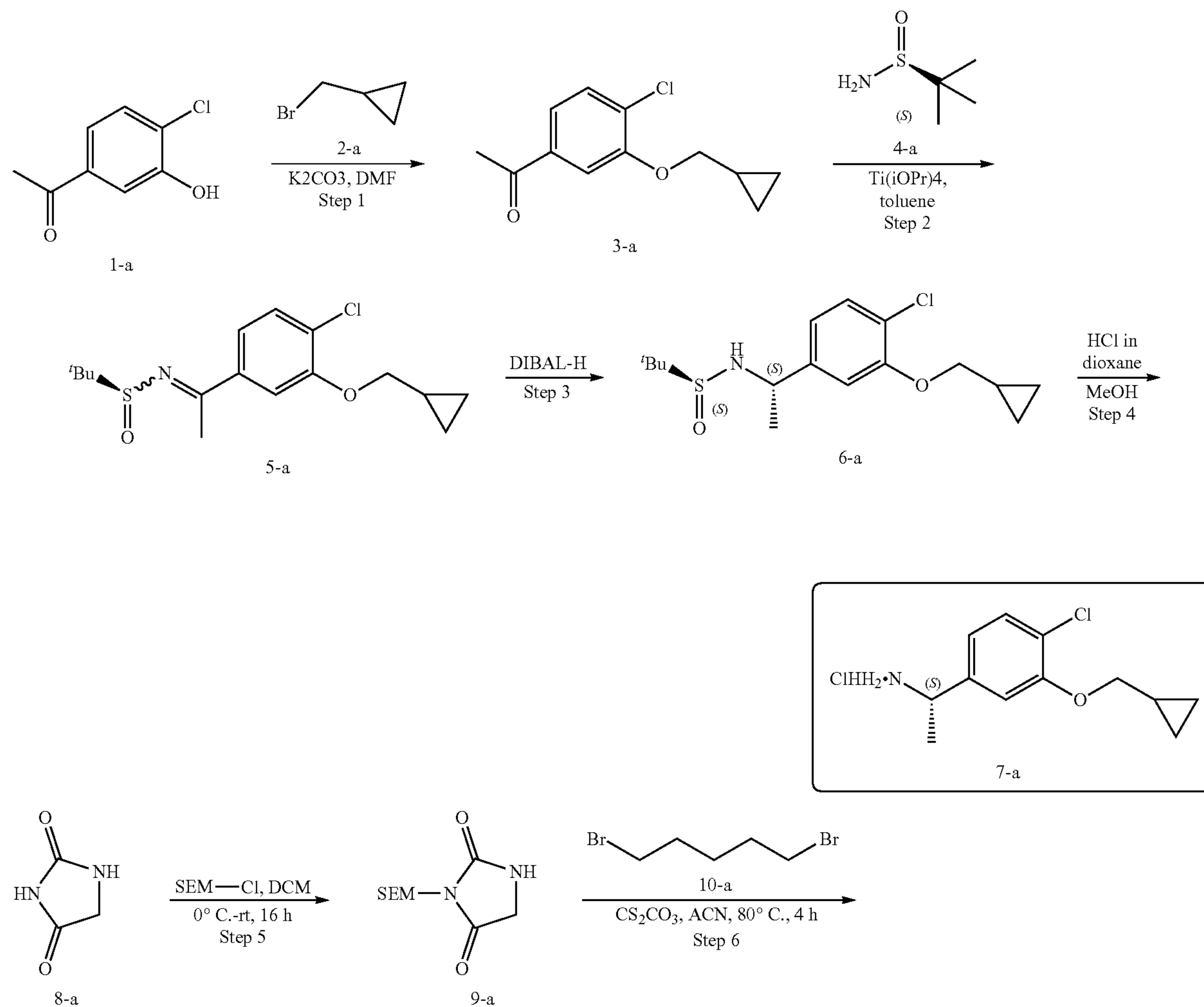
Scheme 1.
